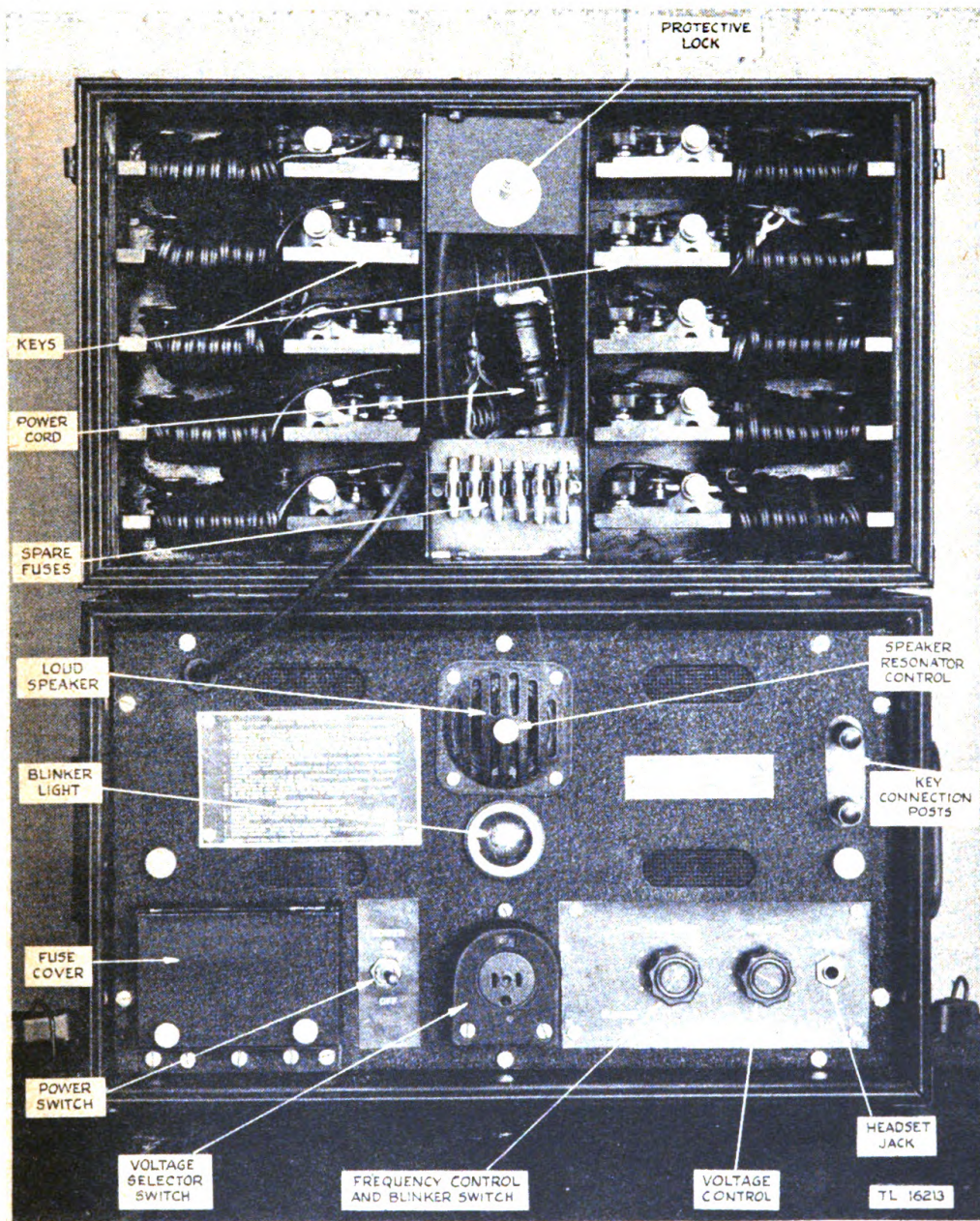
Fig. 3 Code Training Set AN/GSC-T1, front view
