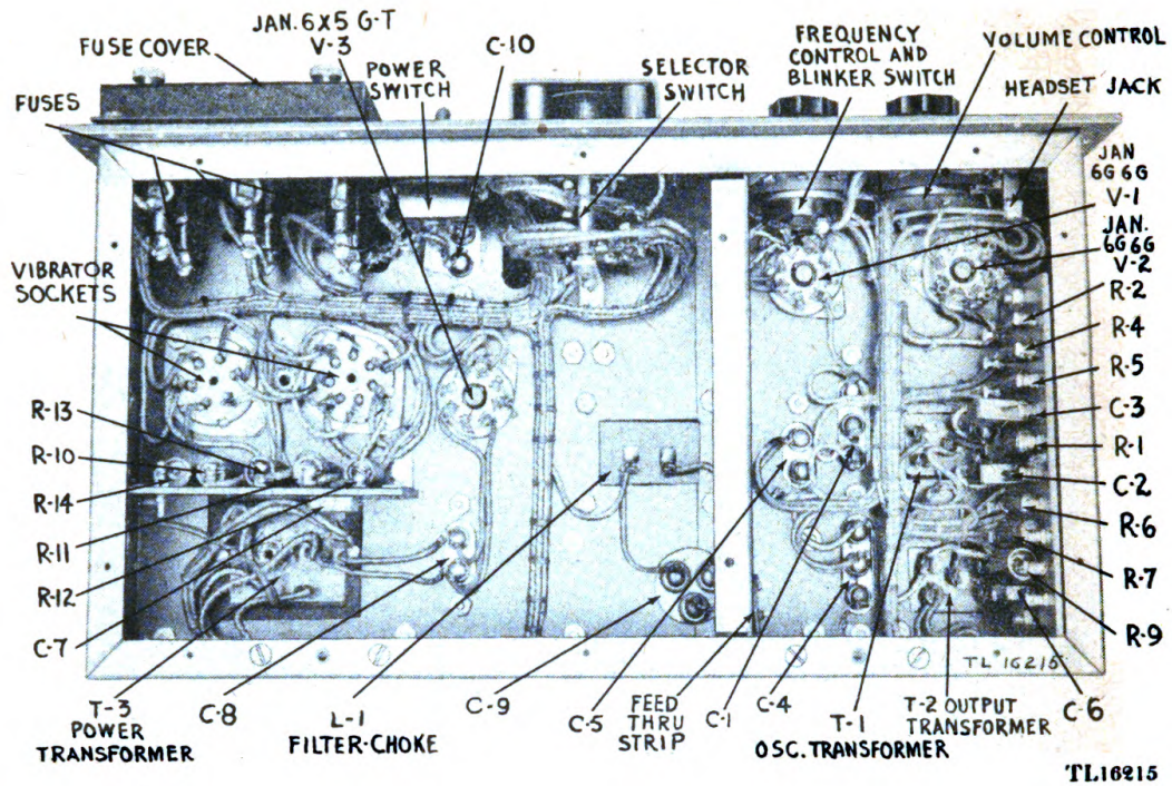
Fig. 5 Code Training Set AN/GSC-T1, bottom view.
