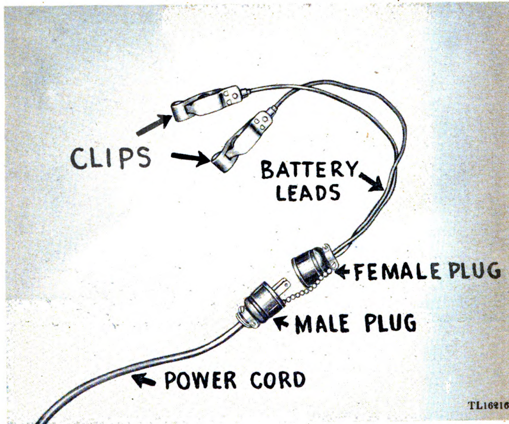
Fig. 6 Power cord and battery leads.
