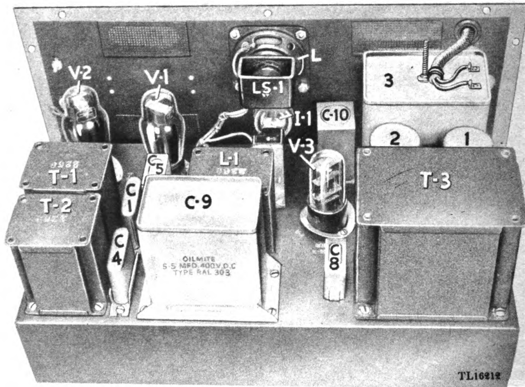
Fig. 2 Code Training Set AN/GSC-T1, top internal view.
