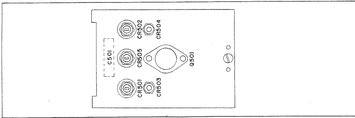
Figure 3-7. Component Locations: Heat Sink Bracket
