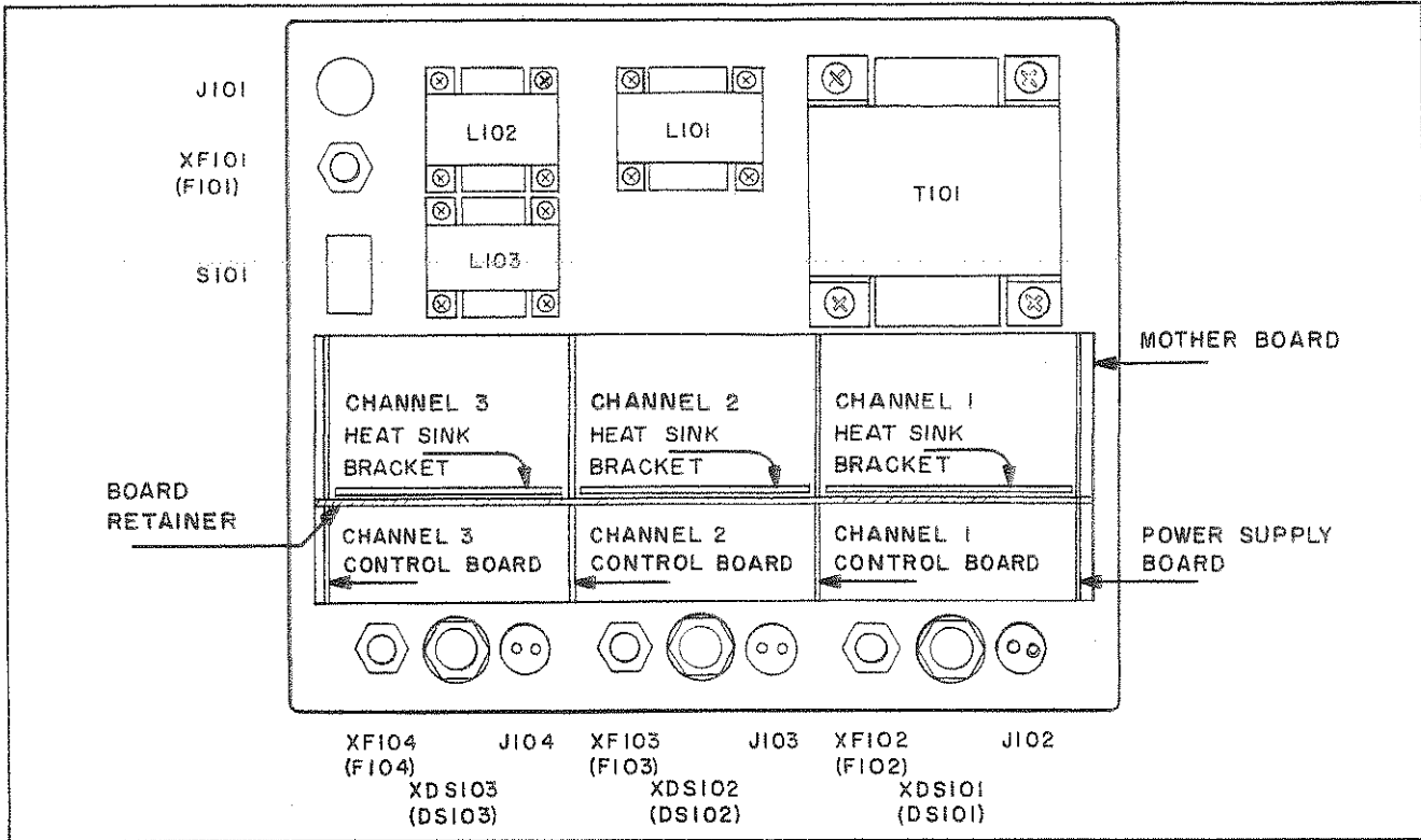
Figure 3-2. Component Locations: Rear of Front Panel
