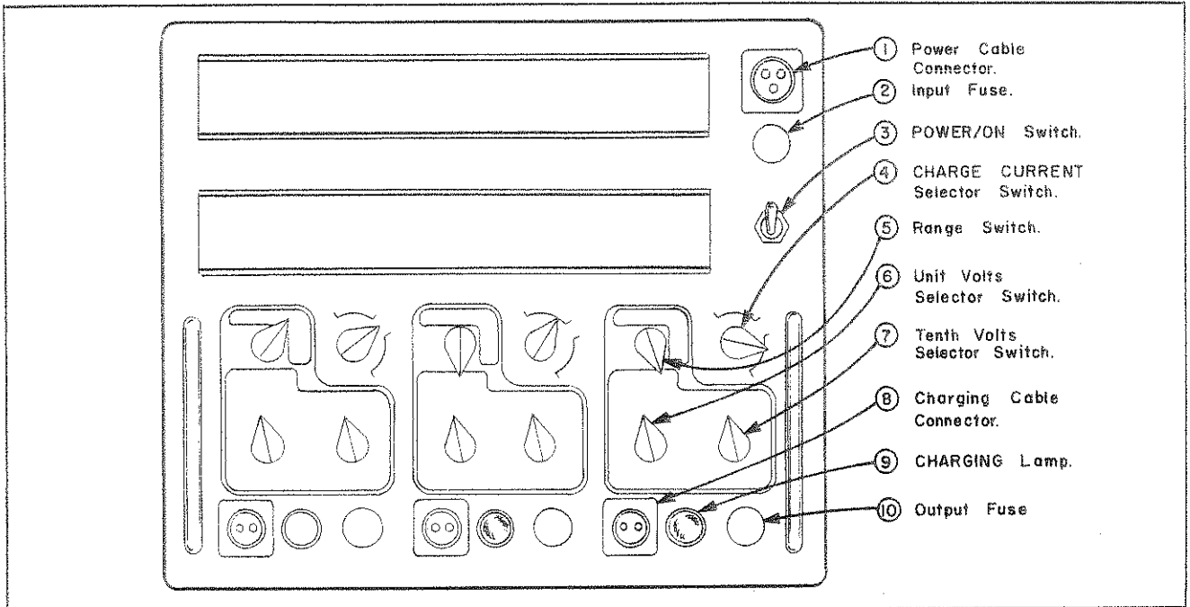
Figure 2-1. Operator Control and Indicator Locations
