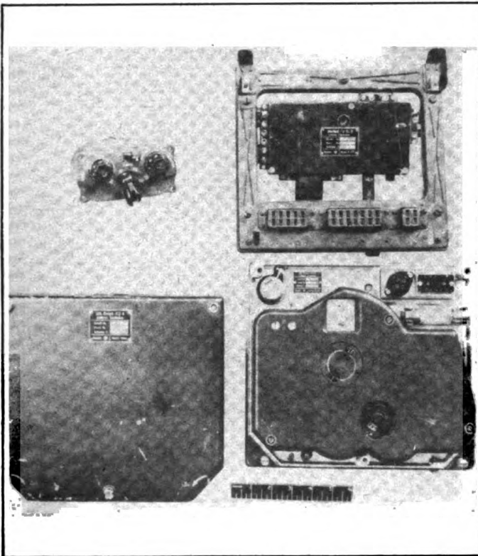
PEIL G 4 - RECEIVER EZ 4, COMPLETE.
