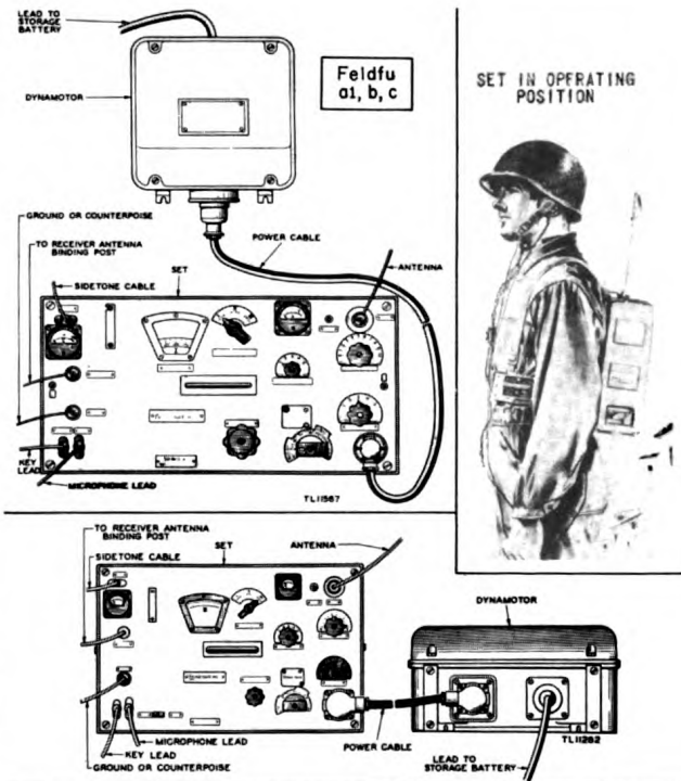
ENGINEER'S DRAWINGS OF COMPONENTS, SHOWING INTERCONNECTIONS.
