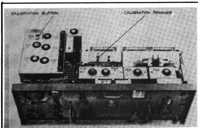
RECEIVER WITH COVER REMOVED
