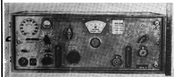
Kw. E. a (GROUND RECEIVER) FRONT VIEW.
