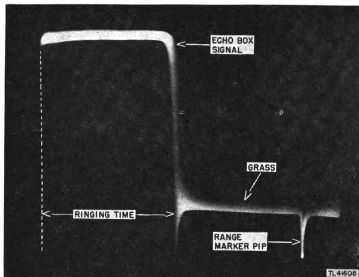
Figure 3. Echo box signal on A-scope.
