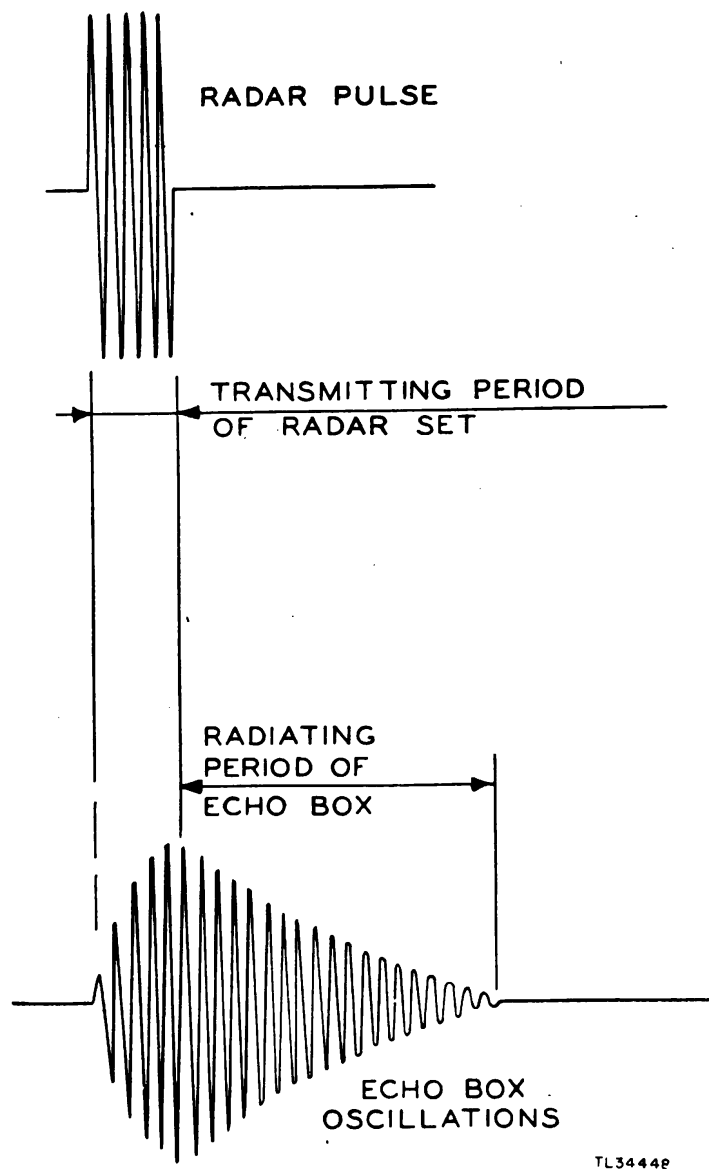
Figure 8. Echo box oscillations.
