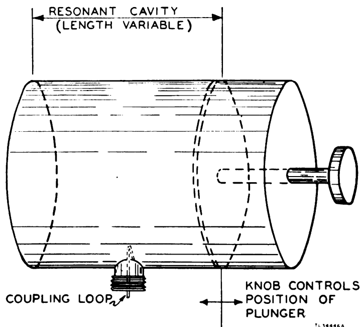
Figure 6. Outline drawing of echo box.
