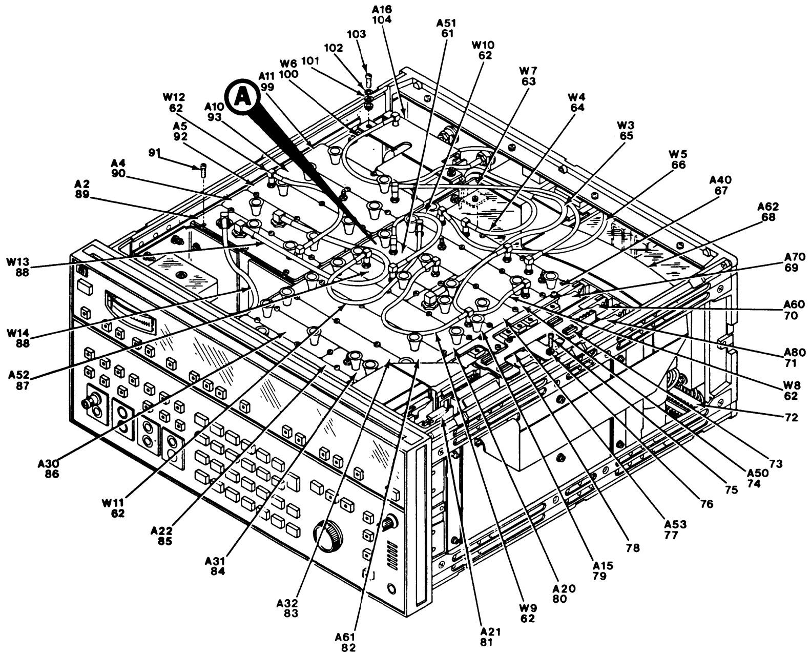
Figure 1. Frequency Selective Level Meter, AN/USM-490 (Sheet 4 of 11).
