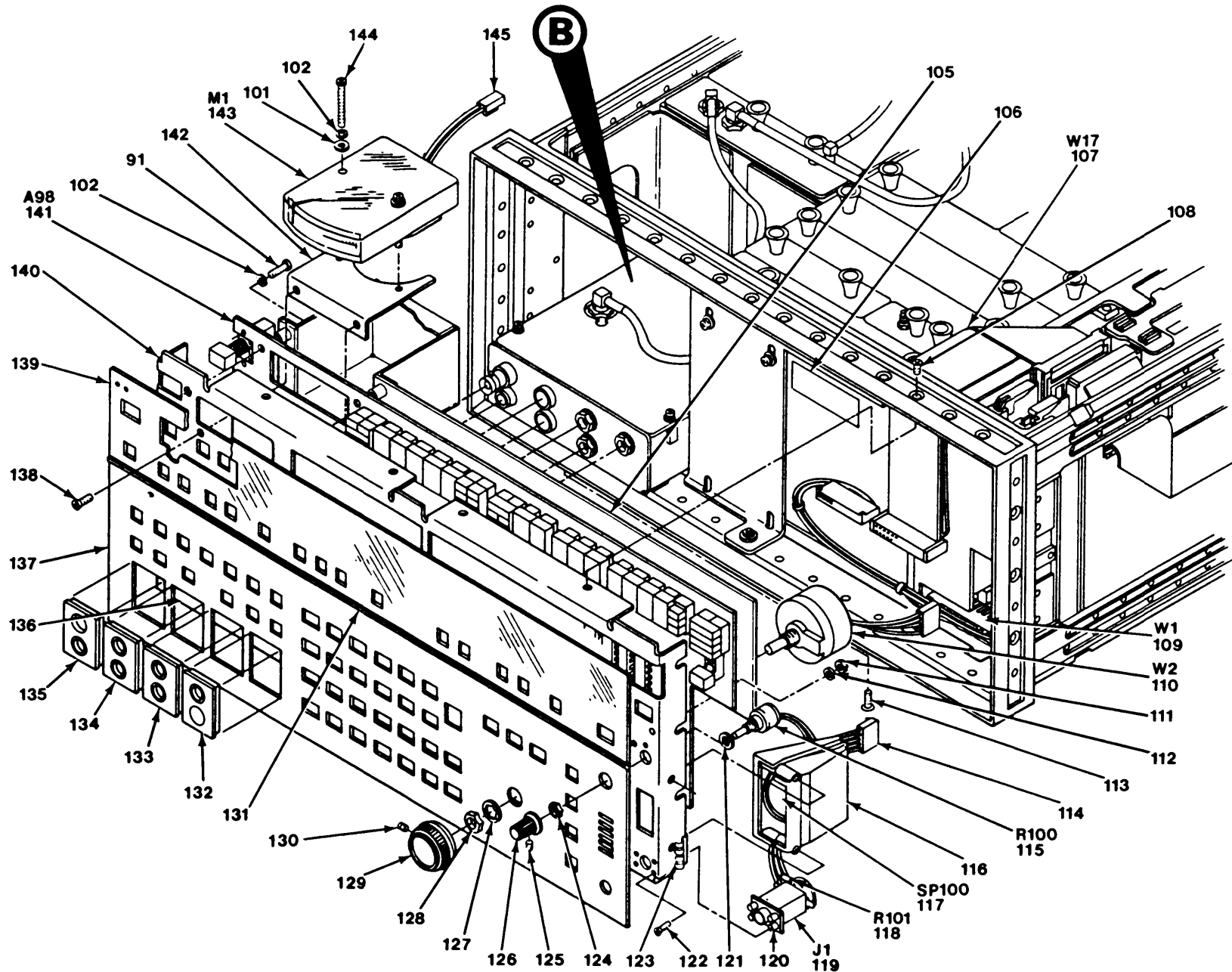
Figure 1. Frequency Selective Level Meter, AN/USM-490 (Sheet 6 of 11).
