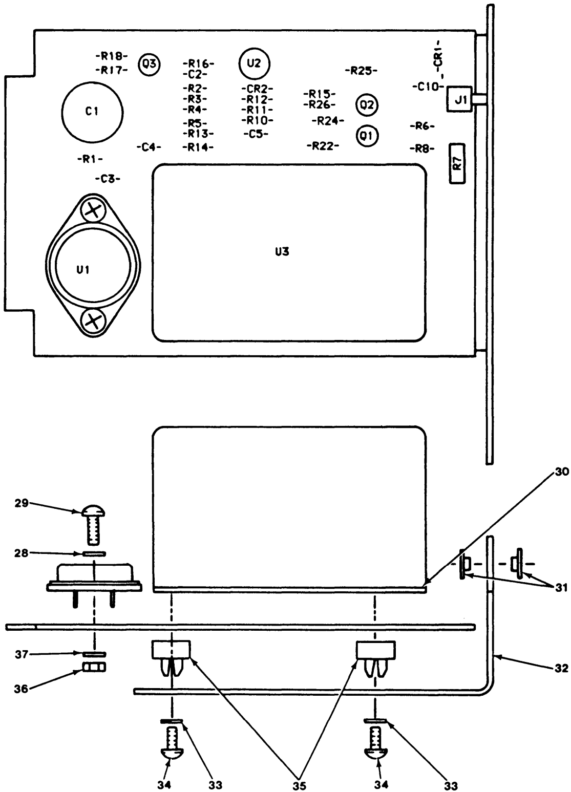
Figure 9. 10 MHz Frequency REF Circuit Card Assembly (Sheet 1 of 2).
