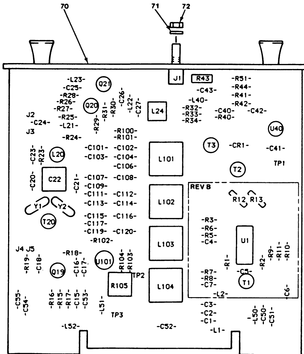
Figure 6. Second Mixer Circuit Card Assembly (Sheet 1 of 2).
