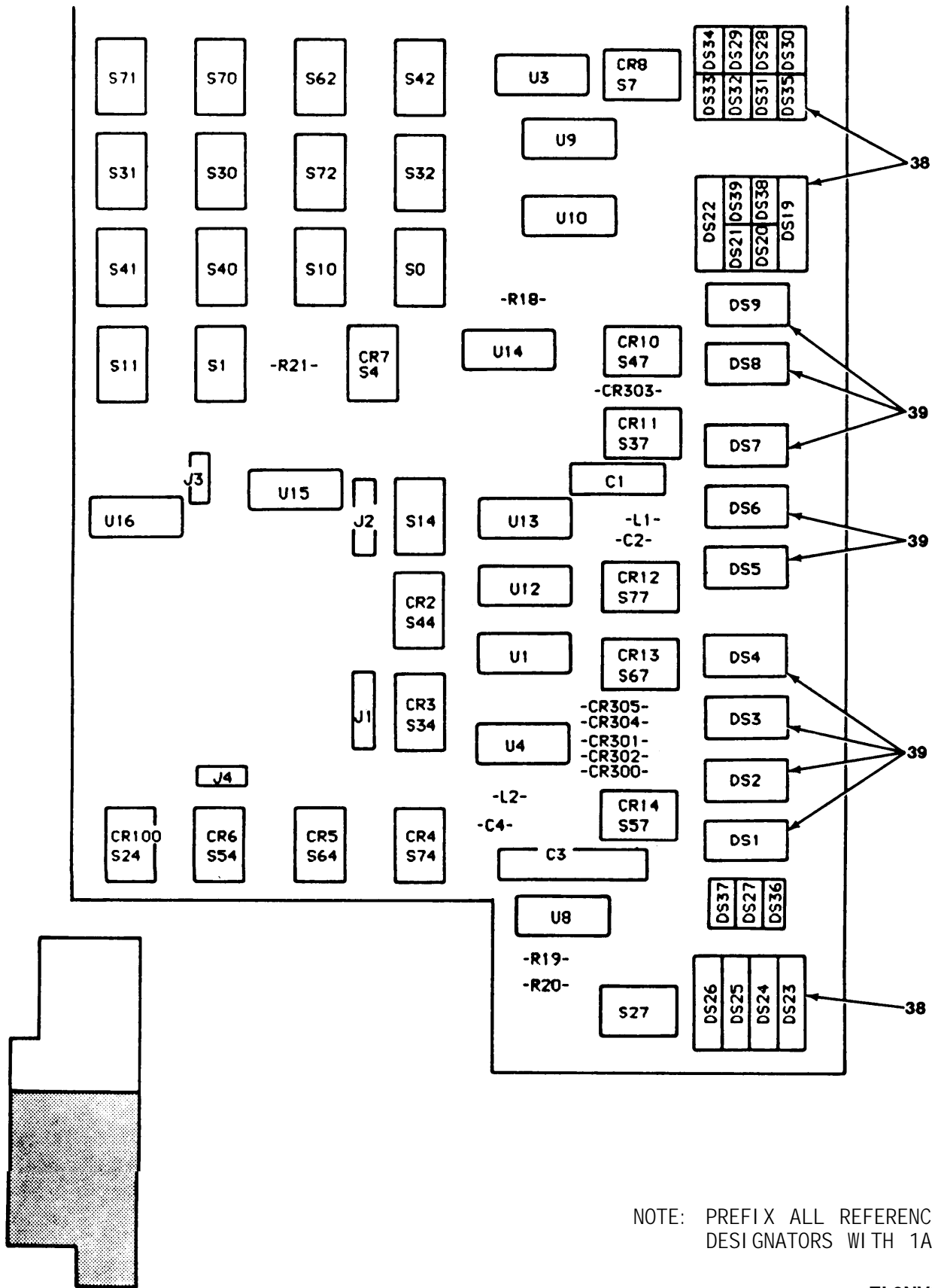
Figure 17. Switch/Display Circuit Card Assembly (Sheet 2 of 3).
