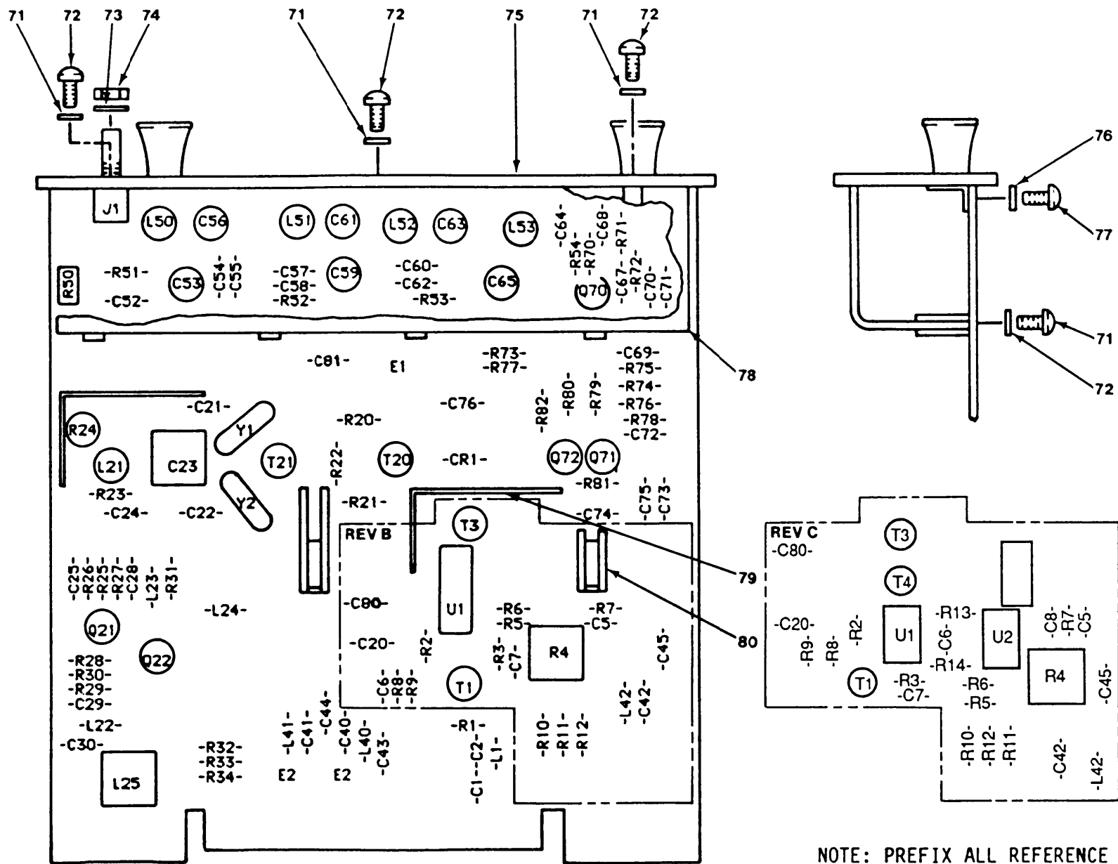
Figure 5. Input Mixer Circuit Card Assembly (Sheet 1 of 2).
