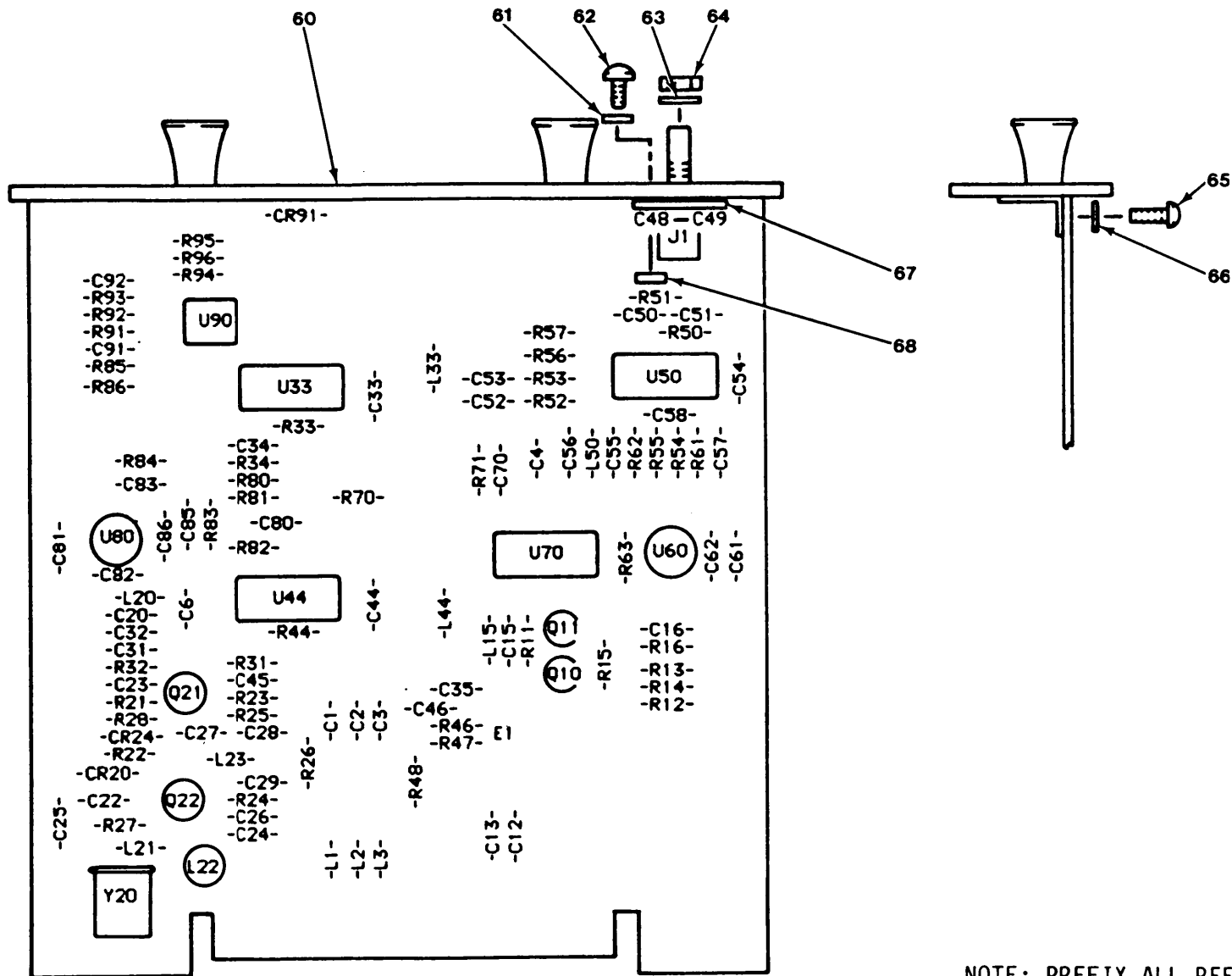
Figure 7. Second LO Circuit Card Assembly (Sheet 1 of 2).
