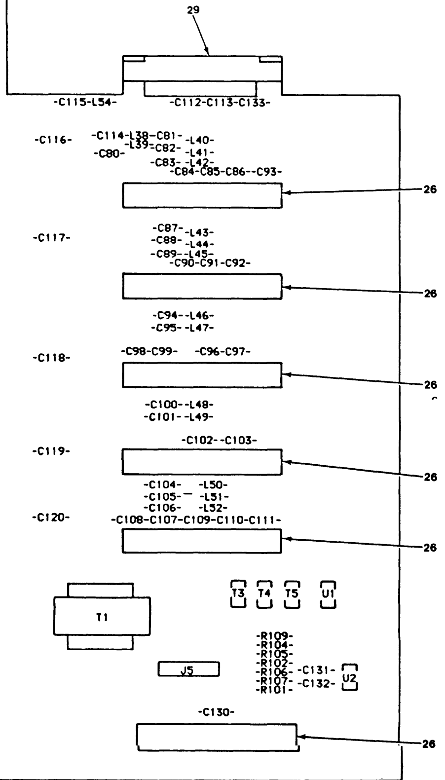
Figure 18. Motherboard Circuit Card Assembly (Sheet 4 of 5).
