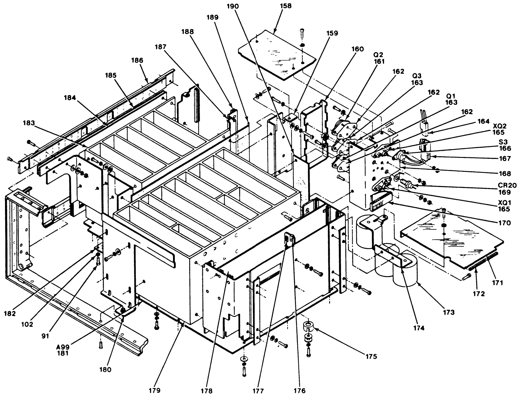
Figure 1. Frequency Selective Level Meter, AN/USM-490 (Sheet 8 of 11).
