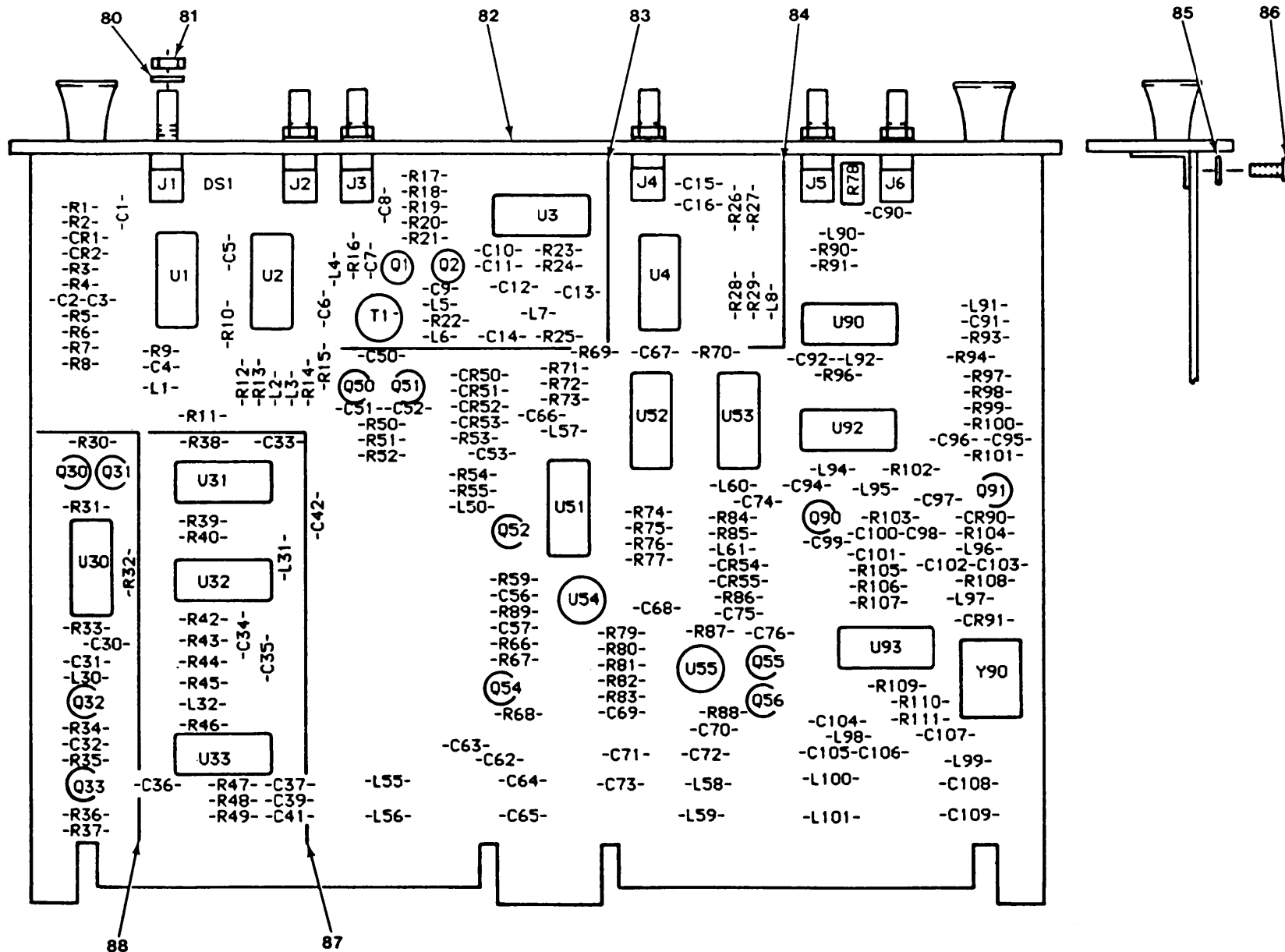
Figure 13. Frequency Reference Circuit Card Assembly (Sheet 1 of 2).
