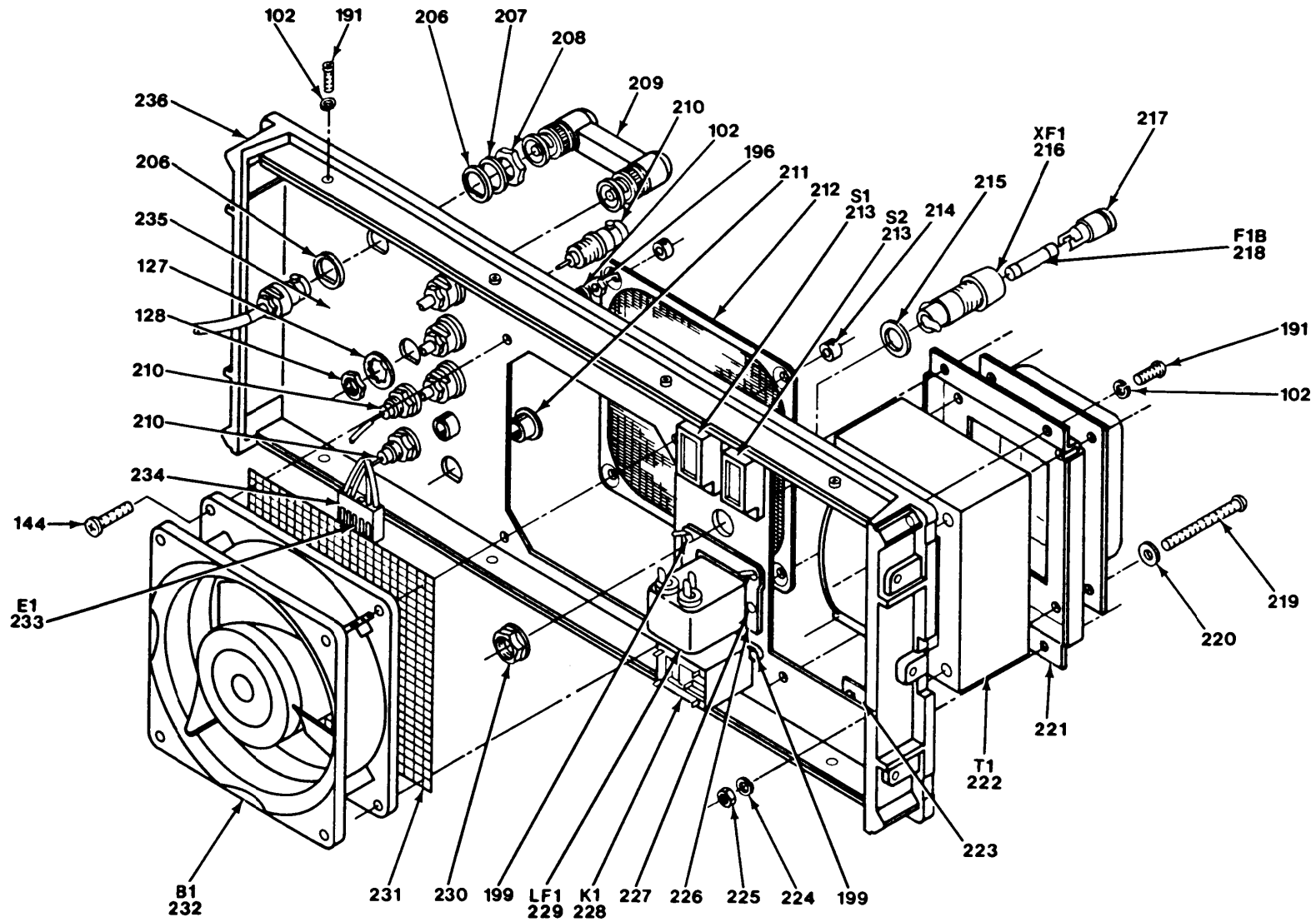
Figure 1. Frequency Selective Level Meter, AN/USM-490 (Sheet 10 of 11).
