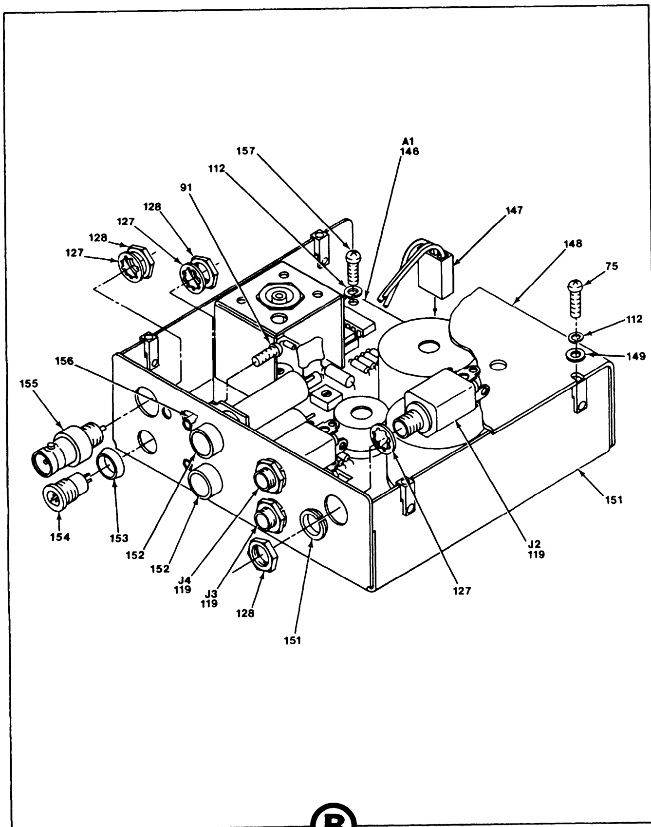
Figure 1. Frequency Selective Level Meter, AN/USM-490 (Sheet 7 of 11).
