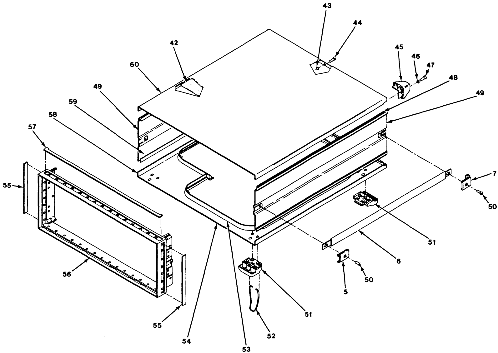
Figure 1. Frequency Selective Level Meter, AN/USM-490 (Sheet 3 of 11).
