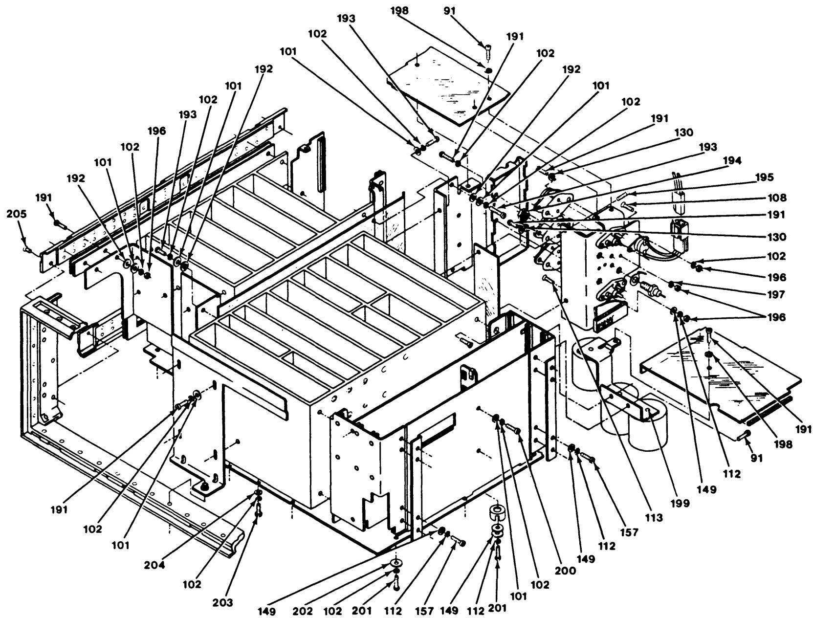
Figure 1. Frequency Selective Level Meter, AN/USM-490 (Sheet 9 of 11).
