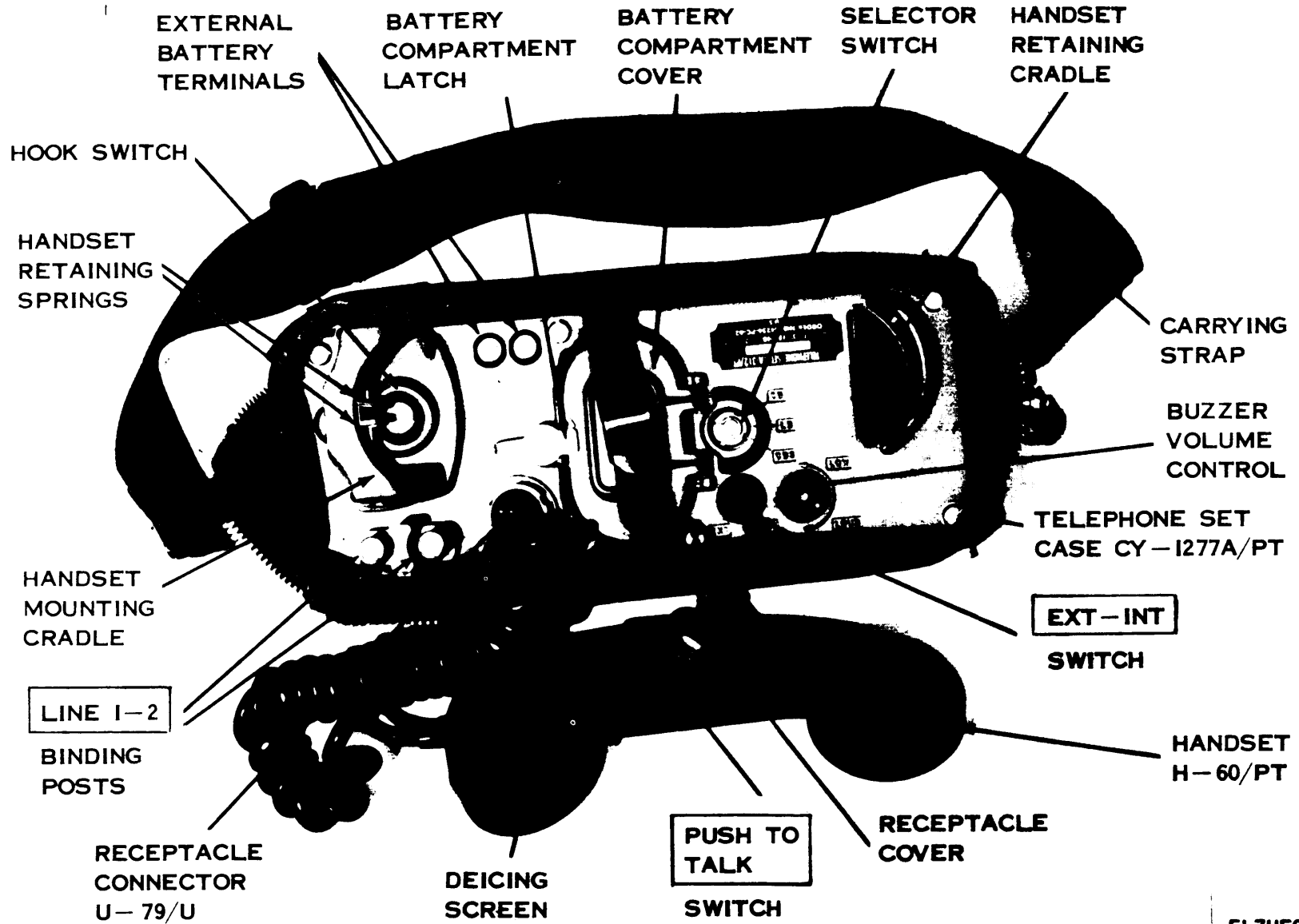
■ Figure 1-16. Telephone Set TA-512/PT.
