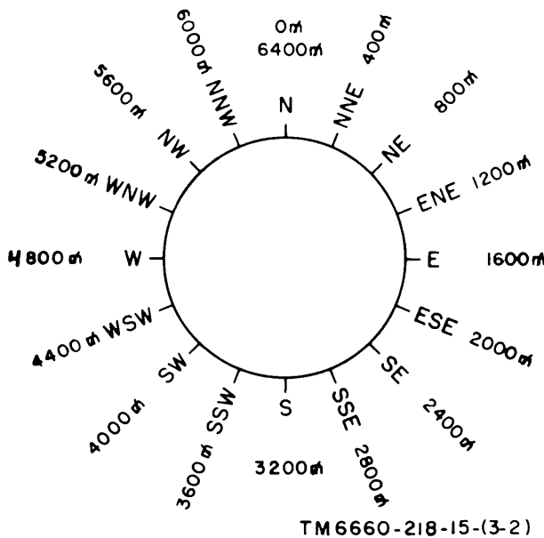
Figure 3-2. Mils scale conversion.
