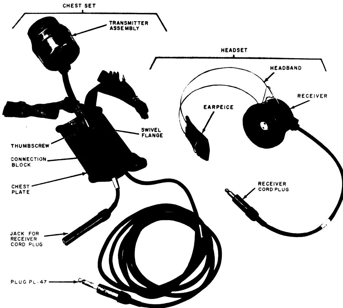
Figure 1-11. Head and chest set.
