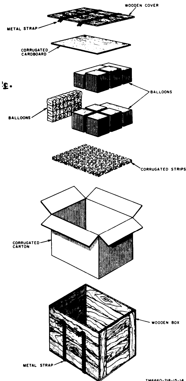
Figure 2-1. Typical packaging diagram, balloon equipment.
