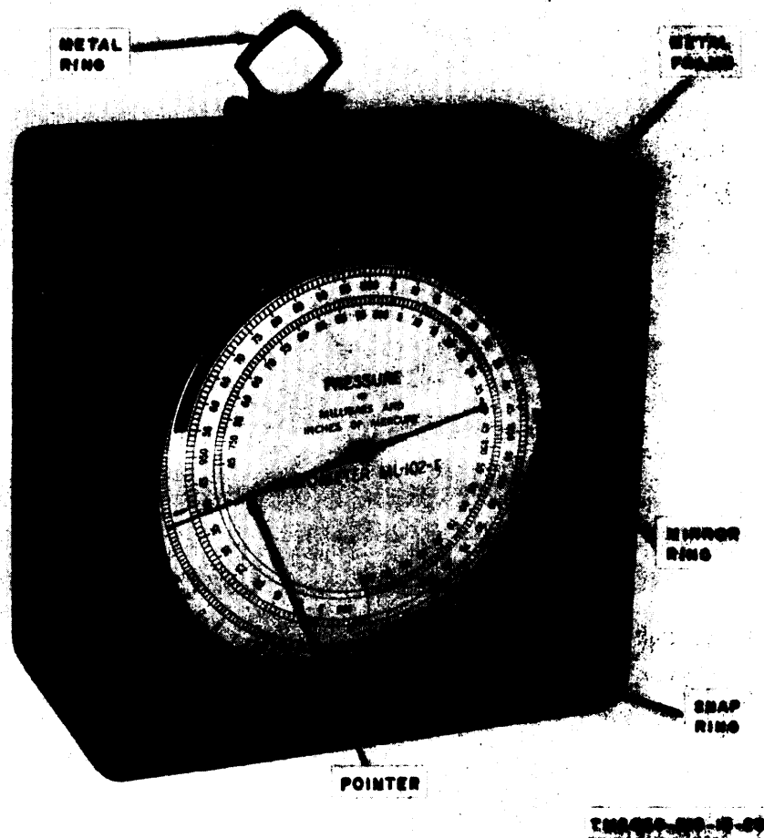
Figure 1-9. Barometer ML-102-E.
