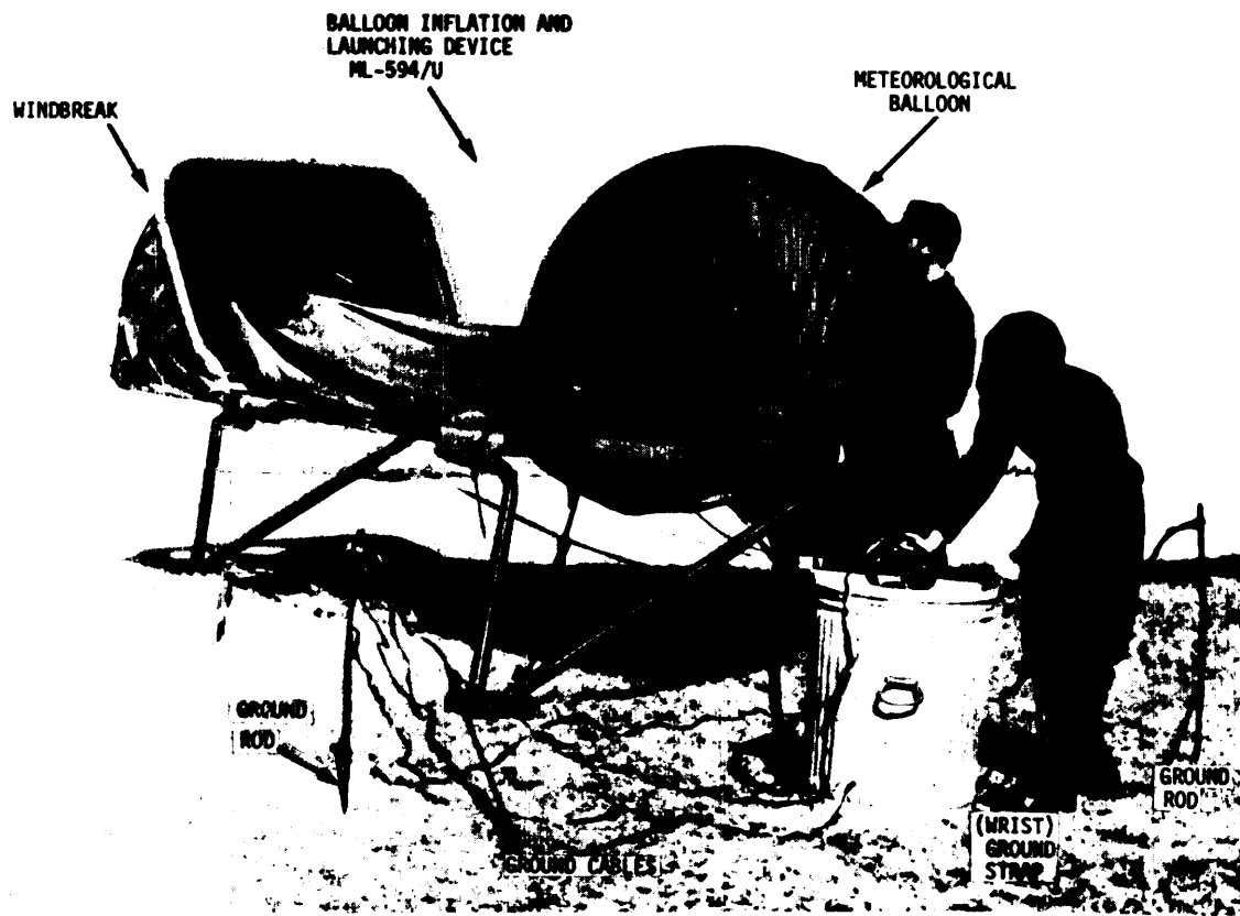
Figure 2-5 ①. Grounding of Hydrogen generating equipment. (Part 1 of 2).
