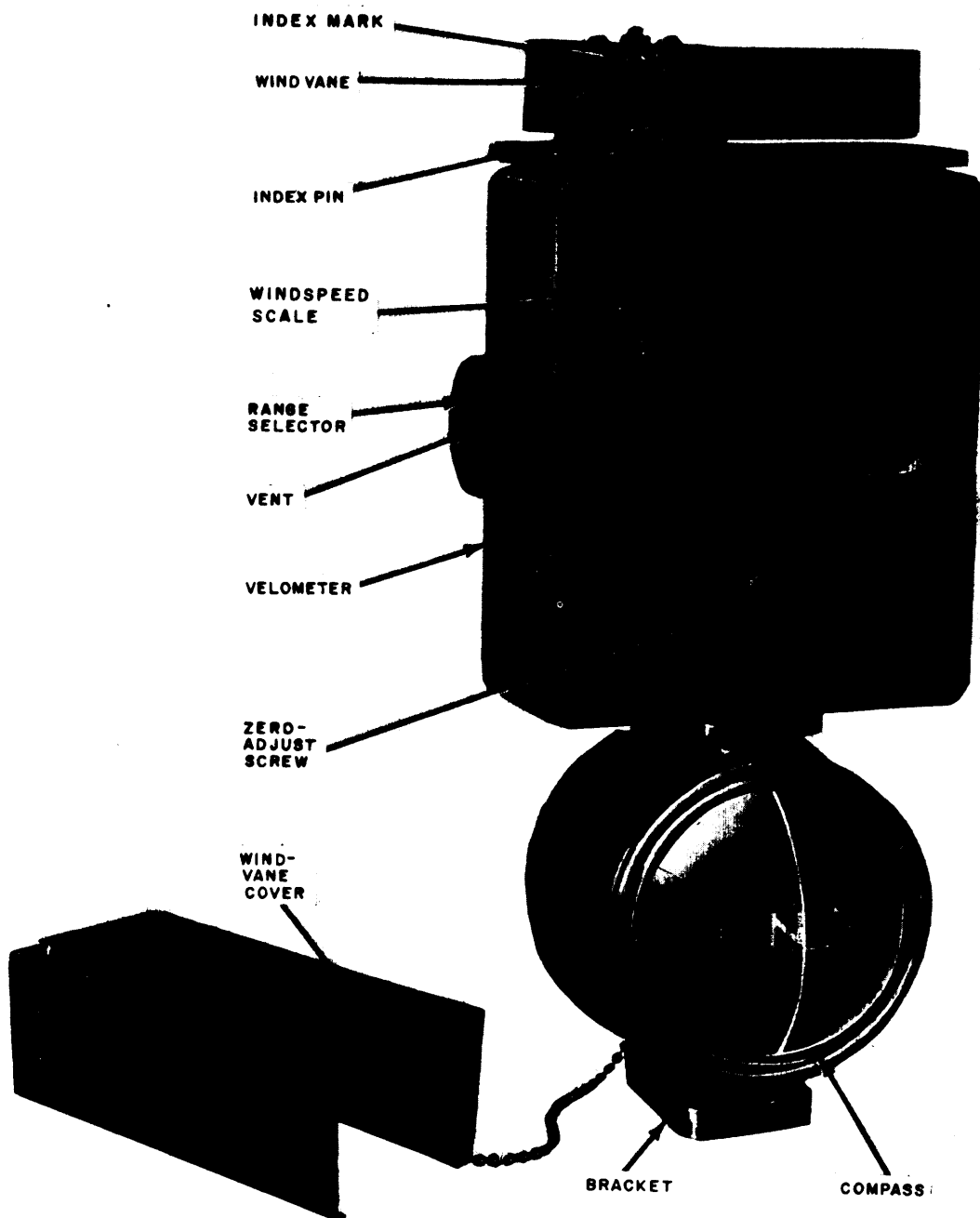
Figure 1-8. Anemometer.
