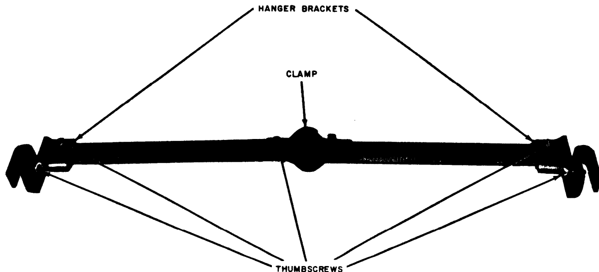
Figure 1-22. Bracket assembly.
