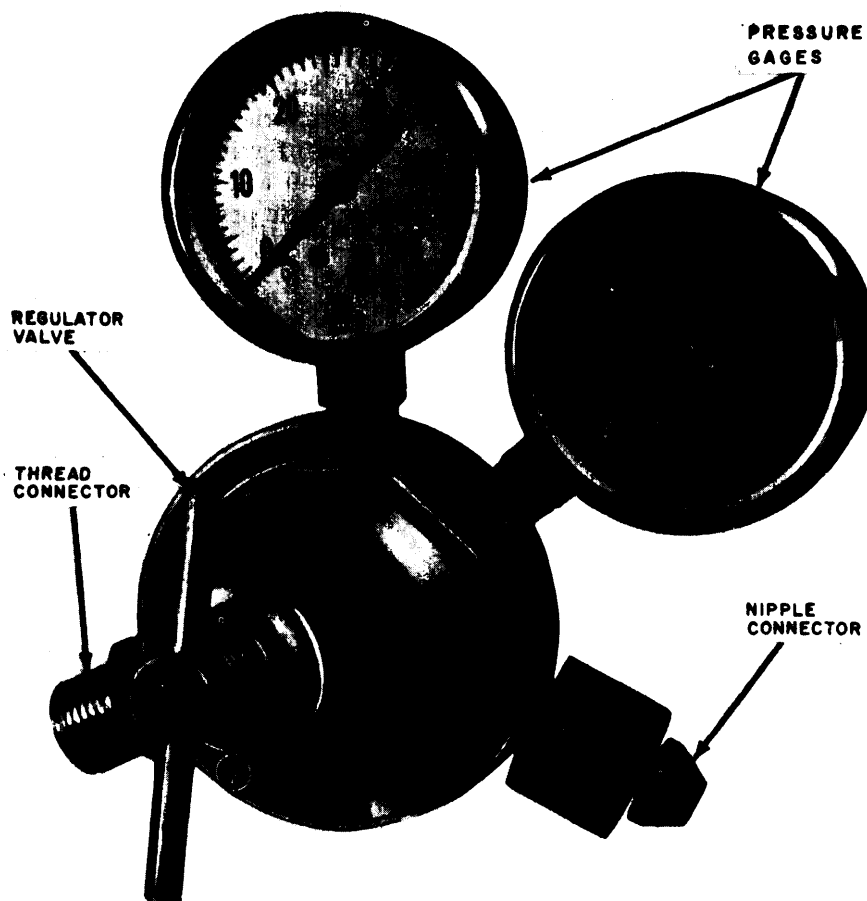
Figure 1-29. Gas regulator.
