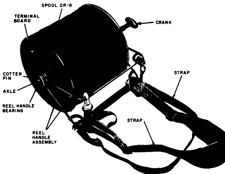
Figure 1-25. Reel,
