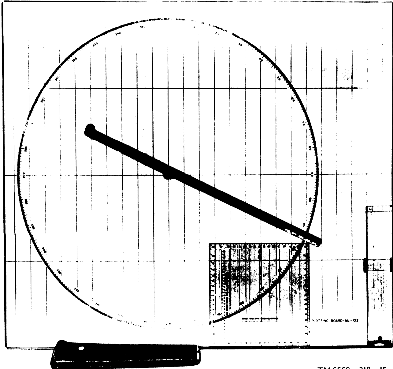
Figure 3-3. Zone wind plotting board.
