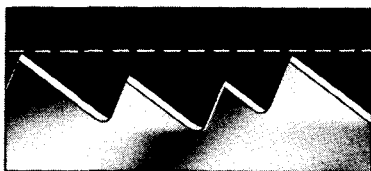
THIS RIP SAW NEEDS JOINTING WHICH IS THE FIRST STEP IN SHARPENING
