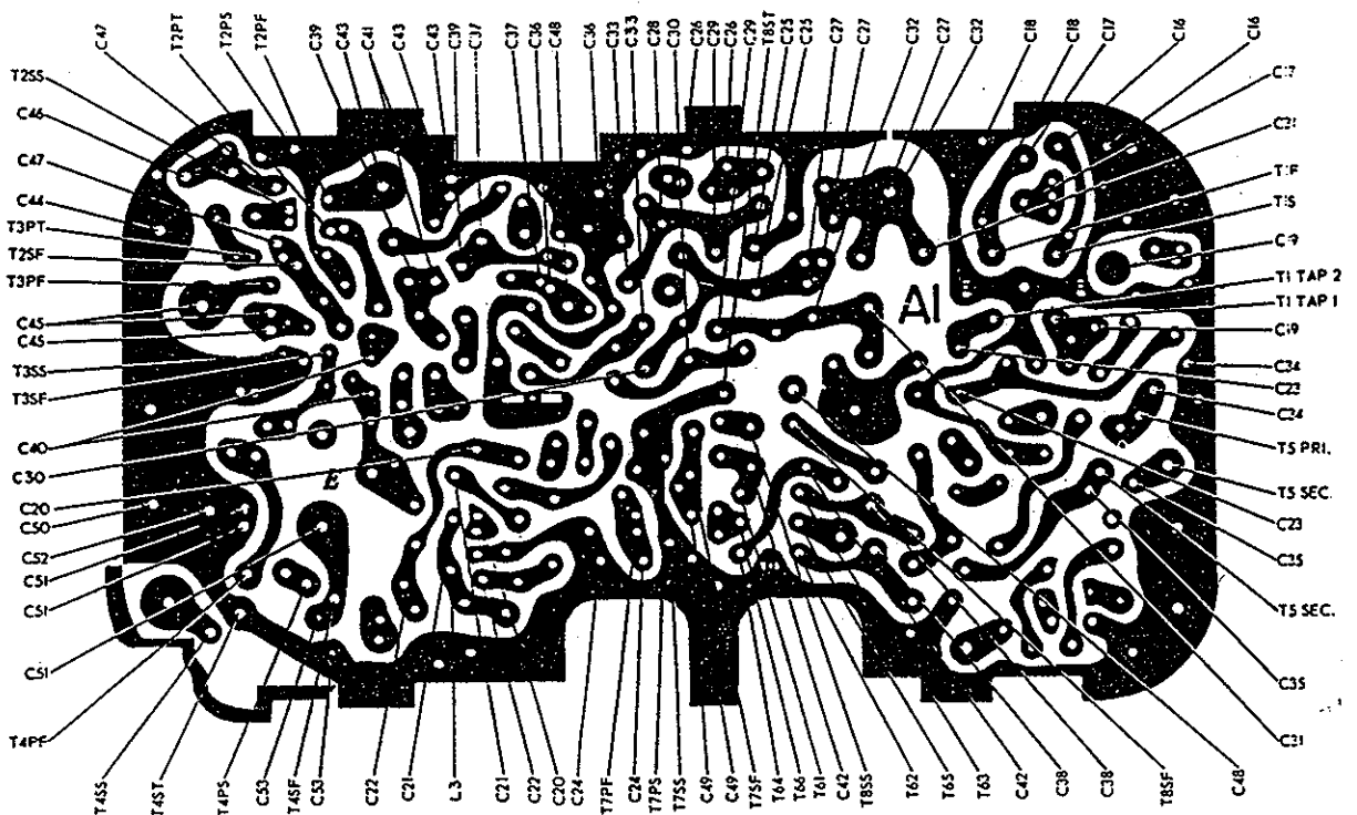
Figure 4-8(3). AN/PRT-4 only, printed board A1, component terminal connections (part 3 of 3).
