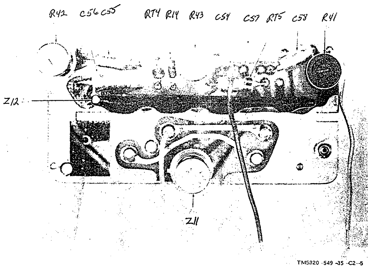
Figure 4-12.2. AN/PRT-4A only, parts location, printed board assembly A3.
