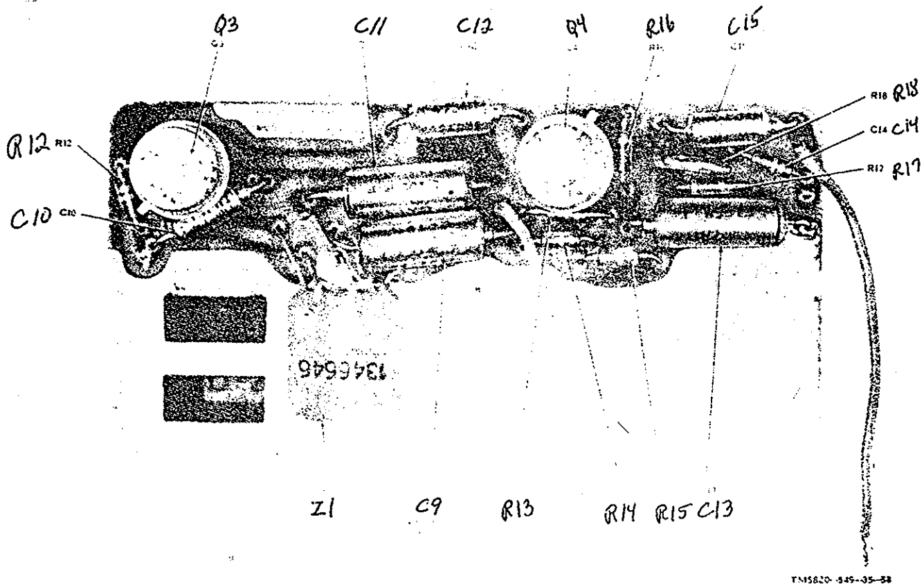
Figure 4-11. AN/PRT-4 only parts locations, printed board assembly A3.
