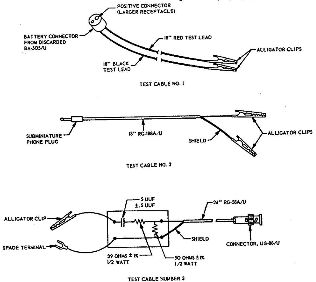
Figure 6-1Ⓞ. Special test cables, construction details.
