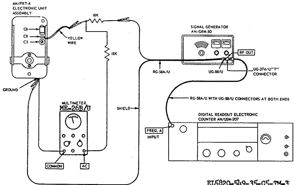
Figure 5-1. AN/PRT-4 quarter-wavelength alignment, test setup.
