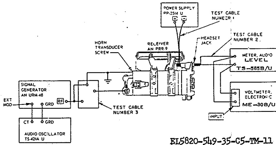
Figure 6-14.1. AN/PRR-9 audio frequency test.
