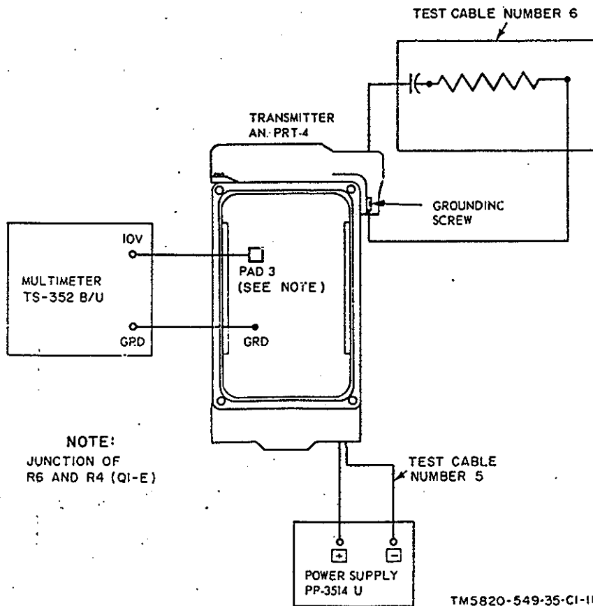
Figure 6-14.4. AN/PRT-4 regulated voltage test.
