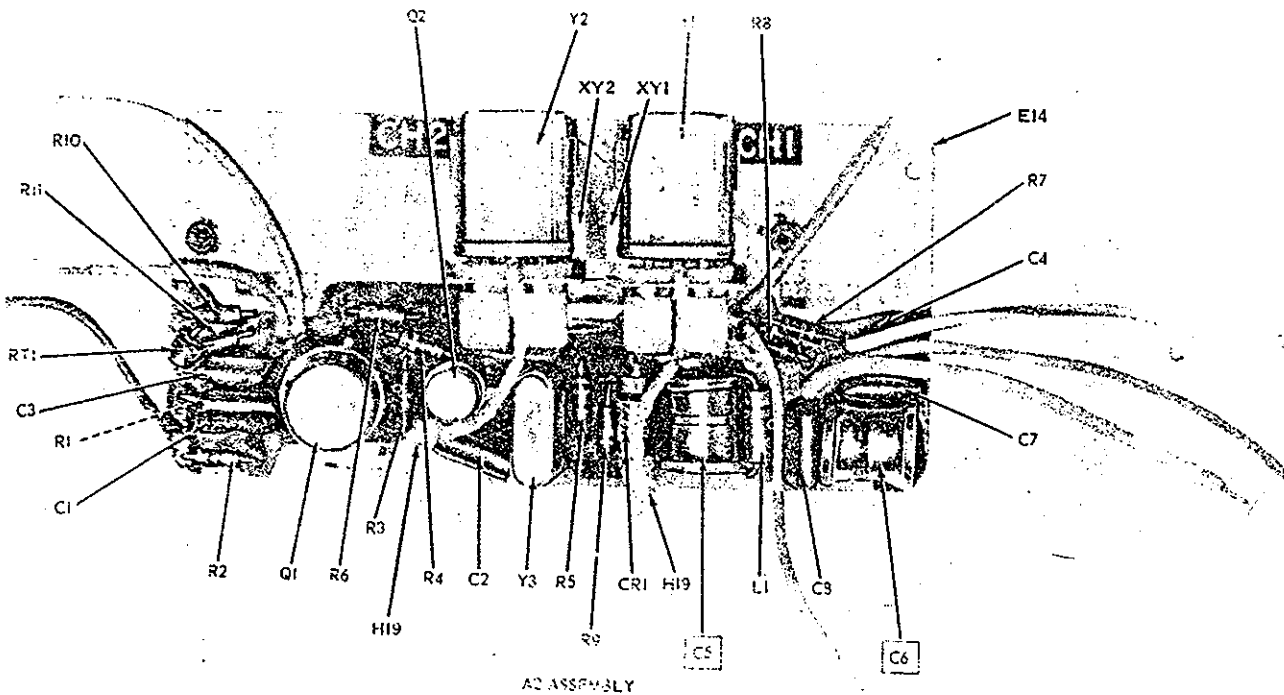
Figure 4-9. AN/PRT-4 parts locations, printed board assembly A2.
