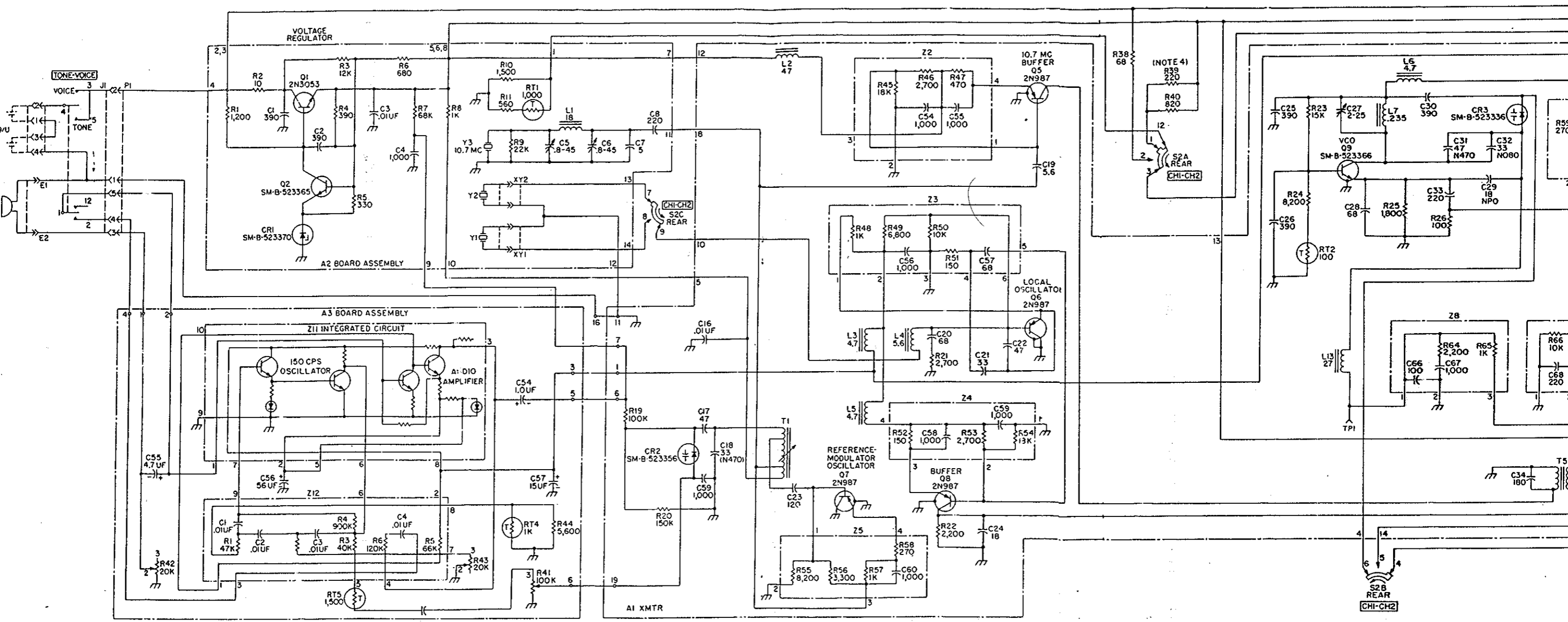
Figure 6-19. Transmitting Set, Radio AN/PRT-4A, schematic diagram.
