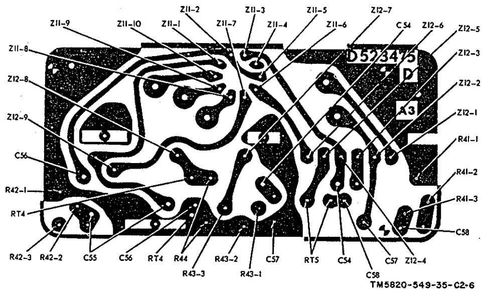
Figure 4-12.3. AN/PRT-4A only, printed board A3, component terminal connections.
