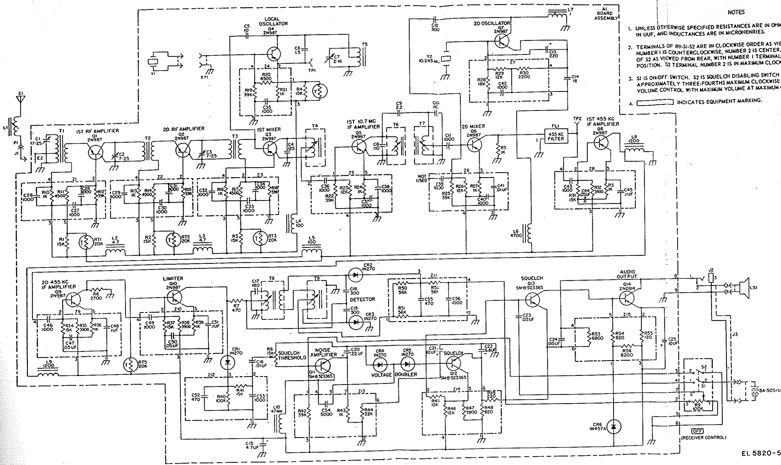
Figure 6-17. Receiving Set, Radio AN/PRR-9 schematic diagram.
