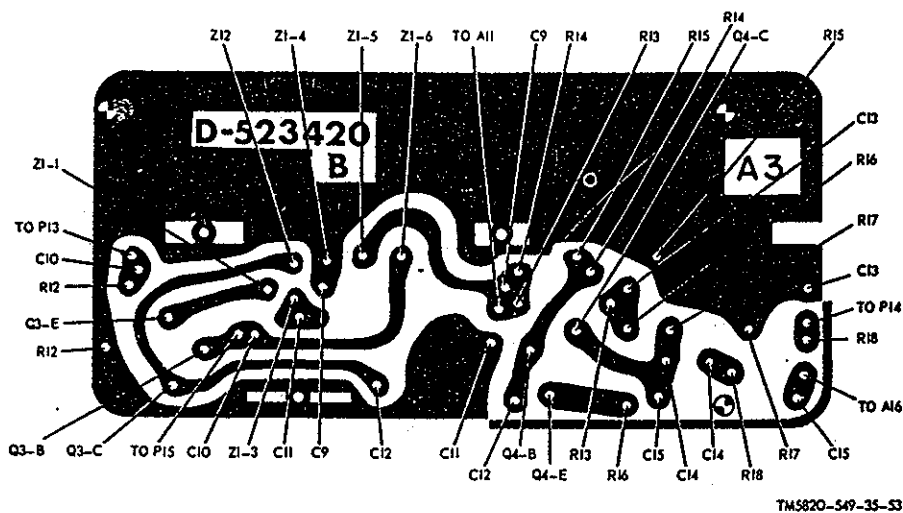
Figure 4-12. AN/PRT-4 only printed board A3, component terminal connections.
