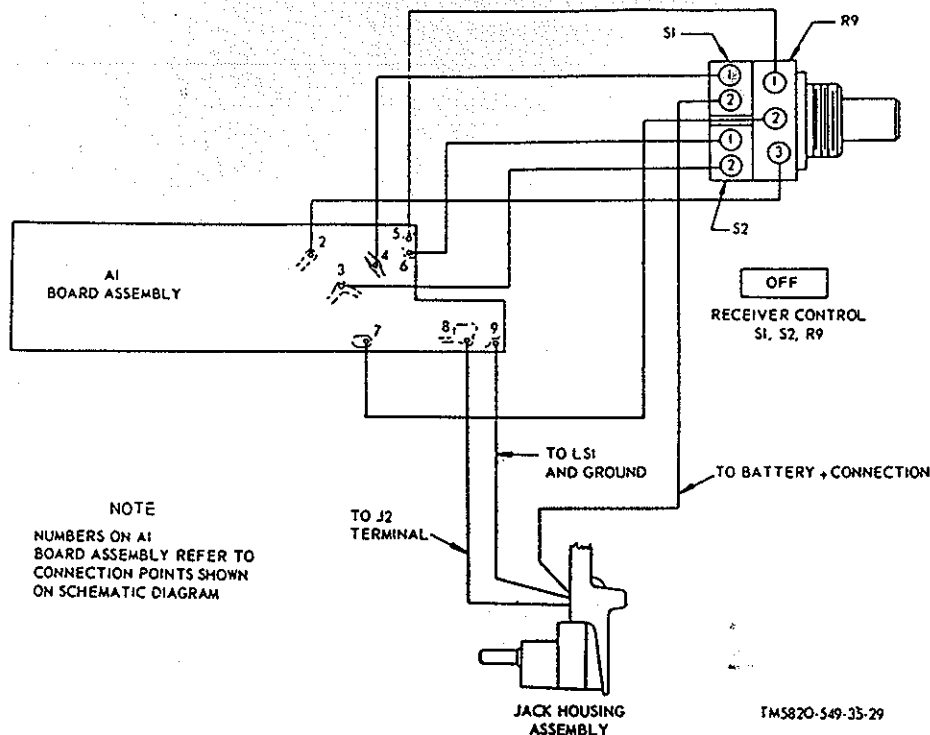
Figure 4-4. AN/PRR-9 switch wiring diagram.
