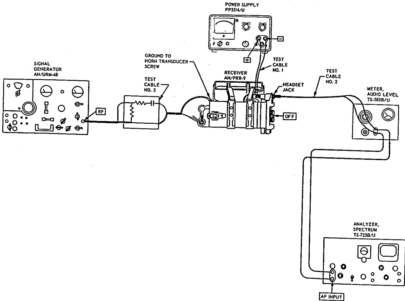
Figure 6-4. AN/PRR-9 audio distortion test.
