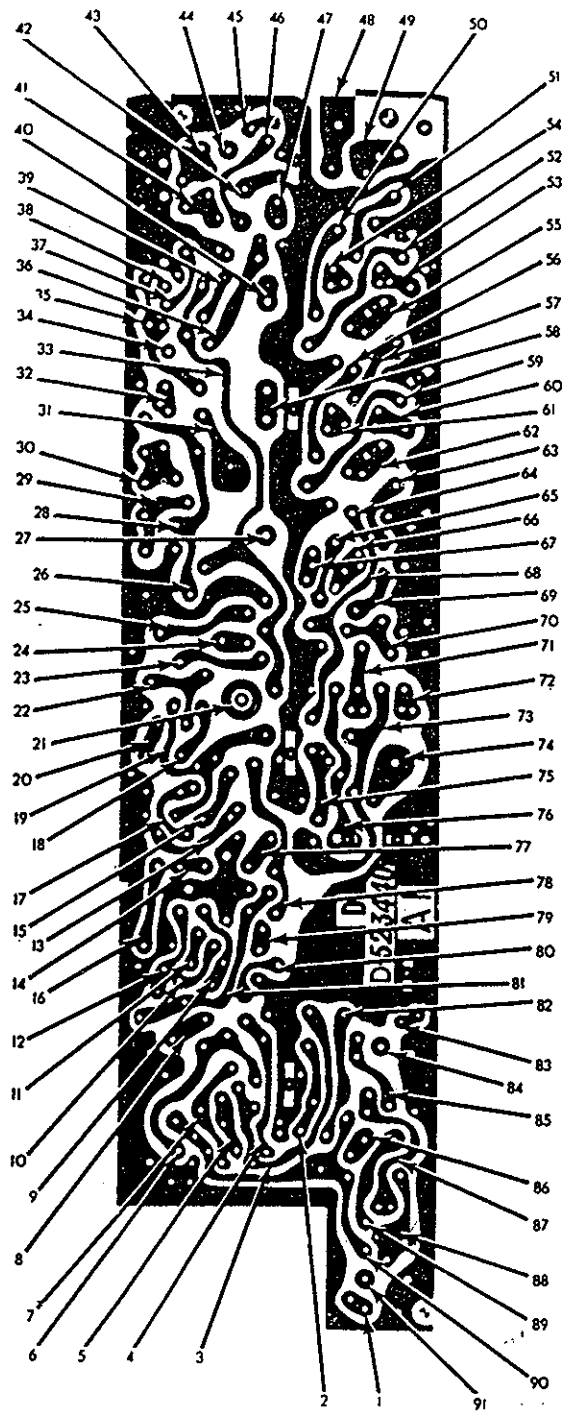
Figure 4-5. AN/PRR-9 printed board, voltage and resistance pad locations.
