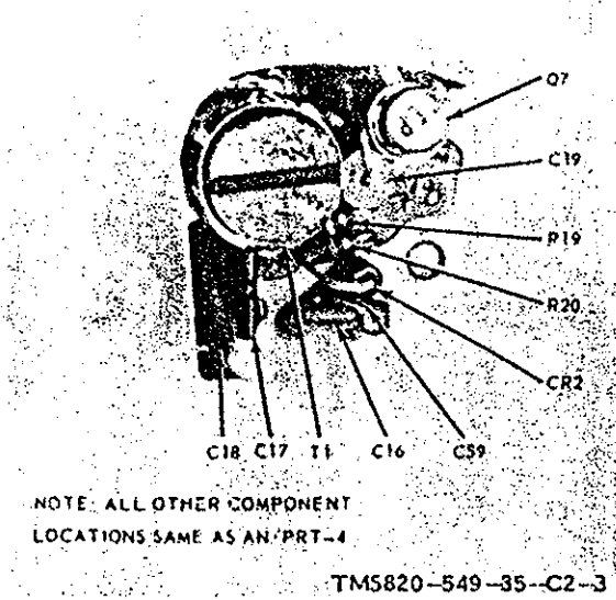
Figure 4-6.1. AN/PRT-4A only, parts location, printed board assembly A1.
