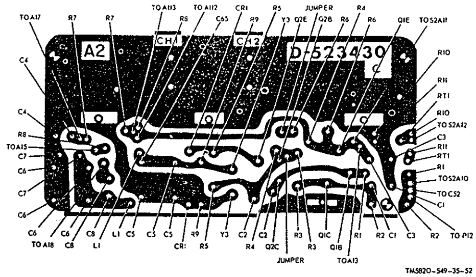
Figure 4-10. AN/PRT-4 printed board A2, component terminal connections.
