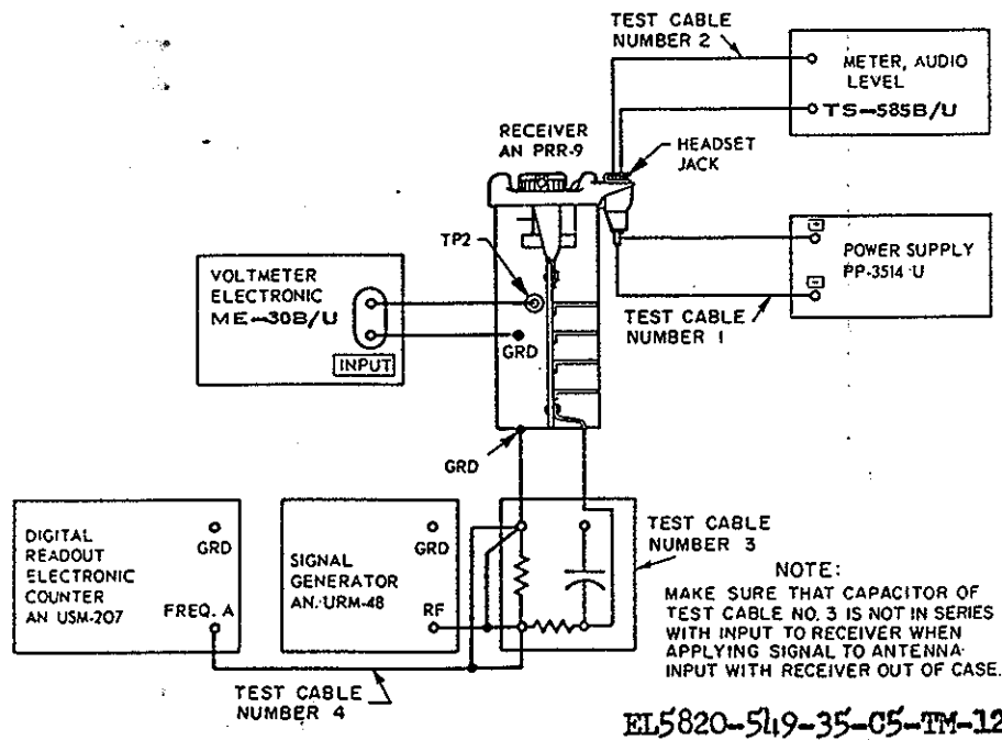
Figure 6-14.2. AN/PRR-9 IF selectivity test.
