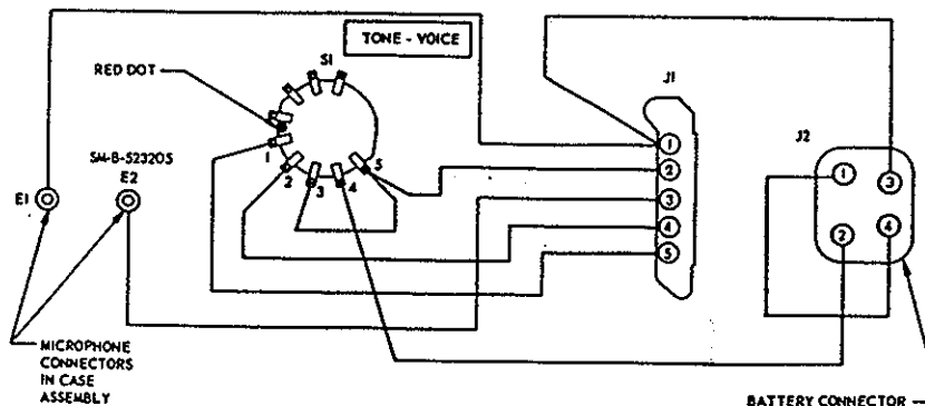
B. S1, TONE-VOICE SWITCH WIRING.
