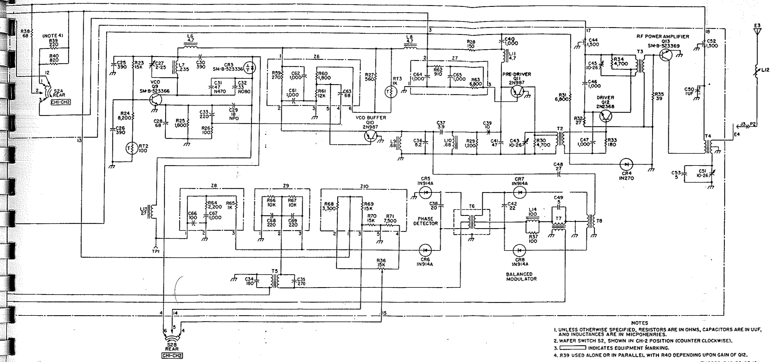
Transmitting Set, Radio AN/PRT-4A, schematic diagram.
