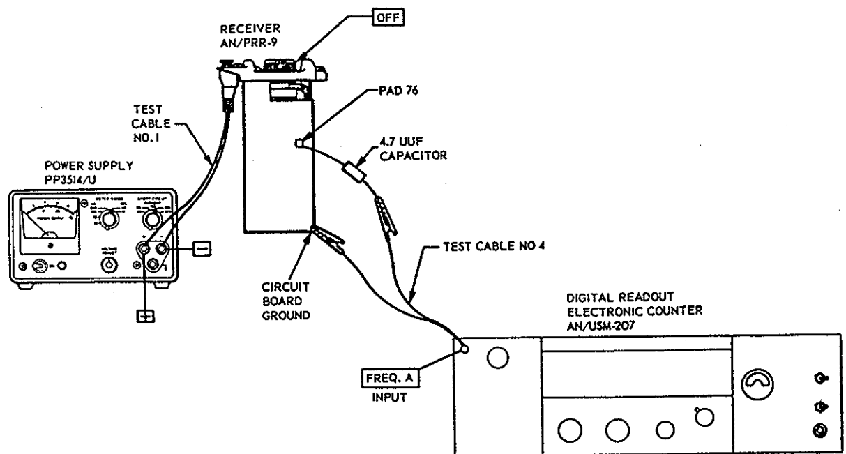
Figure 6-6. AN/PRR-9 local oscillator frequency test.
