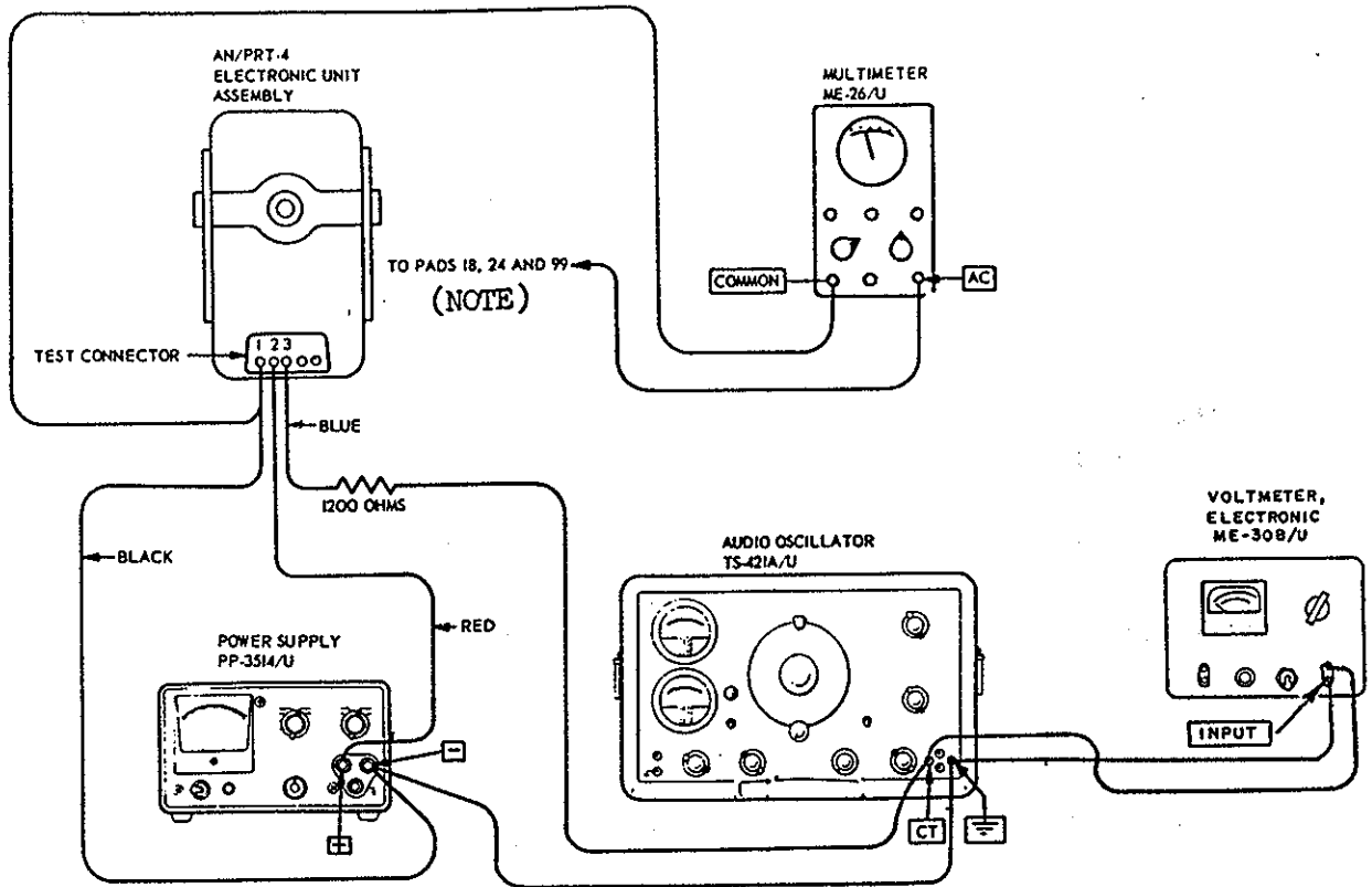
Figure 4-14. AN/PRT-4 audiofrequency test setup.
