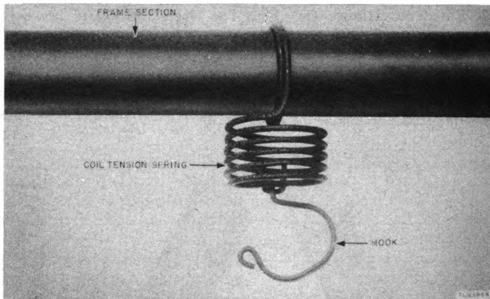
Figure 14. Detailed view of coil tension spring.
