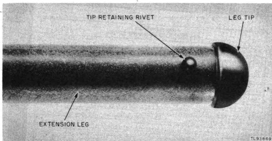
Figure 15. Detailed view of leg tip.
