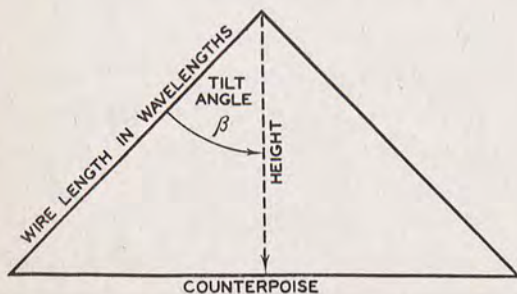
Figure 2A. Half-rhombic antenna triangle showing height of the upper apex, wire length on a leg, and tilt angle.
