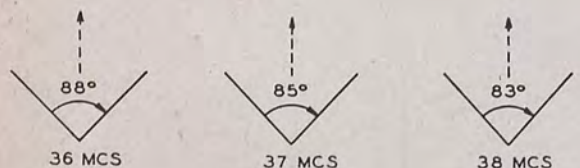
Figure 19. Beam angles at frequencies of 27 to 38 megacycles.
