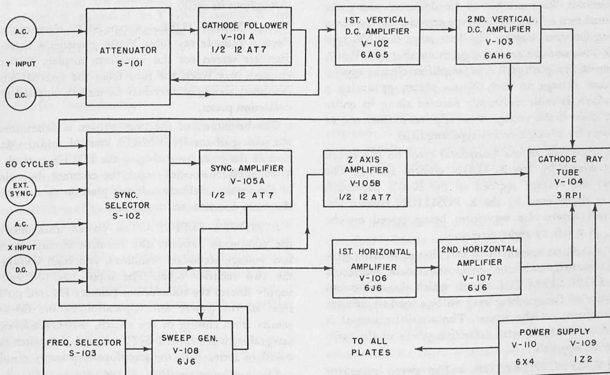
Figure 2-1. Simplified Block Diagram Oscilloscope OS-8A/U
