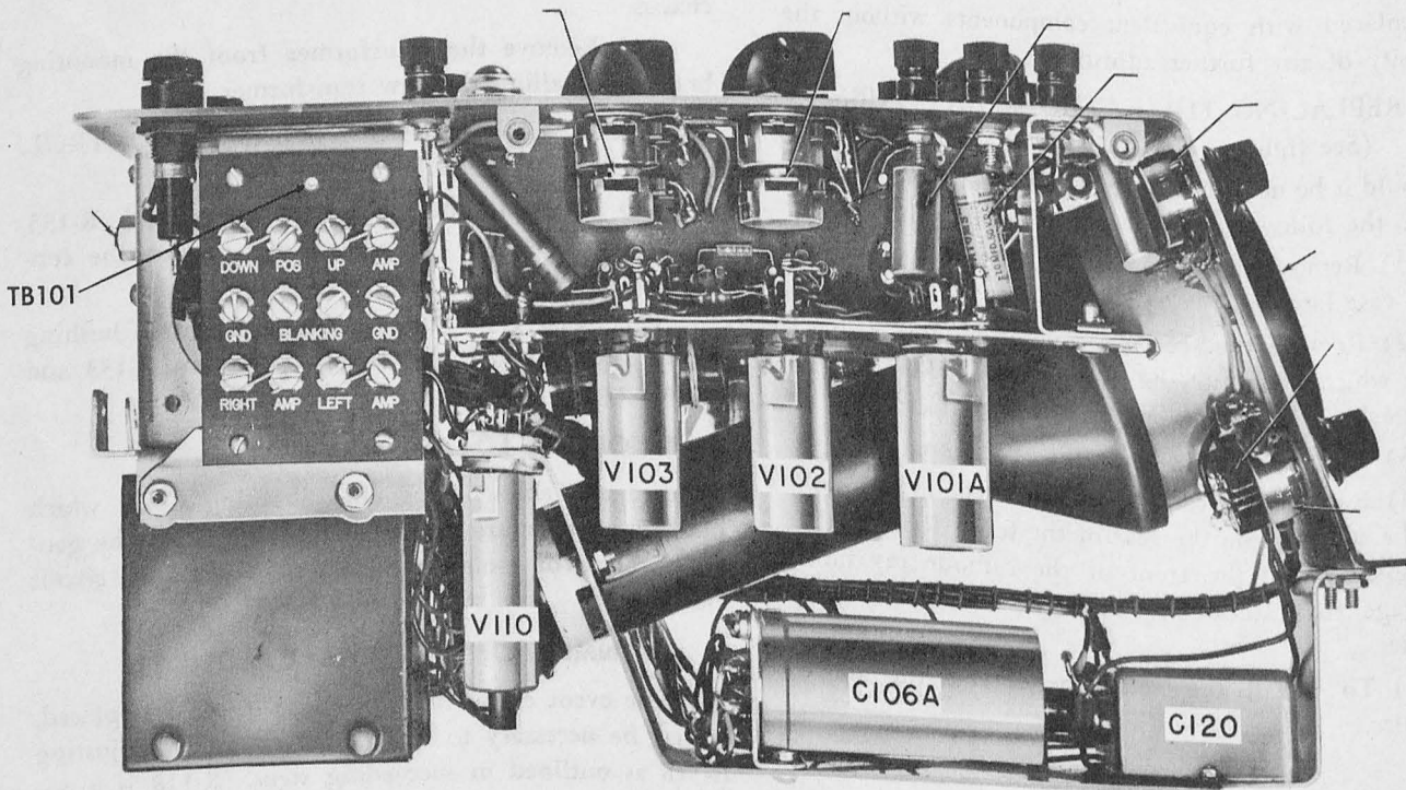
Figure 7-2. Principal Components and Tube Locations
