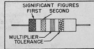
JAN COLOR CODE FOR FIXED COMPOSITION RESISTORS AXIAL TYPE INSULATED
