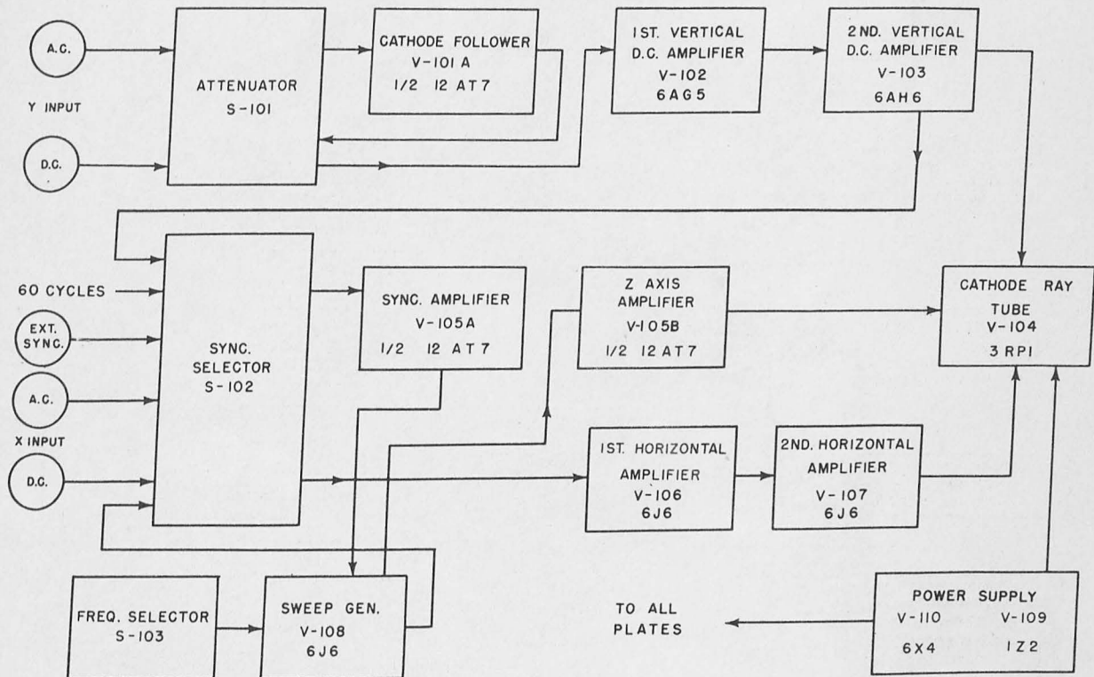
Figure 7-3. Block Diagram of Oscilloscope OS-8A/U
