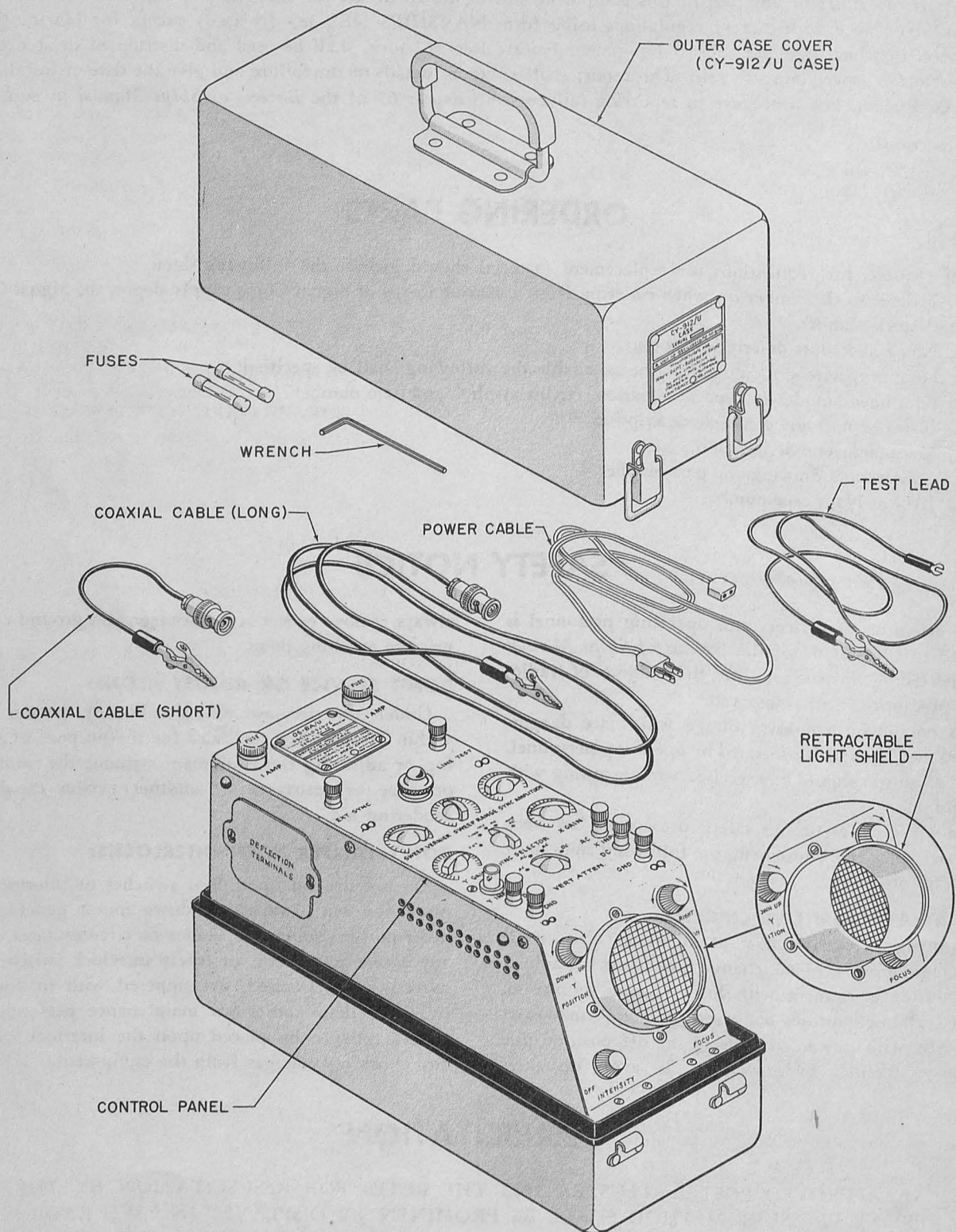
Figure 1-1. Oscilloscope OS-8A/U
