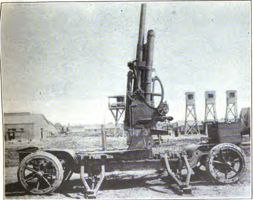
FIG. 41. —3-inch A. A. gun, model 1916, carriage, model 1917, on 3-ton A. A. trailer mount.
