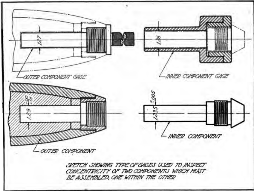
FIG. 223.—Concentricity gauges.
