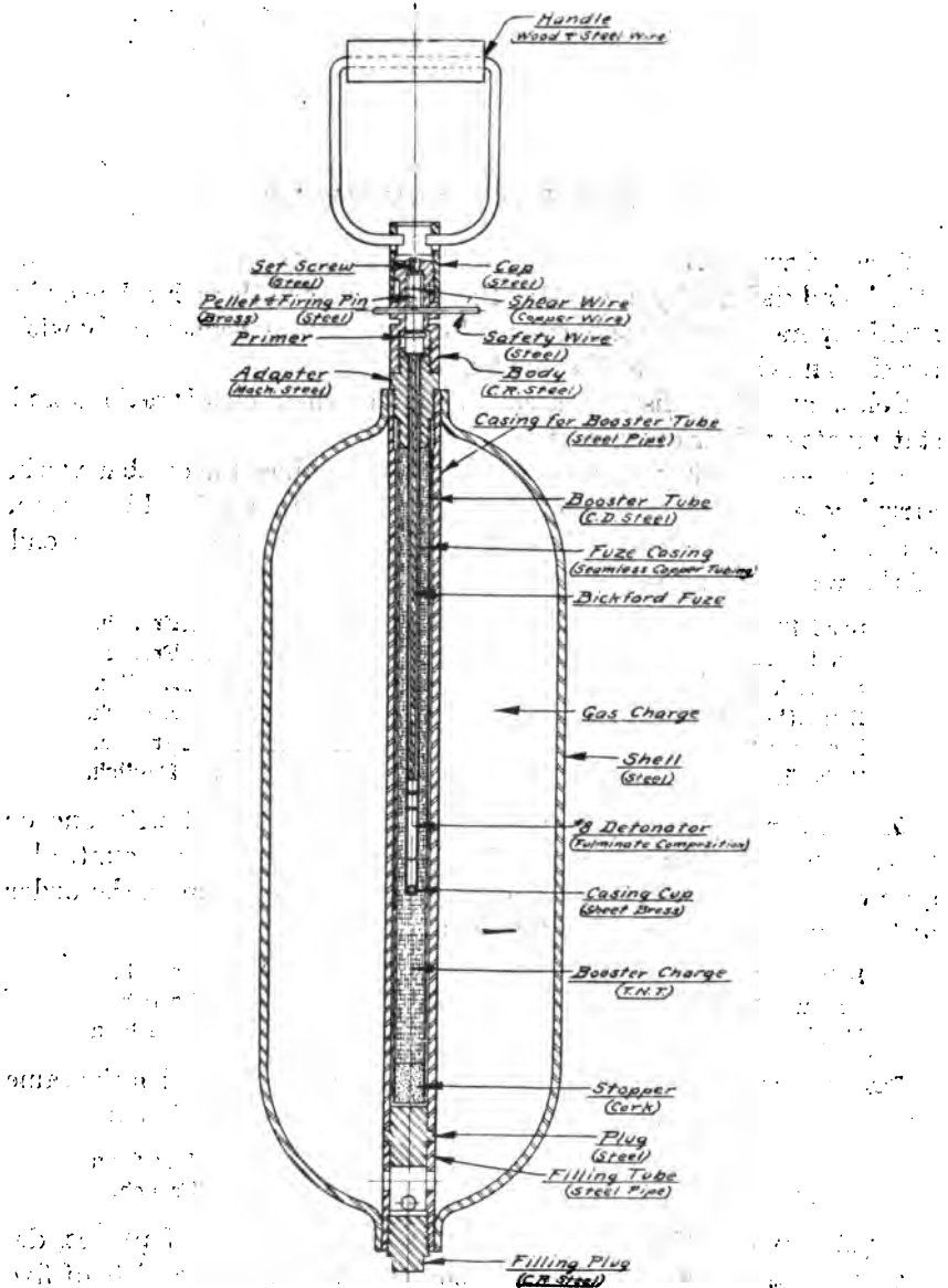
FIG. 109.—Livens projector shell, Mark I—section.
