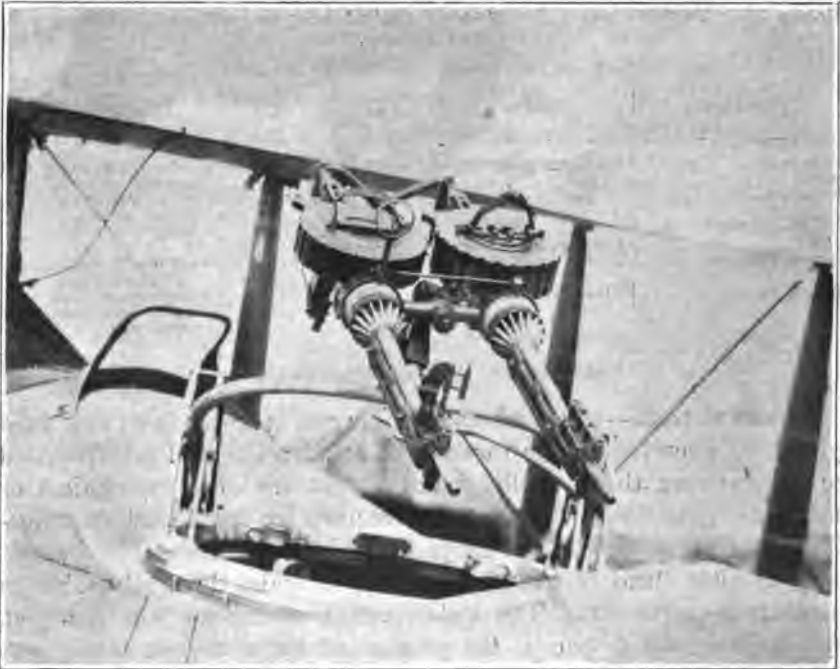
FIG. 110.—Two Lewis Guns mounted in jumelage in a tourelle or turret.
