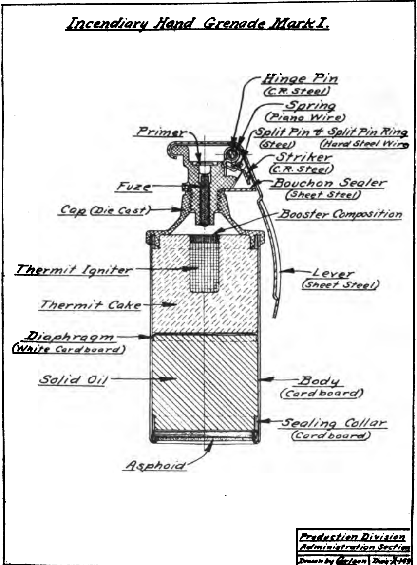
FIG. 91.—Sectional view of incendiary hand grenade, Mark I.
