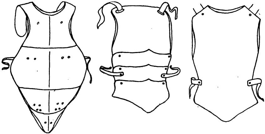
Figure 188.—A light body defense which shall not hamper movement, yet shall be proof against missiles of low and middle velocity, and be so cushioned with sponge rubber as to absorb shock appreciably.
