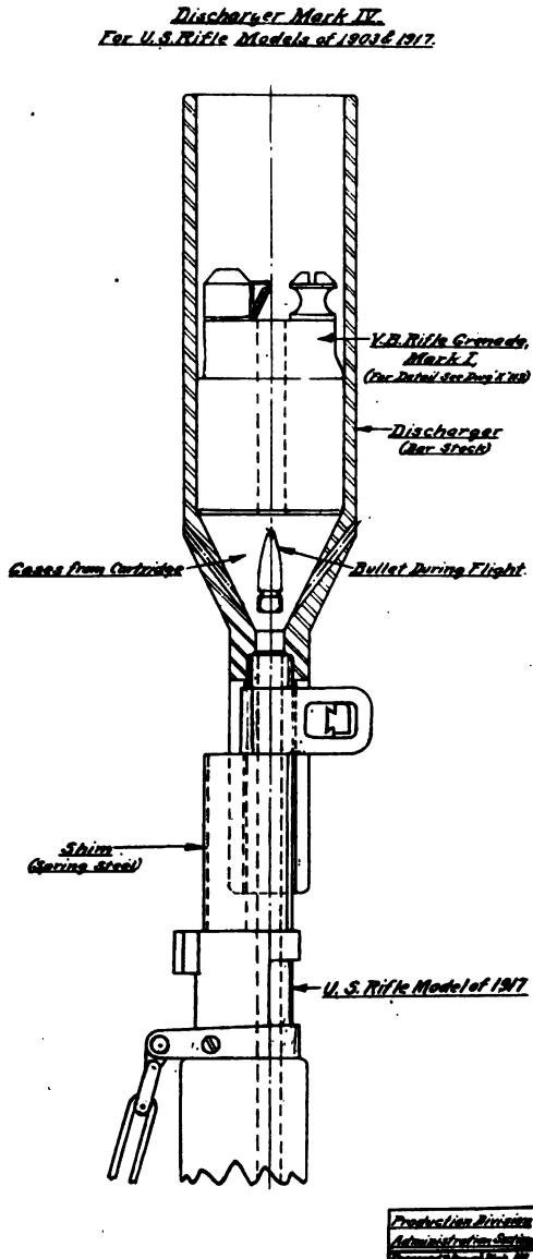
FIG. 94.—Rifle grenade discharger, Mark IV
