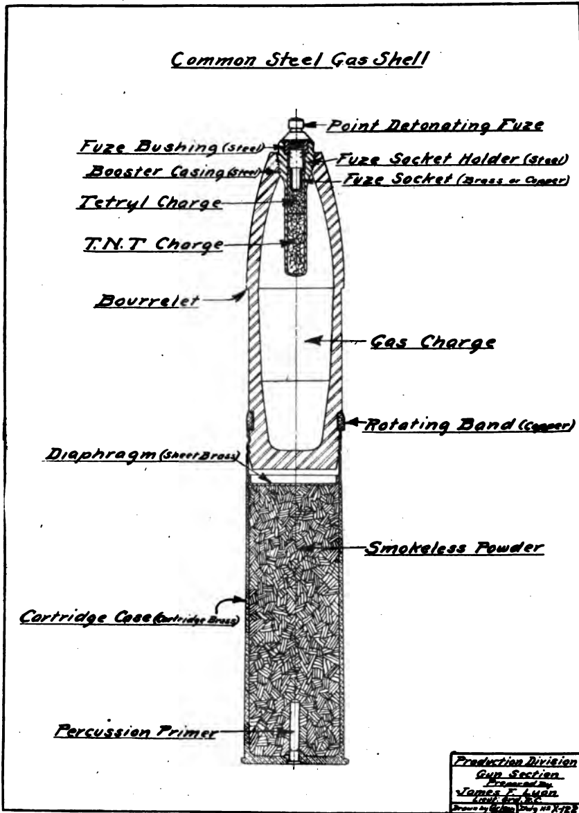
FIG. 53.—Common steel gas shell.
