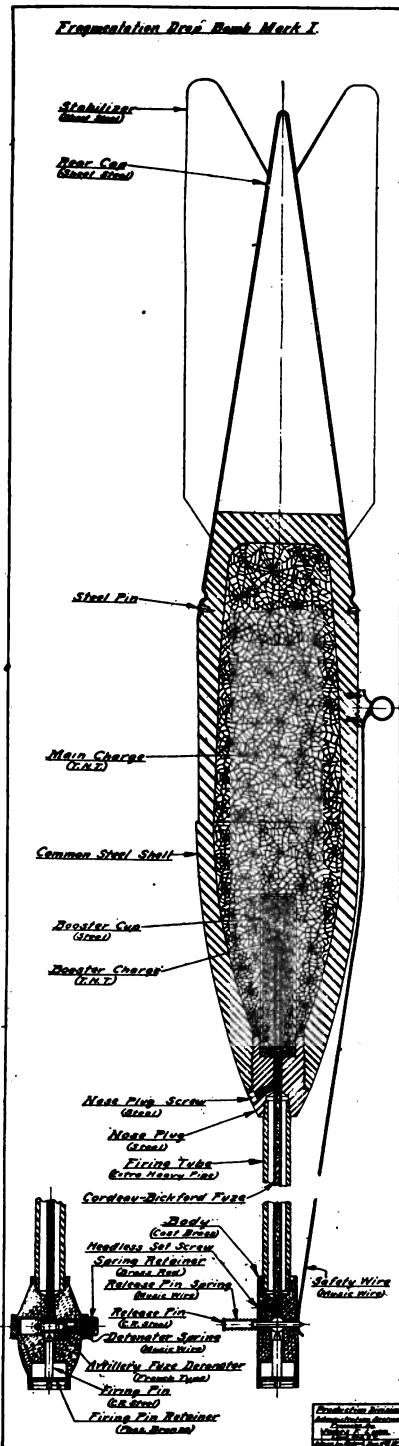
FIG. 117.—Fragmentation drop bomb, Mark I.
