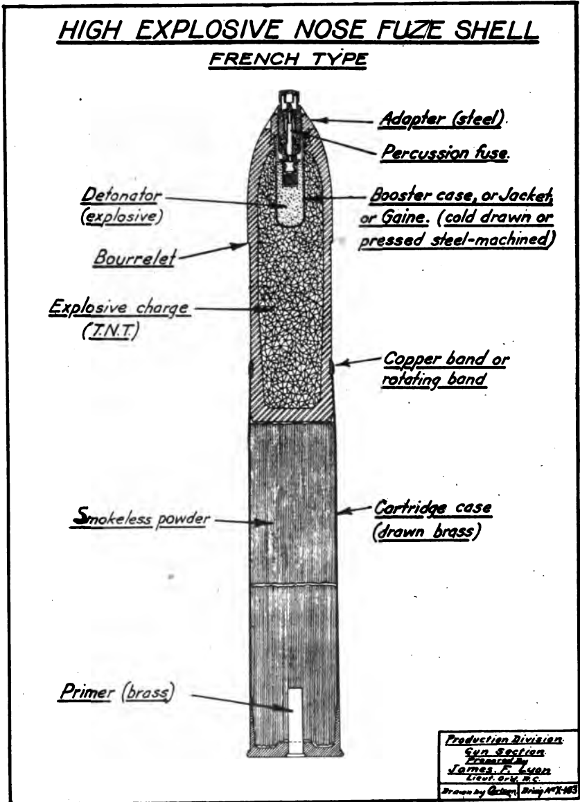
FIG. 52.—High-explosive nose fuze shell, French type.
