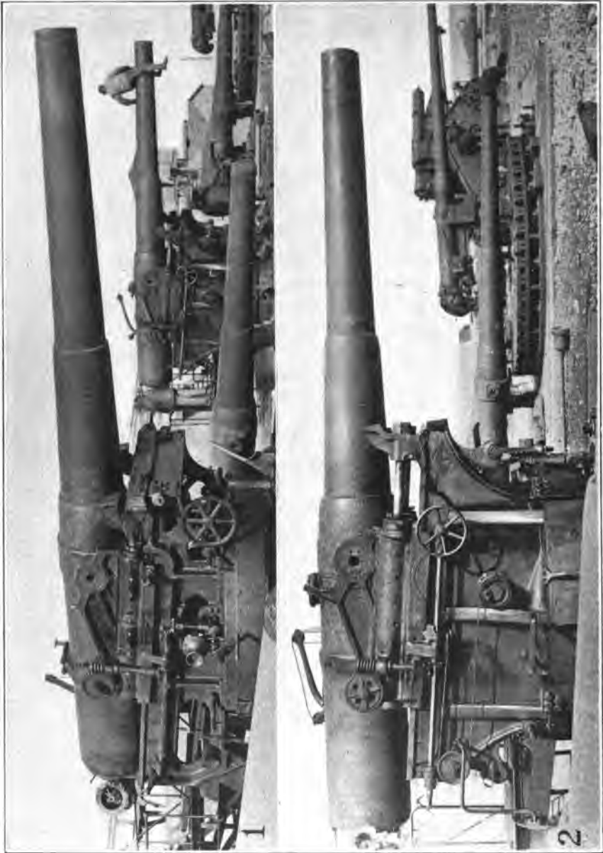
FIG. 28.—8-inch and 10-inch guns on seawall barrette carriages. 1. 10-inch gun, model 1865. 2. 8-inch gun, model 1888.
