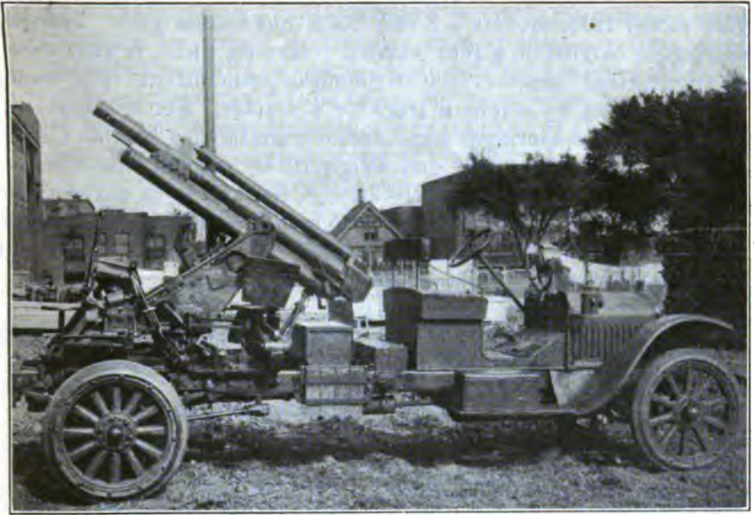
FIG. 40. —75-mm. field gun, model 1916, on A. A. truck mount, model 1917, 24-ton White truck.
