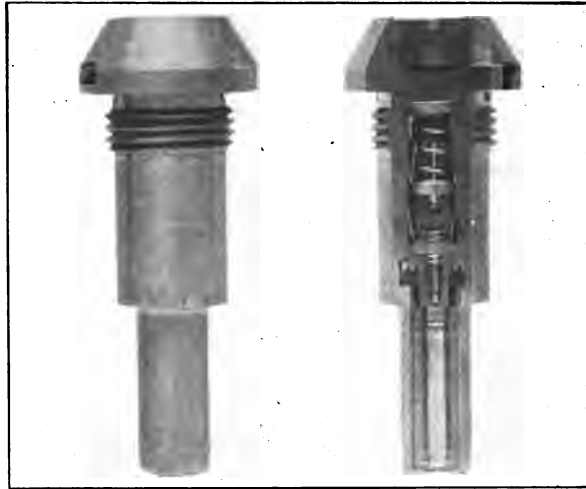
FIG. 59.—Detonating delay fuze, Mark IV. Exterior view and section.
