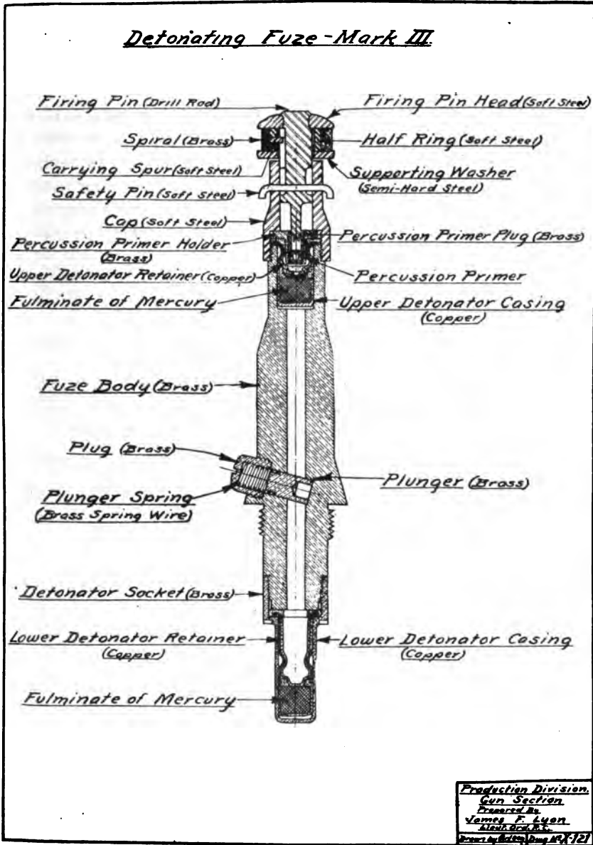
FIG. 58.—Point detonating fuze, Mark III.
