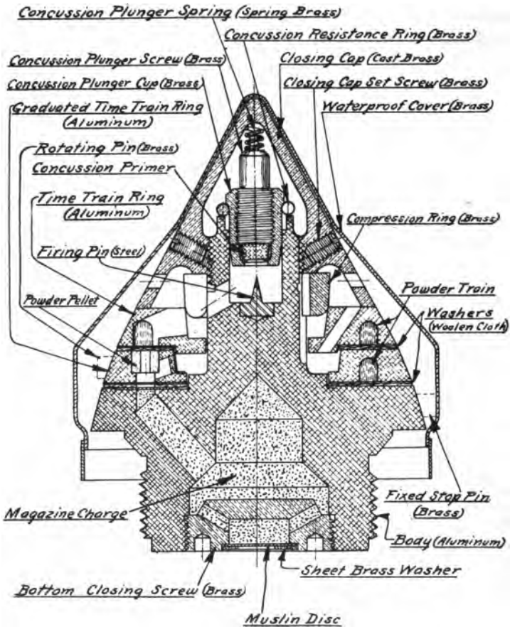
FIG. 69.—Anti-aircraft time fuze, Mark II, type "8."
