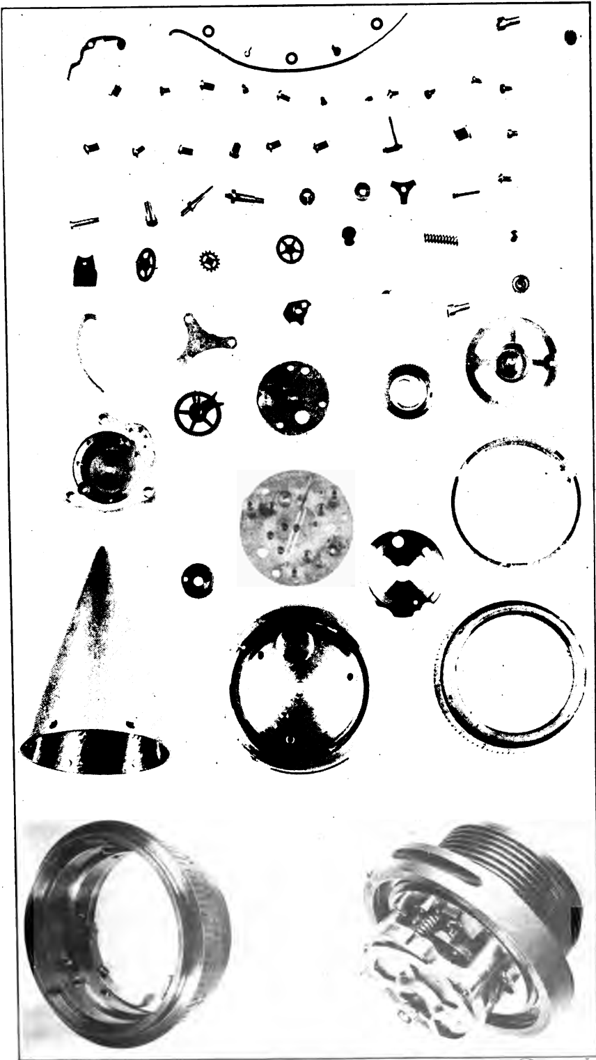
FIG. 70.—Mechanical time fuze, Mark I. Component parts. Digitized by Google 169
