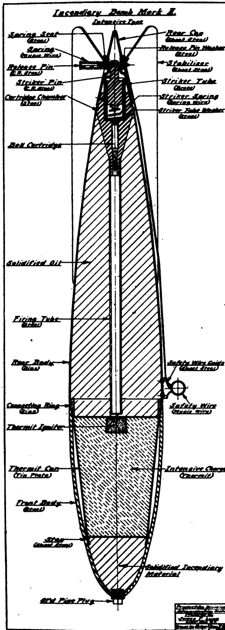
FIG. 123.—Incendiary drop bomb, Mark II.
