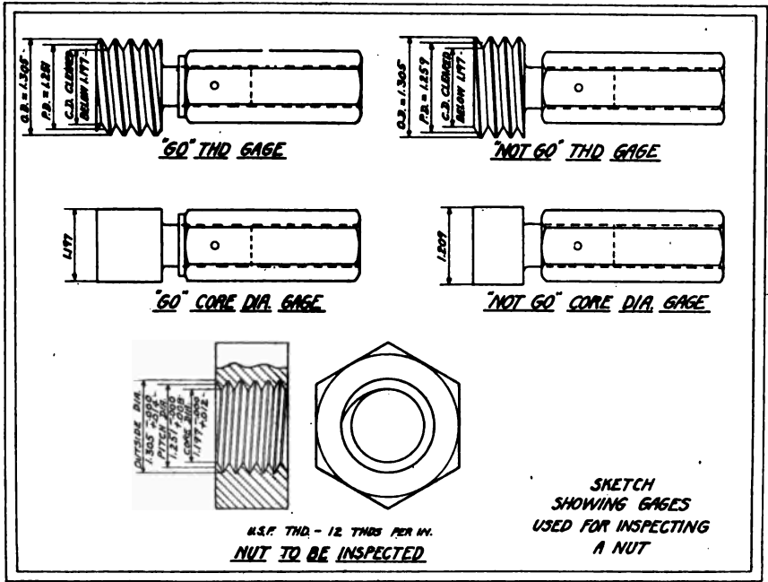
FIG. 217.—Gauges used for inspecting a nut.
