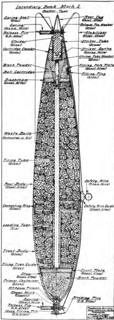
FIG. 120.—Incendiary drop bomb, Mark I.
