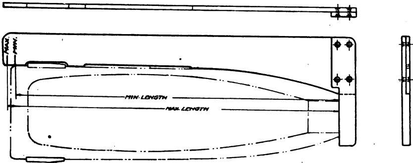
FIG. 214.—Sketch showing type of gauge used to inspect total length and profile of shell.
