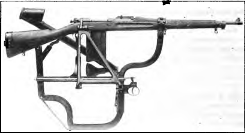
FIG. 151.—Periscope attachment for U. S. service rifle.
