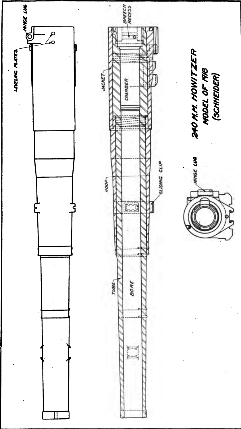
FIG. 24.—240-mm. howitzer, model of 1918 (Schneider).
