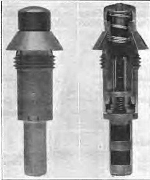
FIG. 62.—Mark V point detonating fuze, exterior view and section.
