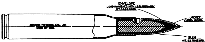
FIG. 157.—Armor-piercing cartridge, caliber .30, model 1918.
