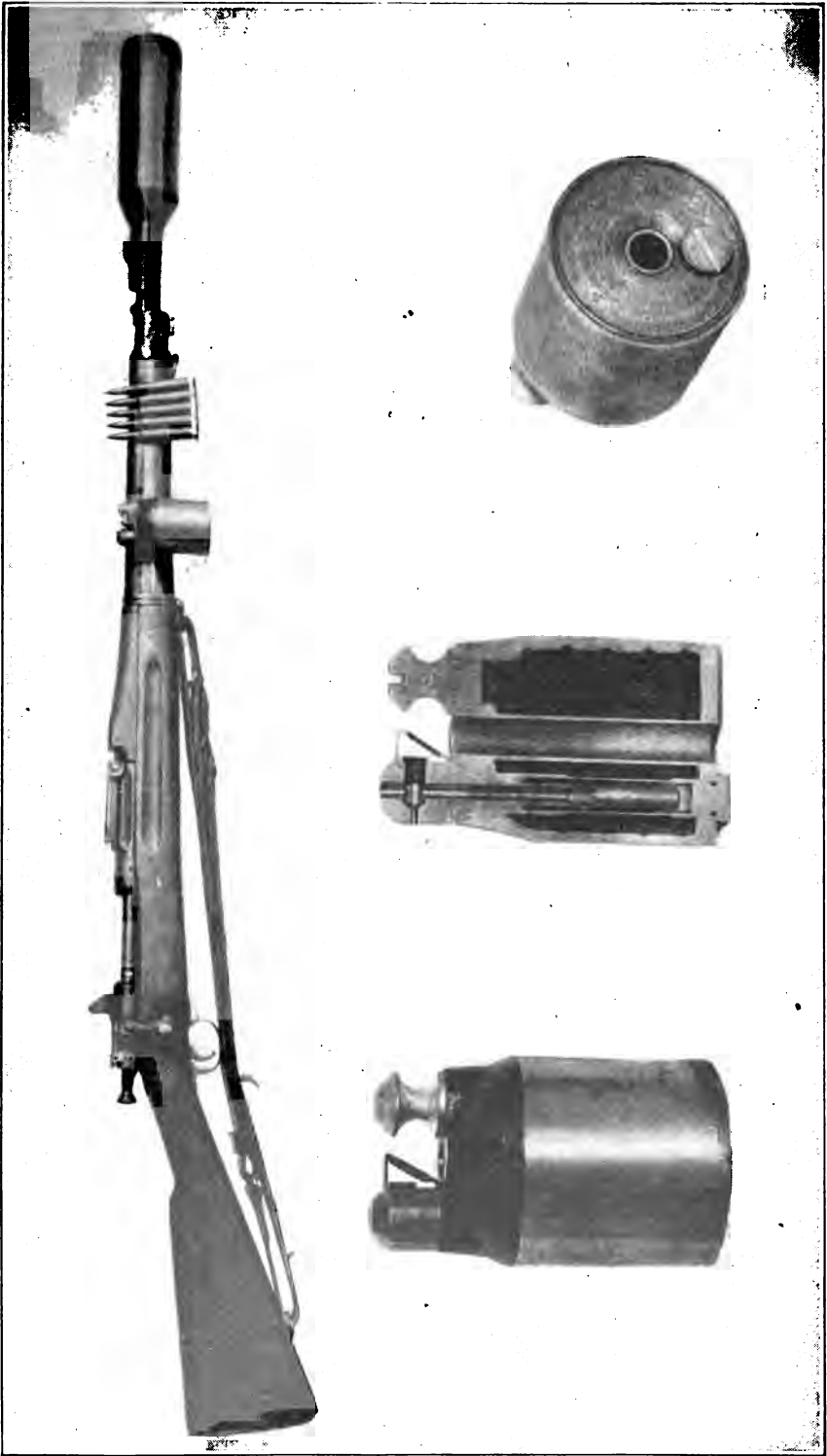
FIG. 83.—V. B. rifle grenade. Discharger mounted on rifle, together with grenade and cartridges. End view of grenade. Side view of grenade. Sectional view of grenade.
