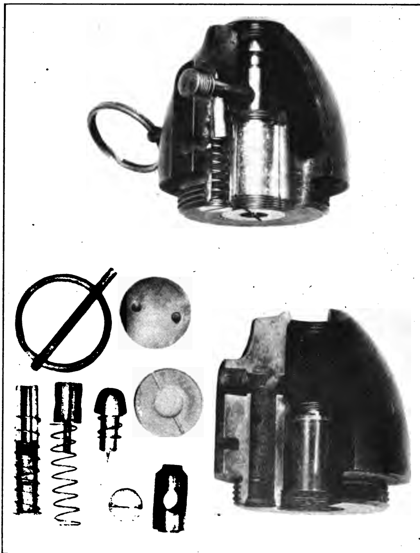
FIG. 106.—Trench mortar fuze, Mark VI. Assembly and section.
