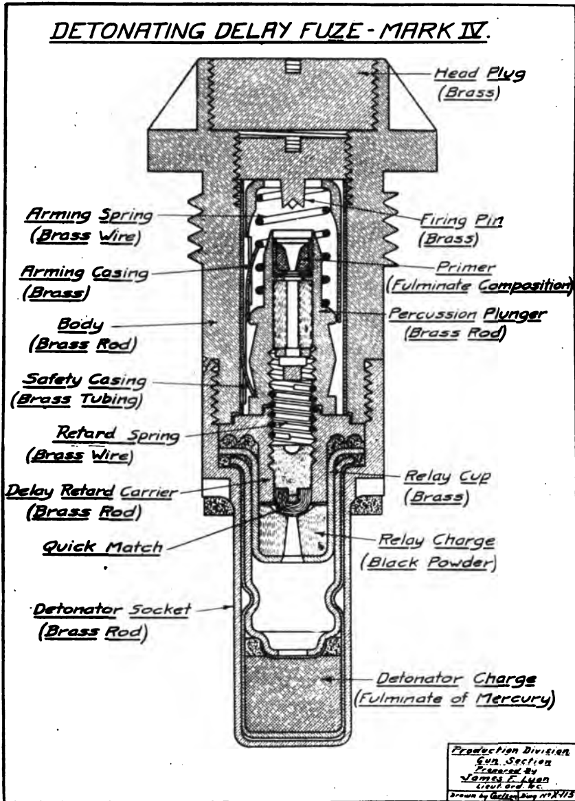
FIG. 60.—Point detonating fuze, Mark IV.
