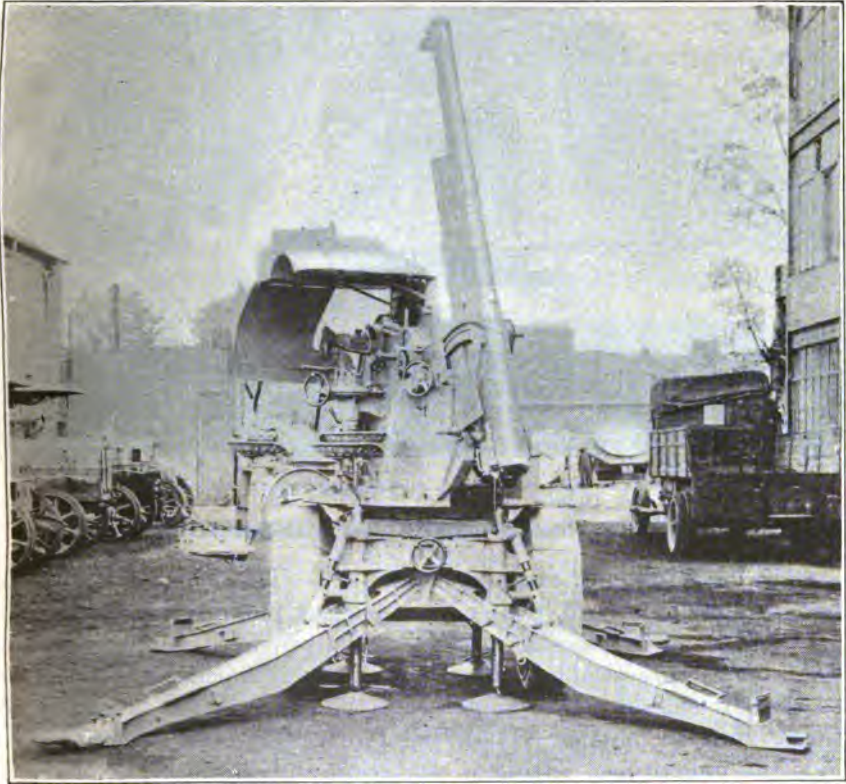
FIG. 43.—French 75-mm. A. A. gun on trailer carriage.
