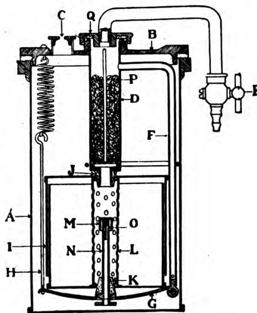
FIG. 6.—Signal lantern generator.
