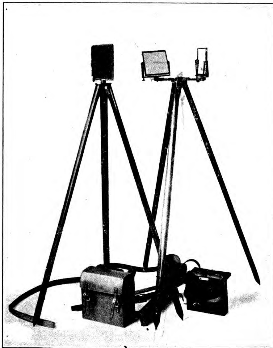
FIG. 1.—Heliograph assembled.
