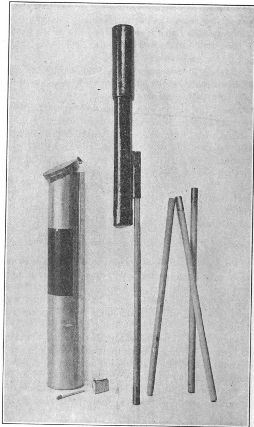
FIG. 11.—Signaling rocket and accessories.
