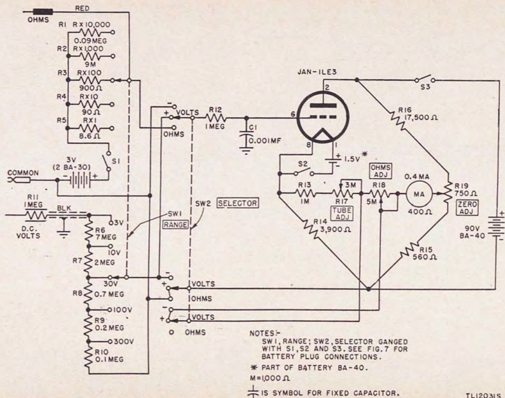
Figure 11. Voltohmmeter I-107-A, above serial No. 50, and Voltohmmeters I-107-B and C, schematic diagram.
