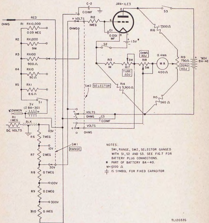
Figure 13. Volt ohmmeters I-107-E, F, and G, schematic diagram.
