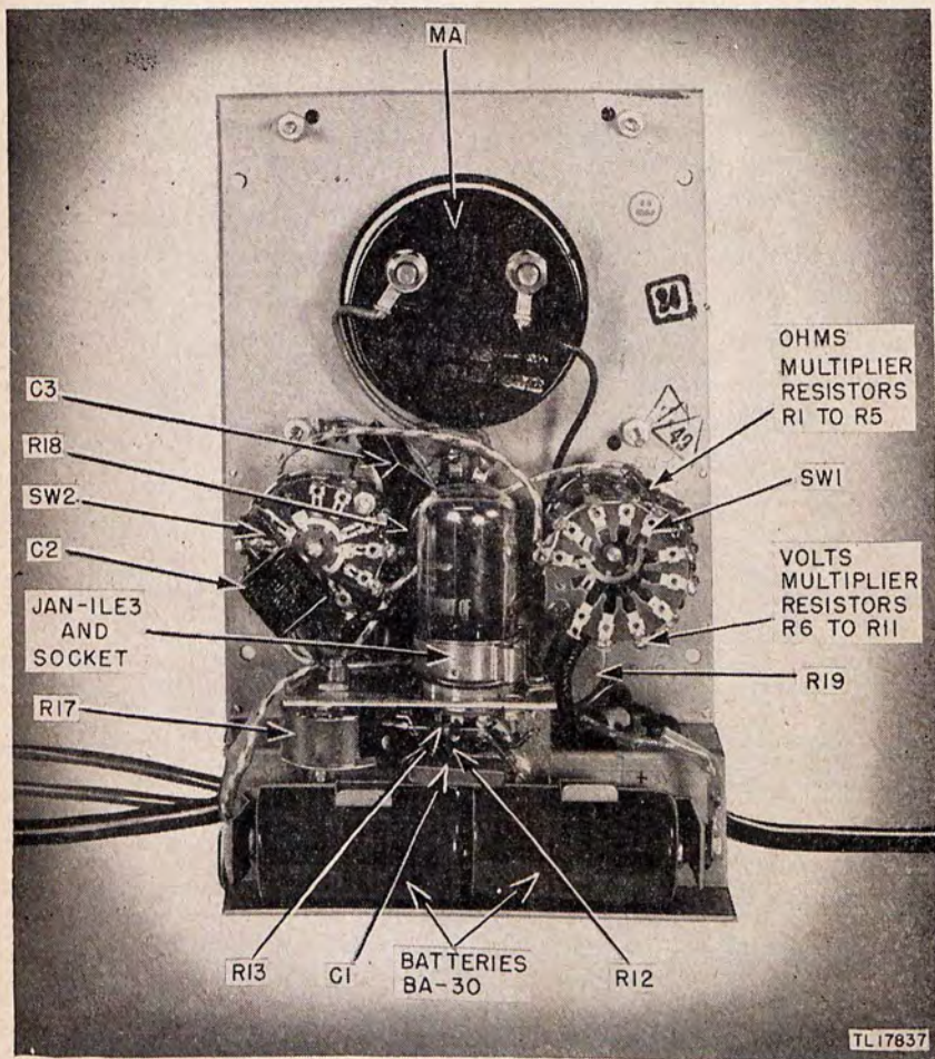
Figure 7. Voltohmmeter I-107-G, rear view.
