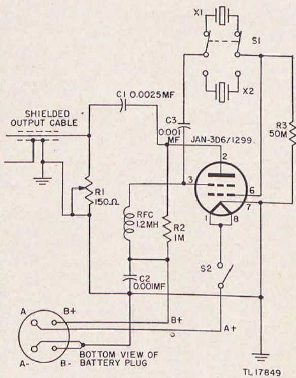
Figure 14. Oscillator VO-4(*), schematic diagram.
