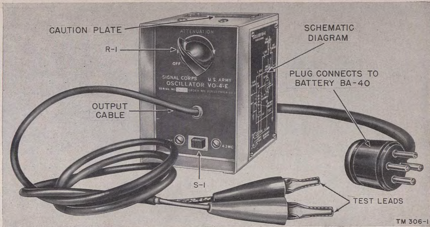
Figure 1.1 (added). Oscillator VO-4-E (RF).
