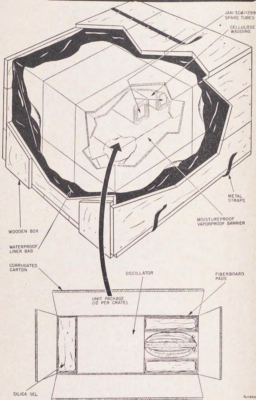
Figure 5. Typical packaging of Oscillator VO-4-(*).
