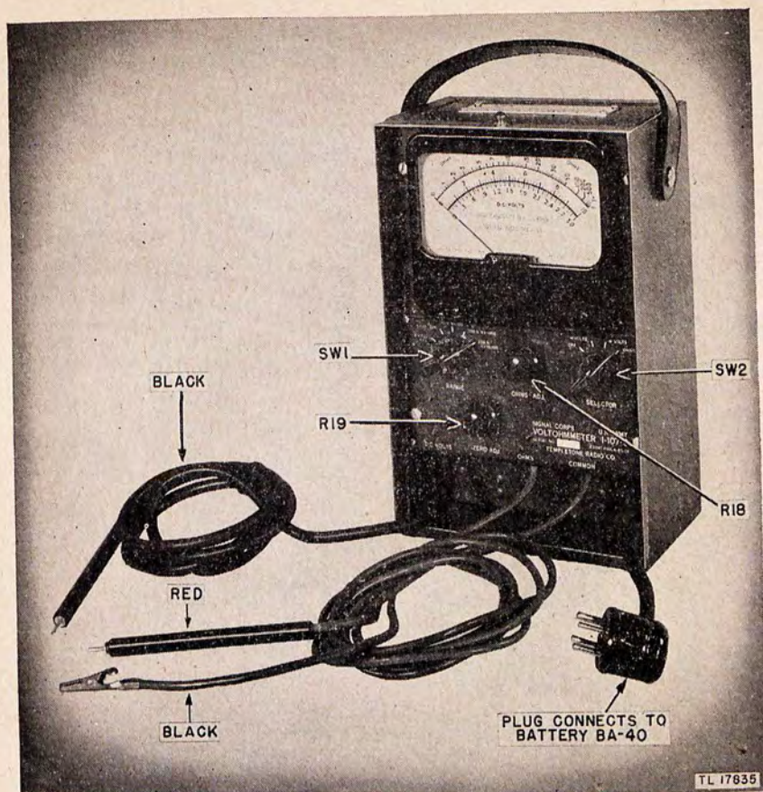
Figure 2. Voltohmmeter I-107-G, front view.
