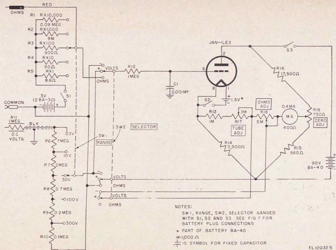
Figure 12. Volt-ohmmeter I-107-D, schematic diagram.
