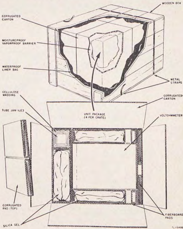
Figure 4. Typical packaging of Voltohmmeter I-107-(*).
