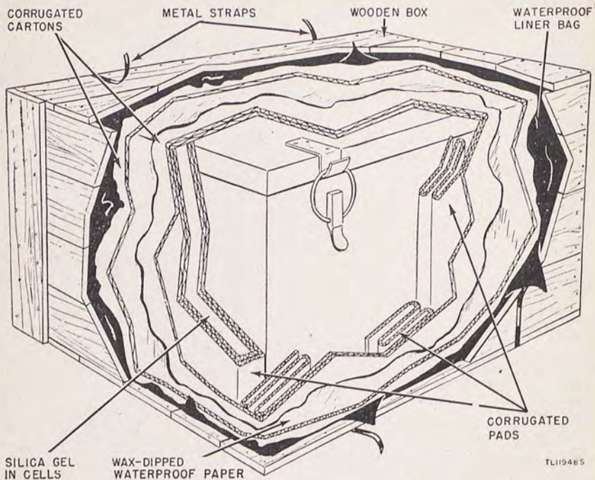
Figure 3. Typical export packaging of Maintenance Equipment ME-13-(*).
