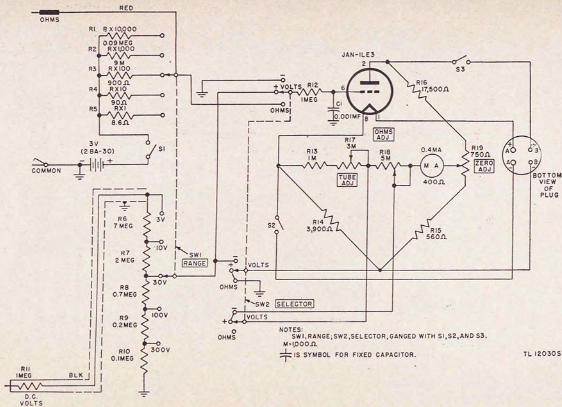
Figure 10. Volt-ohmmeter I-107-A, serial Nos. 1 to 50, inclusive, schematic diagram.
