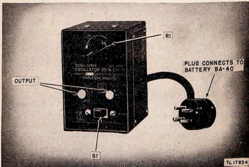
Figure 1. Oscillator VO-4-D, front view.
