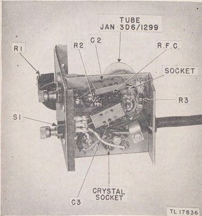
Figure 6. Oscillator VO-4-D, bottom view.
