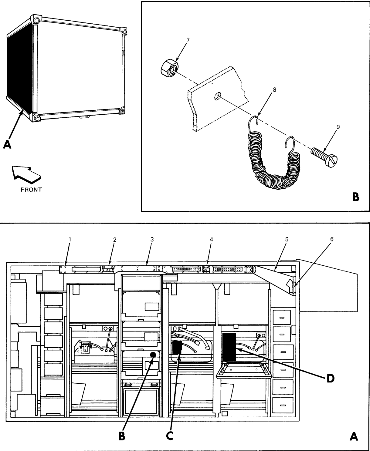
Figure 3. Shelter, Modified S-348A/TSC-58A, Roadside (Sheet 1 of 2).
