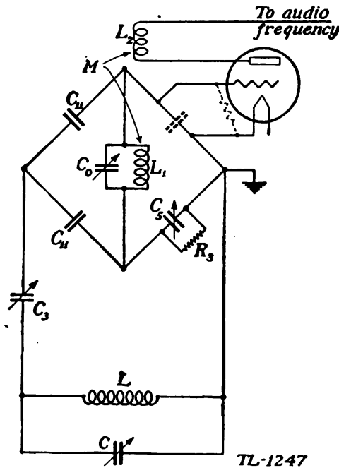
FIGURE 10.—Simplified receiver circuit.
