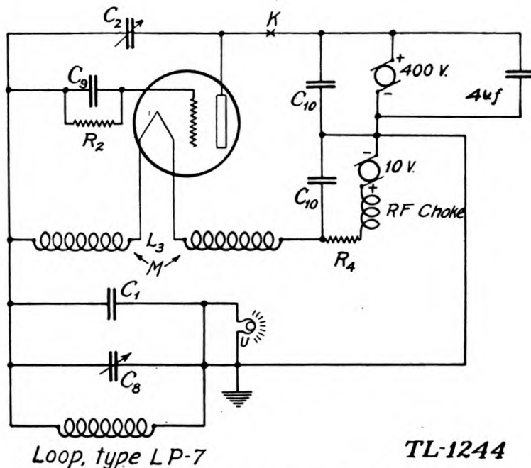
FIGURE 7.—Schematic transmitter circuit.
