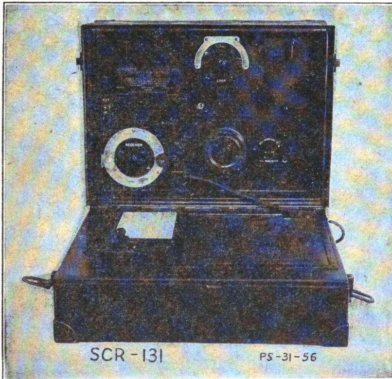
FIGURE 2.—Radio receiver and transmitter BC-148 (151), front view.
