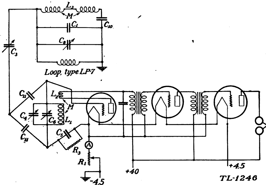
FIGURE 9.—Schematic receiver circuit.
