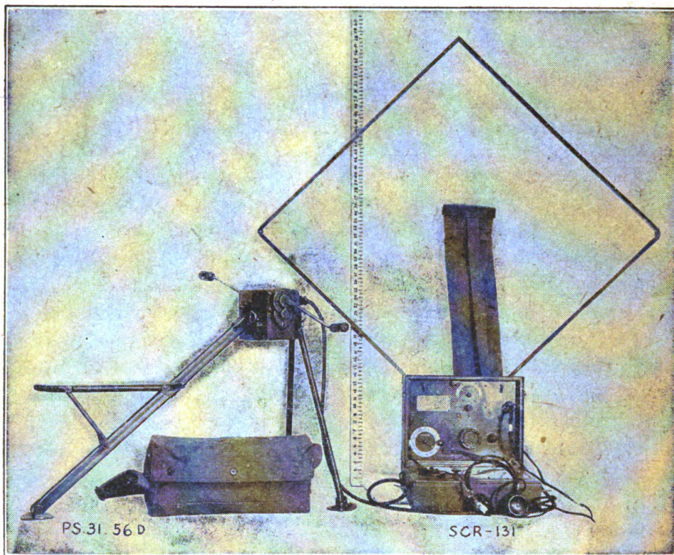
FIGURE 1.—Radio set SCR-131 (161), set up for operation.
