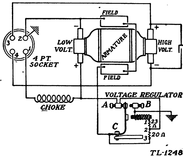
FIGURE 11.—Wiring diagram GN-35.
