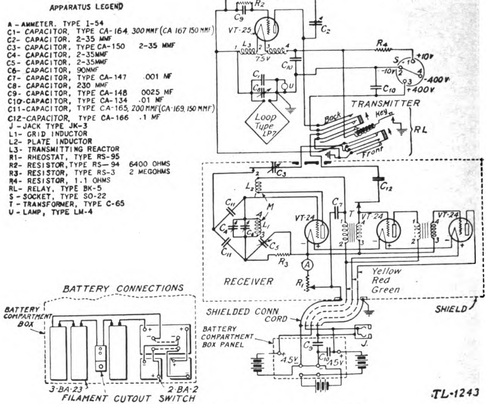
FIGURE 6.—Circuit diagram, SCR-131 (161).
