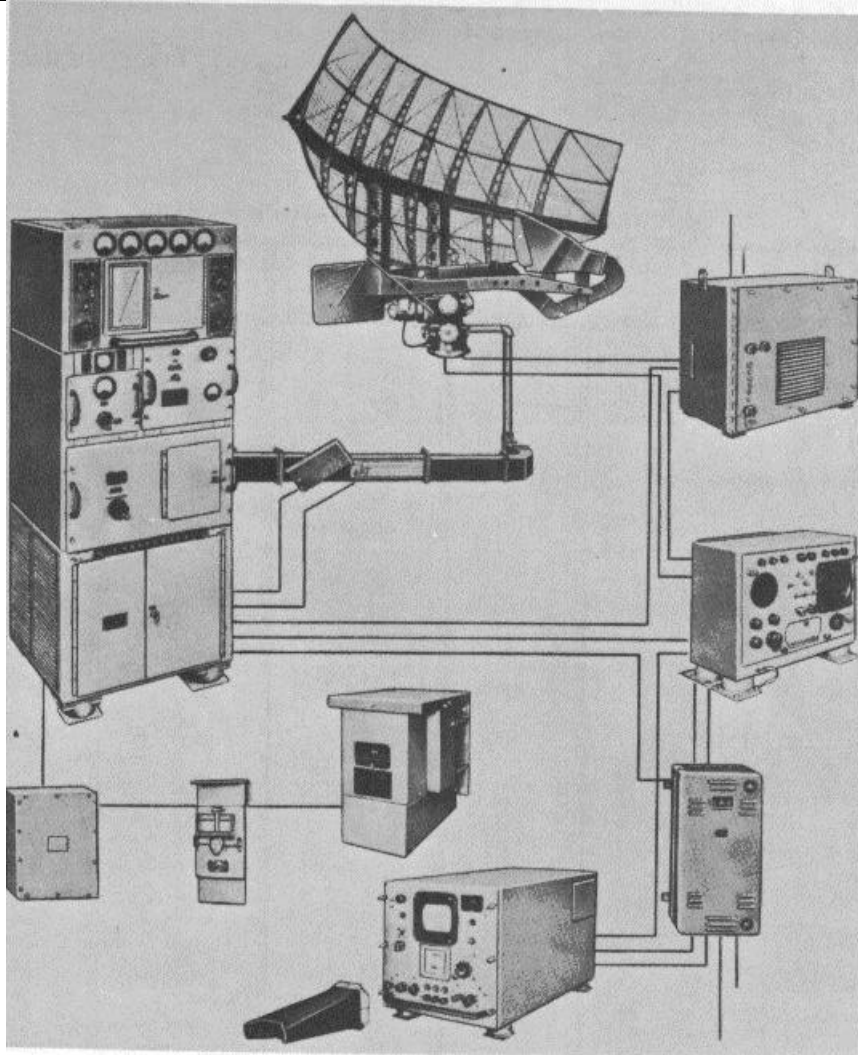
AN/SPS-6: 1
