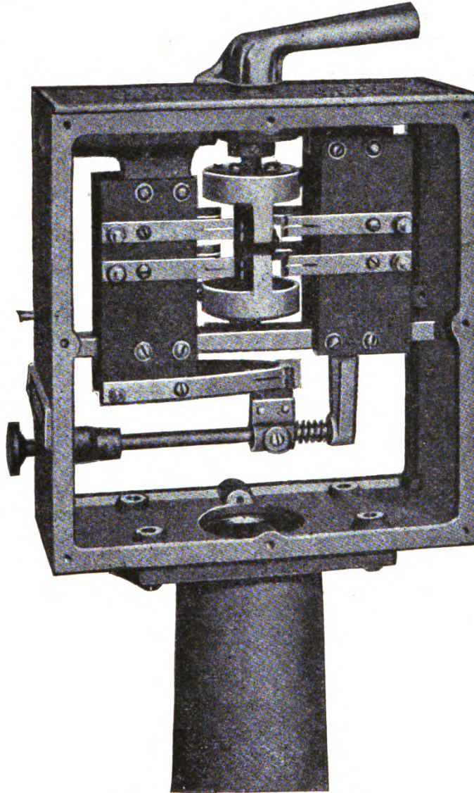
FIG. 41.—Truck-light controller.
