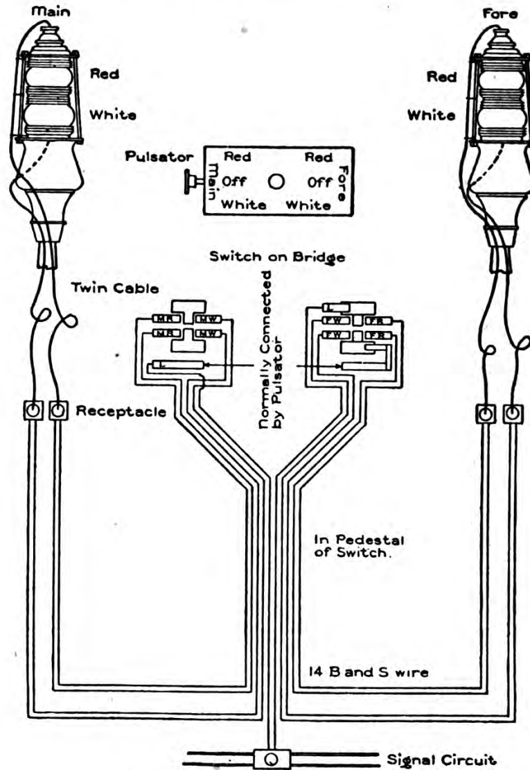
FIG. 40.—Wiring diagram, truck lights.
