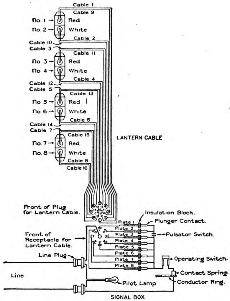
FIG. 38.—Diagram of Connections of Night Signal Set.
