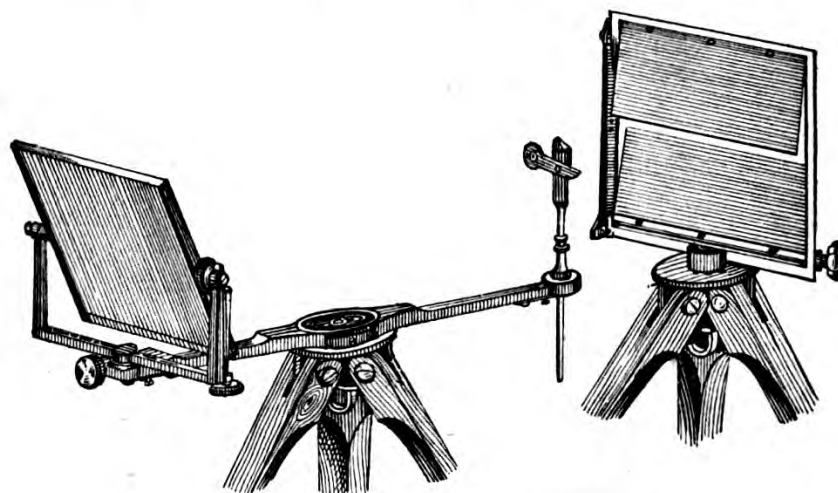
FIG. 8.—Heliograph in use with one mirror.
