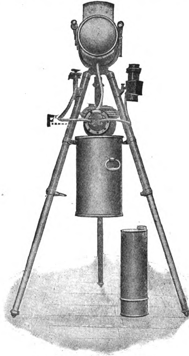
FIG. 29.—Station Signaling Lantern.
