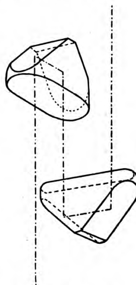
FIG. 45.—Porro prism.
