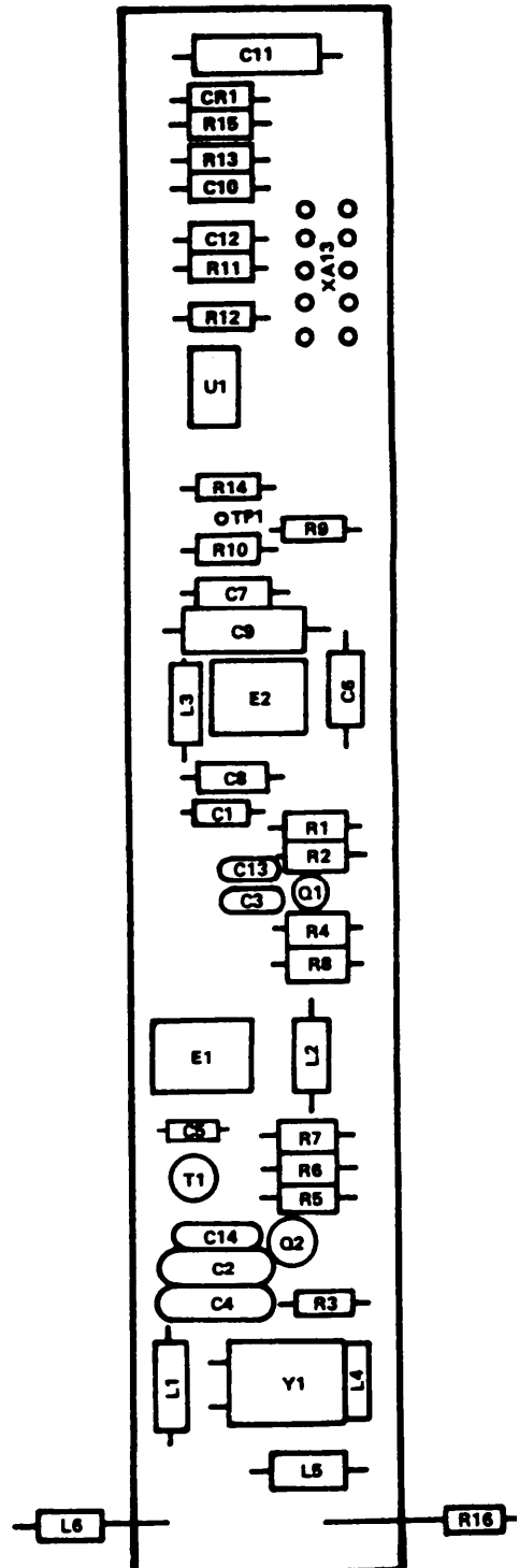
Figure 14. Circuit Card Assembly, 47-MHz APC
