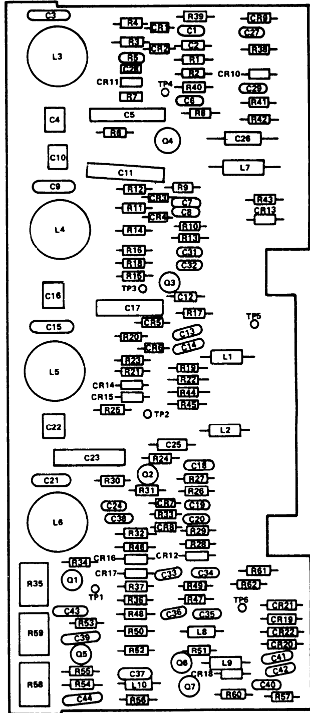
Figure 2. Circuit Card Assembly, LC Filter
