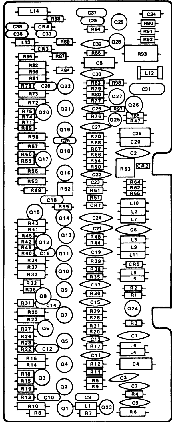
Figure 10. Circuit Card Assembly, Log Amplifier
