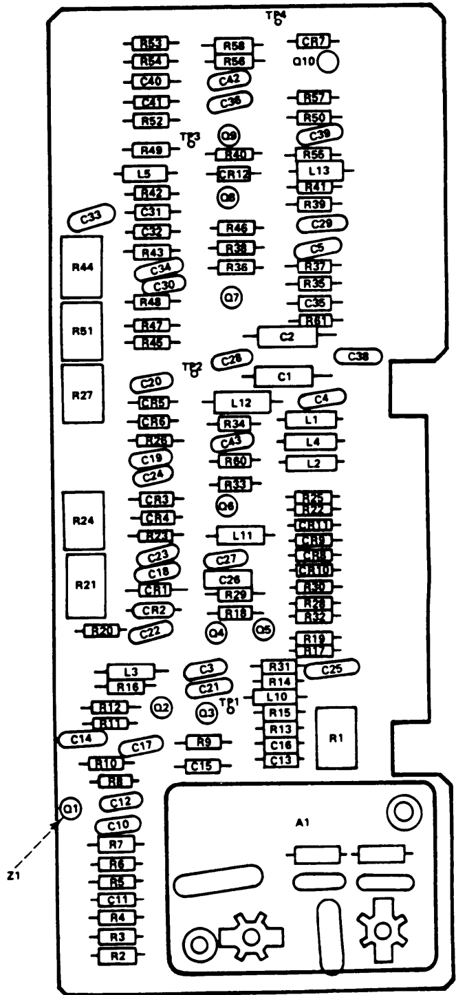
Figure 3. 3-MHz Amplifier Board Assembly
