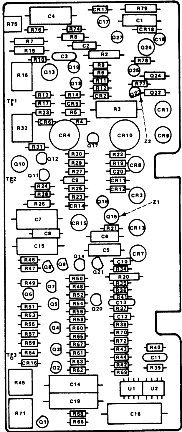
Figure 7. Circuit Card Assembly, Power Supply
