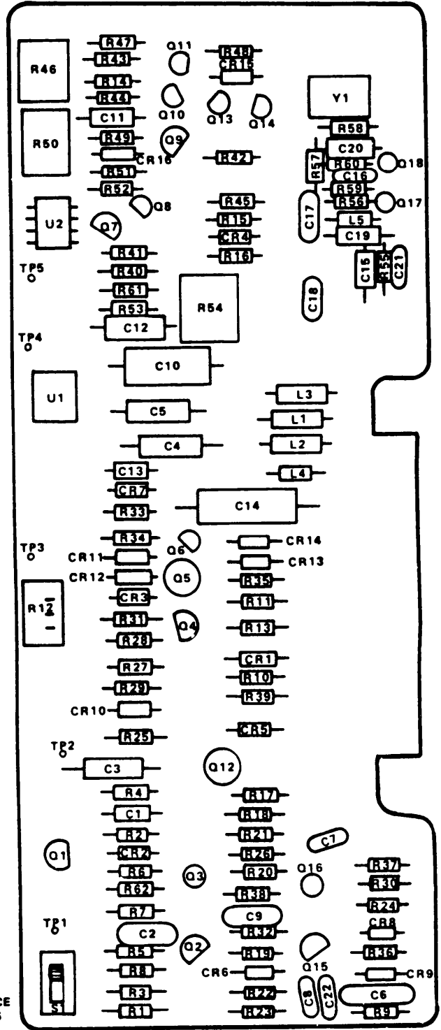
Figure 8. Circuit Card Assembly, Scan Generator
