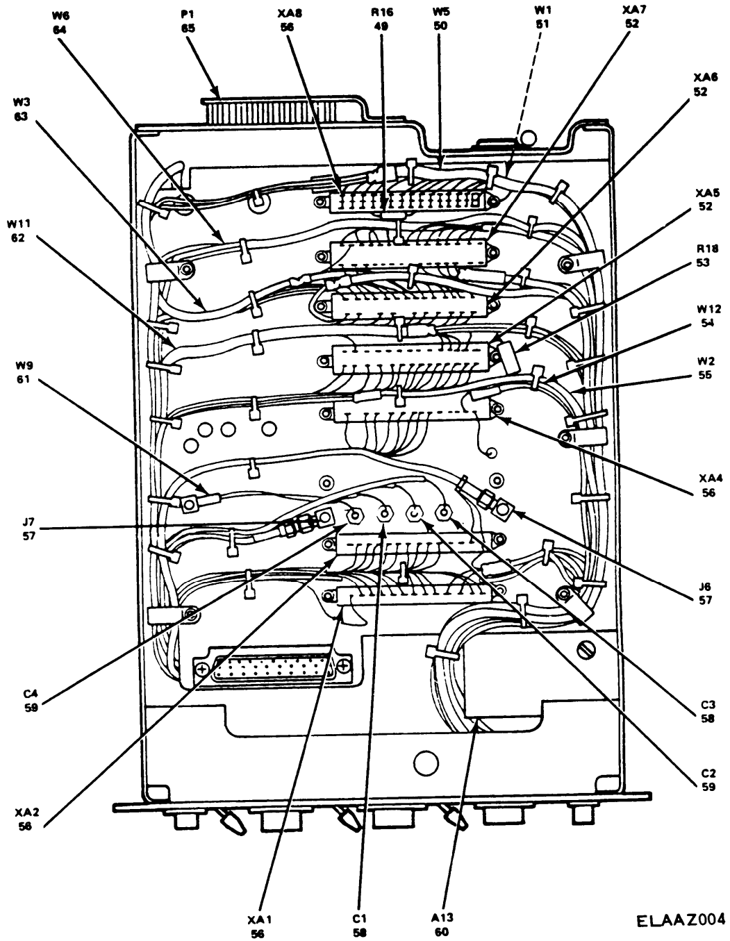
Figure 1. IF Plug-In PL-1388/U (Hewlett-Packard Model 8552B) (Sheet 4 of 6)
