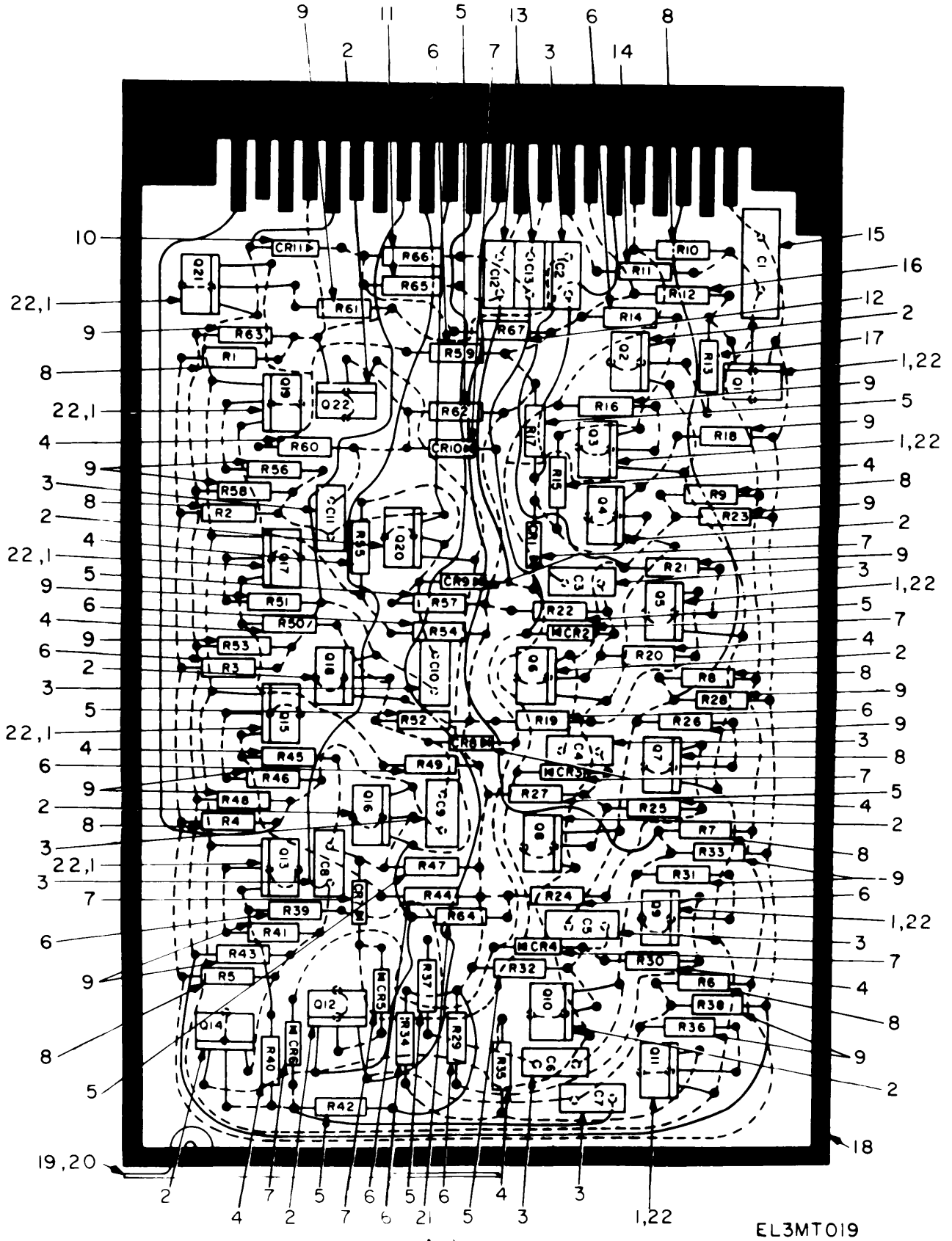
Figure 19. Test Set Subassembly A19.
