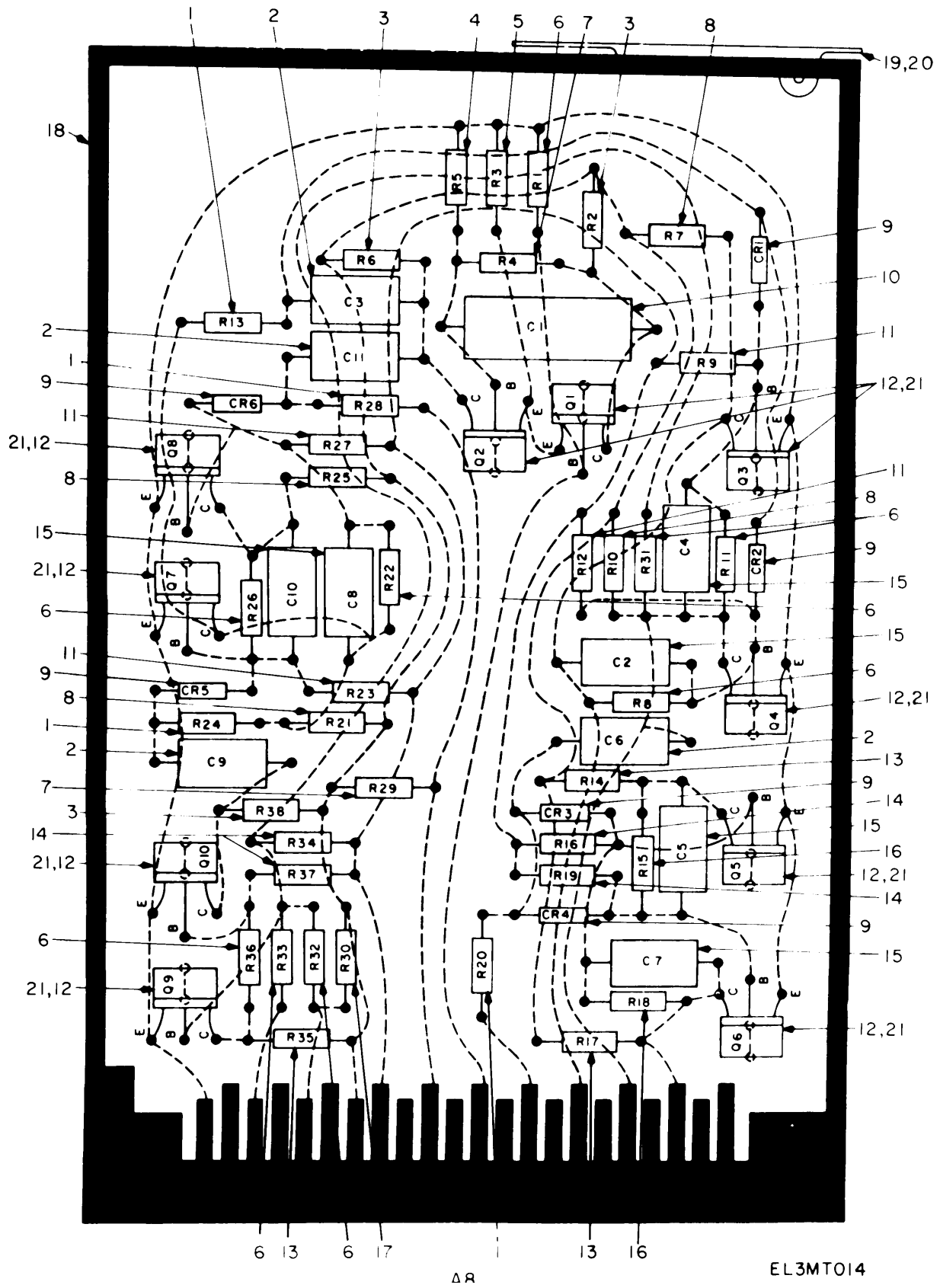
Figure 14. Test Set Subassembly A8.
