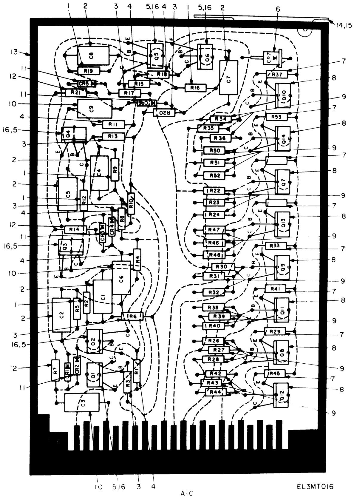
Figure 16. Test Set Subassembly
