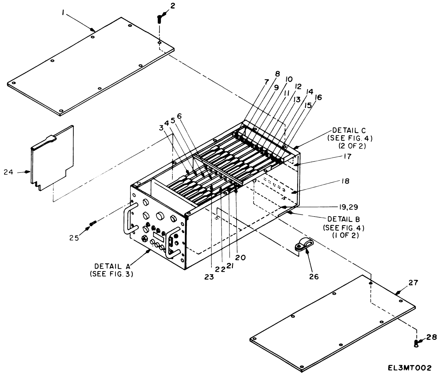
Figure 2. Teletypewriter Test Set (SMD552591 and SMD889357).
