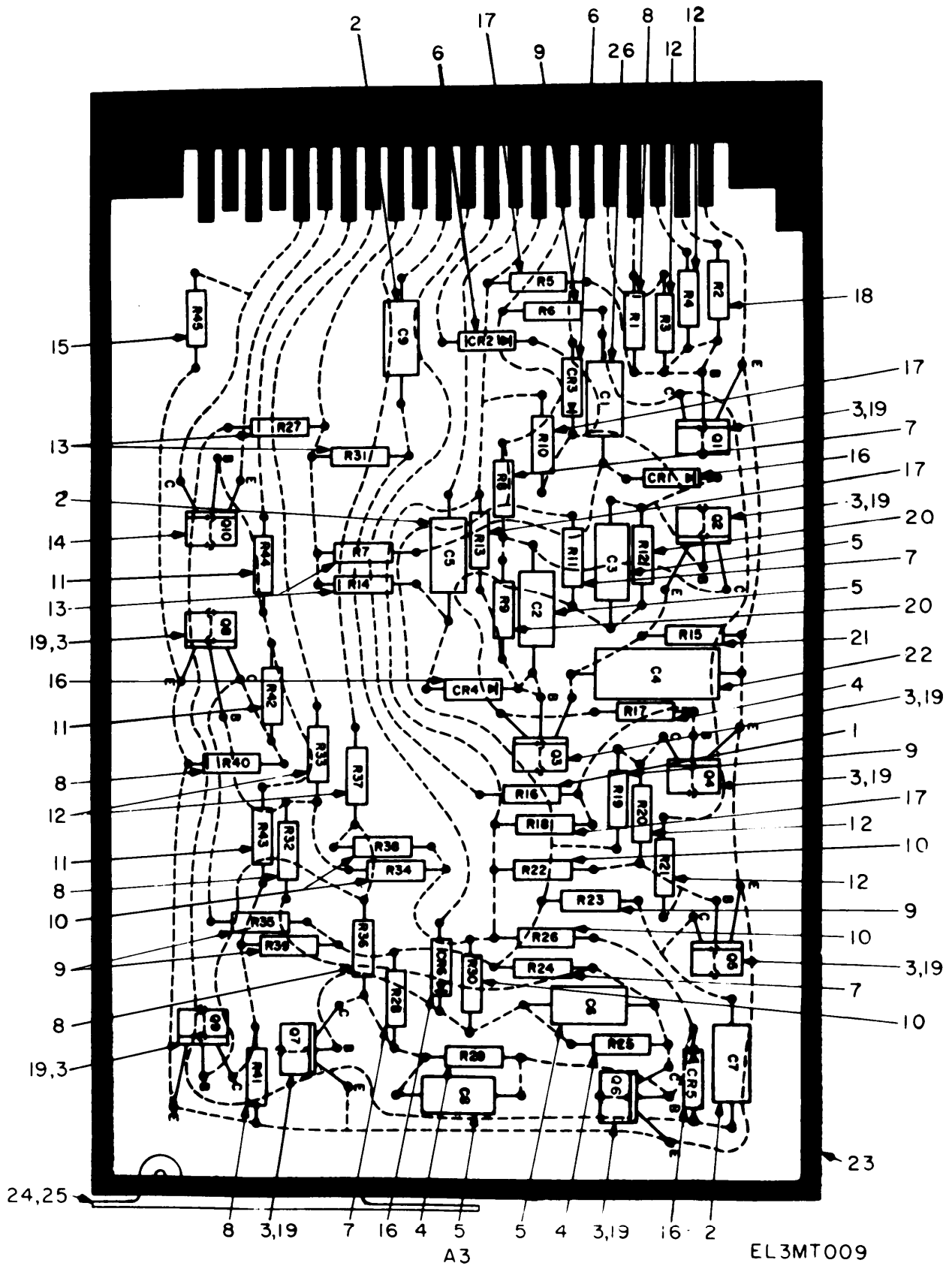
Figure 9. Test Set Subassembly A3.
