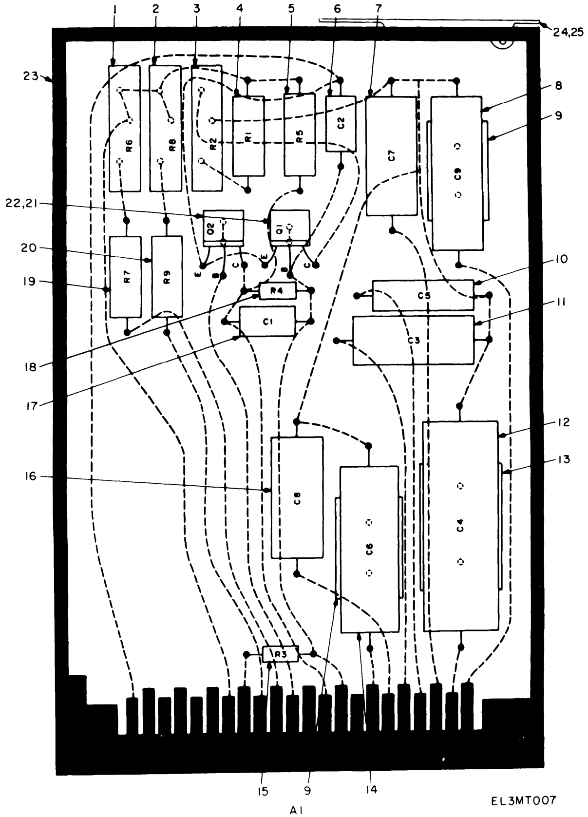
Figure 7. Test Set Subassembly A1.
