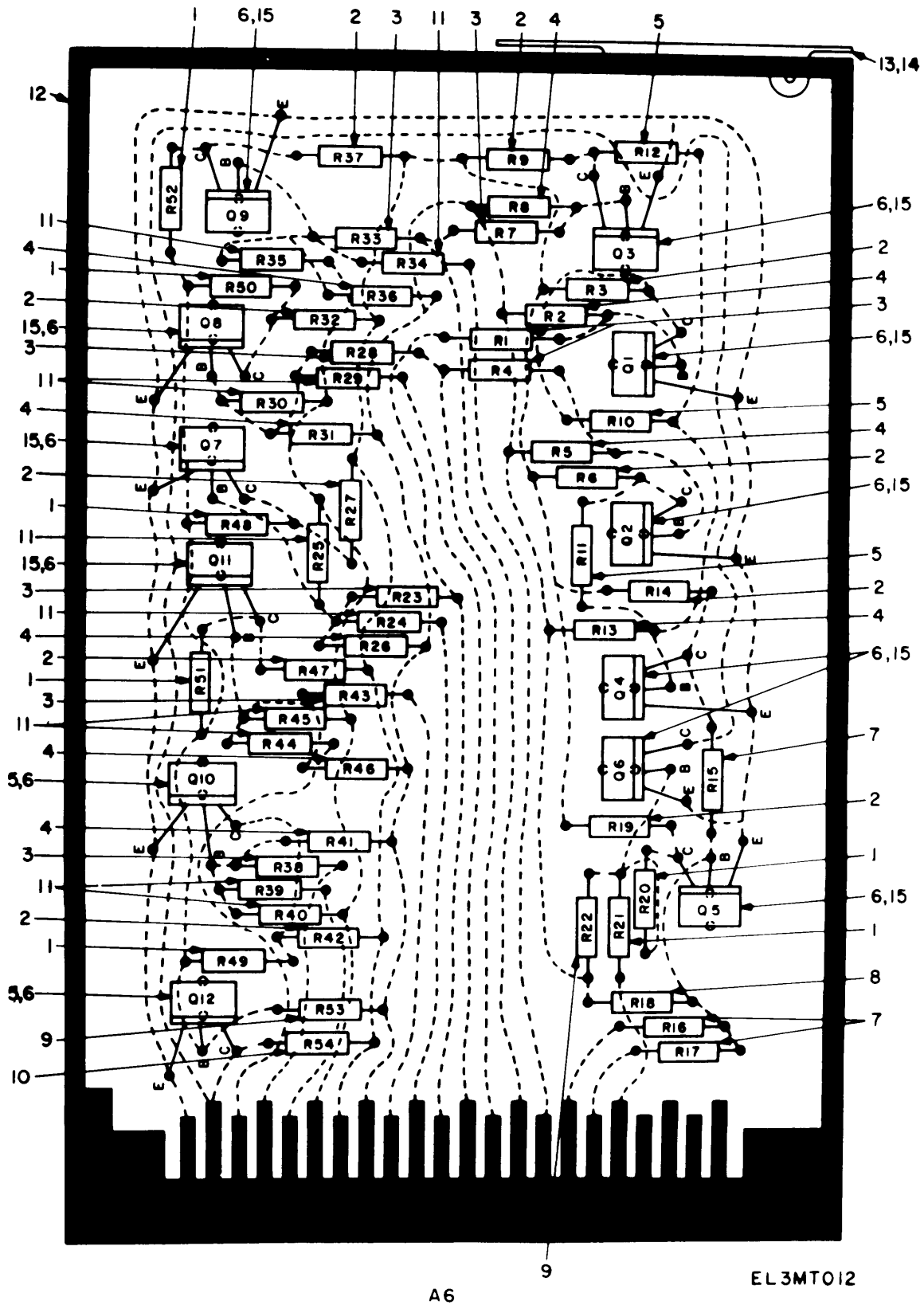
Figure 12. Test Set Subassembly A6.
