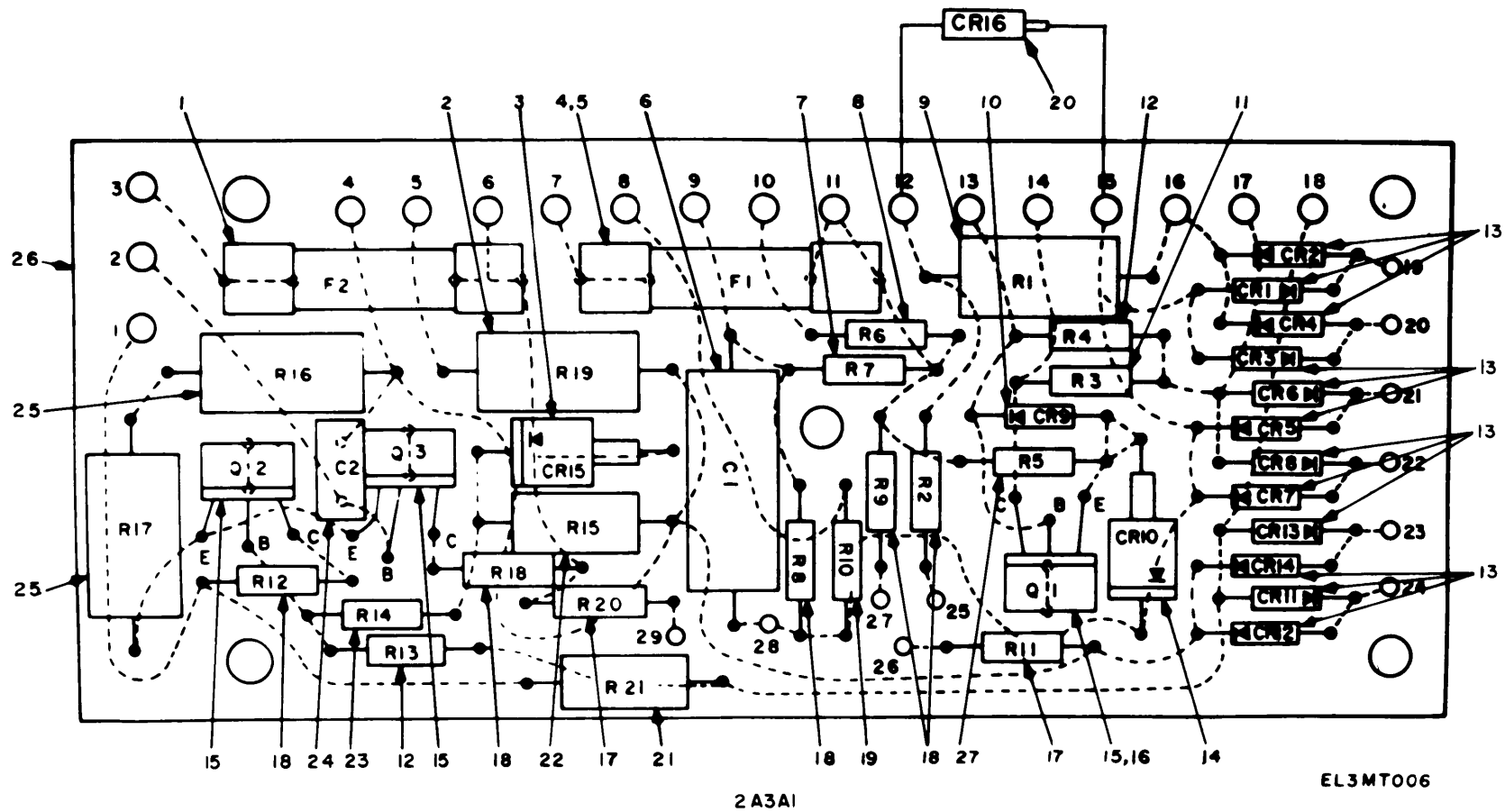
Figure 6. Component Board Assembly 2A3A1.
