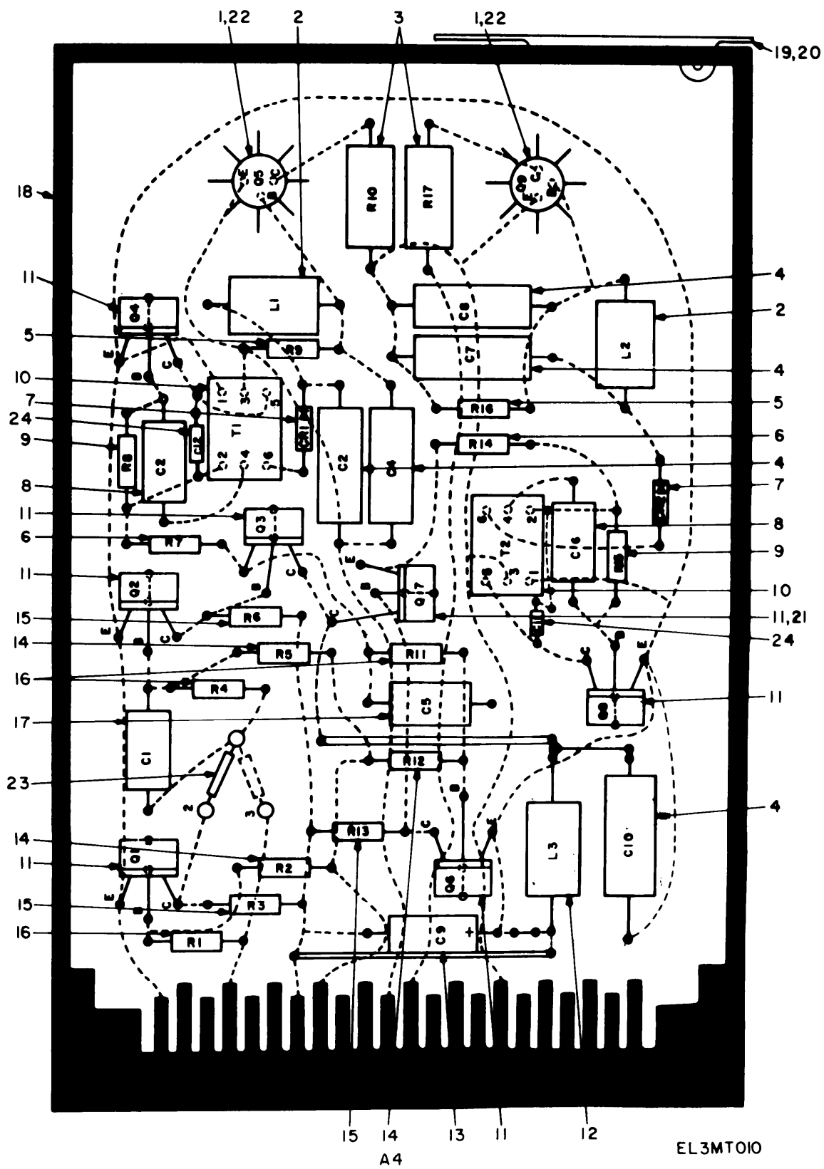
Figure 10. Test Set Subassembly A4.
