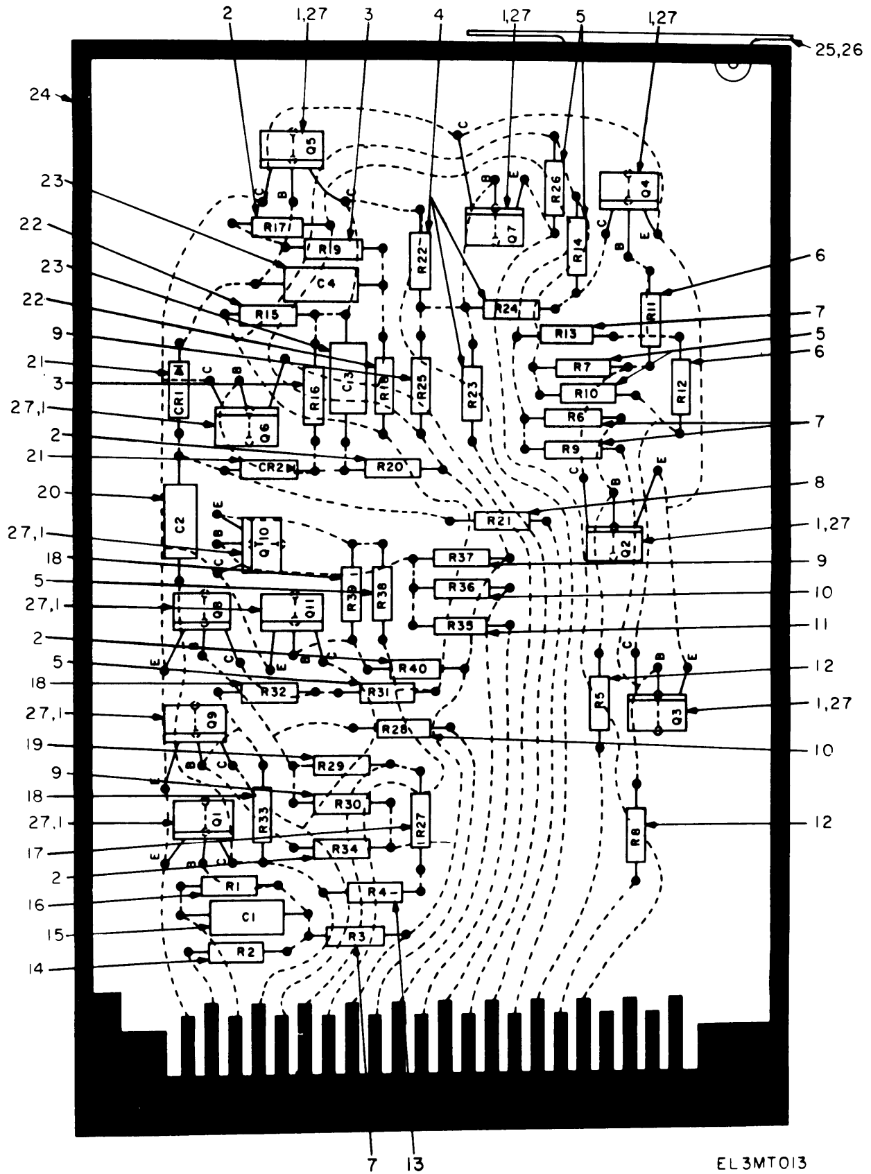
Figure 13. Test Set Subassembly A7.
