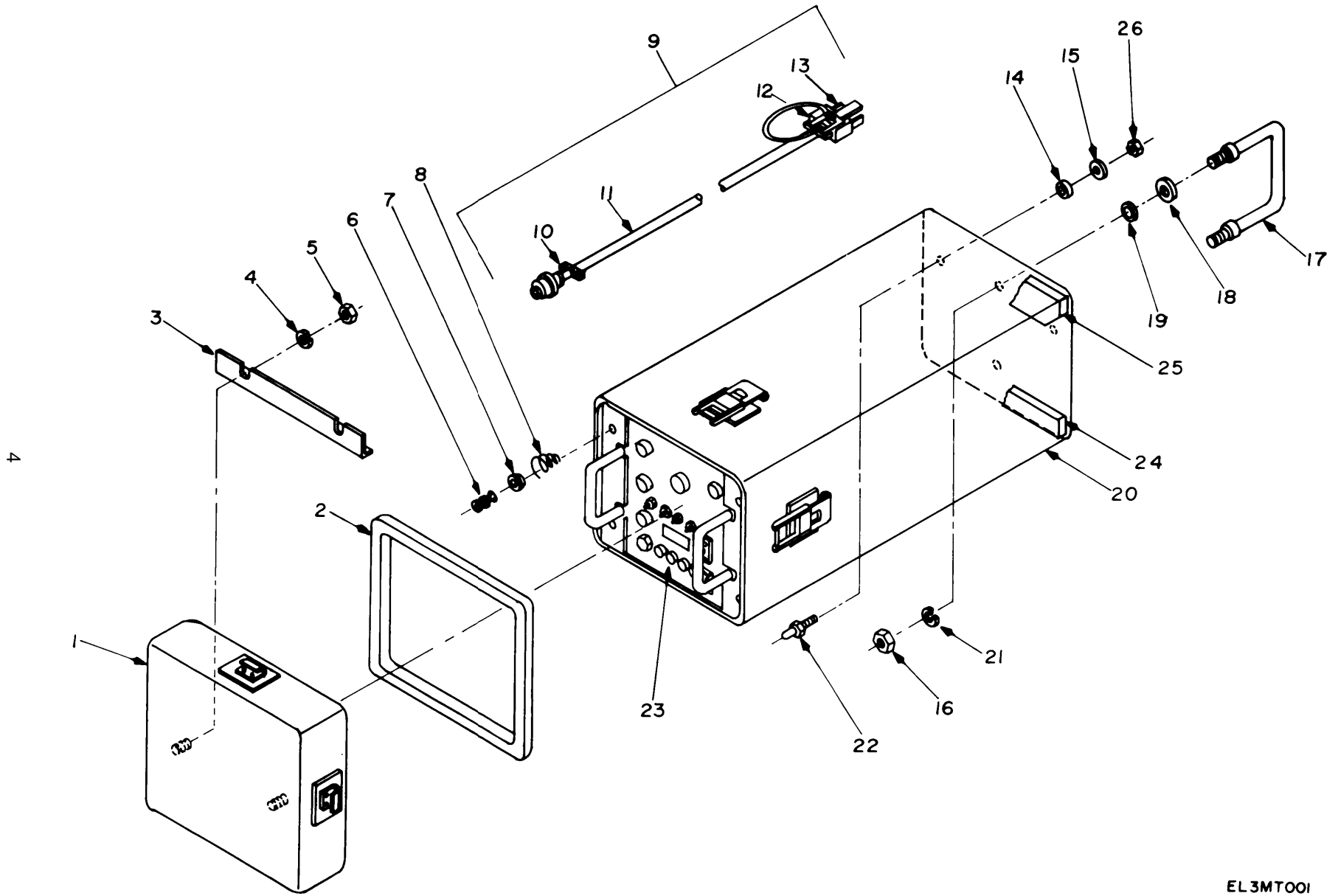
Figure 1. Teletypewriter Test Set TS-799/UGM-1 and TS-799A/UGM-1.
