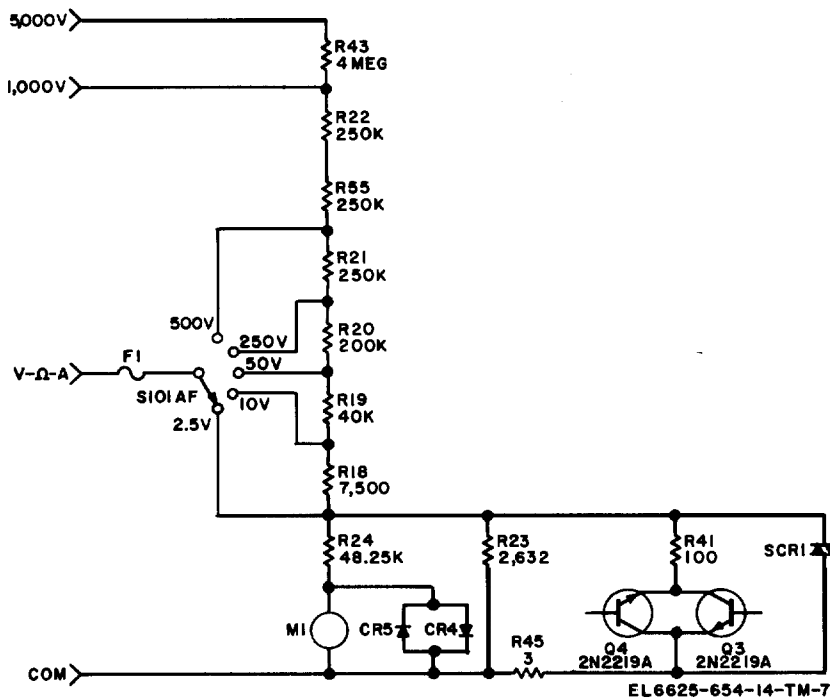
Figure 4-. Simplified 1K Ω/V Vdc circuit.
