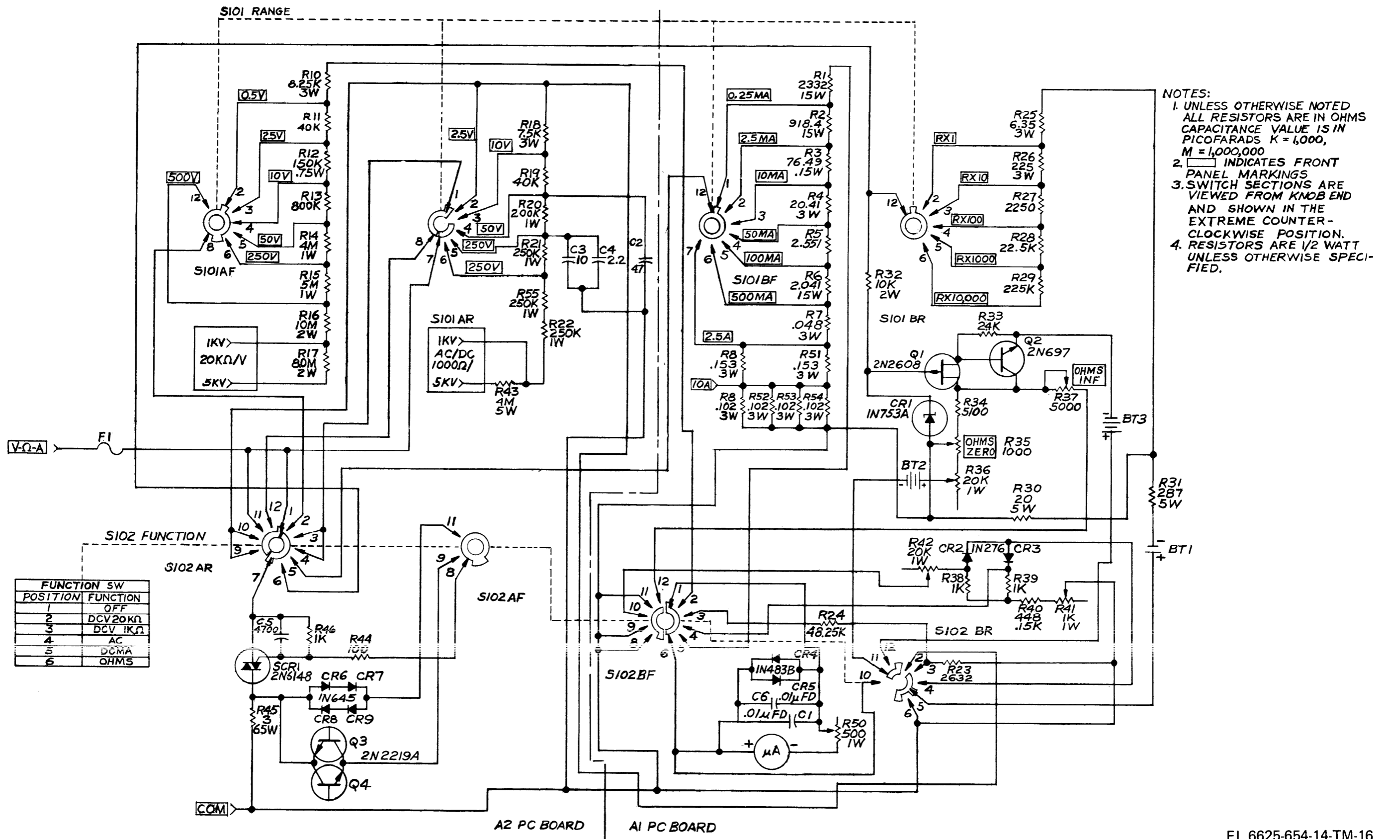
Figure 5-6. Multimeter AN/USM-223, schematic diagram.
