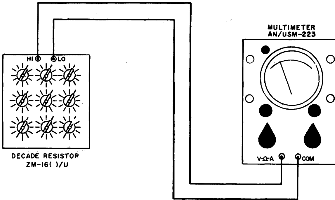
Figure 5-3. Ohmmeter function performance test connection.
