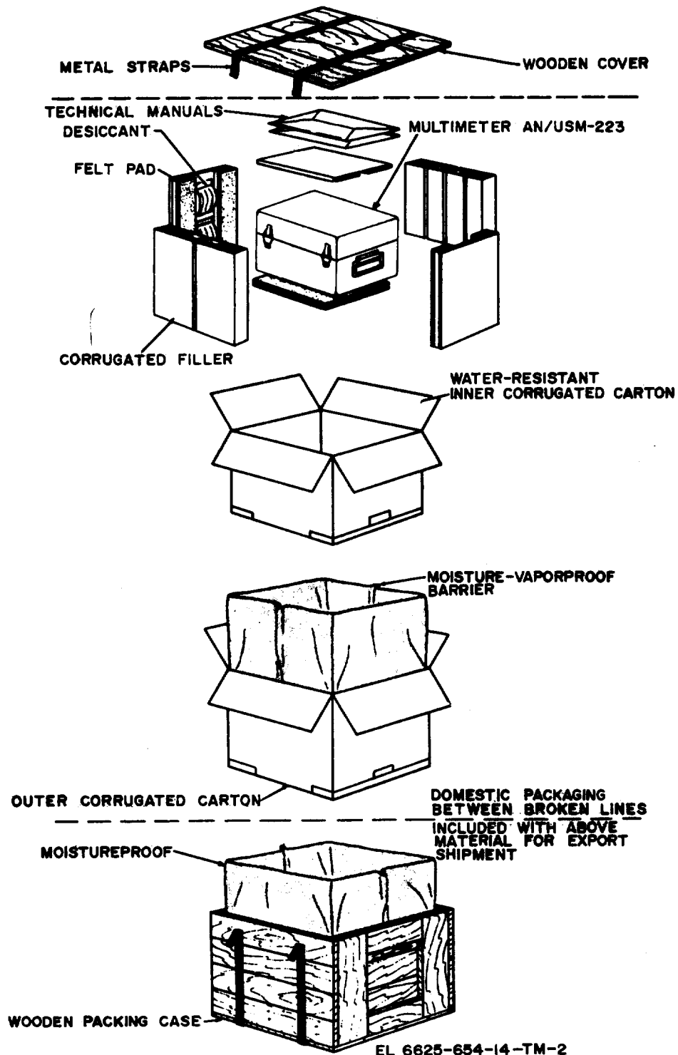
Figure 2-1. Packaging diagram.
