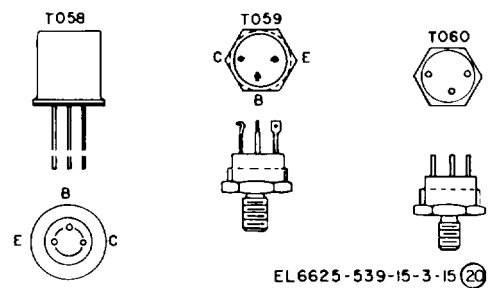
Figure D-1 (20). Transistor outline drawings (part 20 of 20).
