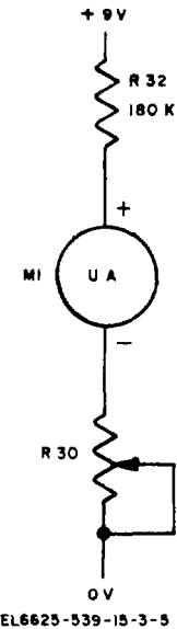
Figure 5-1. Battery check, simplified schematic diagram.
