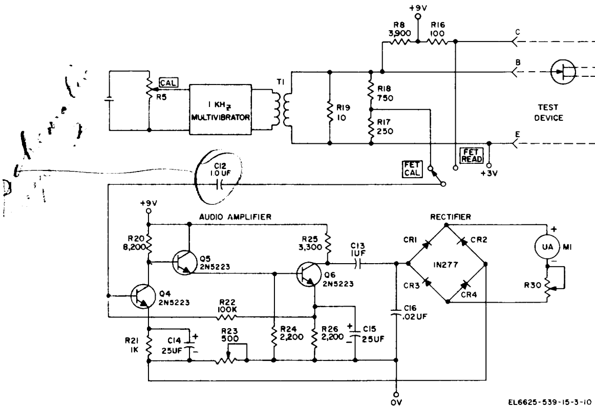
Figure 5-6. F. E. T. checks, simplified schematic diagram.
