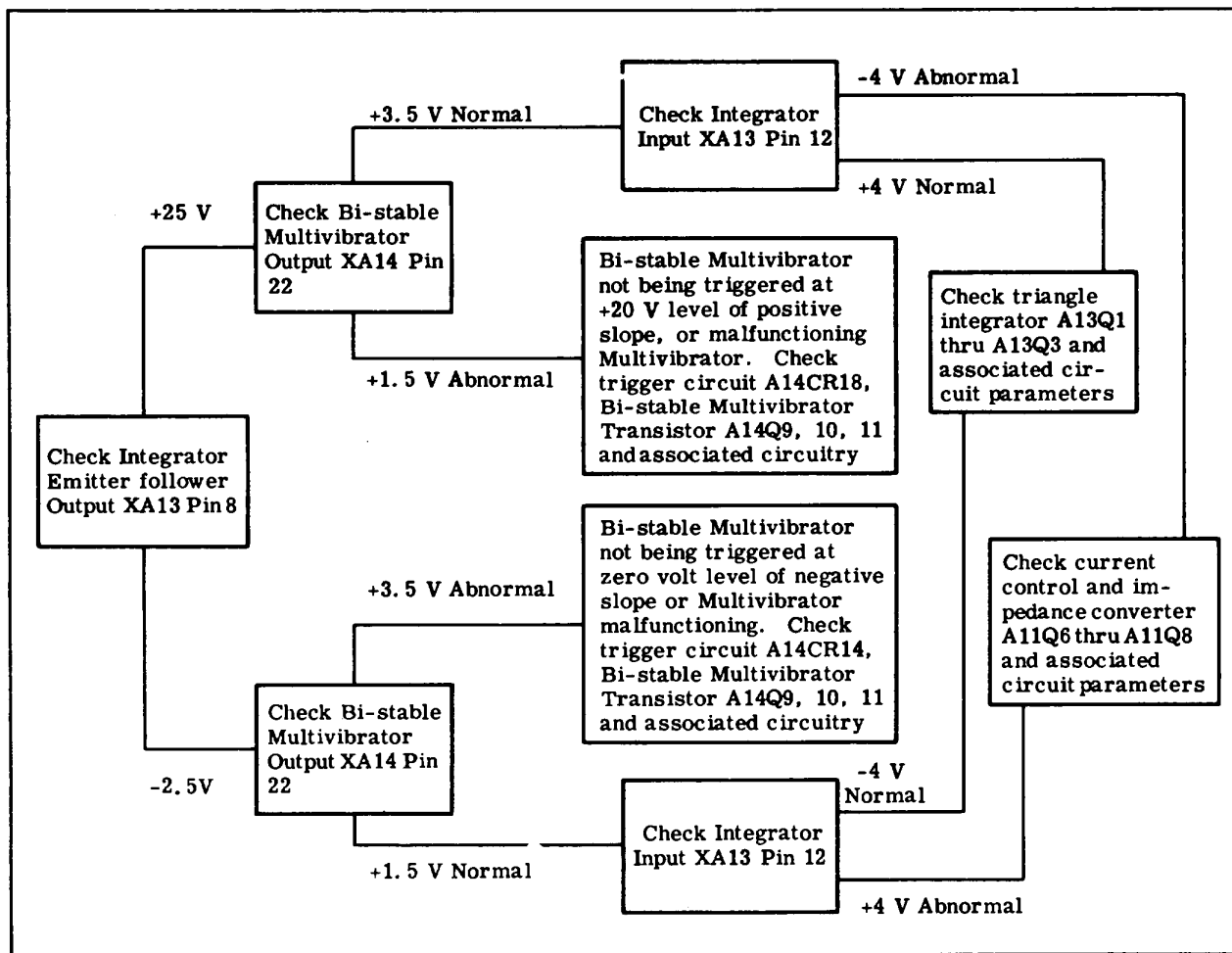
Figure 5-8. Troubleshooting Tree
