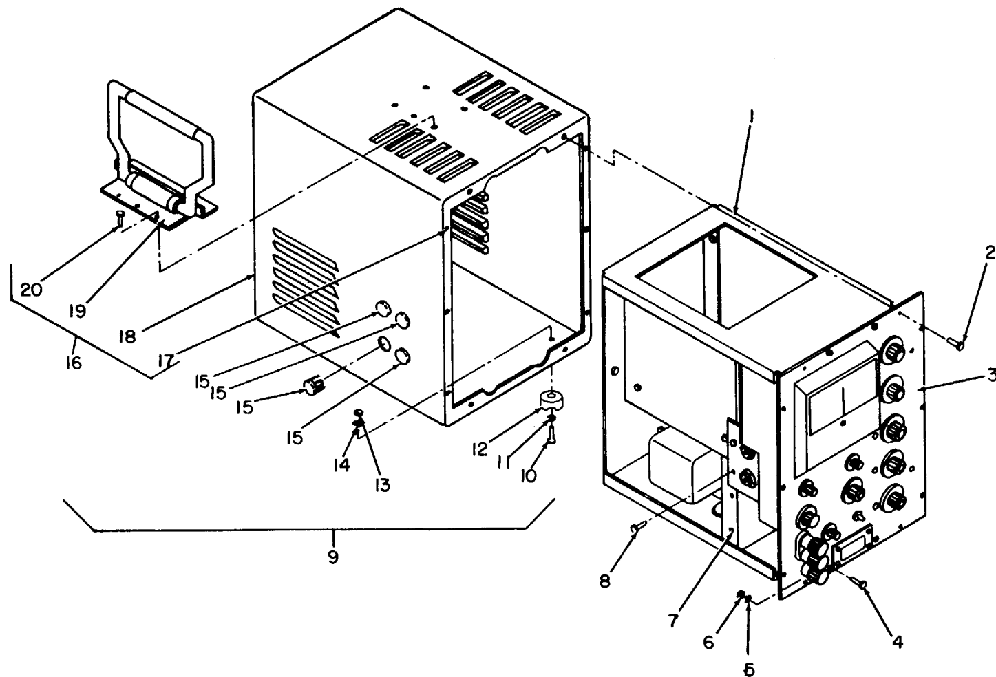
Figure 2. Voltmeter, Electronic ME-161B/U.
