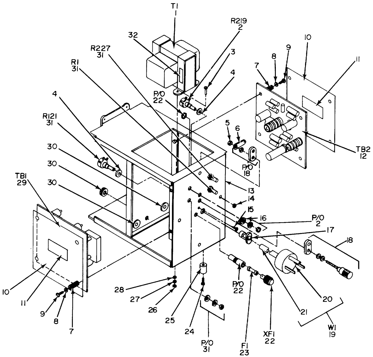
Figure 3. Voltmeter, Electronic ME-161B/U, Chassis Electrical Equipment.
