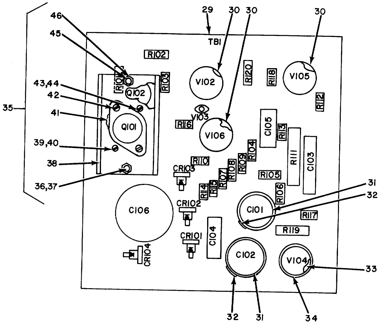
Figure 10. Voltmeter, Electronic ME-161B/U, Circuit Card Assembly, TB1 (Sheet 1 of 2).
