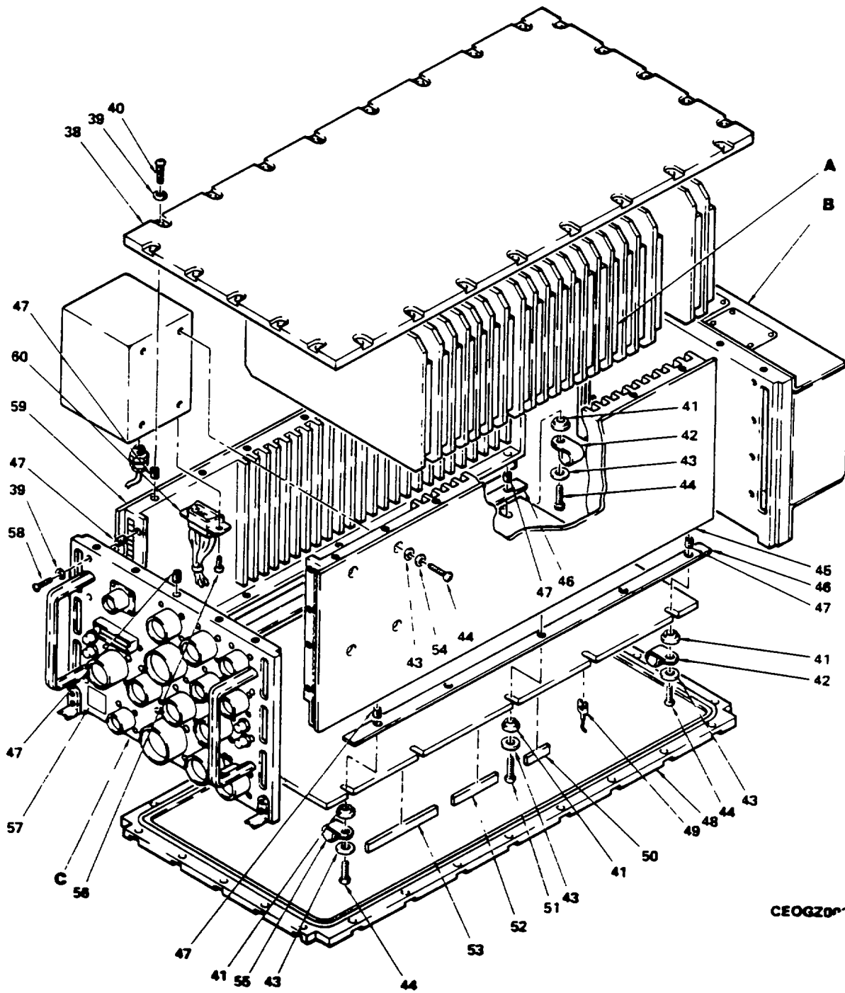
Figure 1. Interface Unit J-4522/U (Sheet 2 of 41)
