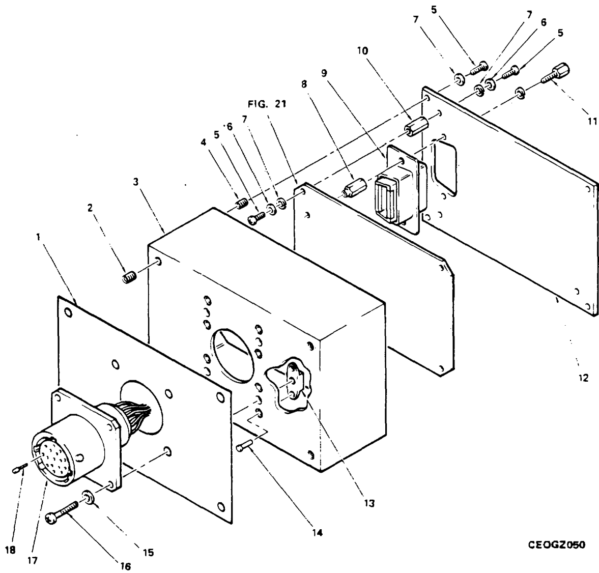
Figure 20. Module Assembly, NAV Filter (FL1)
