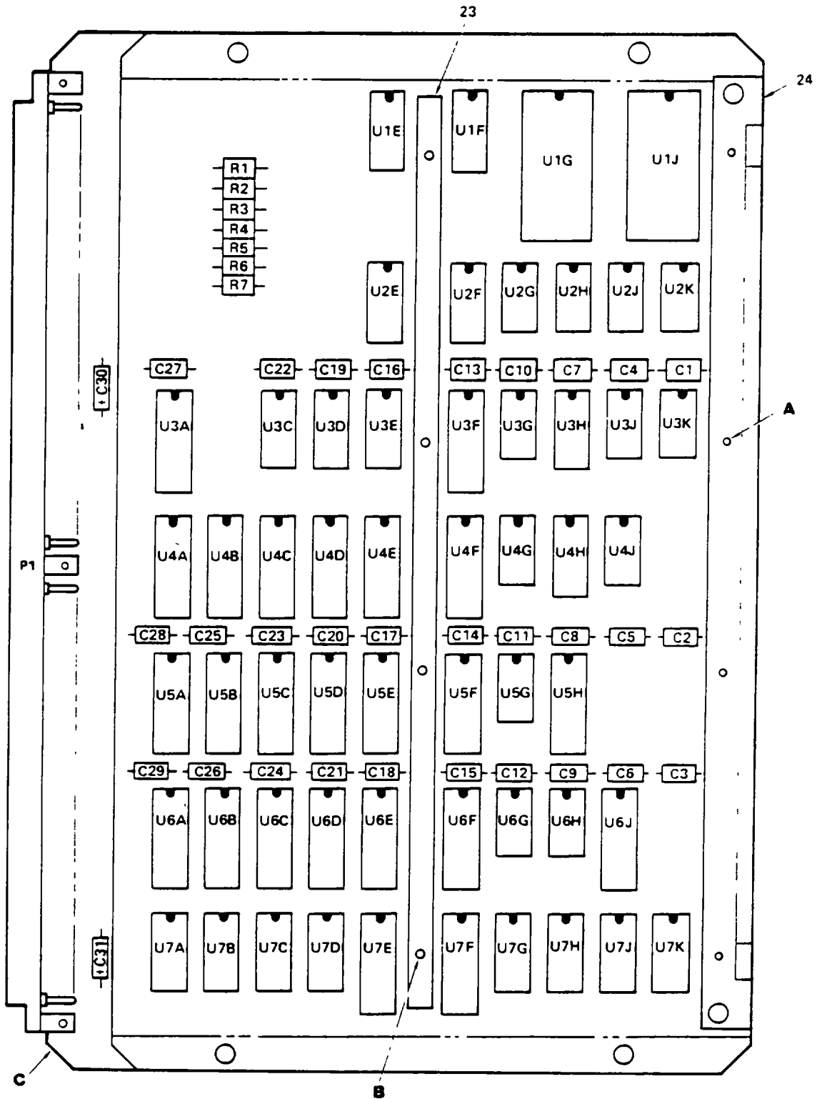
Figure 8. Circuit Card Assembly, IU NAV (A16) (Sheet 1 of 2)
