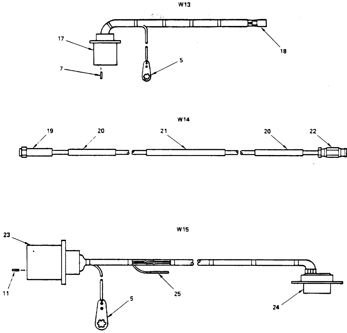
Figure 23. Cable Assemblies W1-W15 (Sheet 3 of 3)
