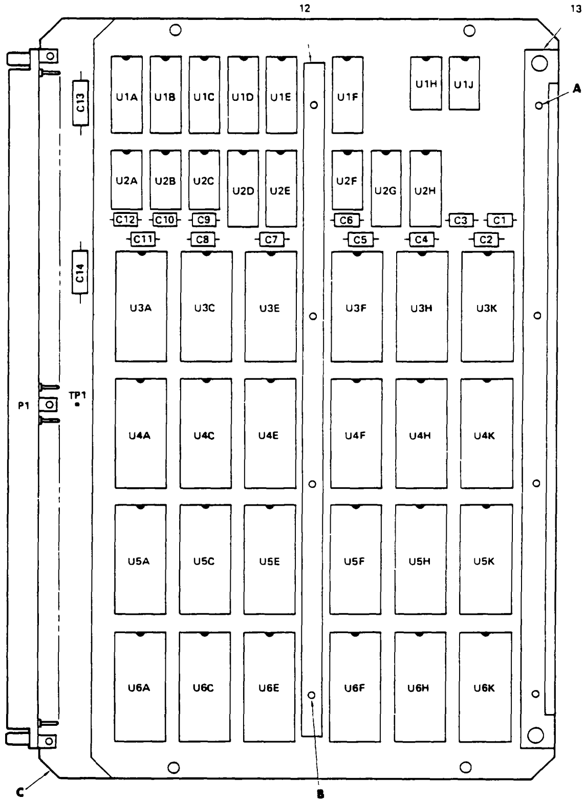
Figure 7. Circuit Card Assembly, Static Ram (A17, A21) (Sheet 1 of 2)
