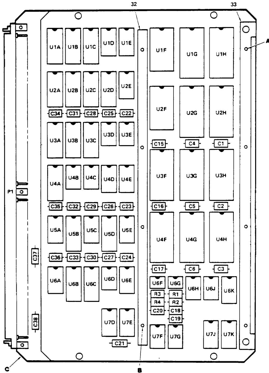
Figure 2. Circuit Card Assembly, IU BUS 1 (A20) (Sheet 1 of 2)
