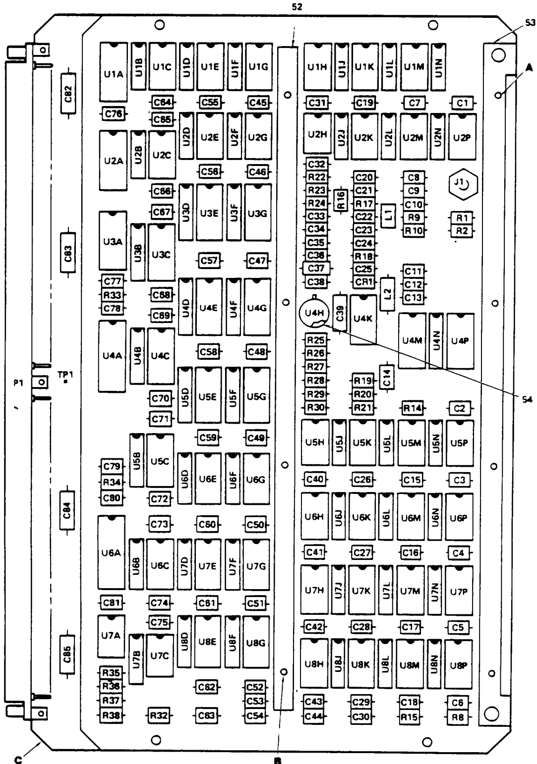
Figure 4. Circuit Card Assembly, MOIA (A1) (Sheet 1 of 3)
