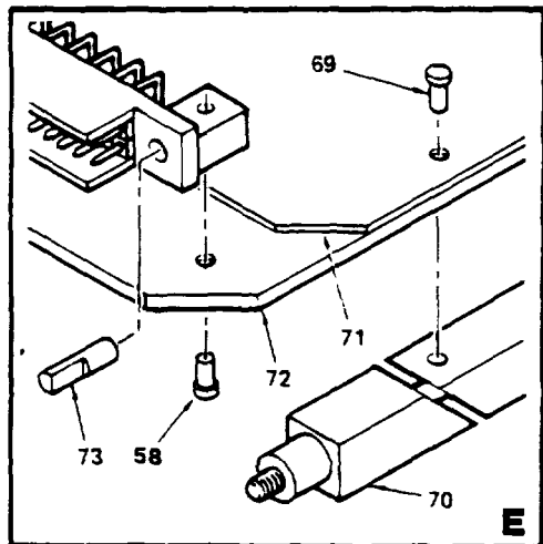
Figure 14. Circuit Card Assembly, Battery Regulator (A3) (Sheet 3 of 3)
