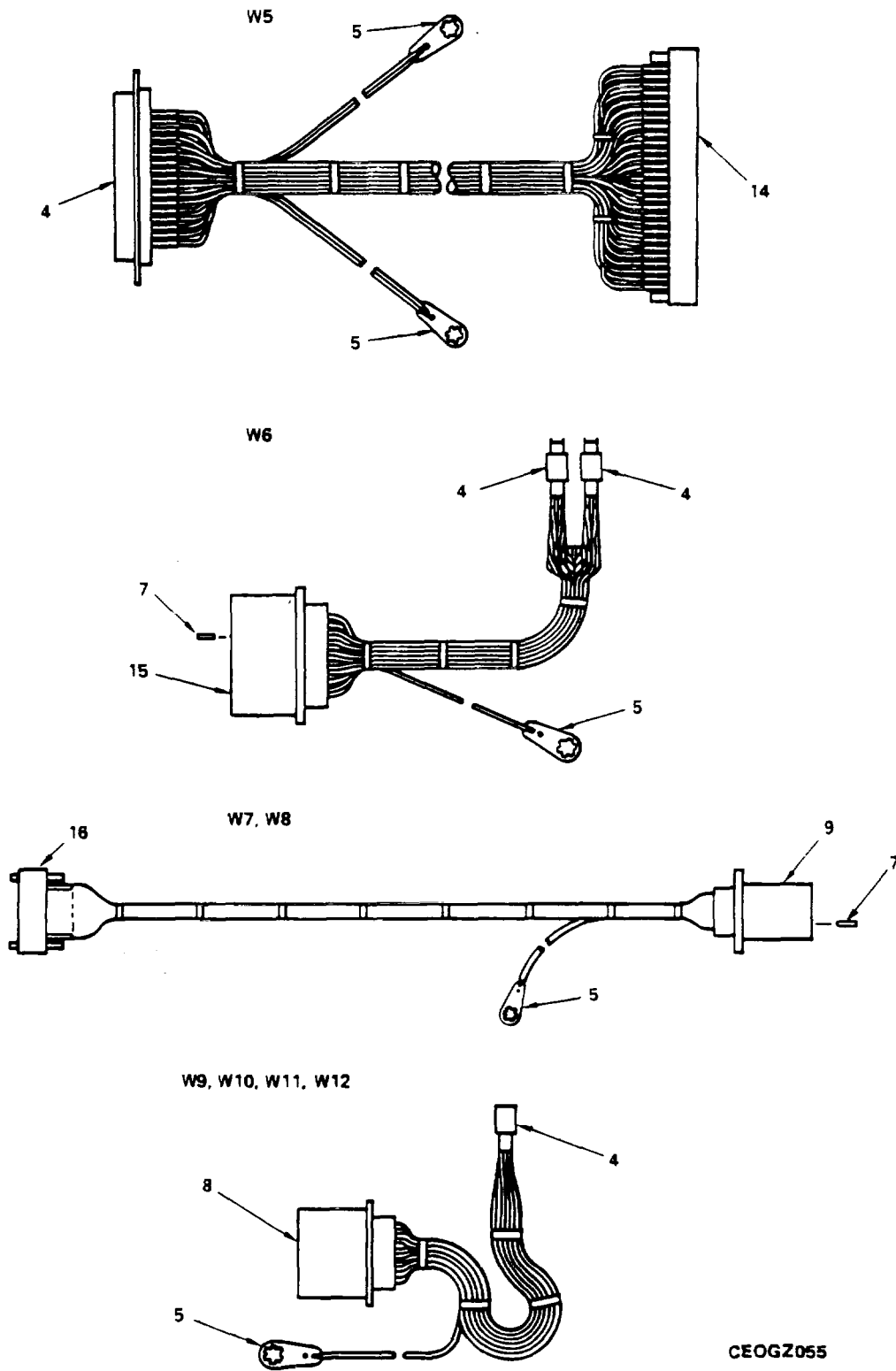
Figure 23. Cable Assemblies W1-W15 (Sheet 2 of 3)
