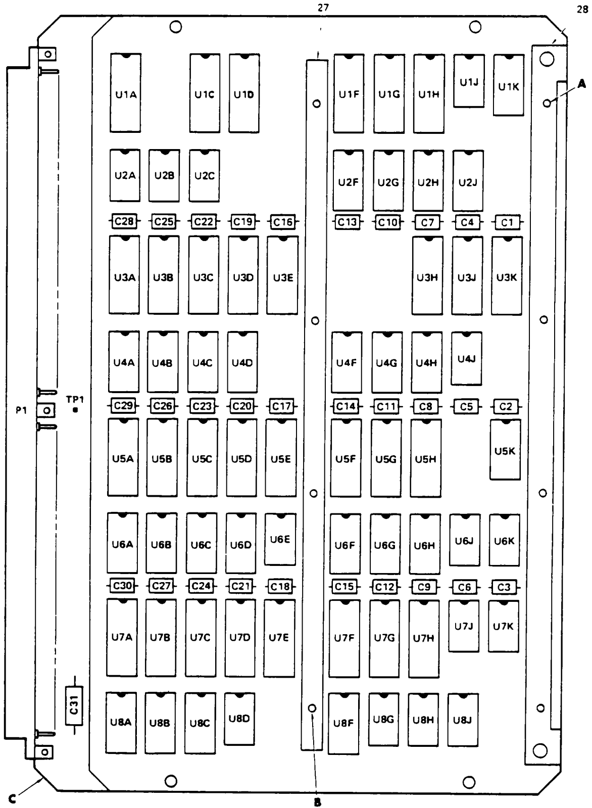
Figure 5. Circuit Card Assembly, TOIB (A4) (Sheet 1 of 2)
