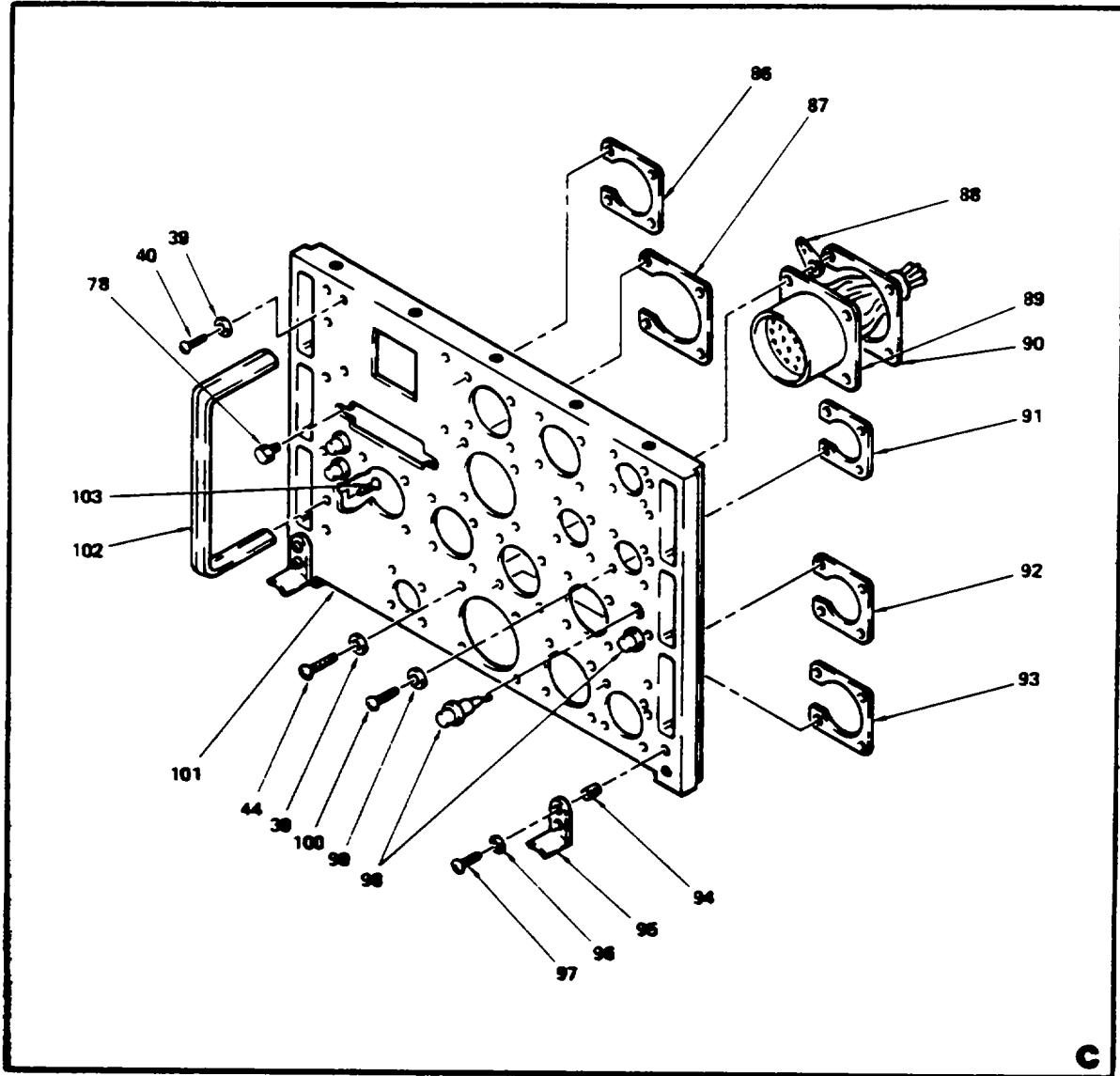
Figure 1. Interface Unit J-4522/U (Sheet 4 of 4)
