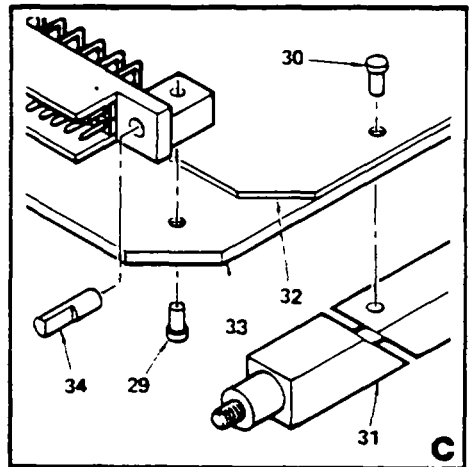
Figure 3. Circuit Card Assembly, IU BUS 2 (A14) (Sheet 2 of 2)
