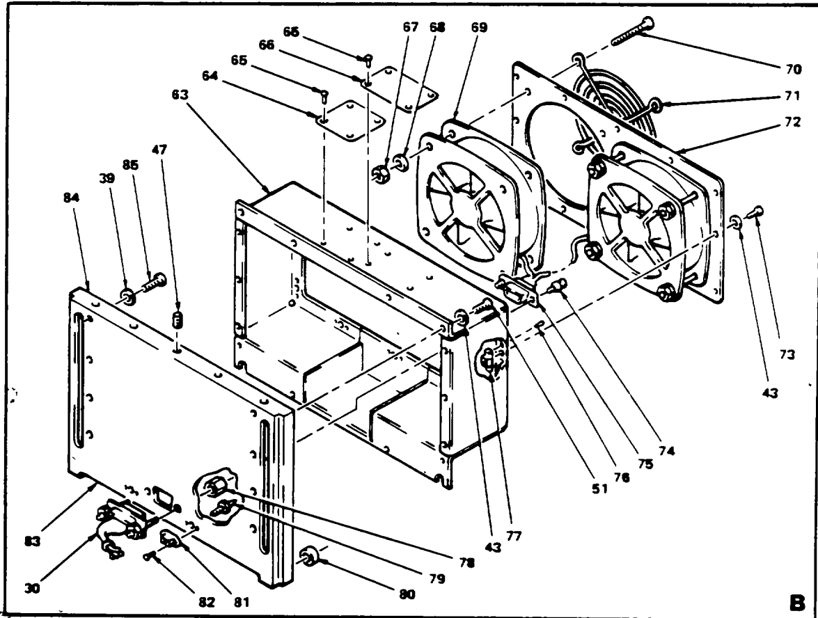
Figure 1. Interface Unit J-4522/U (Sheet 3 of 4)
