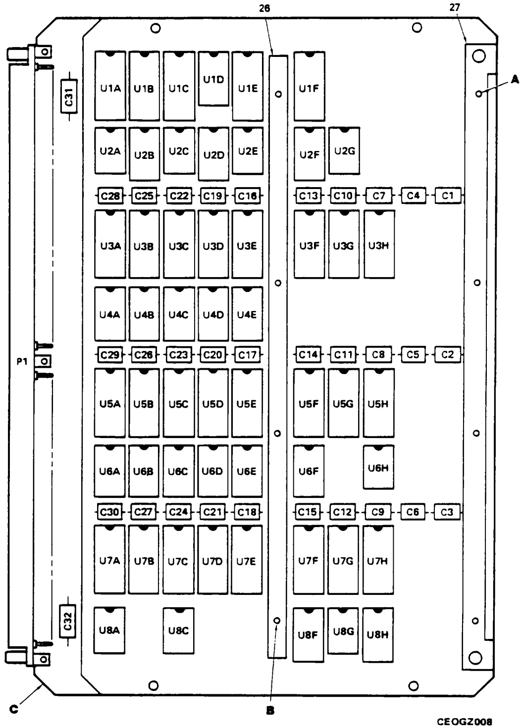
Figure 3. Circuit Card Assembly, IU BUS 2 (A14) (Sheet 1 of 2)
