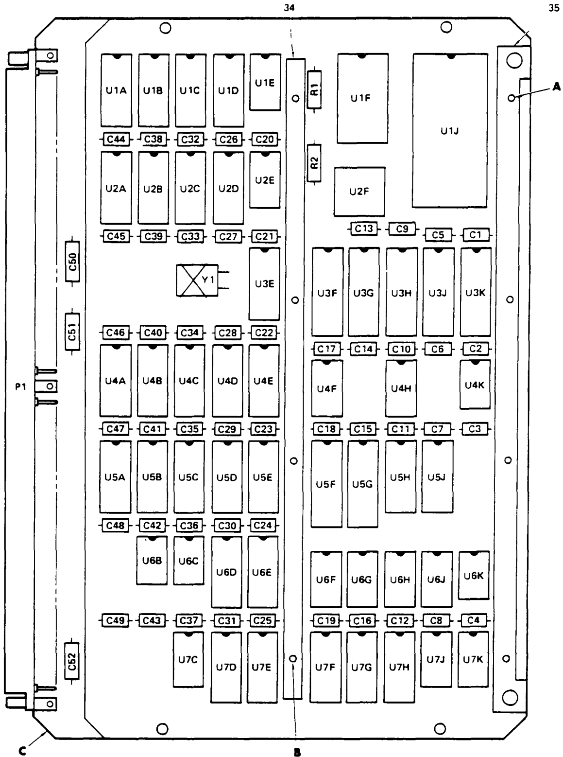
Figure 6. Circuit Card Assembly, 1553 IF JA15, A27) (Sheet 1 of 2)
