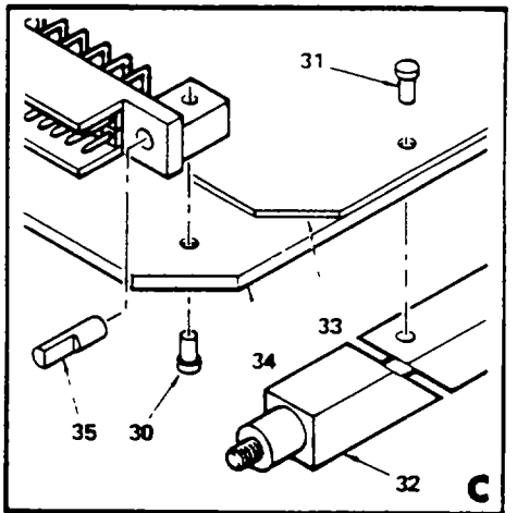
Figure 5. Circuit Card Assembly, TIB (A4) (Sheet 2 of 2)
