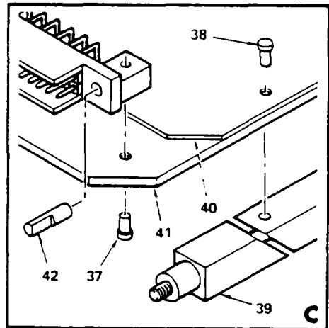
Figure 6. Circuit Assembly, 1553 if (A15,A27) (Sheet 2 of 2)
