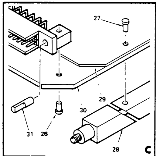
Figure 8. Circuit Card Assembly, IU NAV (A16) (Sheet 2 of 2)
