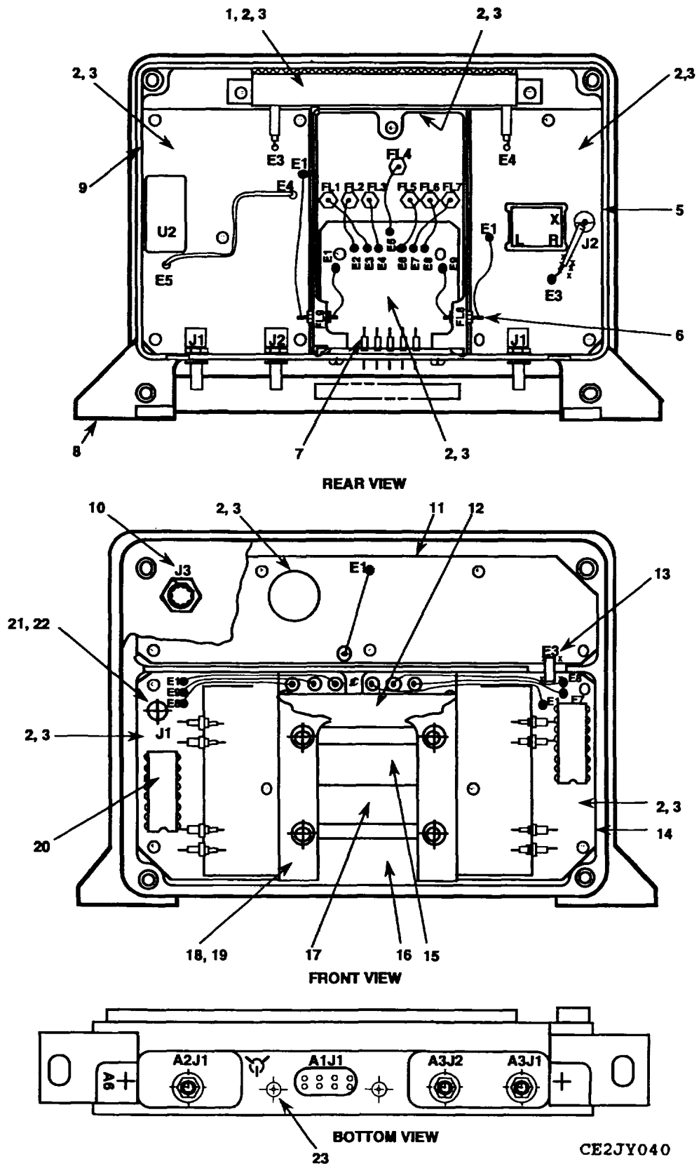
Figure 40. Electronic Component Assembly.
