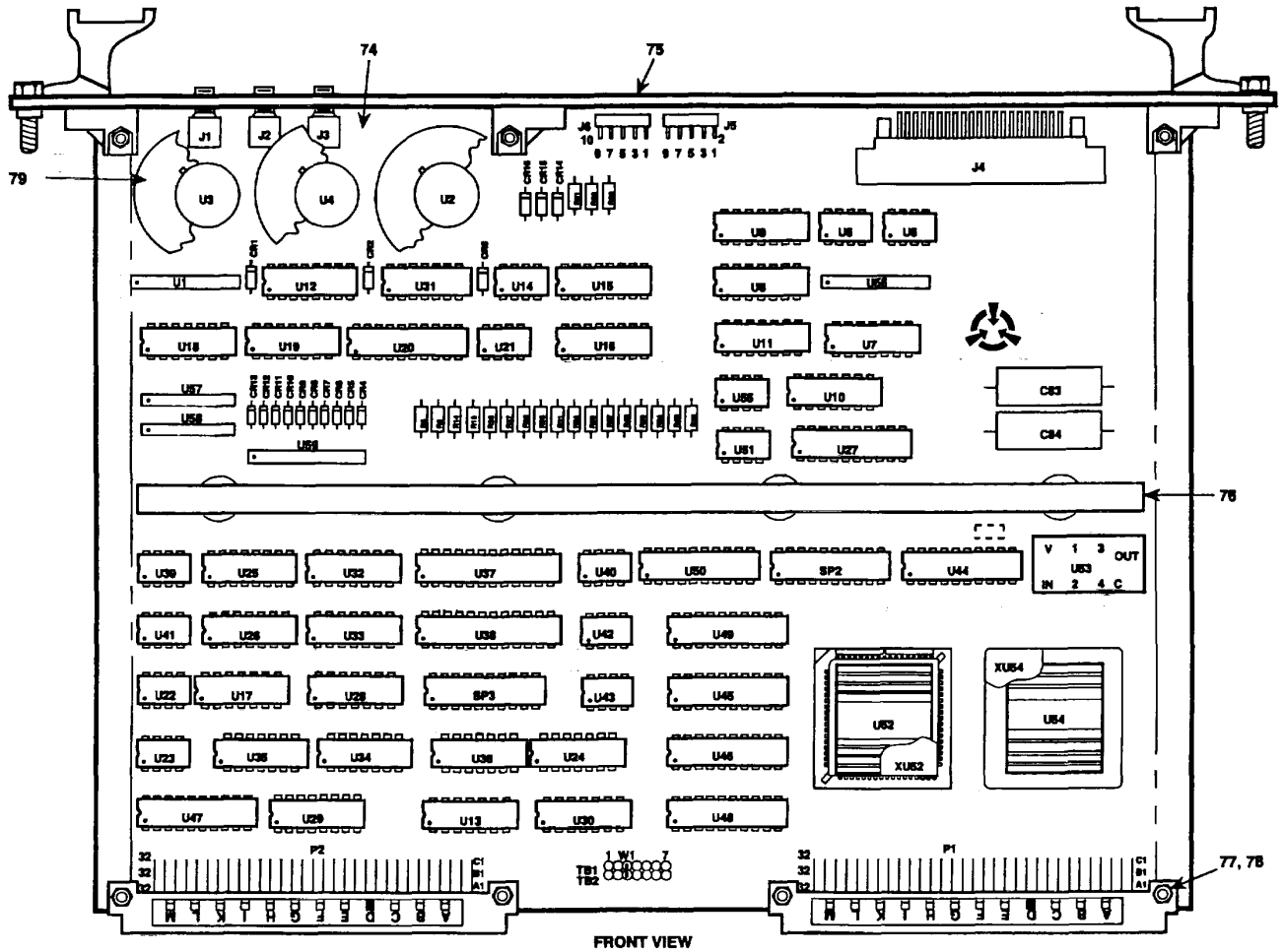
FRONT VIEW
