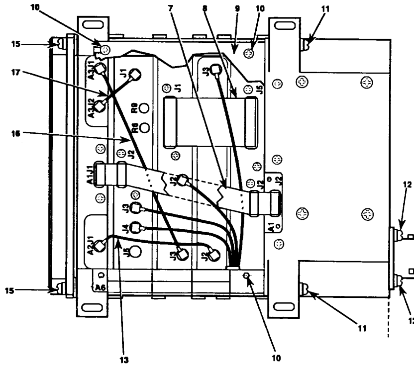
Figure 28. Radio Receiver.
