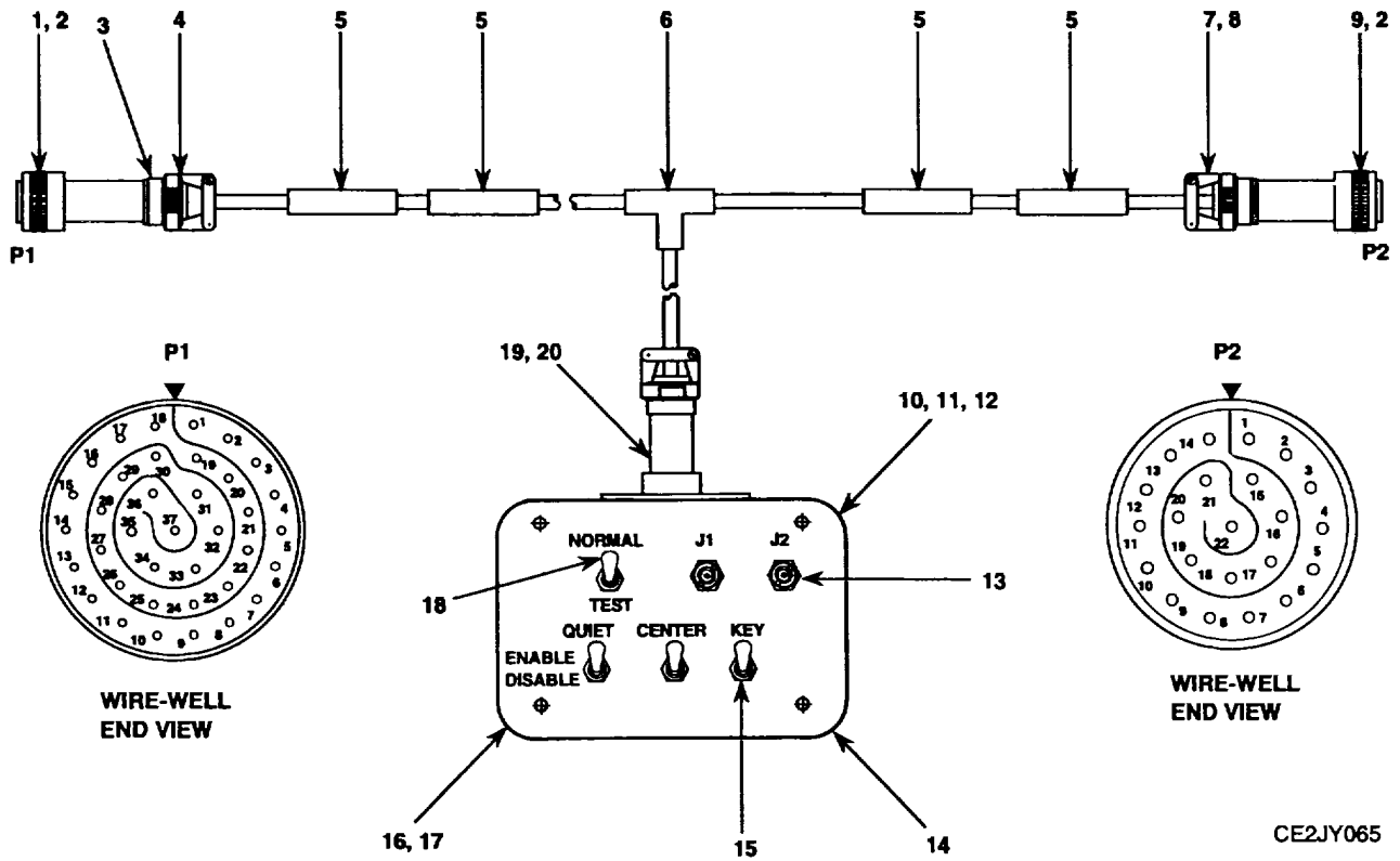
Figure 65. Cable Assembly, SP, Electrical.
