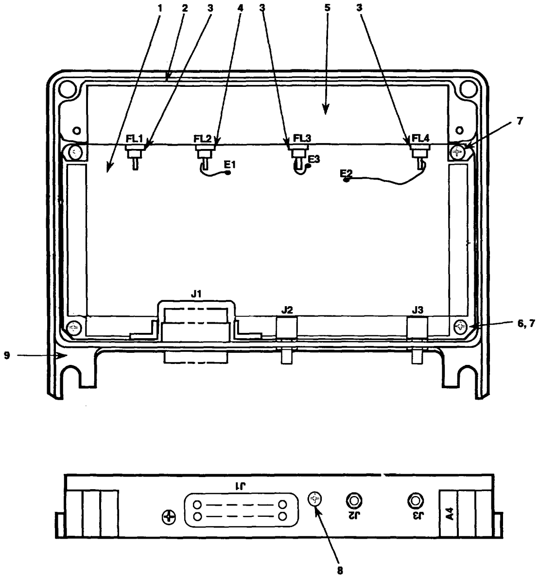
Figure 35. Electronic Component Assembly.
