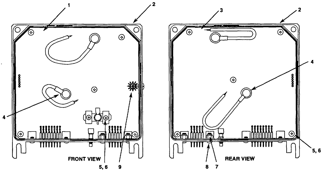
Figure 21. Electronic Component Assembly.
