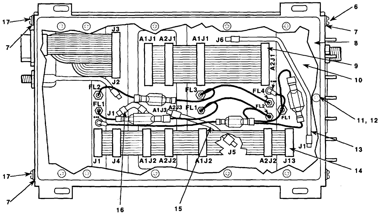
Figure 10. Radio Transmitter.
