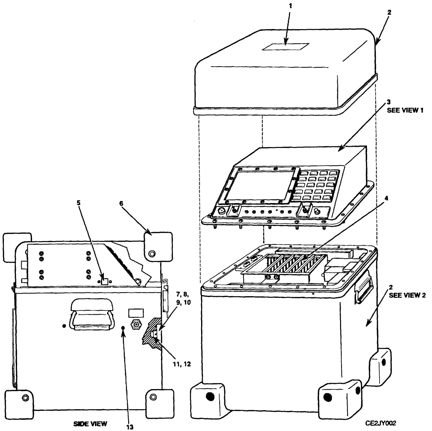
Figure 2. Test Controller (sheet 1 of 3).
