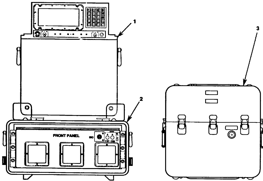
RADIO RELAY TEST SET (FRONT VIEW)
