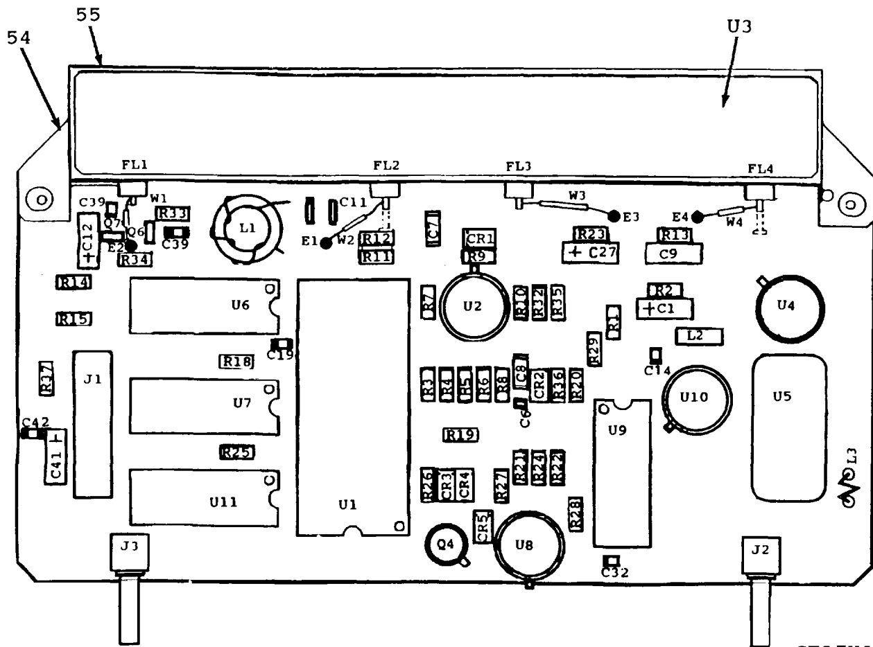
FRONT VIEW
