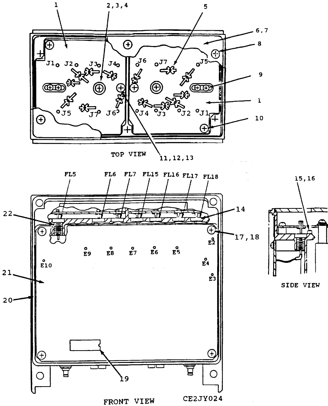
Figure 24. Electronic Component Assembly (sheet 1 of 2).
