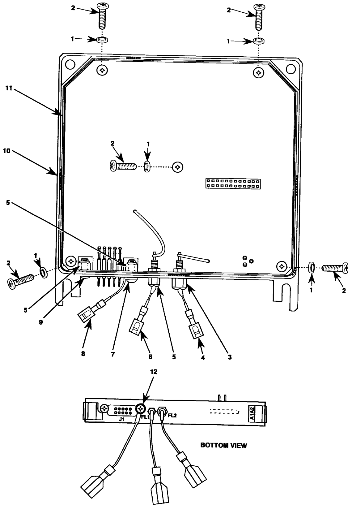
Figure 15. Electronic Component Assembly.
