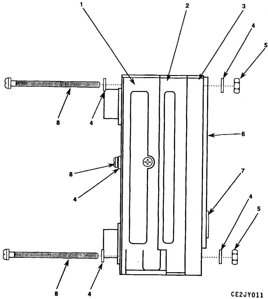
Figure 11. Electronic Component Assembly.
