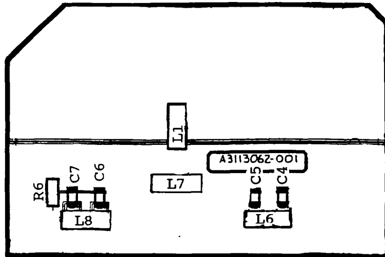
REAR VIEW
