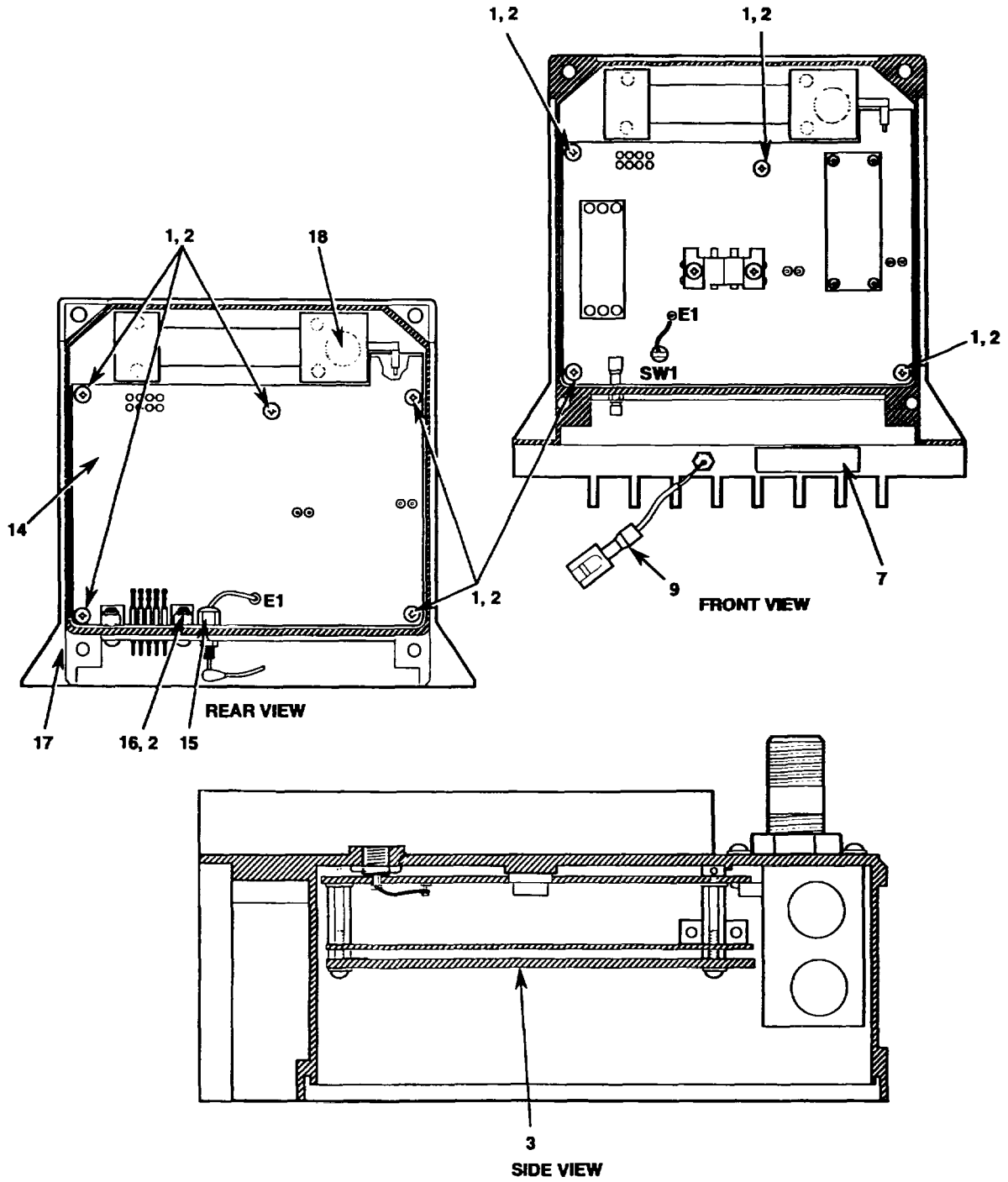
Figure 27. Electronic Component Assembly.
