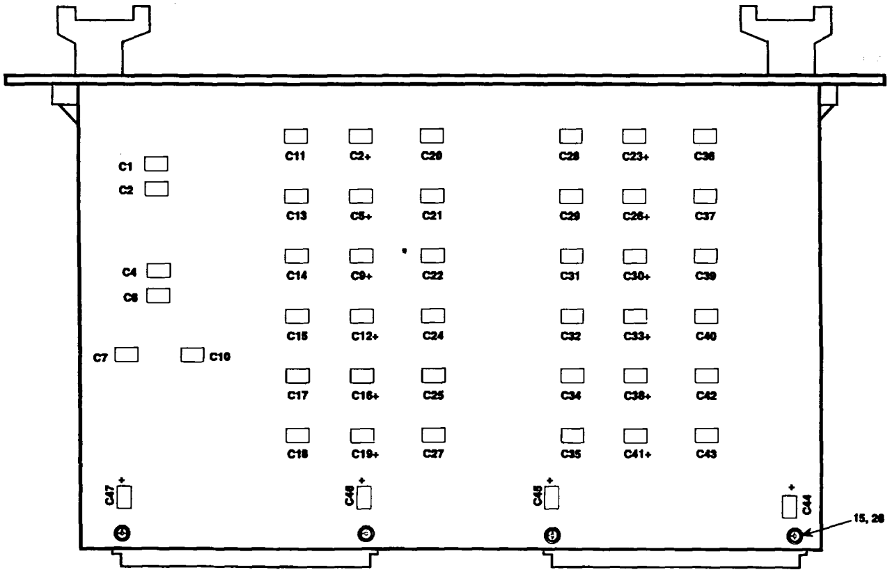
REAR VIEW
