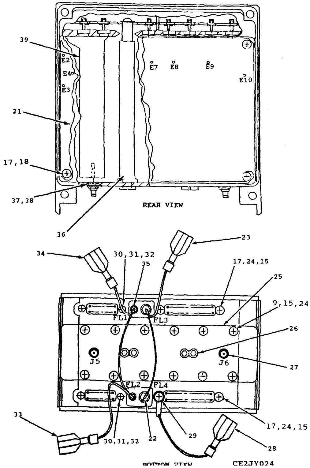
Figure 24. Electronic Component Assembly (sheet 2 of 2).
