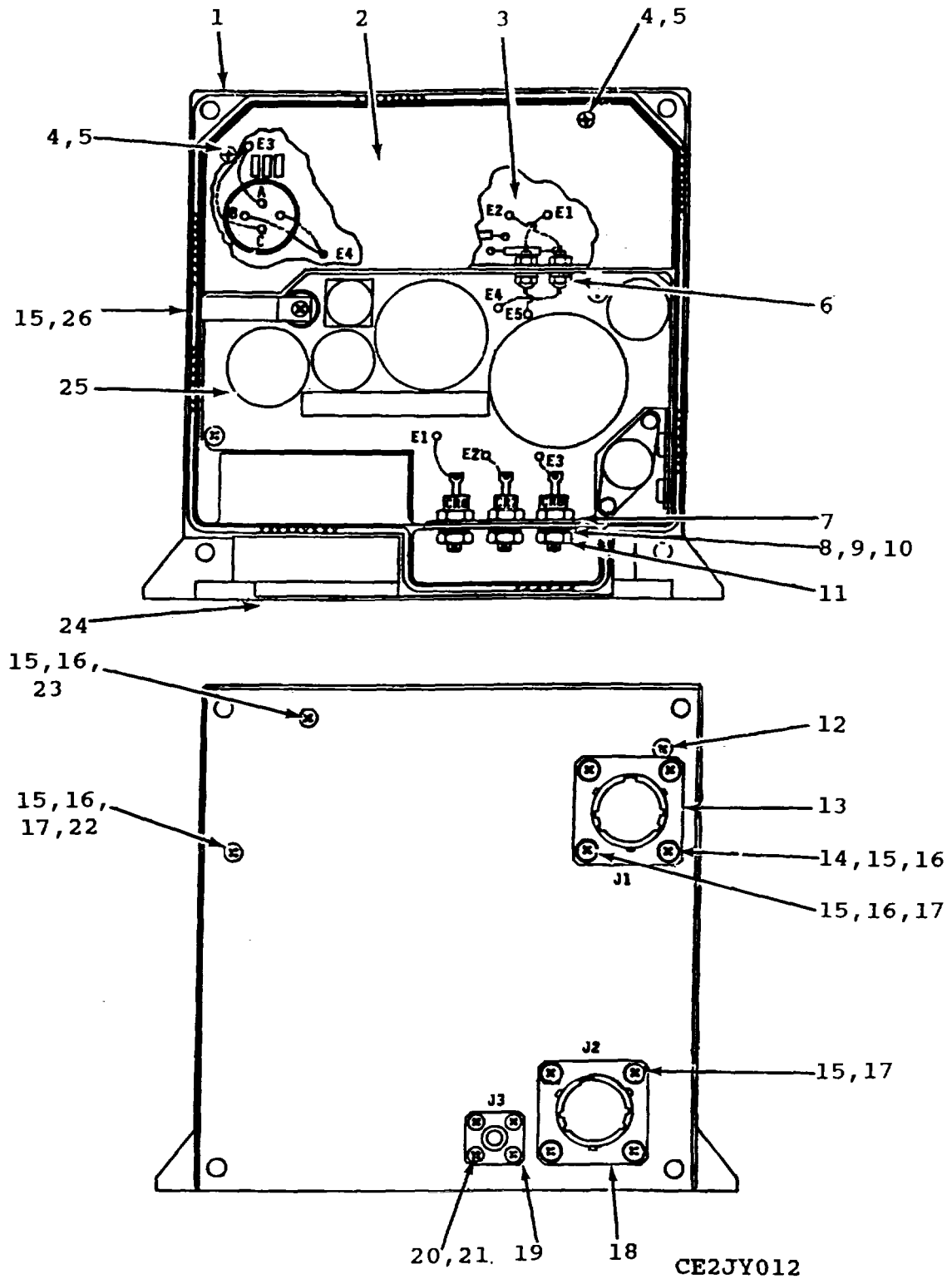
Figure 12. Filter Assembly, Electrical
