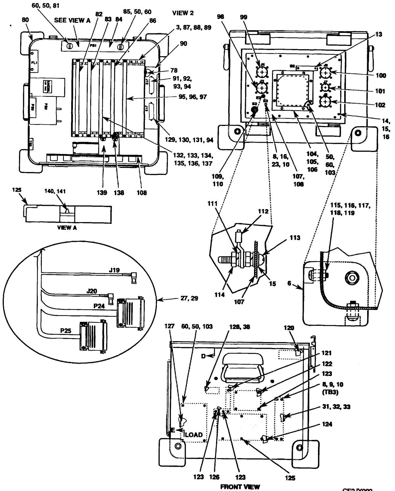
Figure 2. Test Controller (sheet 3 of 3).
