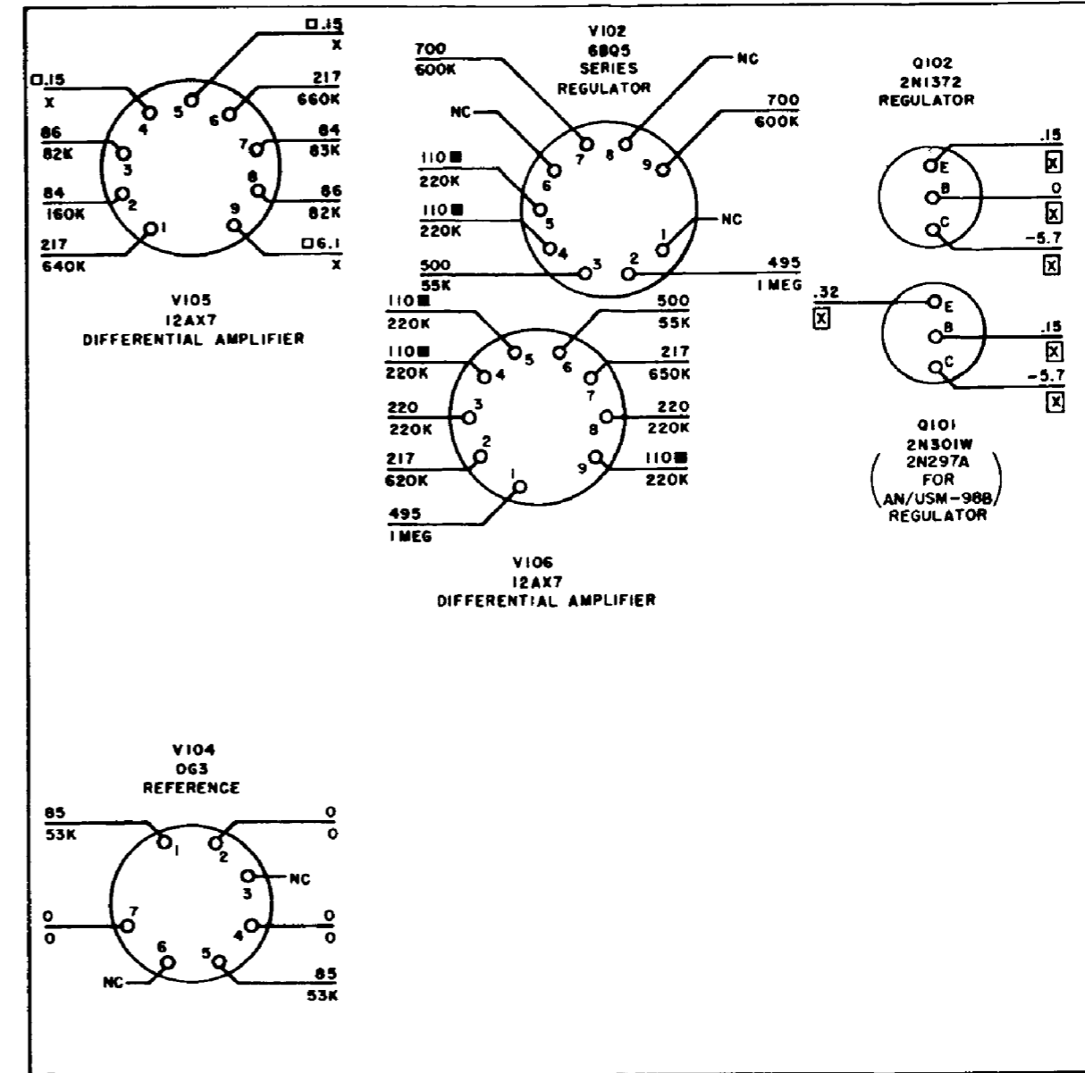
B. 500-VOLT REFERENCE POWER SUPPLY PRINTED CIRCUIT BOARD
