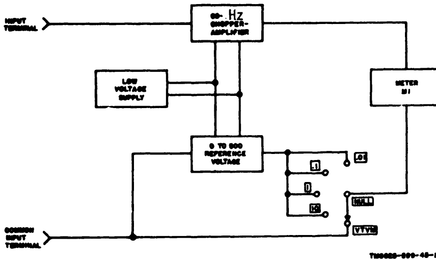
Figure 1-1. Voltmeter, Electronic AN/USM-98(*), block diagram.
