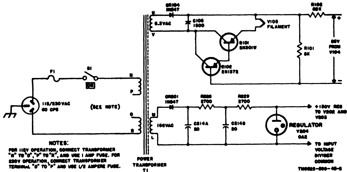
Figure 1-5. Low-voltage power supply, schematic diagram AN/USM-98A.
