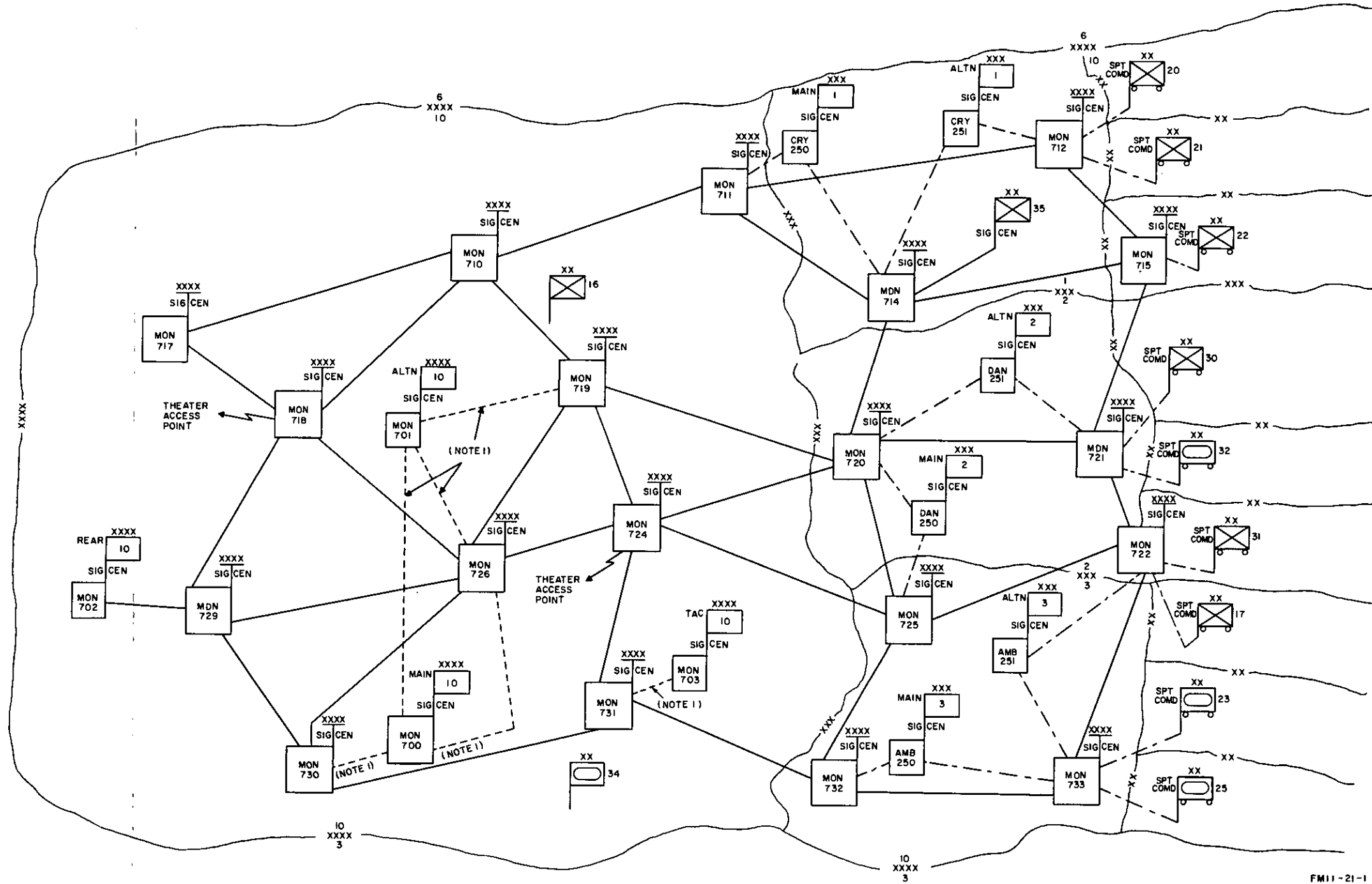
Figure 1. Type field army multichannel communication system.
