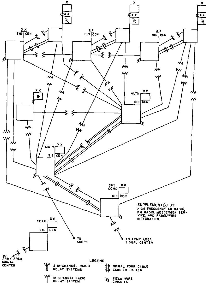
Figure 4. Type division area communication system.
