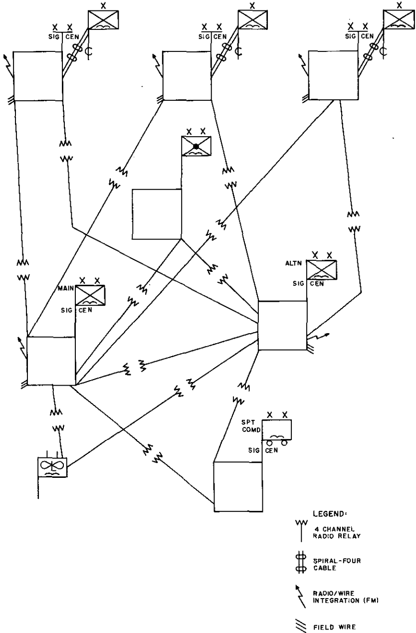
Figure 8. Type Airborne Division Multichannel Communication Network.
