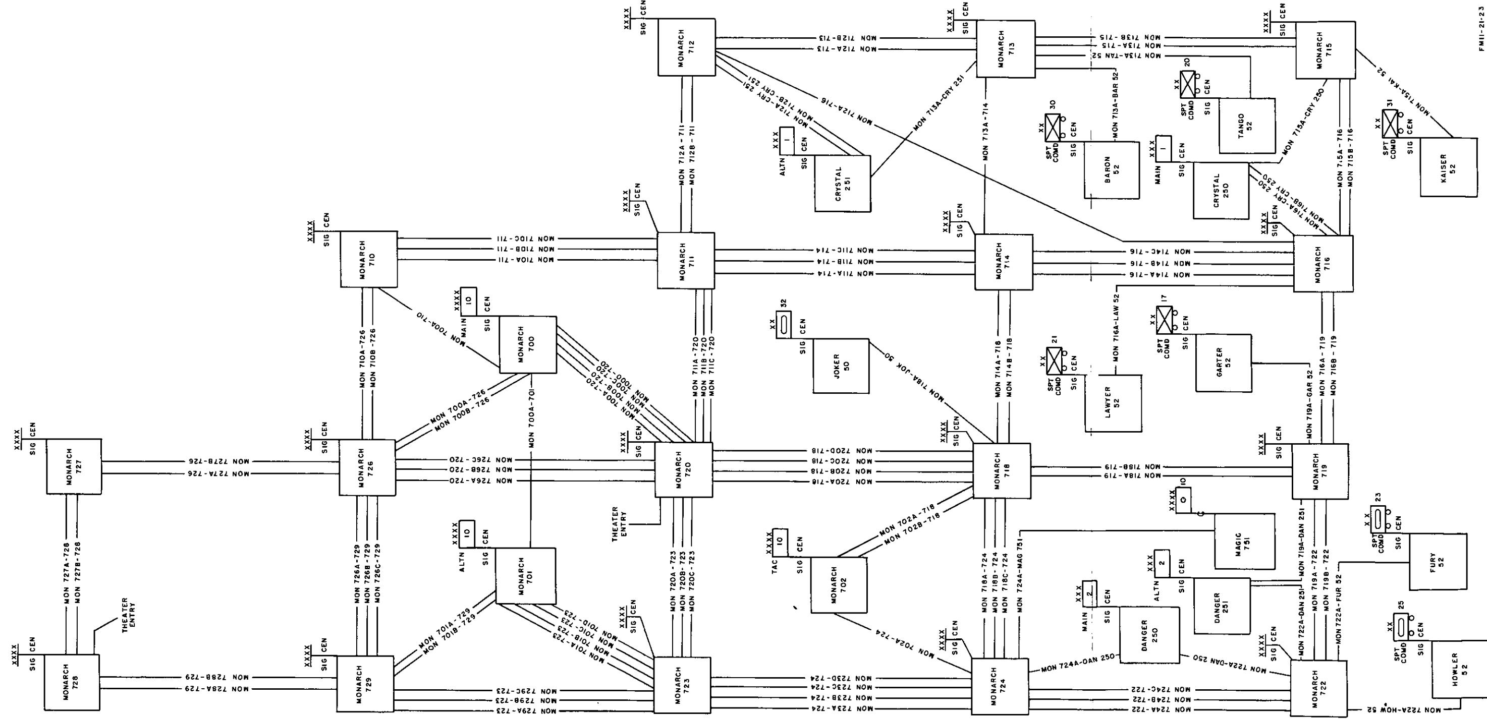
Figure 11. Type army (two-corps) systems diagram.
