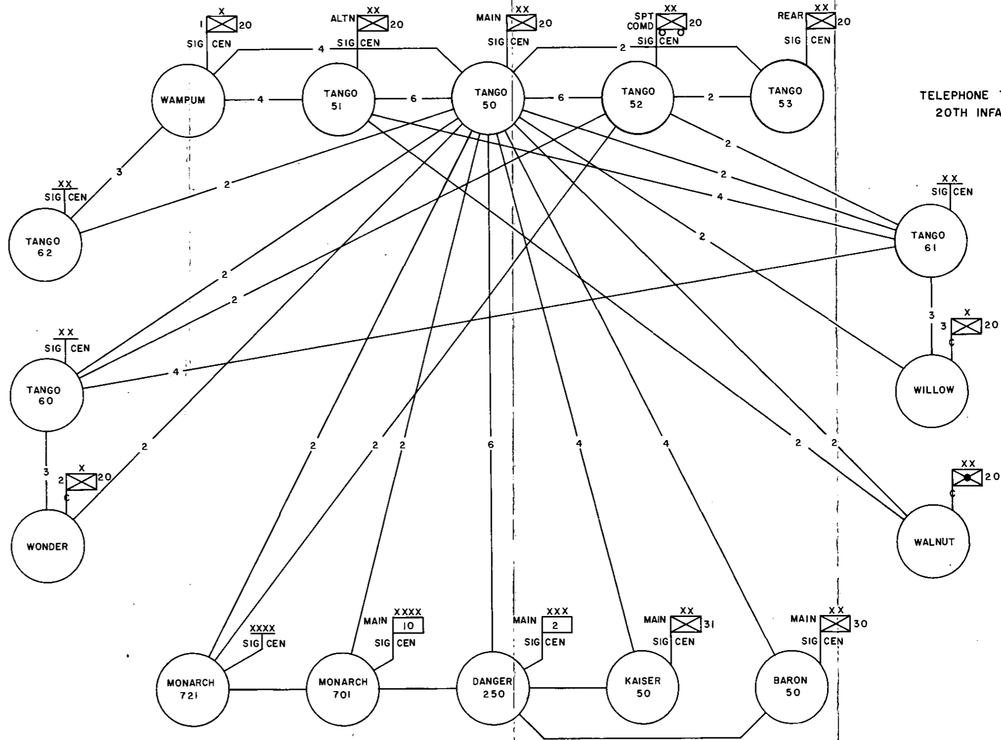
Figure 13. Type infantry division telephone traffic diagram.
