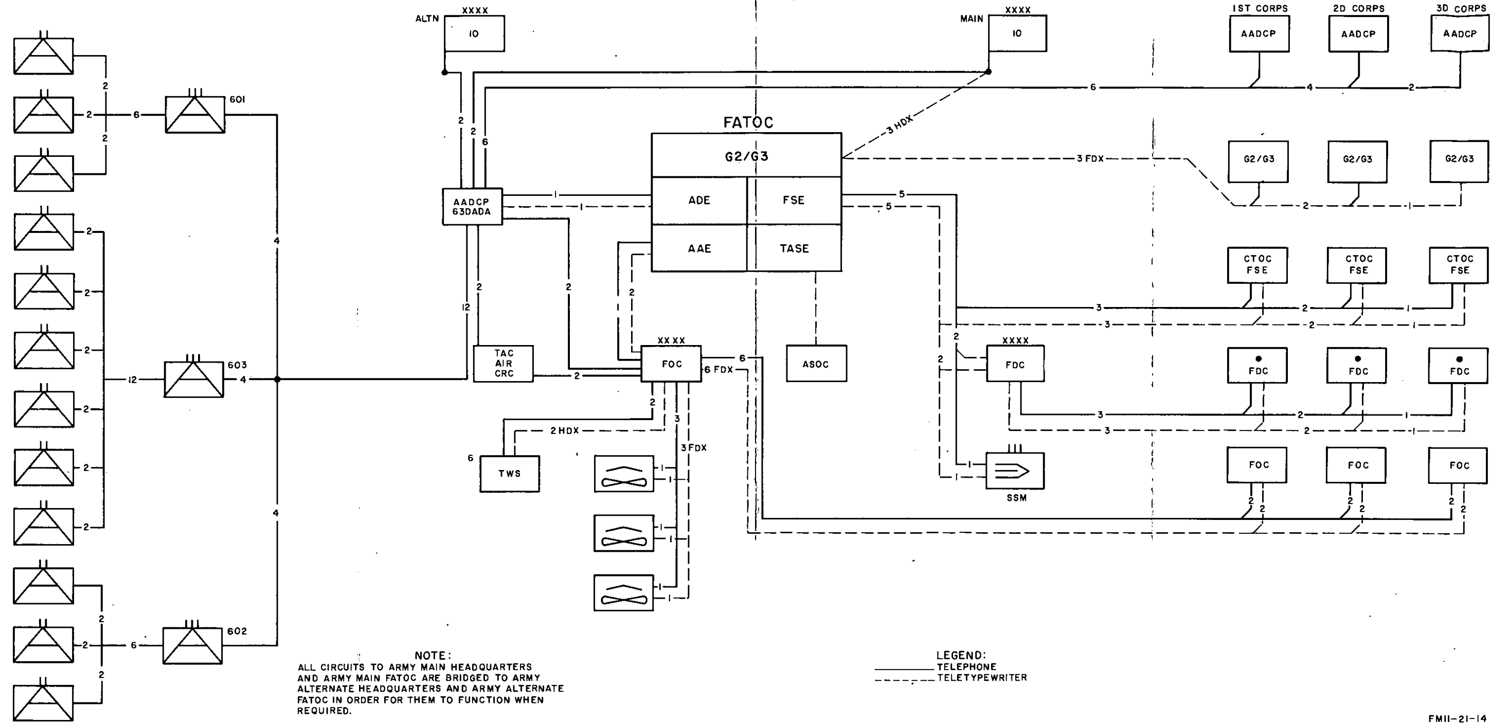
Figure 17. Type army sole-user telephone and teletypewriter traffic diagram.
