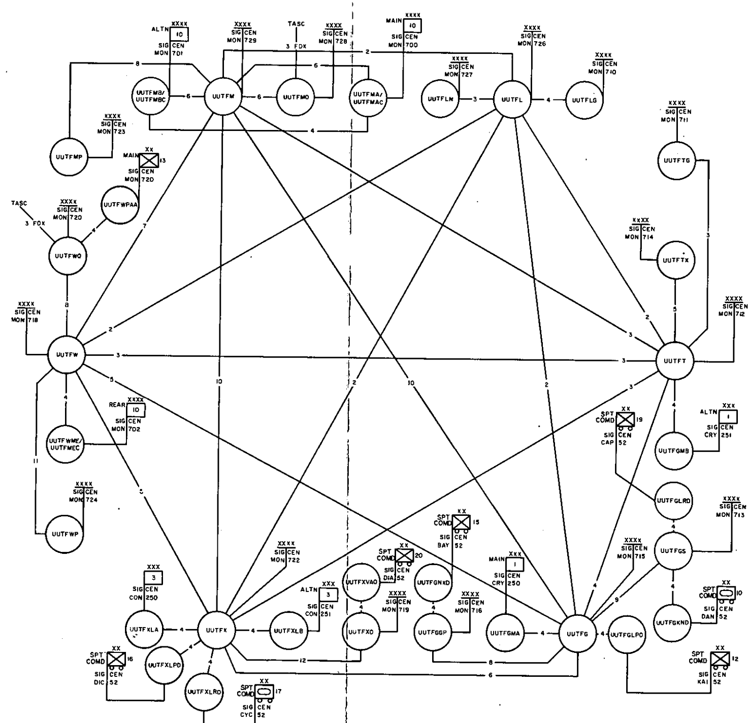
Figure 16. Type field army teletypewriter traffic diagram.
