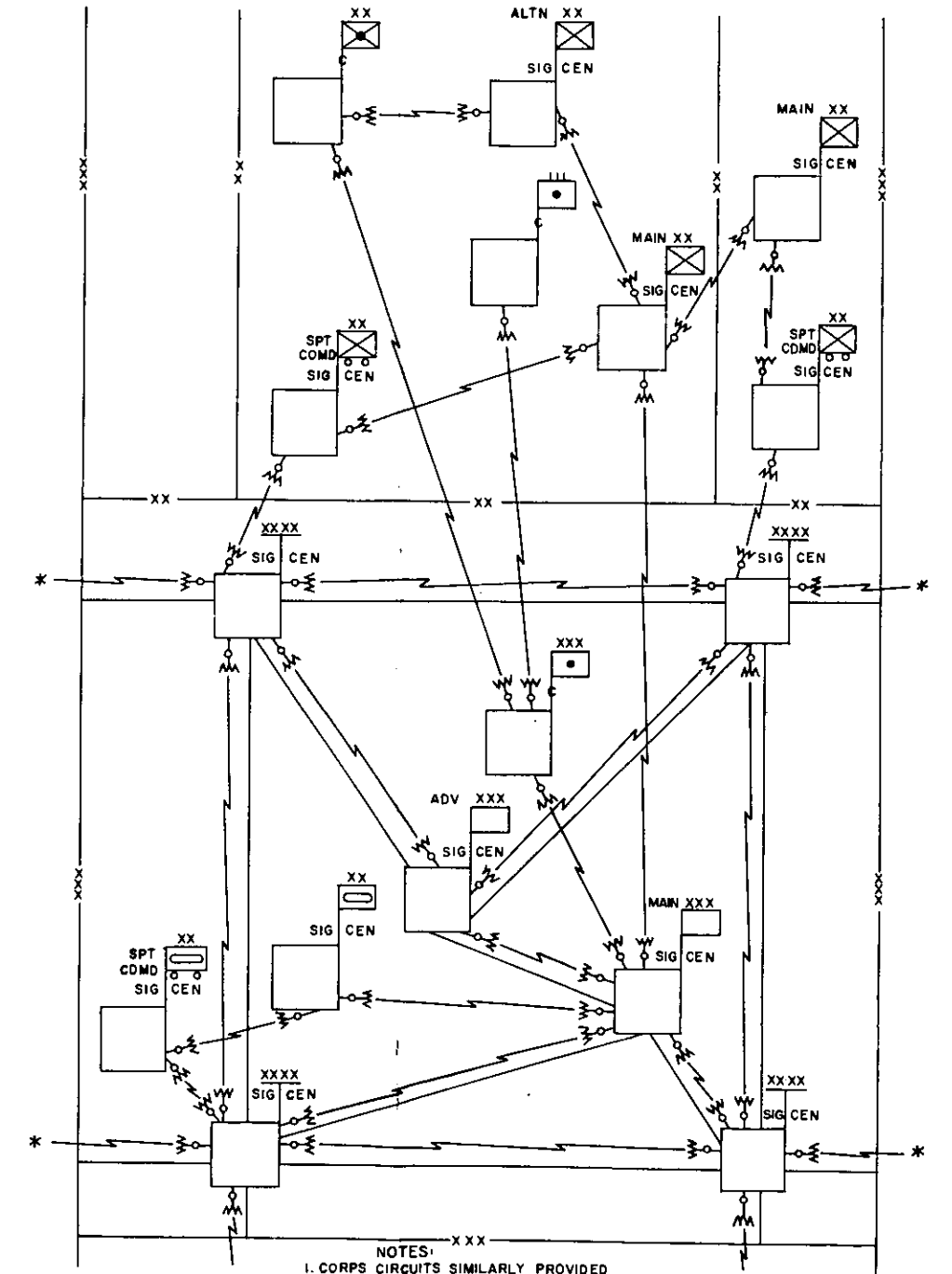
Figure 2. Corps communication system integrated with the field army communication system, schematic diagram.
