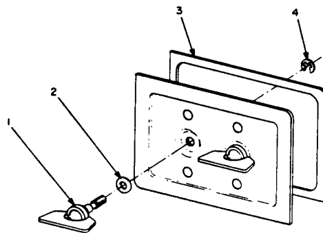
FIGURE 18. DUST COVER ASSEMBLY.
