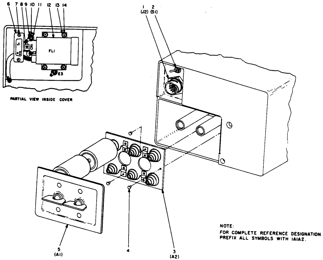
FIGURE 18. DUST COVER ASSEMBLY.
