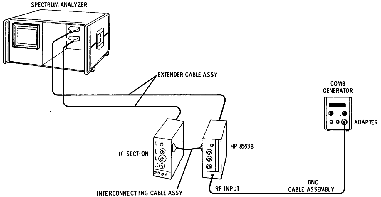
Figure 5-15. APC Tuning Stabilizer Final Check Test Setup
