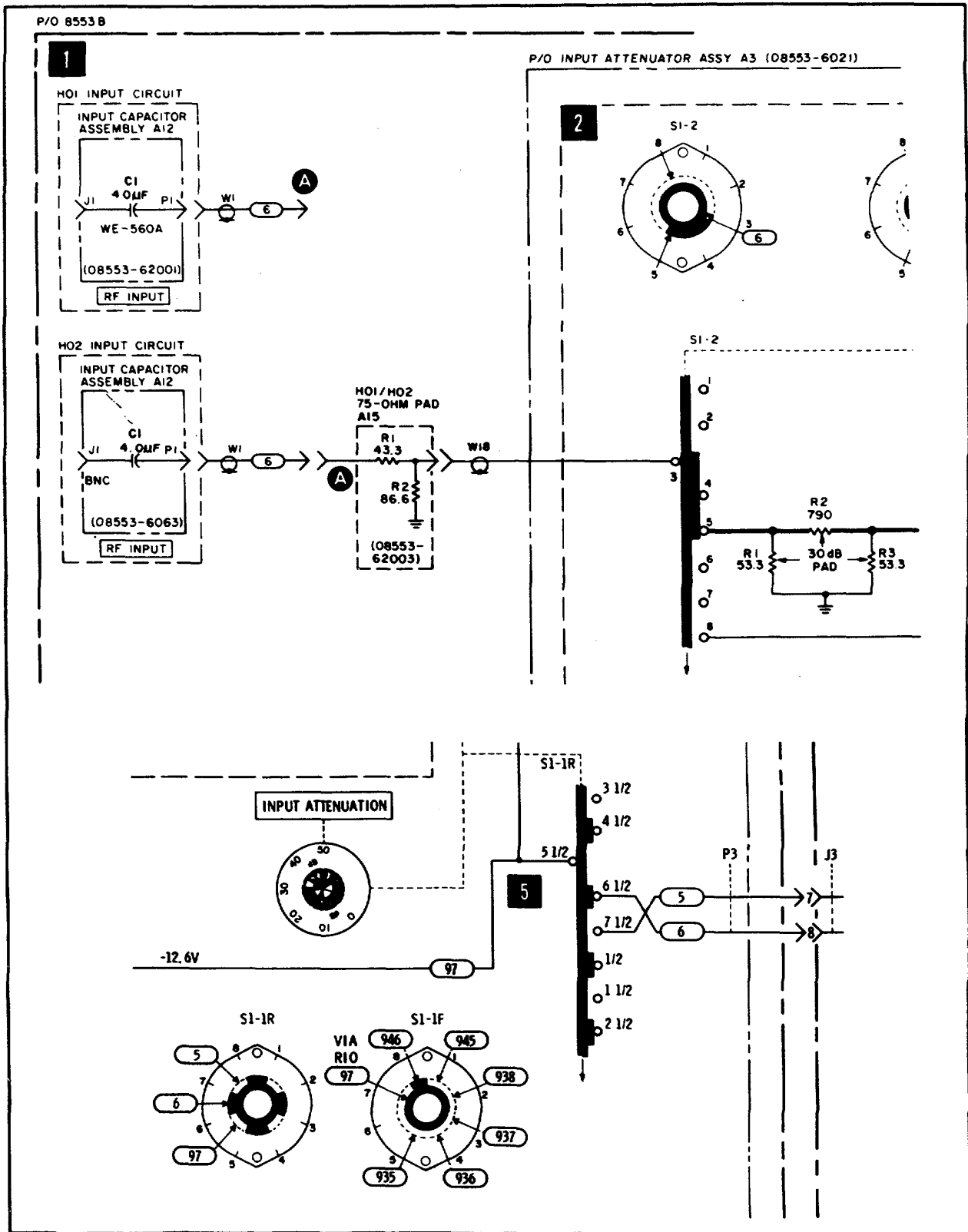
Figure 7-5. HO1/HO2 Schematic Changes for Service Sheet 3, Figure 8-26.
