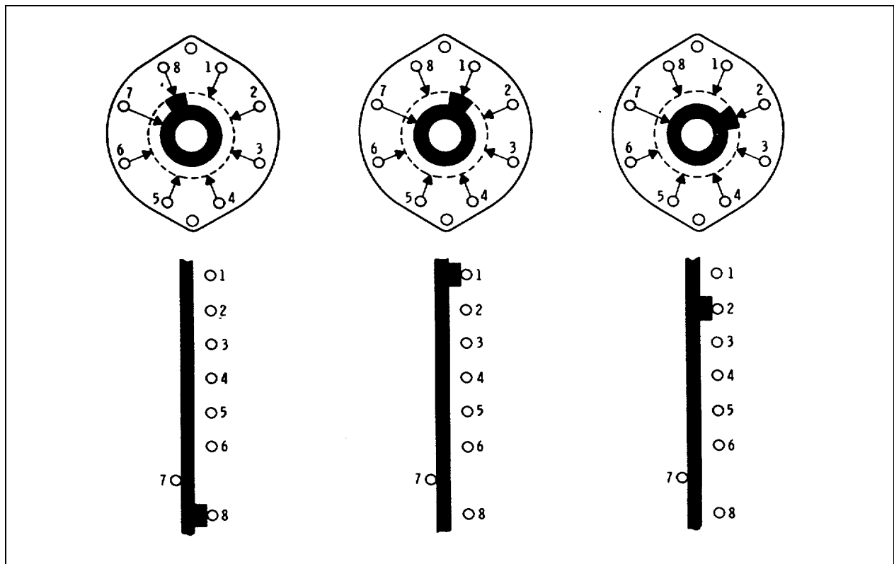
Figure 8-15. Three Positions of Index Light Selector Wafer
