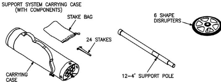
Figure 1-2. ULCANS Components
