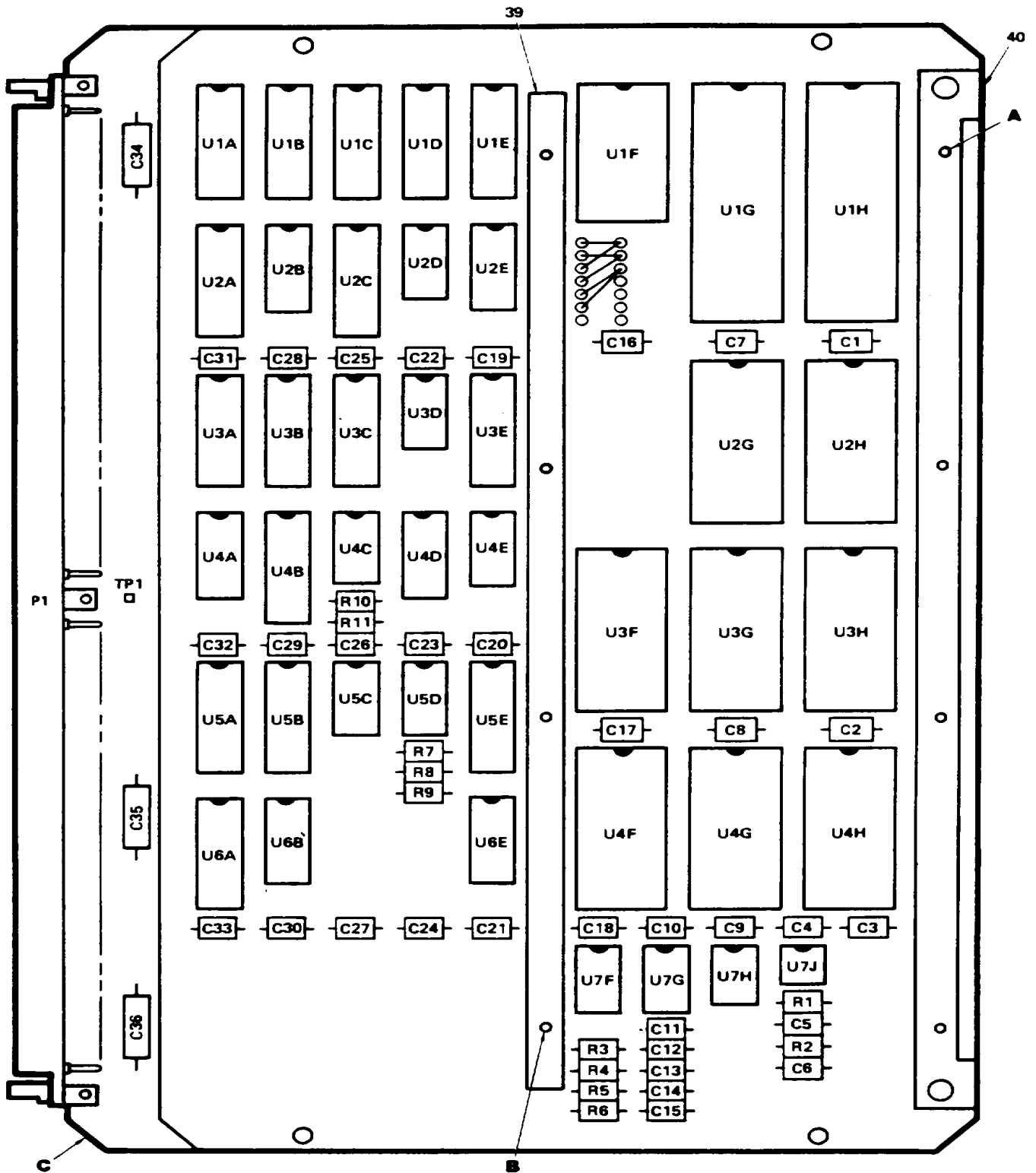
Figure 11. Circuit Card Assembly, TS BUS (A13) (Sheet 1 of 2)
