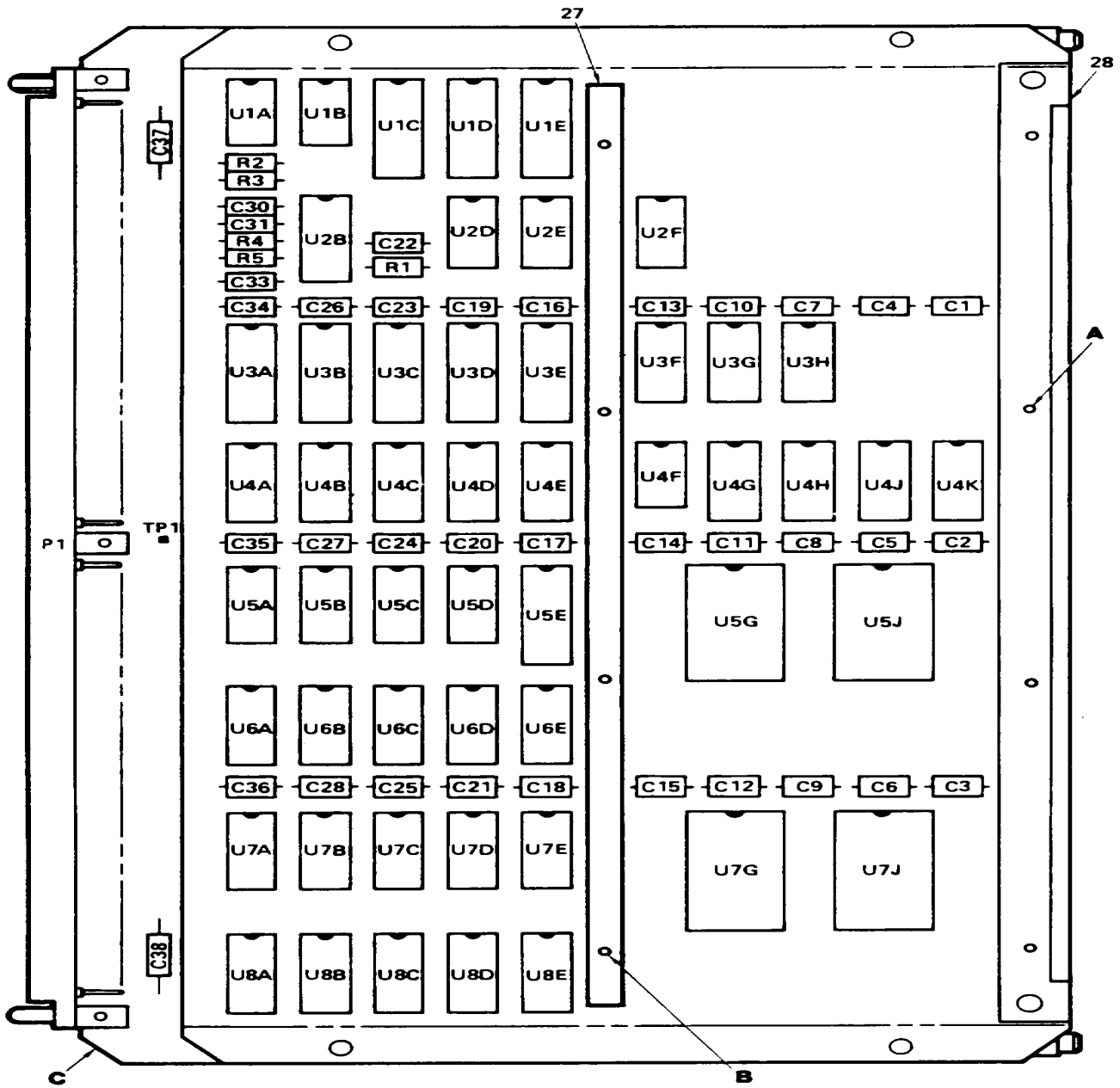
Figure 4. Circuit Card Assembly, C Simulator (A4) (Sheet 1 of 2)
