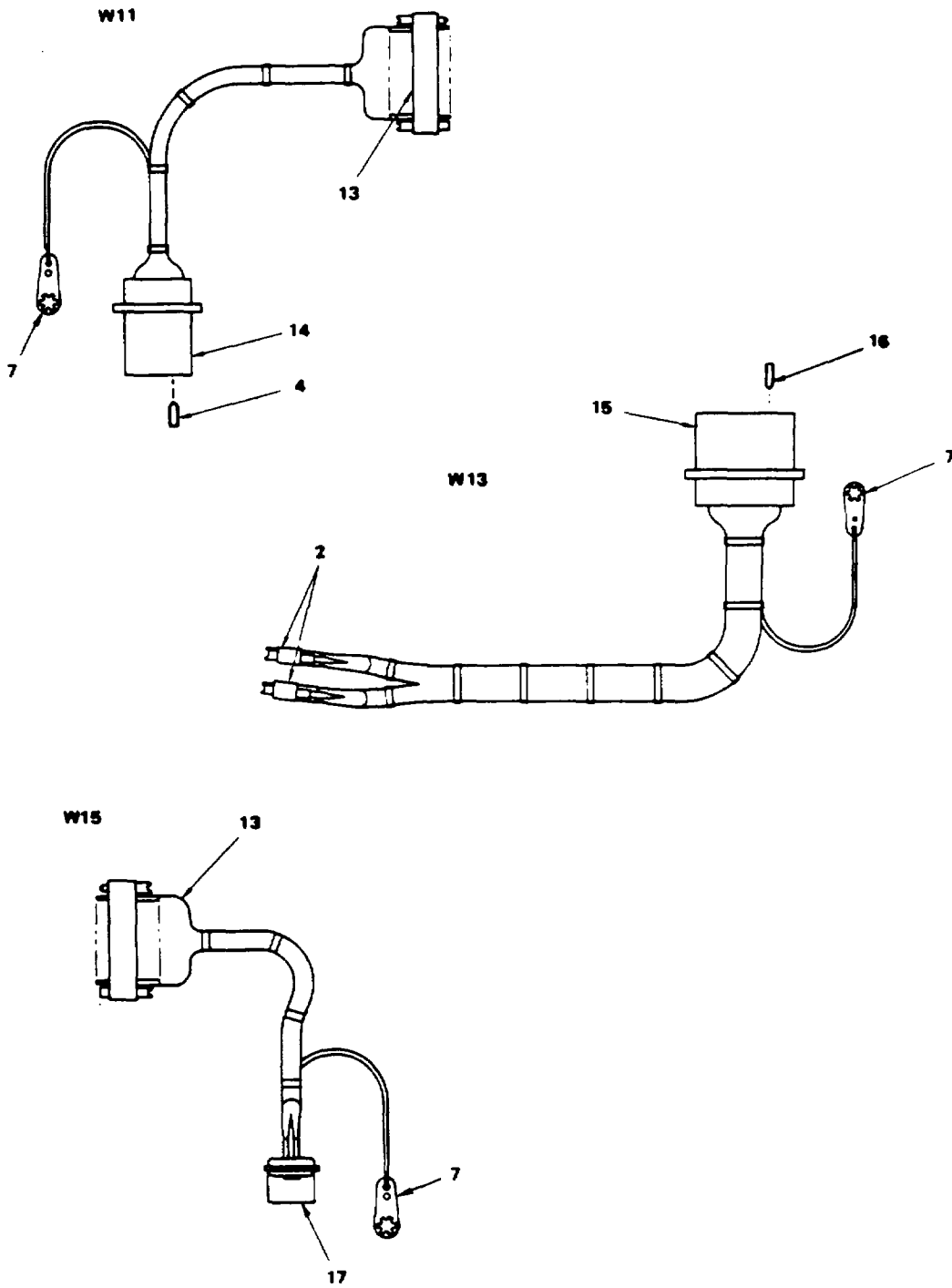
Figure 18. Cable Assemblies (W2-W11, W13-W15) (Sheet 3 of 3)
