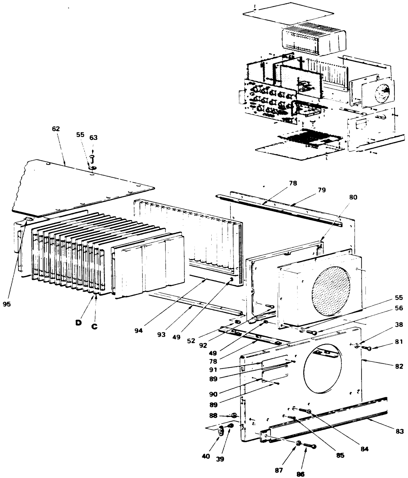
Figure 1. Test Interface Unit TS-4421/U (Sheet 3 of 5)
