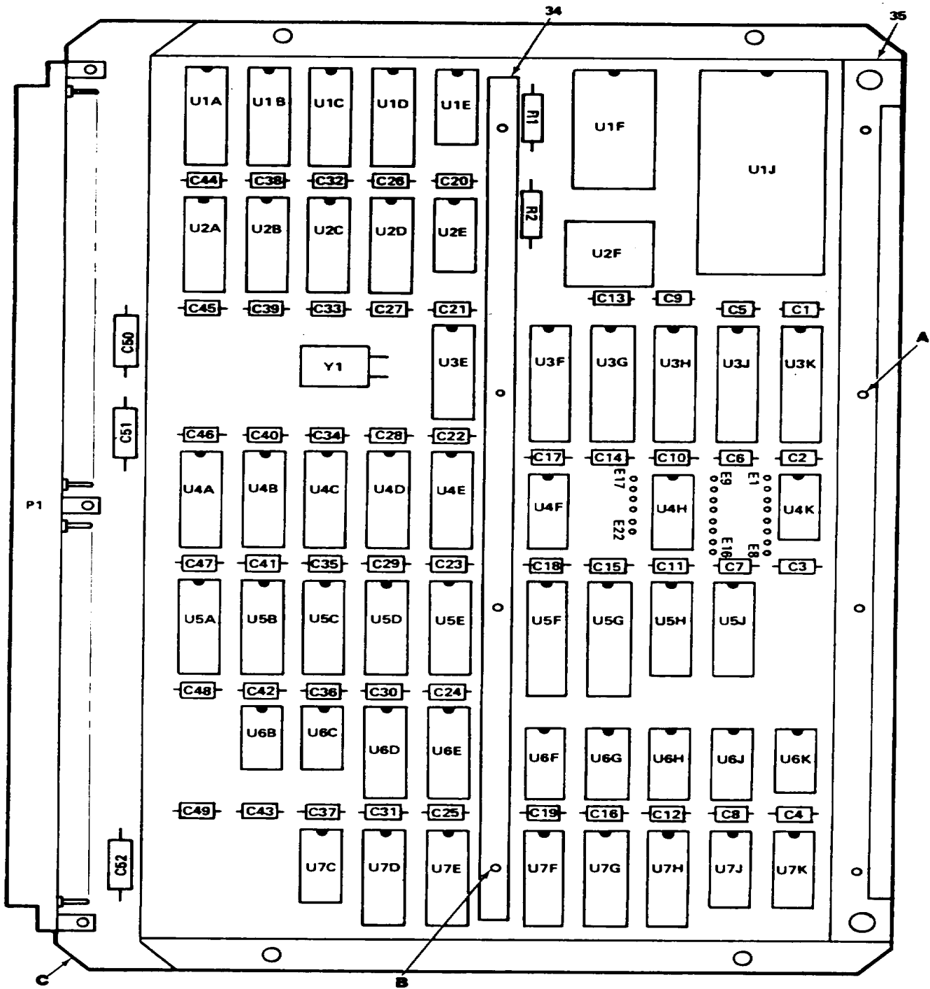
Figure 8. Circuit Card Assembly, 1553 IF (A10) (Sun 1 of 2)
