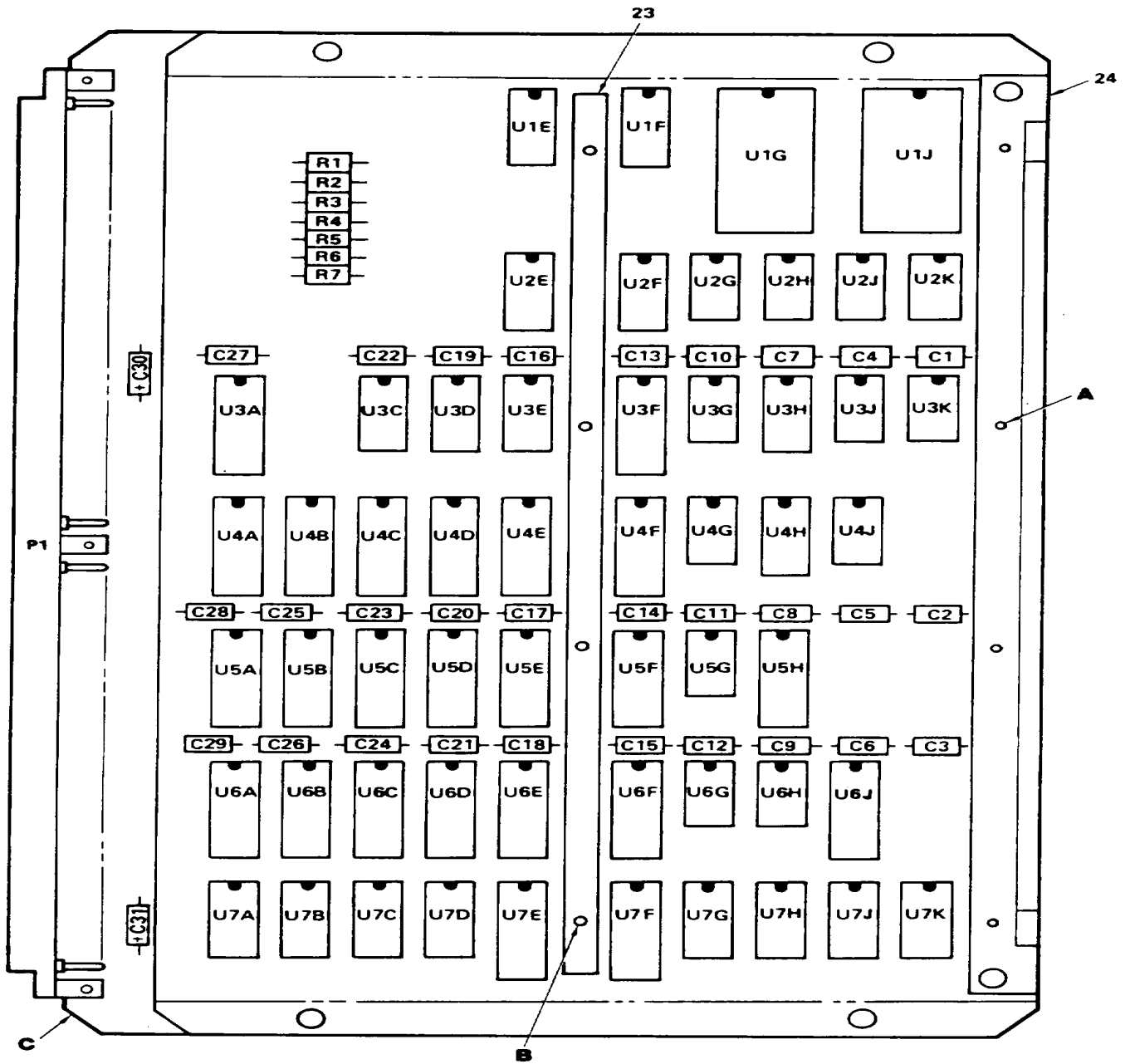
Figure 10. Circuit Card Assembly, IU DL (A12) (Sheet 1 of 2)
