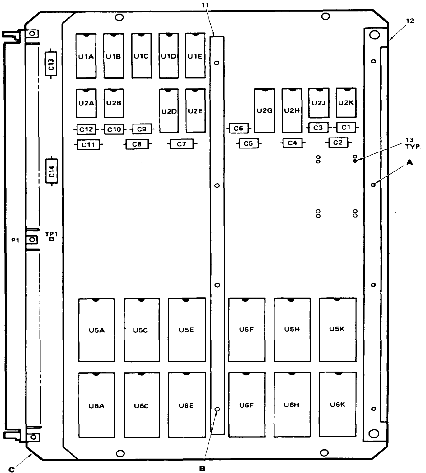
Figure 13. Circuit Card Subassembly, PSRAM (A15) (Sheet 1 of 2)
