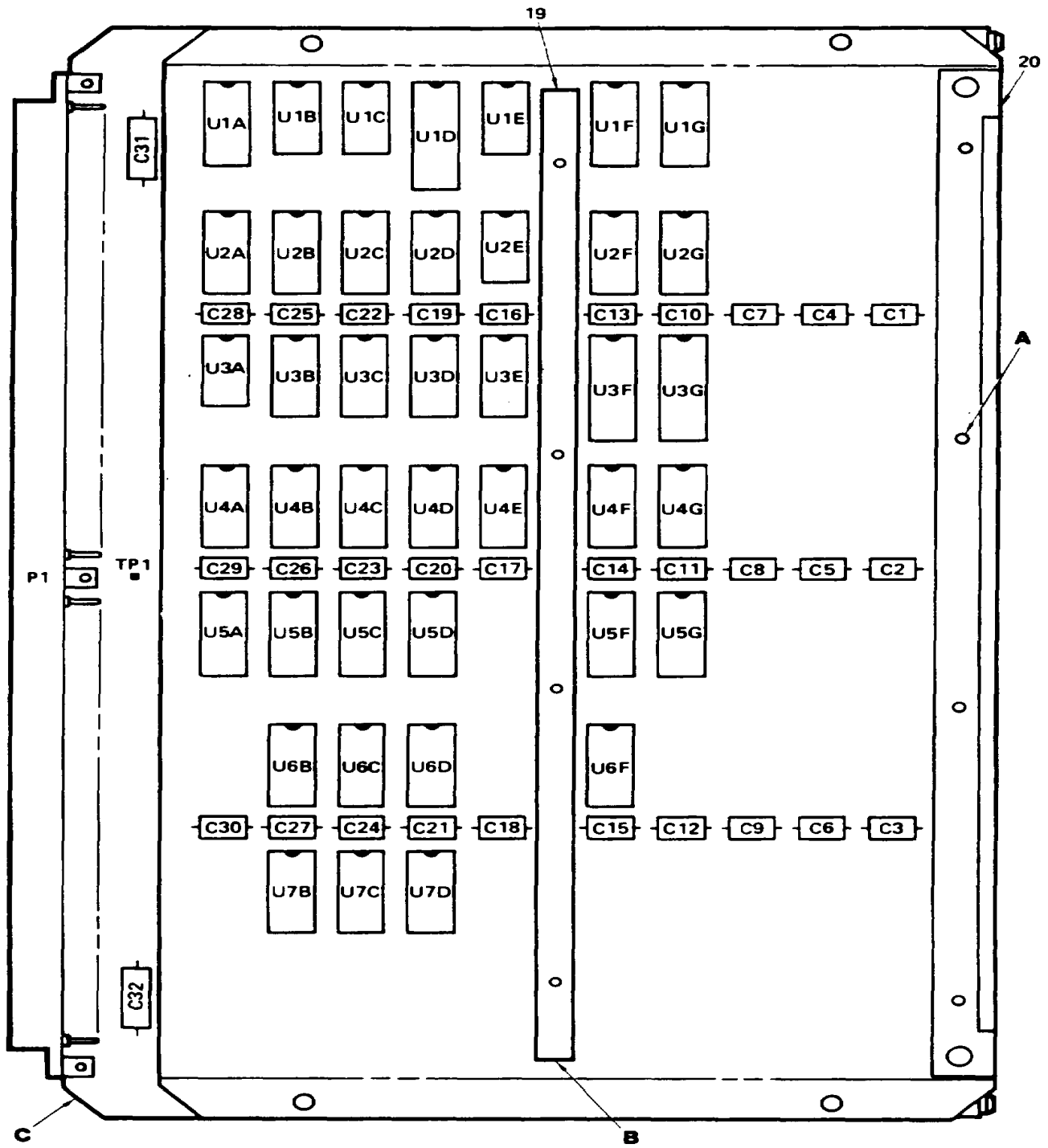
Figure 6. Circuit Card Assembly, TS LO (A8) (Sheet 1 of 2)
