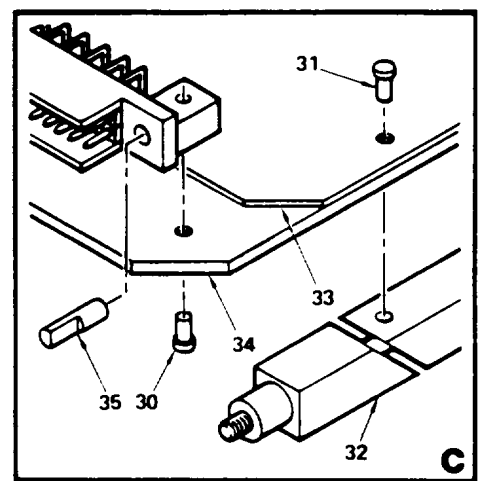
Figure 4. Circuit Cad Assembly, CP Simulator (A4) (Sheet 2 of 2)
