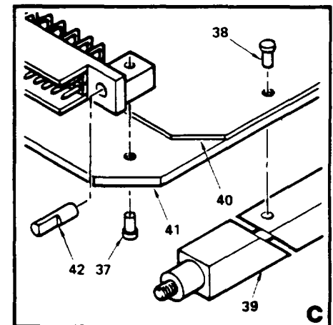
Figure 3. Circuit Card Assembly, CP Interface (A3) (Sheet 2 of 2)
