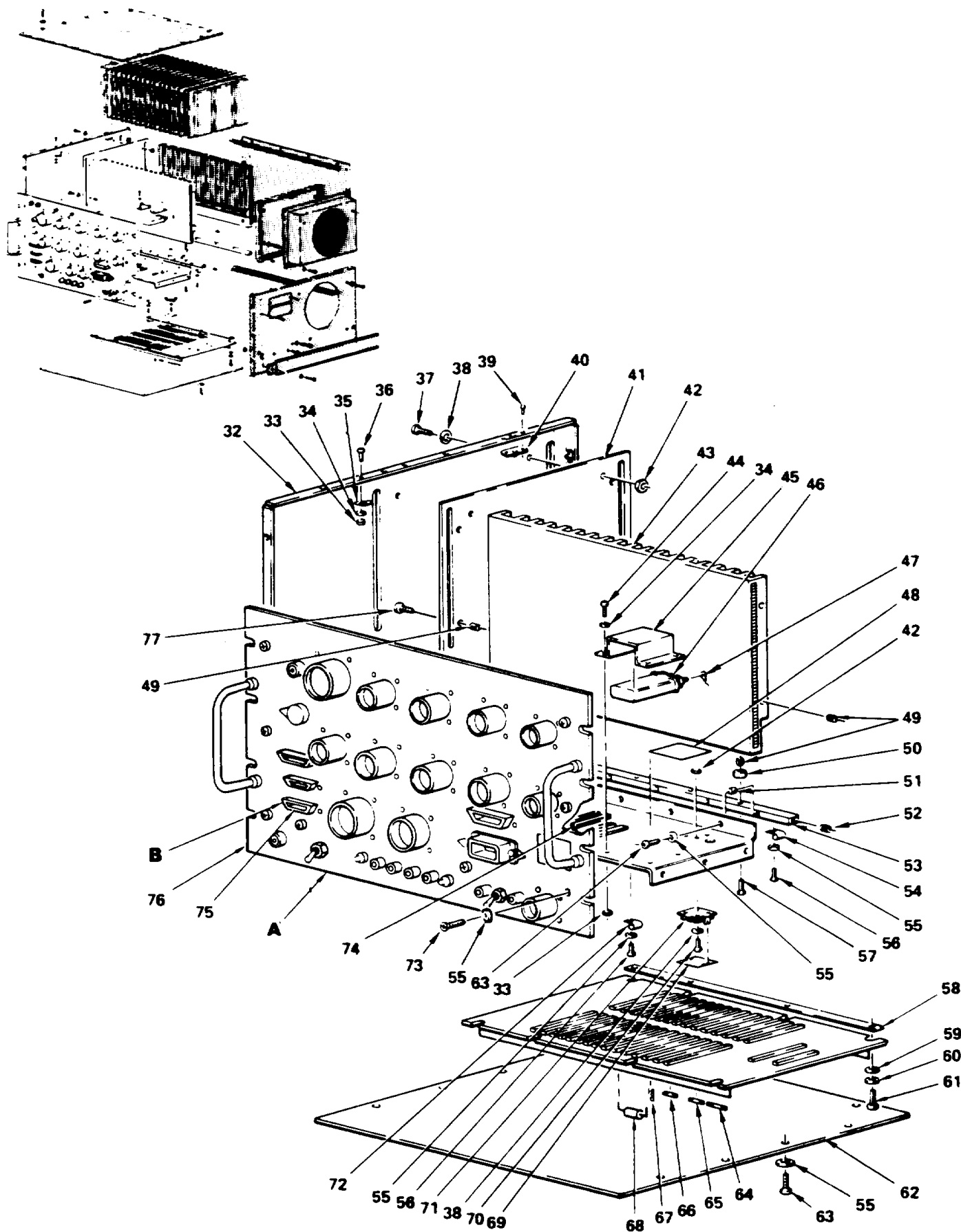
Figure 1. Test Set, Interface Unit TS-4221/U (Sheet 2 of 5)
