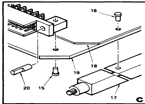
Figure 7. Circuit Card Assembly, TS RF (A9) (Sheet 2 of 2)
