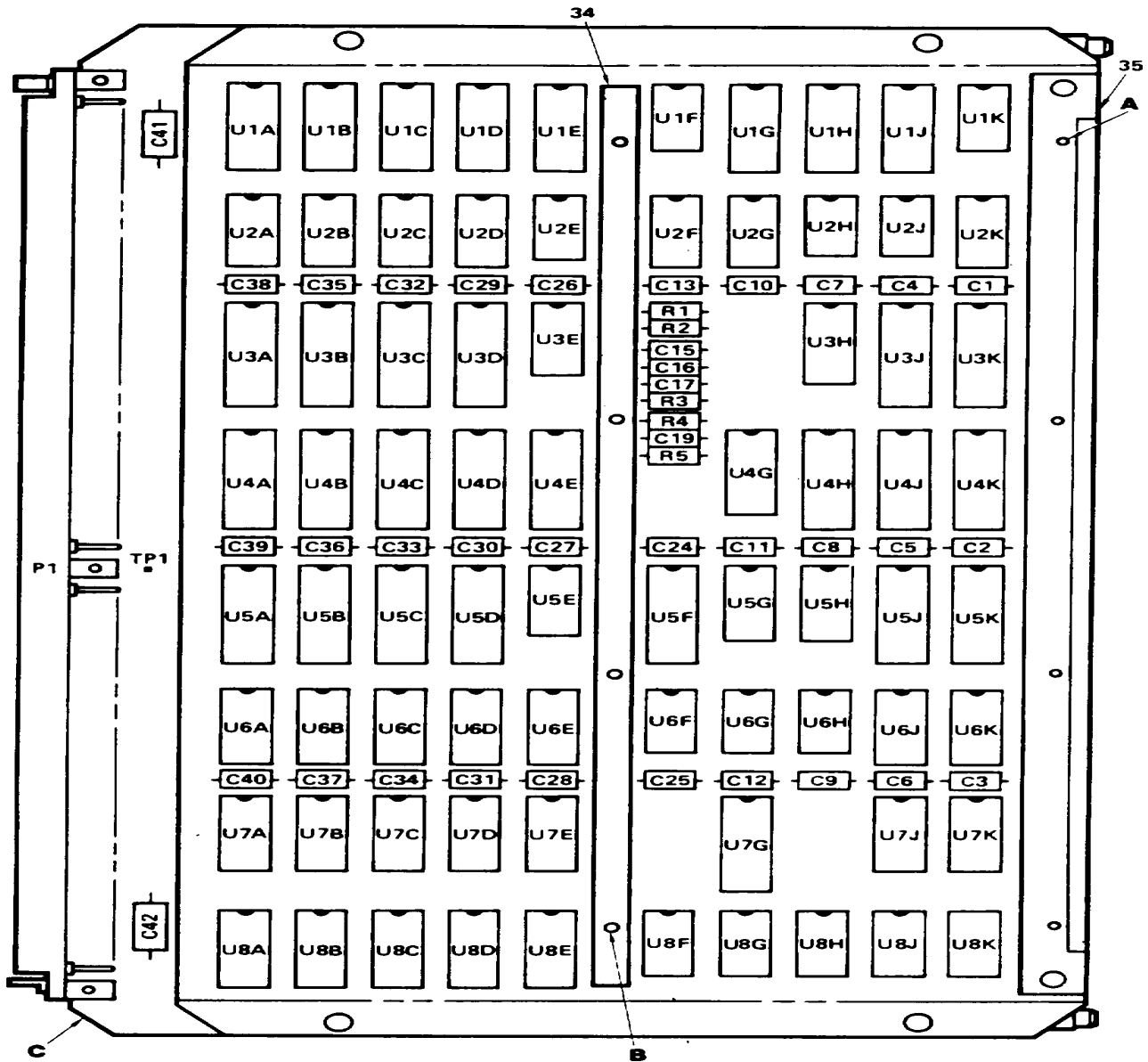
Figure 3. Circuit Card Assembly, C Interface (A3) (Sheet 1 of 2)
