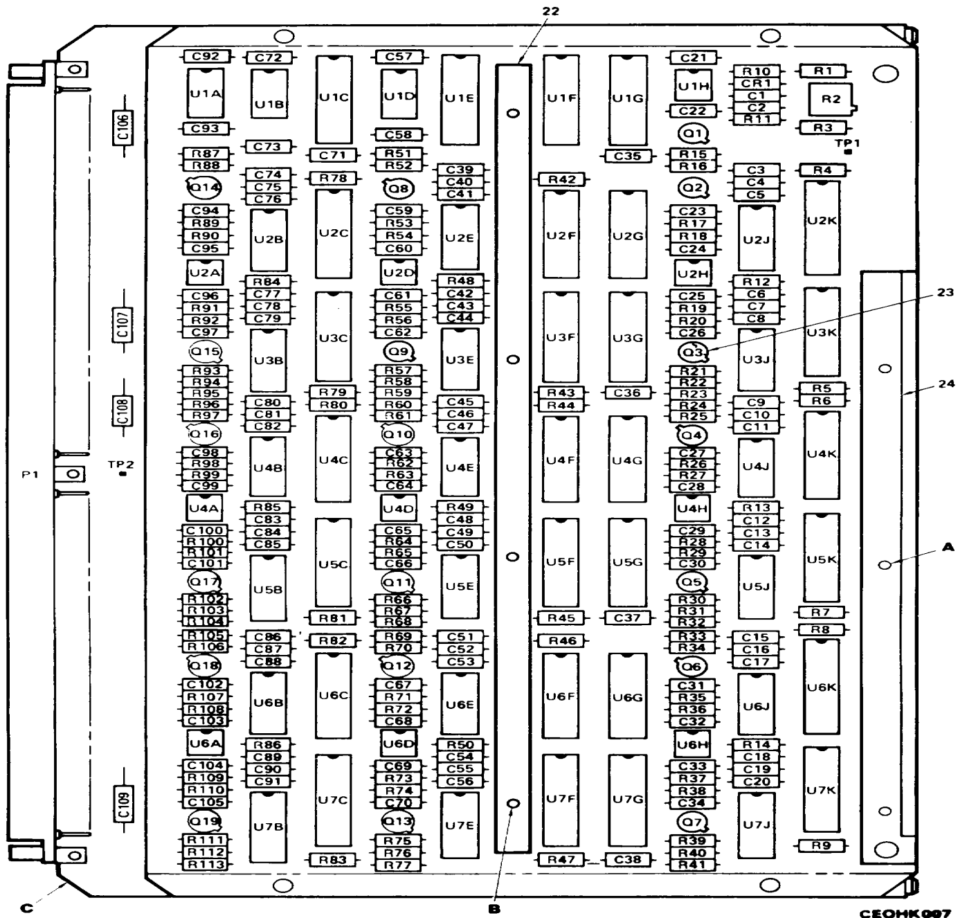
Figure 2. Circuit Card Assembly, TS D/A (A5, A6) (Sheet 1 of 3)
