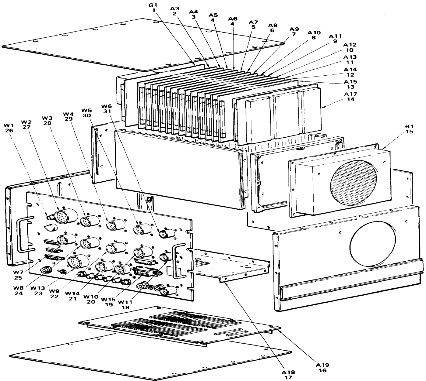
Figure 1. Test Set, Interface Unit TS-4221/U (Sheet 1 of 5)
