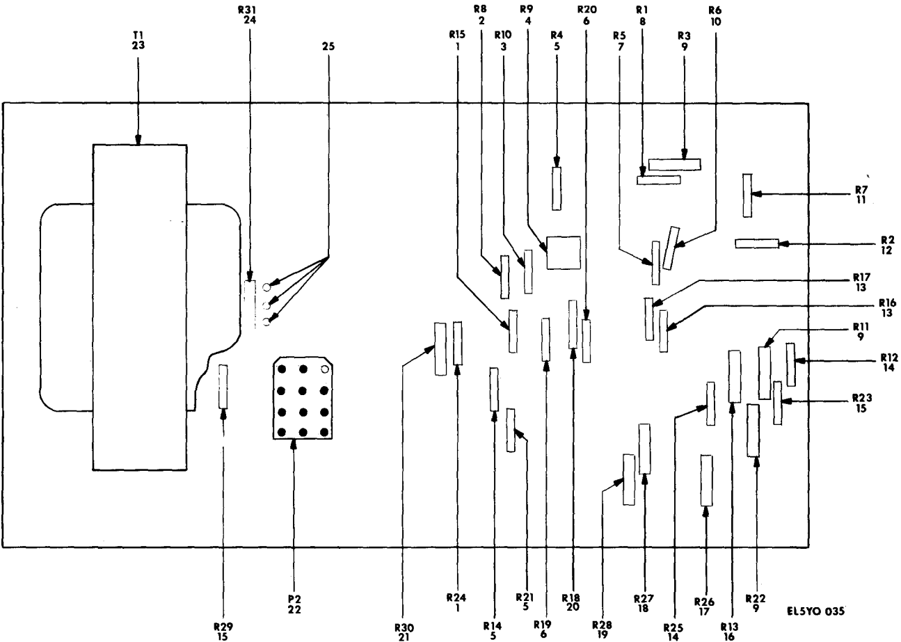
Figure 2-10. Power Supply PS6A (Sheet 1 of 4).
