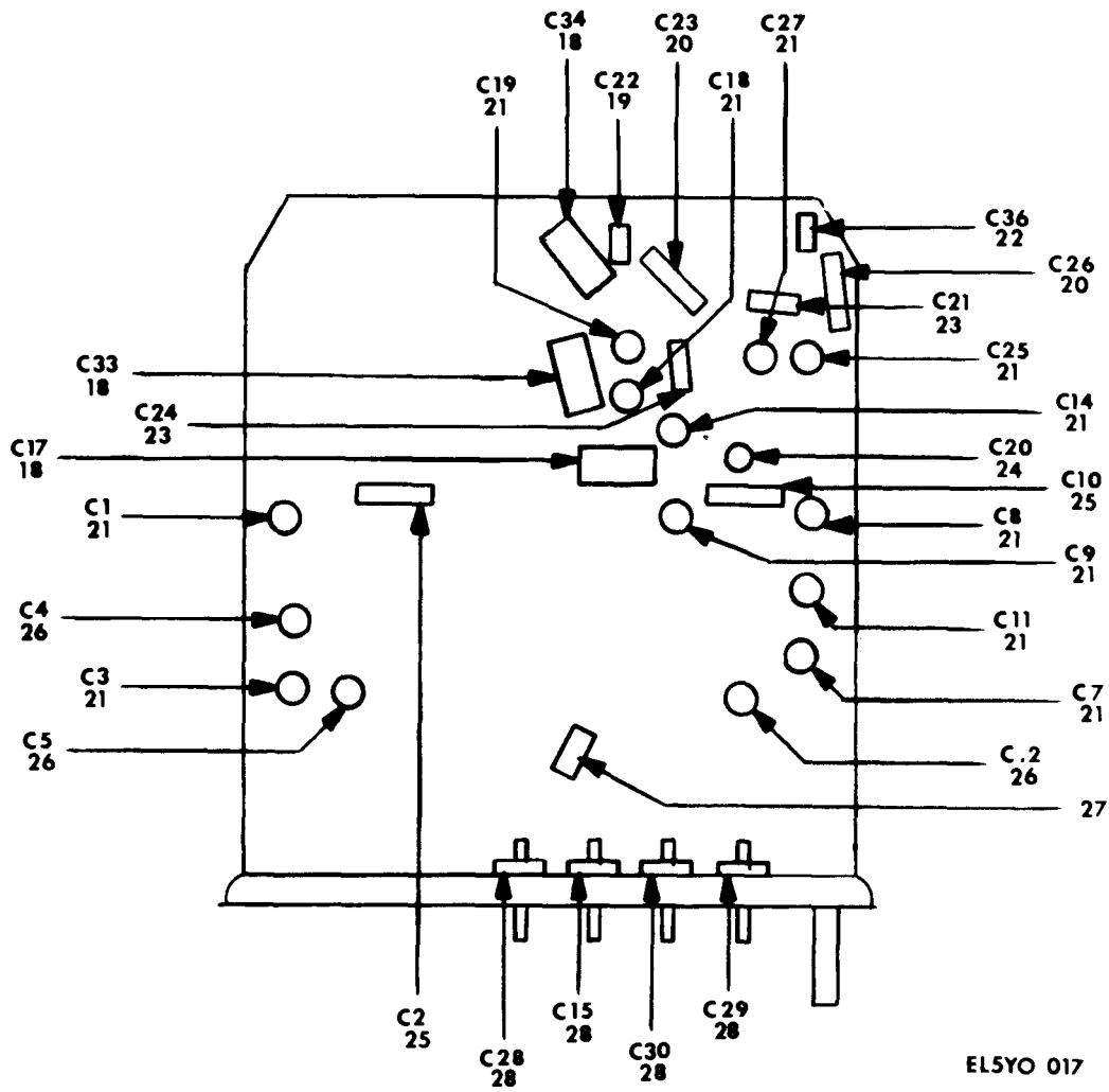
Figure 2-7. Module M9H (Sheet 2 of 5).
