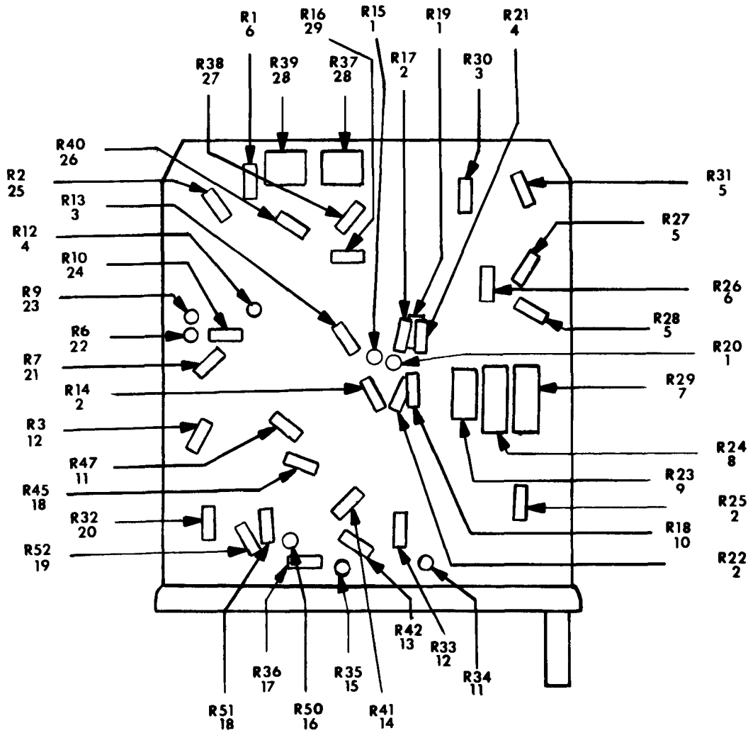
Figure 2-8. Module M10H (Sheet 1 of 7).
