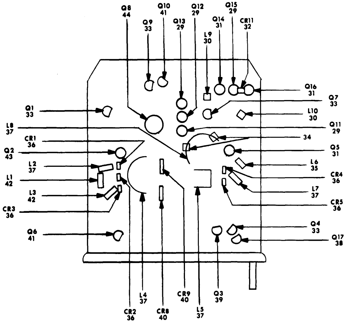
Figure 2-7. Module M9H (Sheet 3 of 5).
