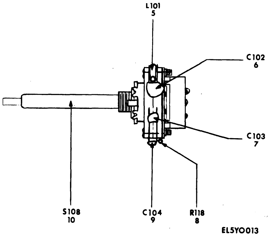
Figure 2-5. Sweep Generator SG-677A/U, Marker Size Switch Assembly (Sheet 2 of 2).
