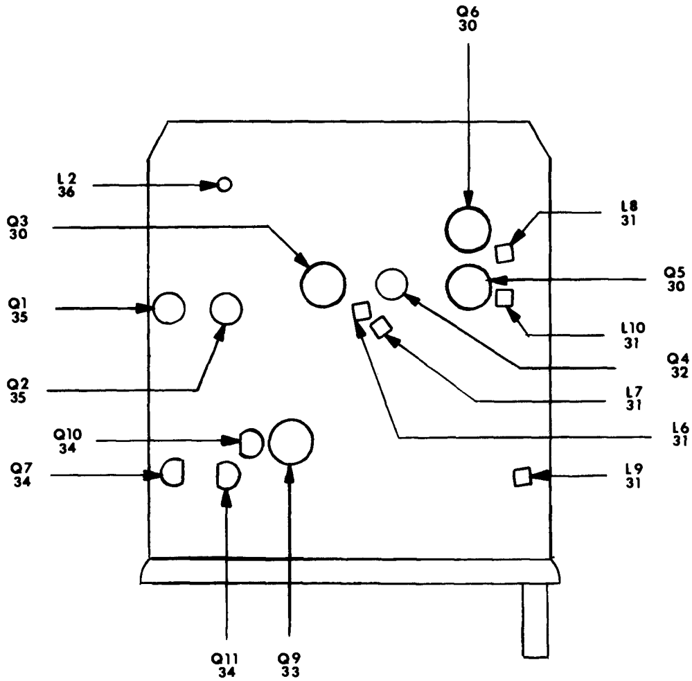
Figure 2-8. Module M10H (Sheet 2 of 7).
