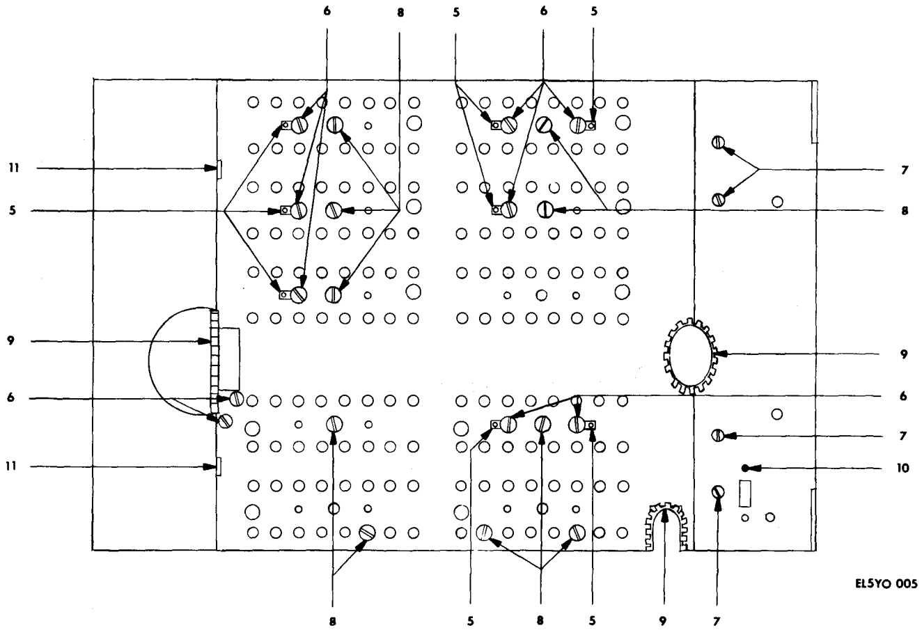
Figure 2-3 Sweep Generator SG-677A/U. Chassis Assembly, (Sheet 2 of 6).
