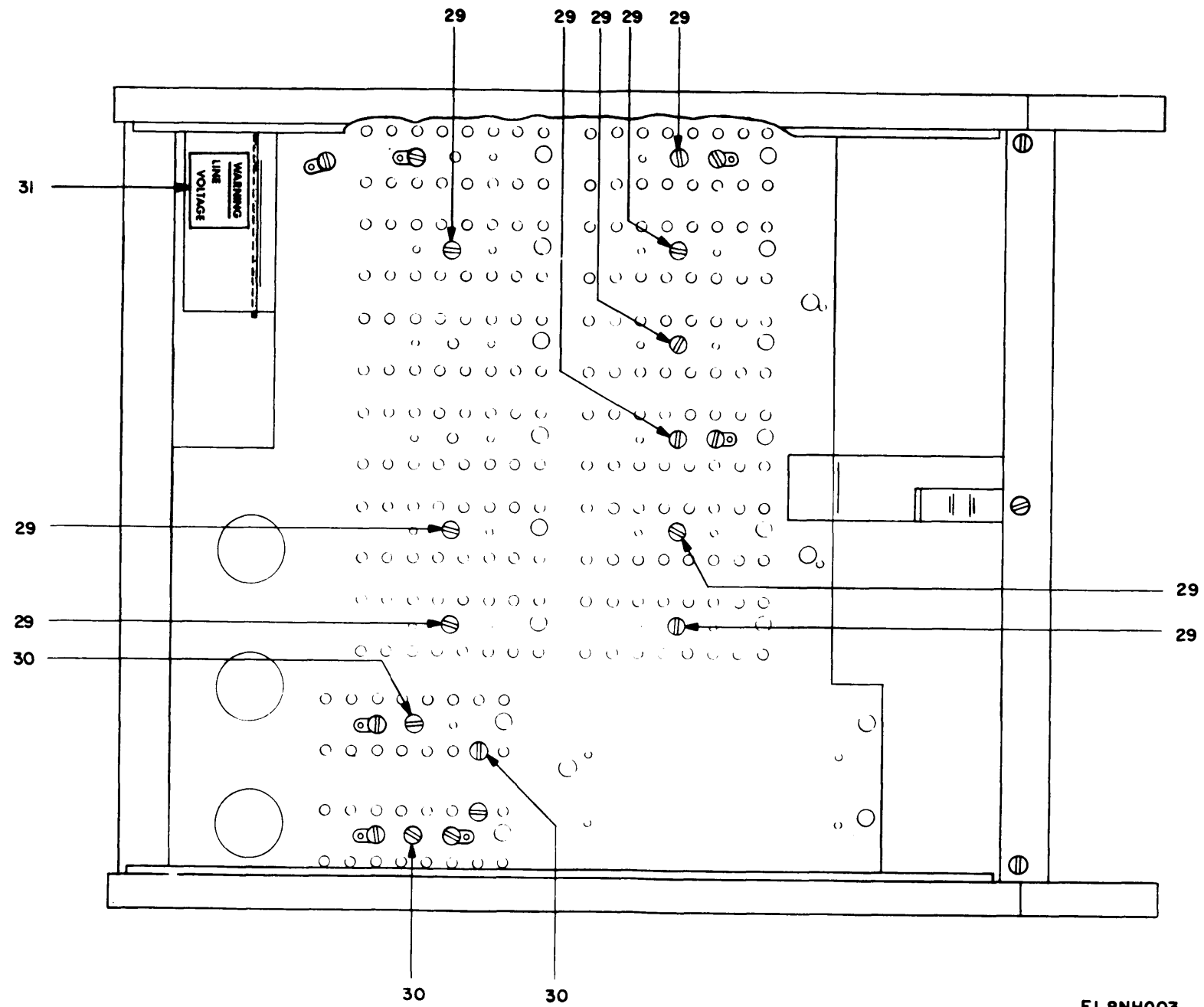
FIGURE 1. SIGNAL GENERATOR 8G-1170/U. (SHEET 3 OF 16)
