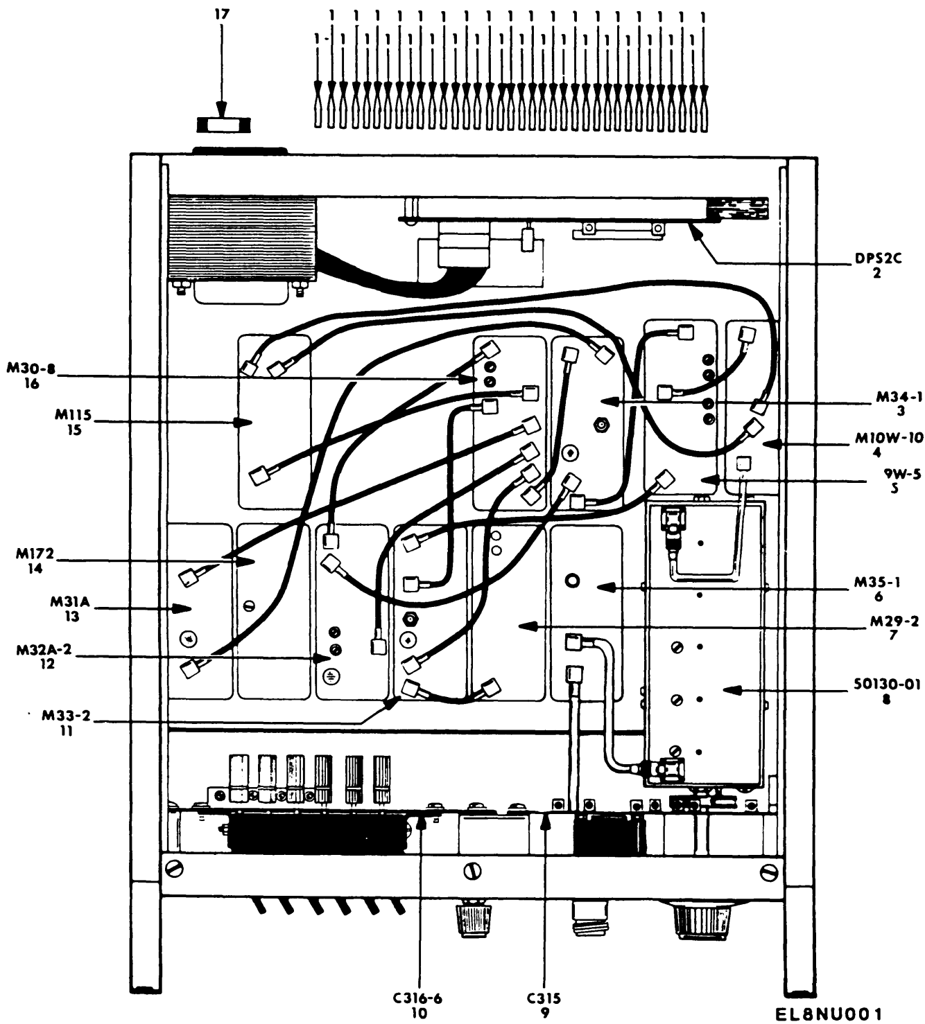
FIGURE 1. SIGNAL GENERATOR SG-1170/U. (SHEET 1 OF 15)
