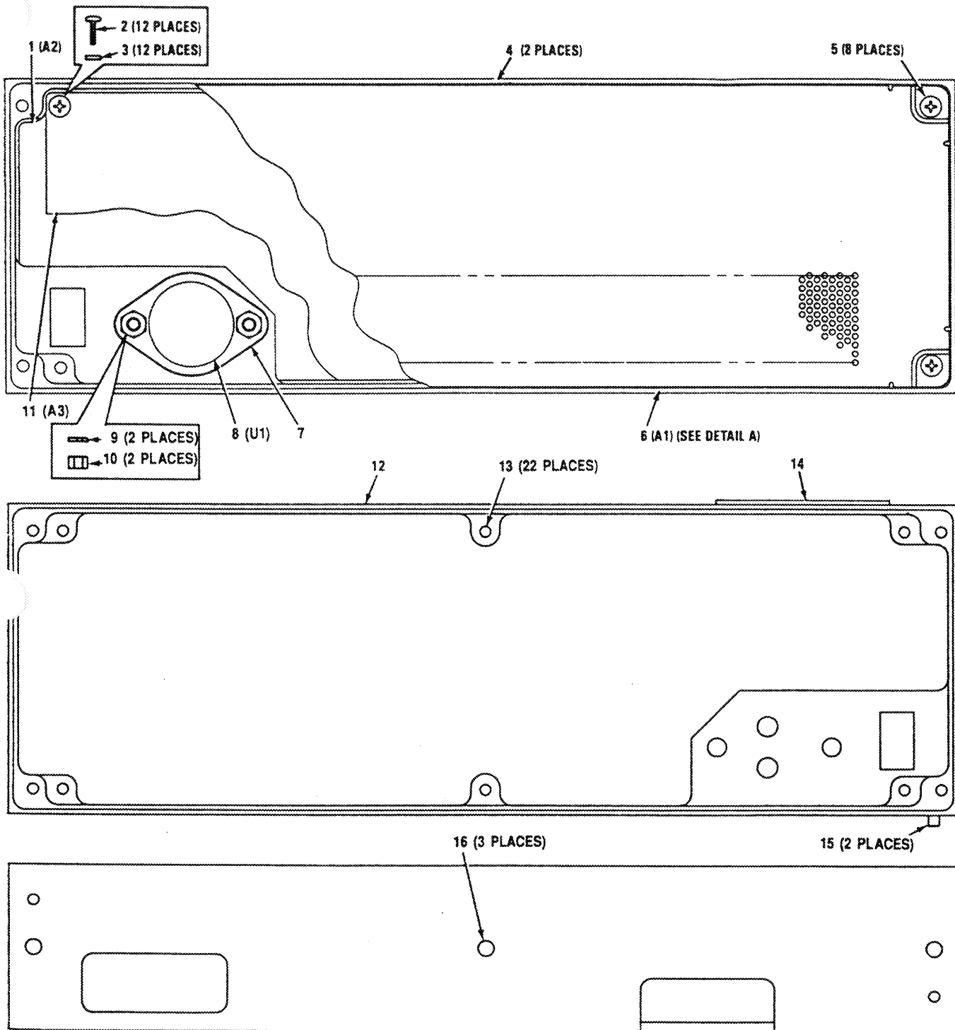
DETAIL A
