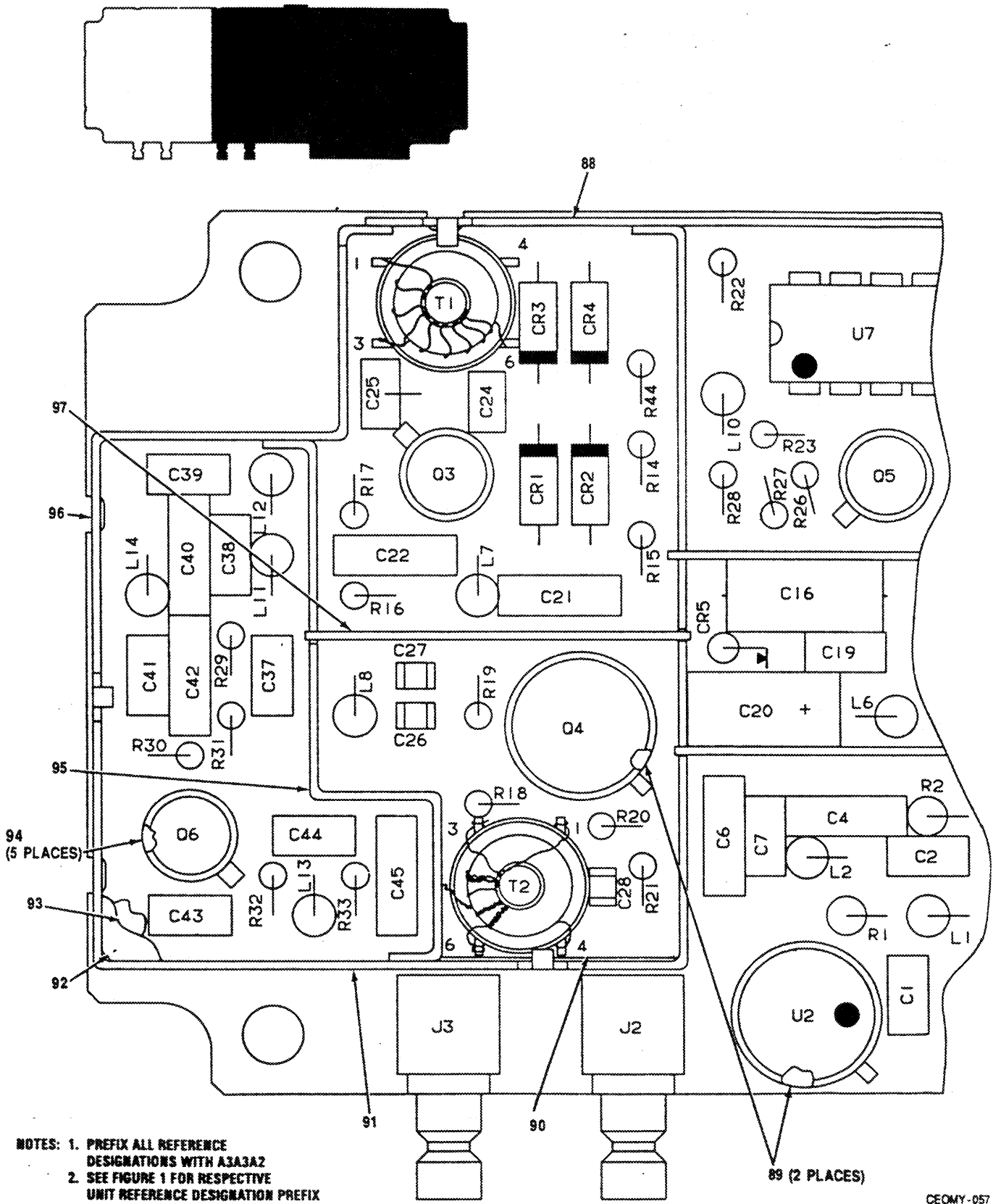
Figure 14. Reference CCA A3A3A2 (A3024370) (Sheet 2 of 5)
