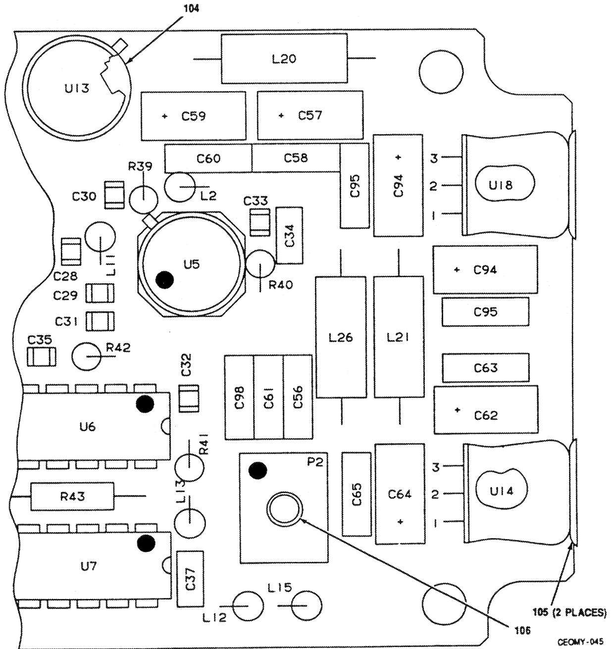
Figure 11. Sum Loop 2 CCA A3A2A2 (A3024360) (Sheet 5 of 6)
