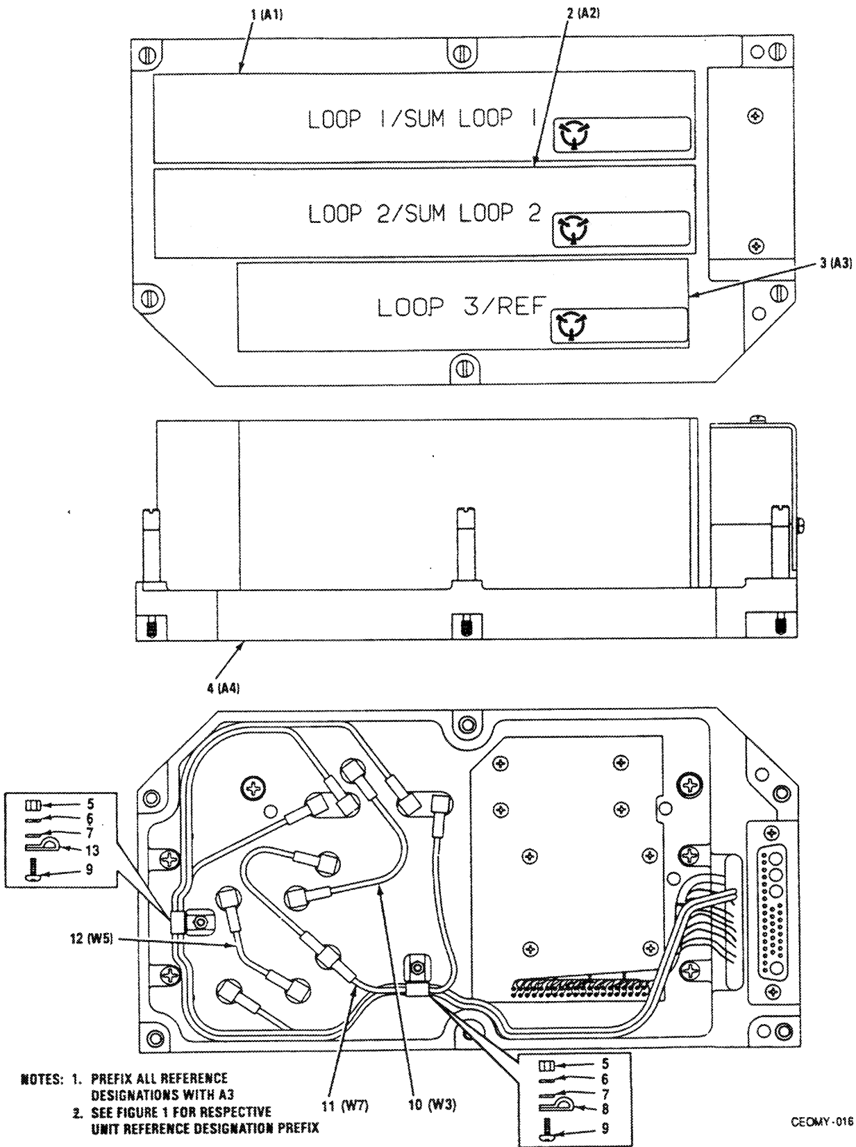
Figure 5. Synthesizer A3 (A3024340)
