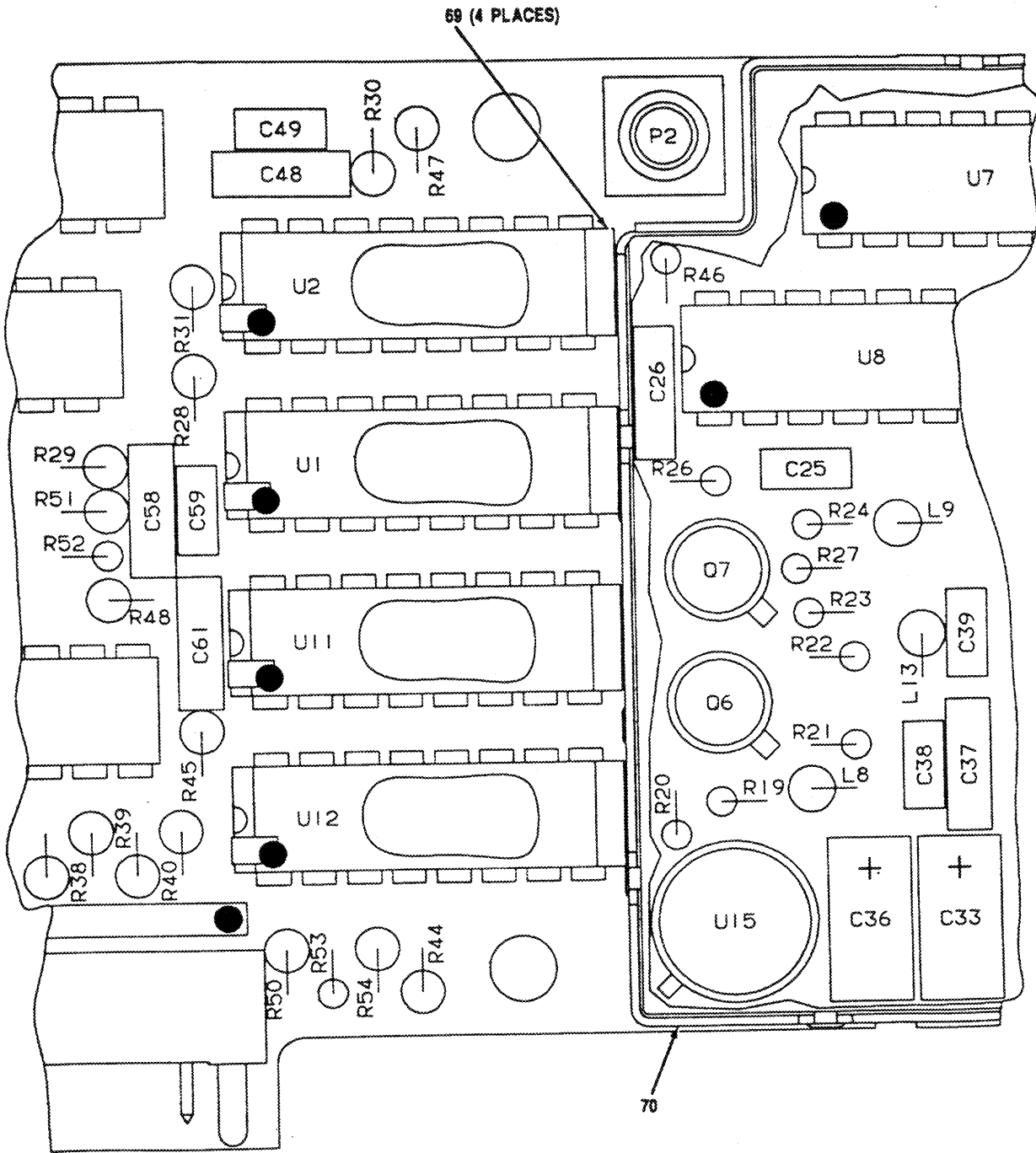
Figure 13. Loop 3 CCA A3A3A1 (A3024366) (Sheet 3 of 5)
