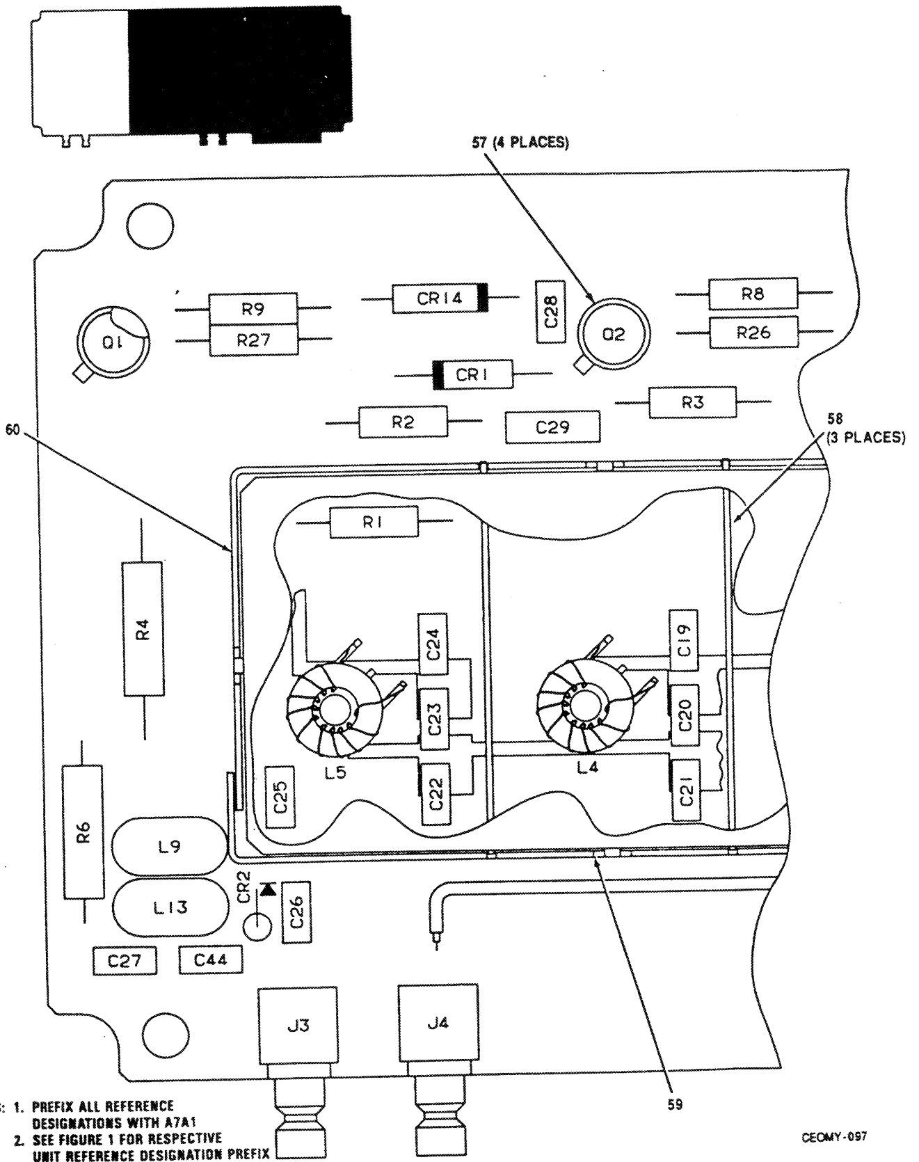
Figure 24. RF Switch CCA A7A1 (A3024650) (Sheet 2 of 5)
