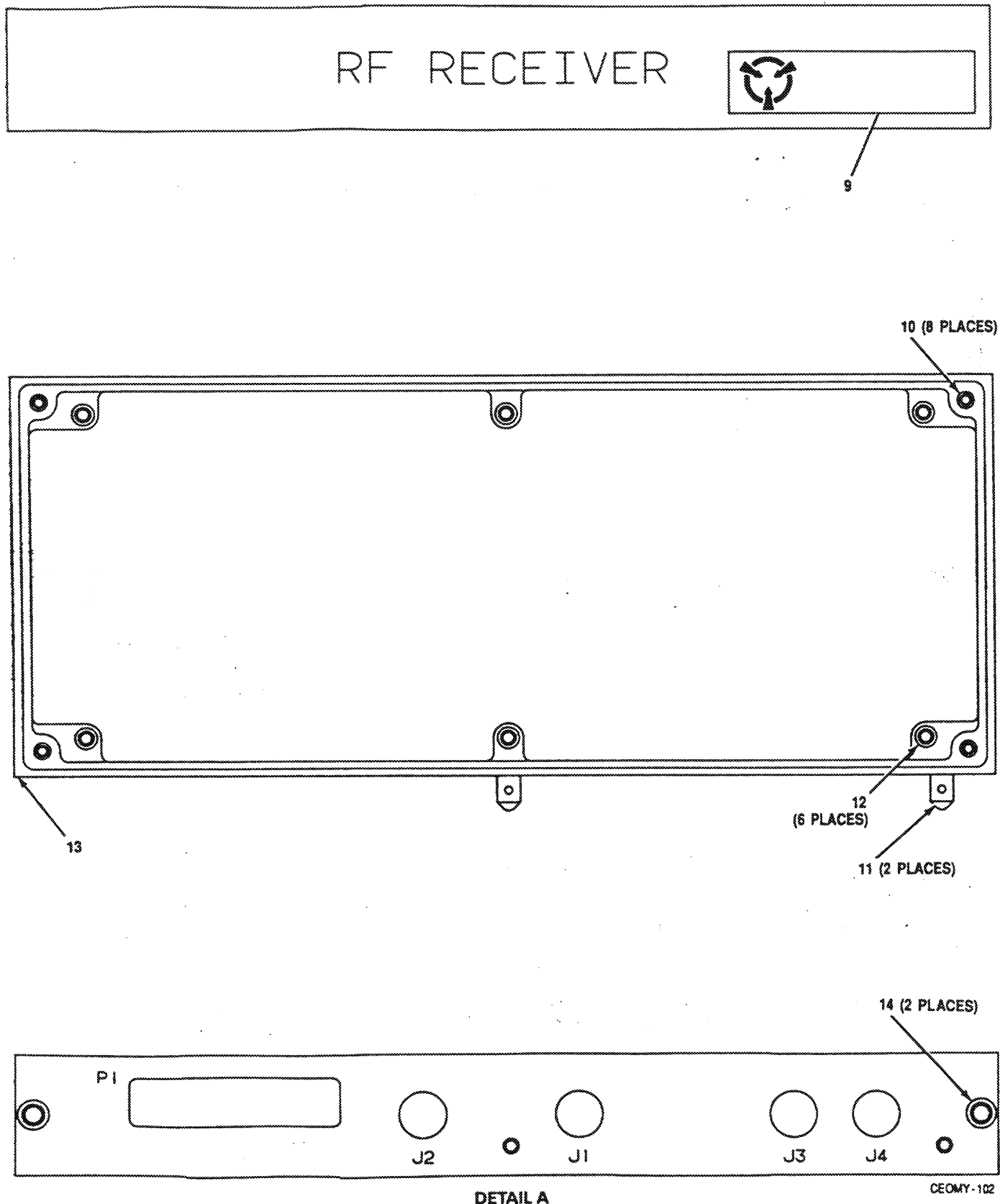
Figure 25. RF Receiver Assembly A8 (A3024644) (Sheet 2 of 2)
