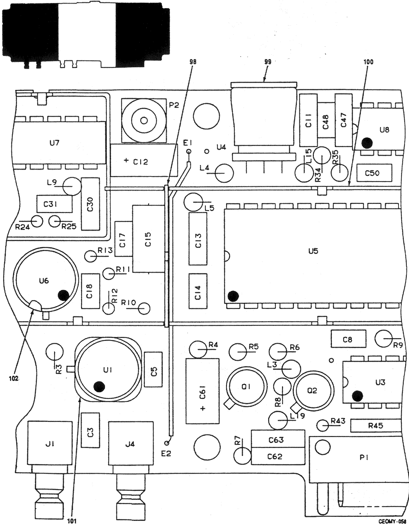
Figure 14. Reference GCA A3A3A2 (A3024370) (Sheet 3 of 5)
