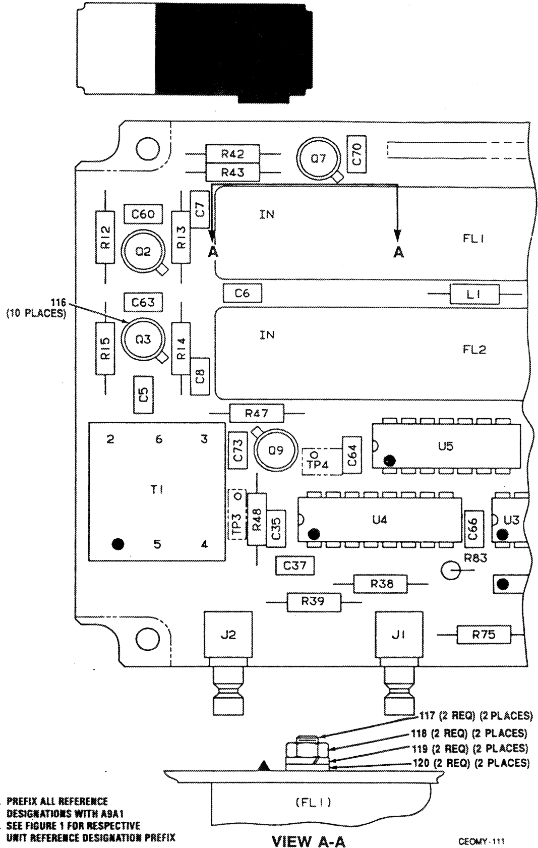
Figure 28. IF Receiver CCA A9A1 (A3024640) (Sheet 2 of 5)
