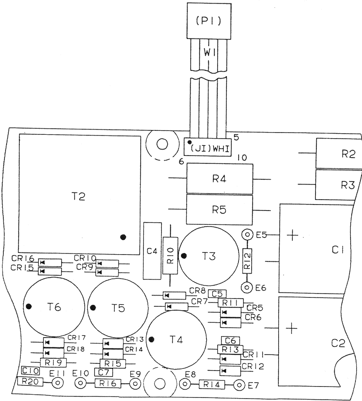
Figure 33. Regulator Output CCA PS1A3 (A3028133) (Sheet 3 of 5)
