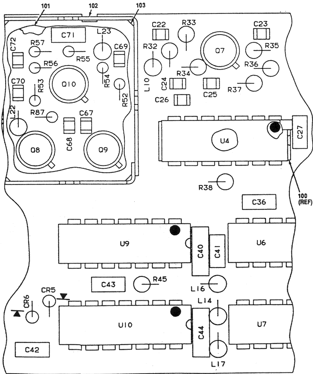
Figure 11. Sum Loop 2 CCA A3A2A2 (A3024360) (Sheet 4 of 6)
