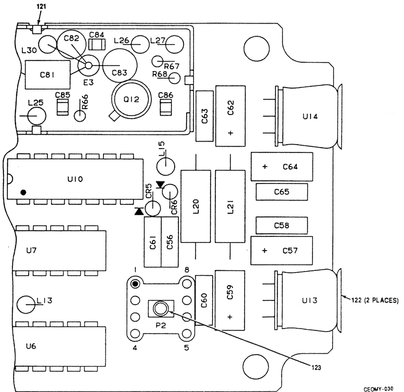
Figure 8. Sum Loop 1 CCA A3A1A2 (A3024350) (Sheet 5 of 6)
