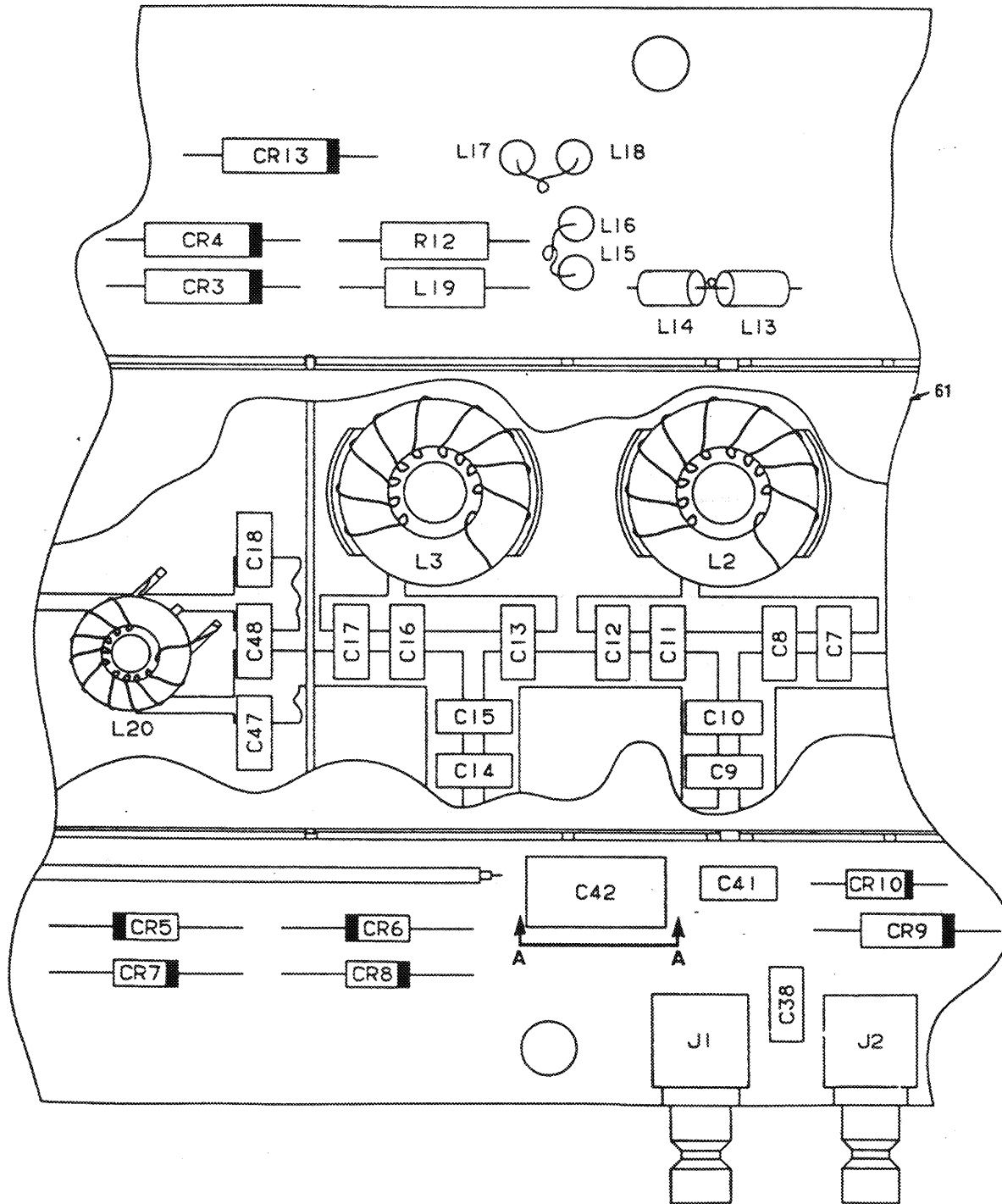
Figure 24. RF Switch CCA A7A1 (A3024650) (Sheet 3 of 5)
