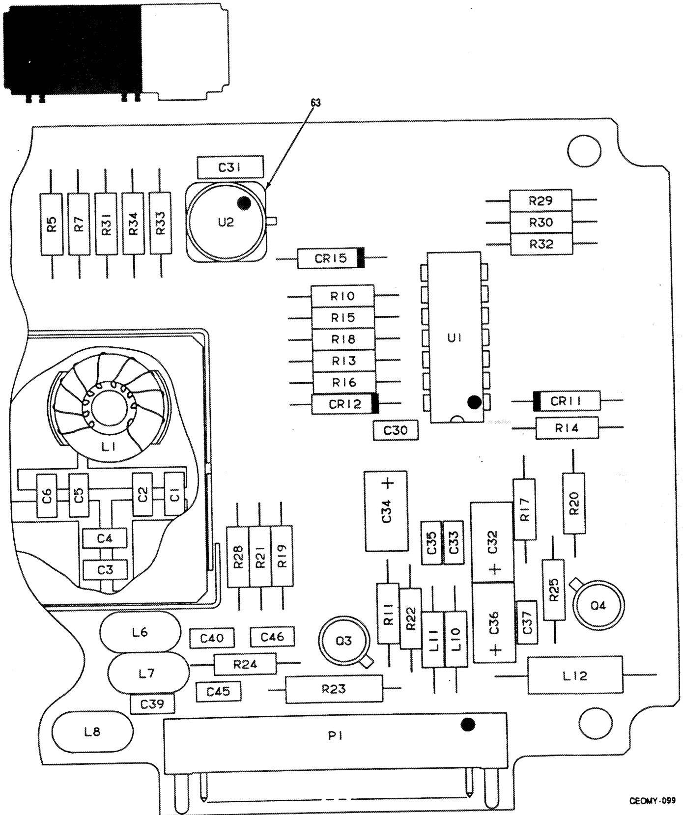
Figure 24. RF Switch CCA A7A1 (A3024650) (Sheet 4 of 5)
