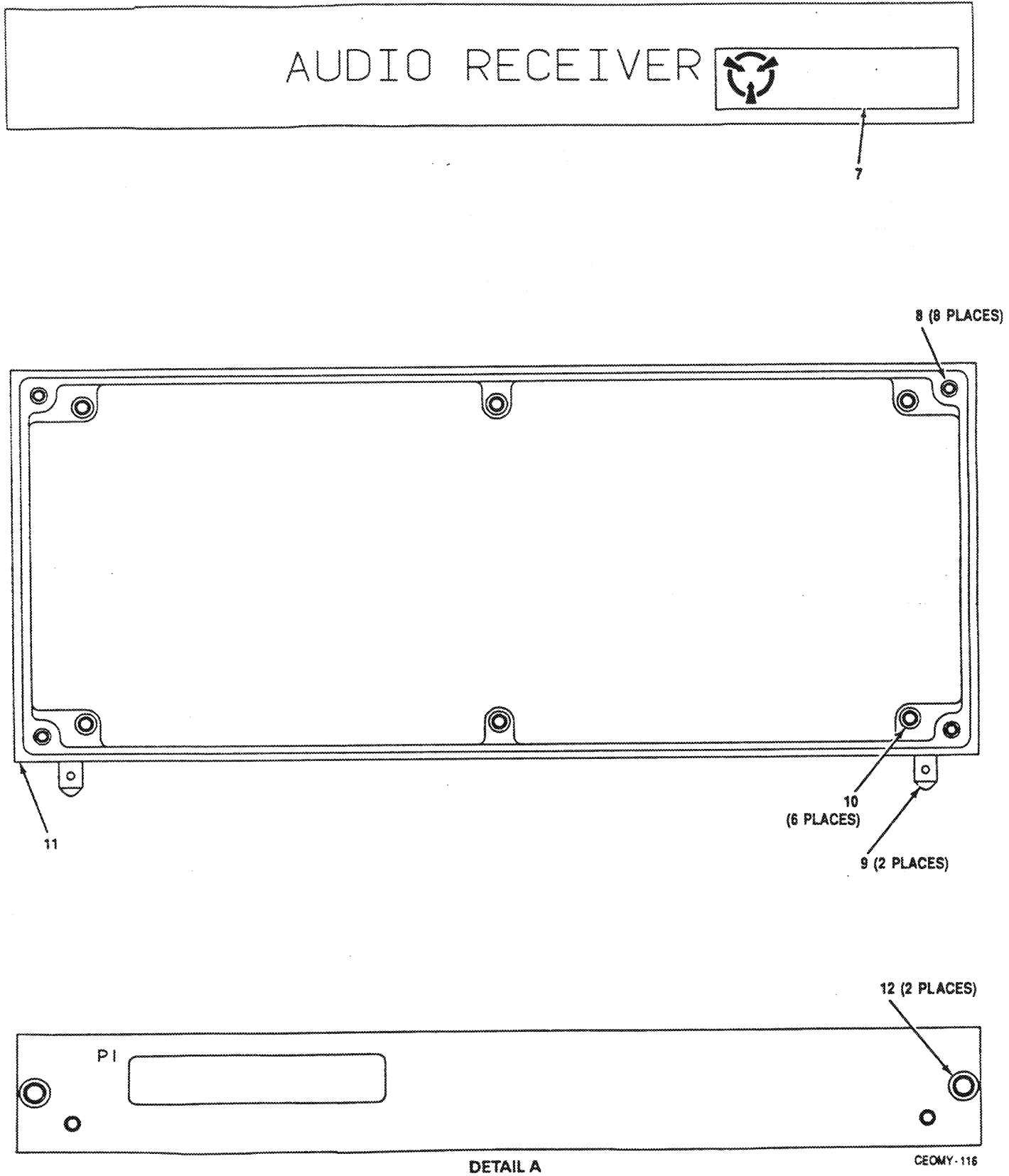
Figure 29. Audio Receiver Assembly A10 (A3024654) (Sheet 2 of 2)
