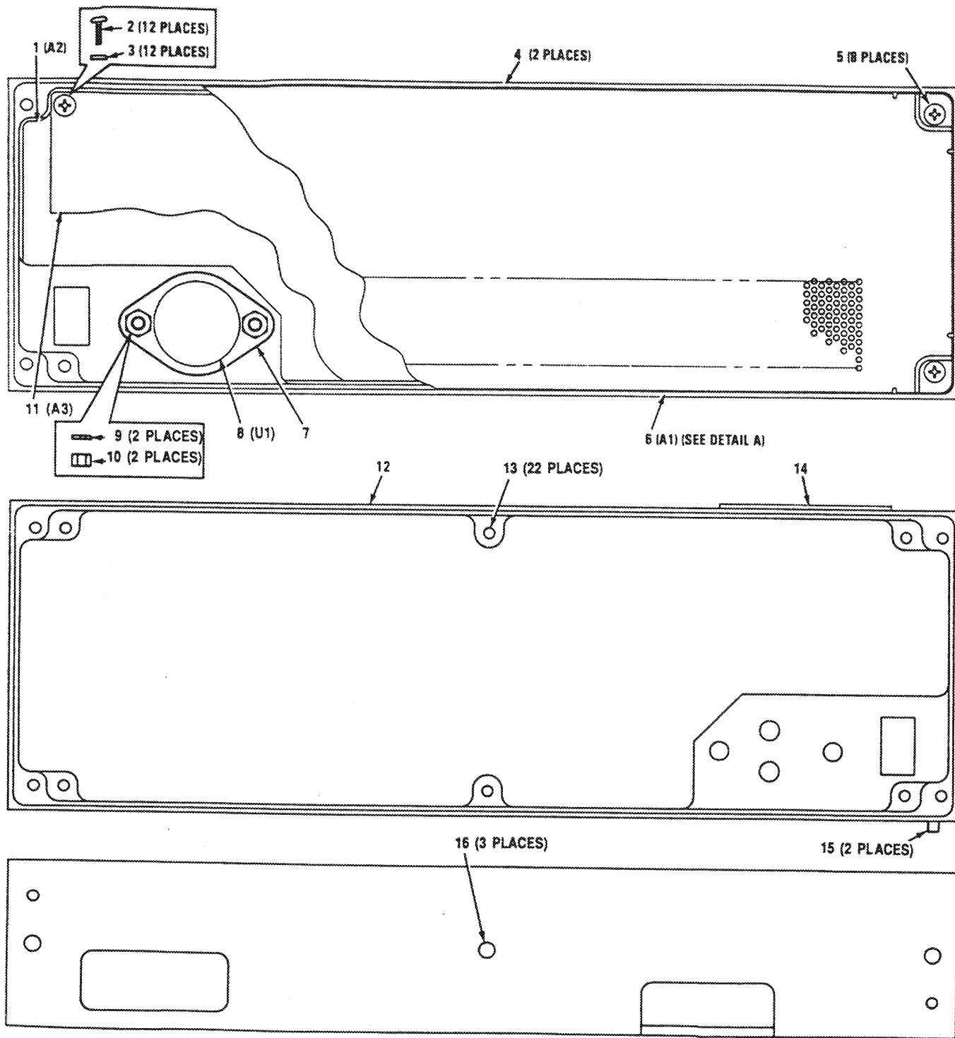
DETAIL A
