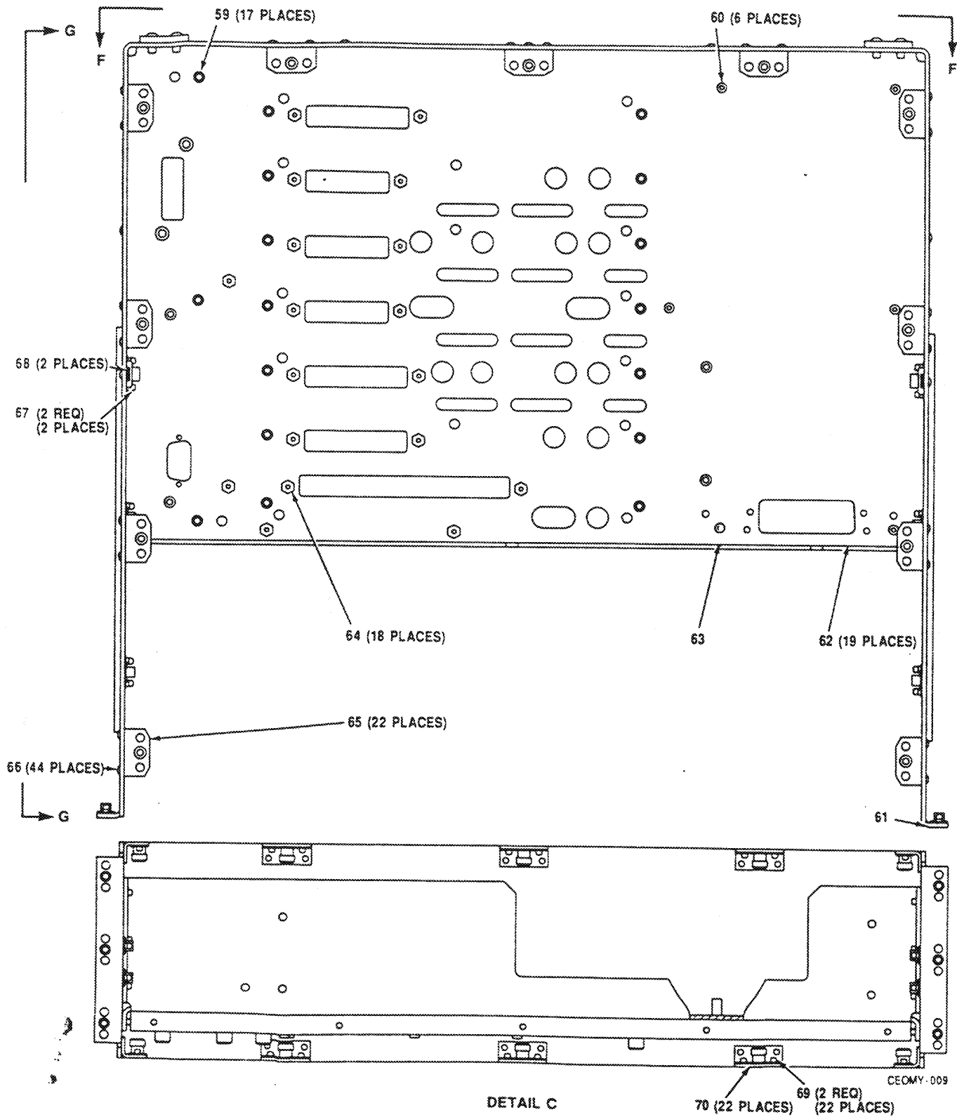
Figure 2. Chassis Assembly A1 (A3024604) (Sheet 5 of 9)
