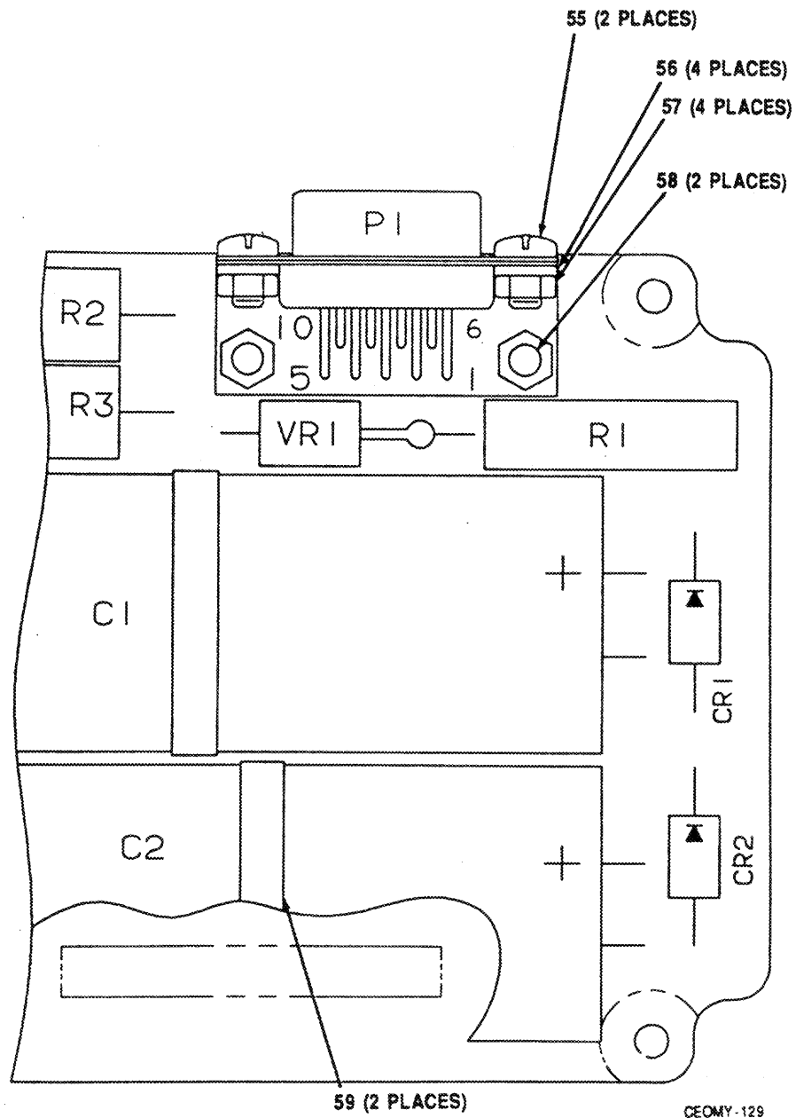
Figure 33. Regulator Output CCA PS1A3 (A3028133) (Sheet 4 of 5)
