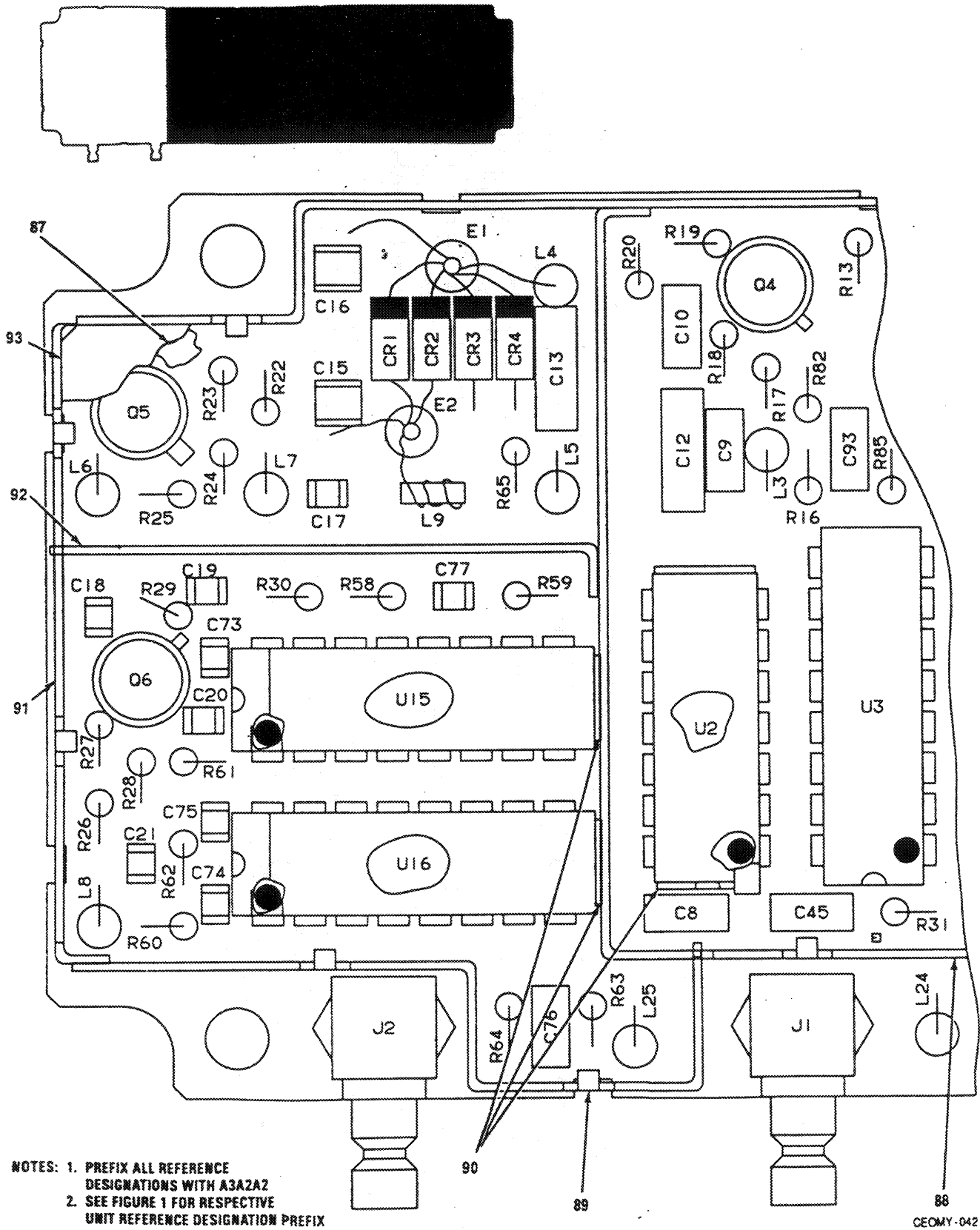
Figure 11. Sum Loop 2 CCA A3A2A2 (A3024360) (Sheet 2 of 6)
