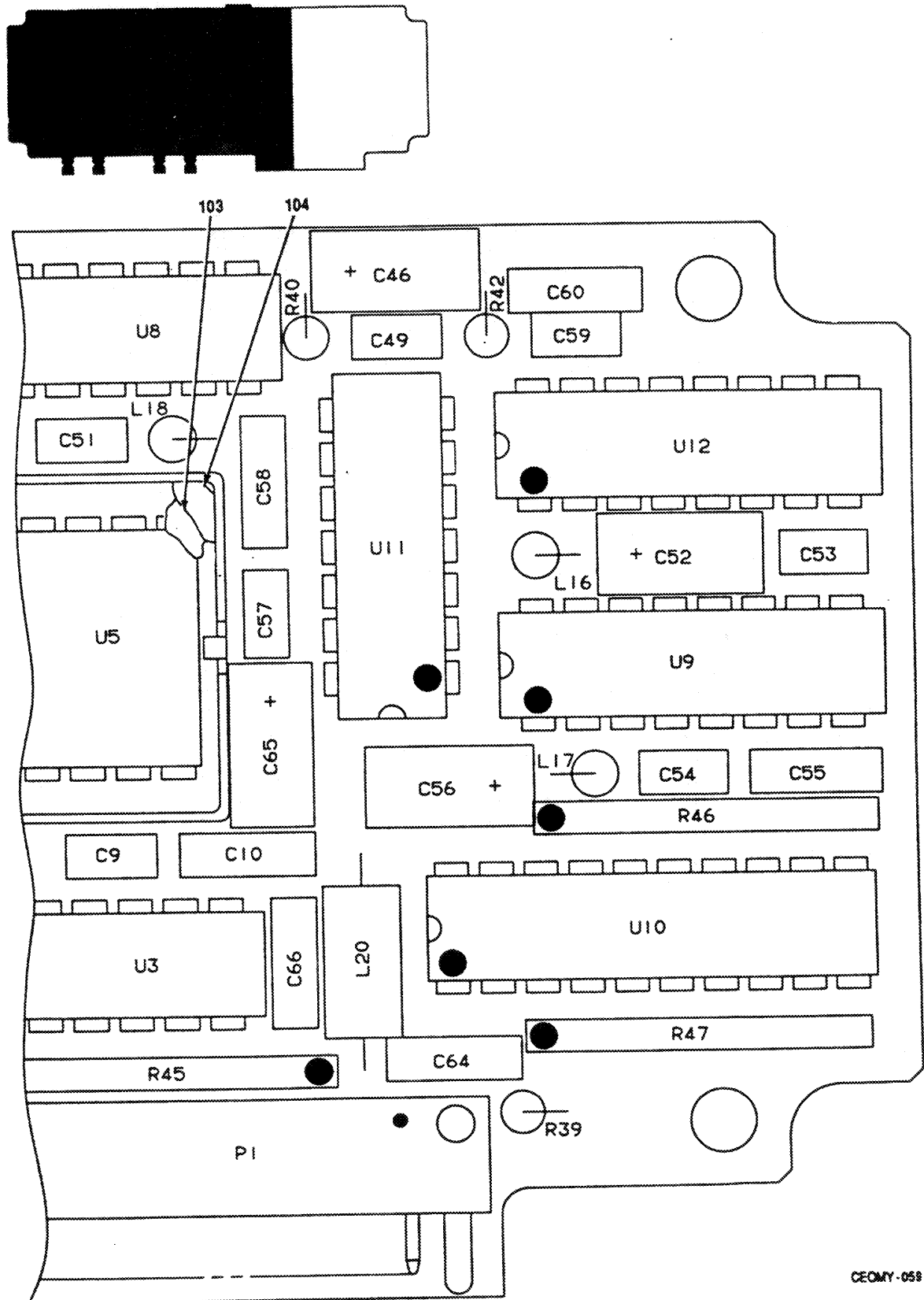
Figure 14. Reference CCA A3A3A2 (A3024370) (Sheet 4 of 5)
