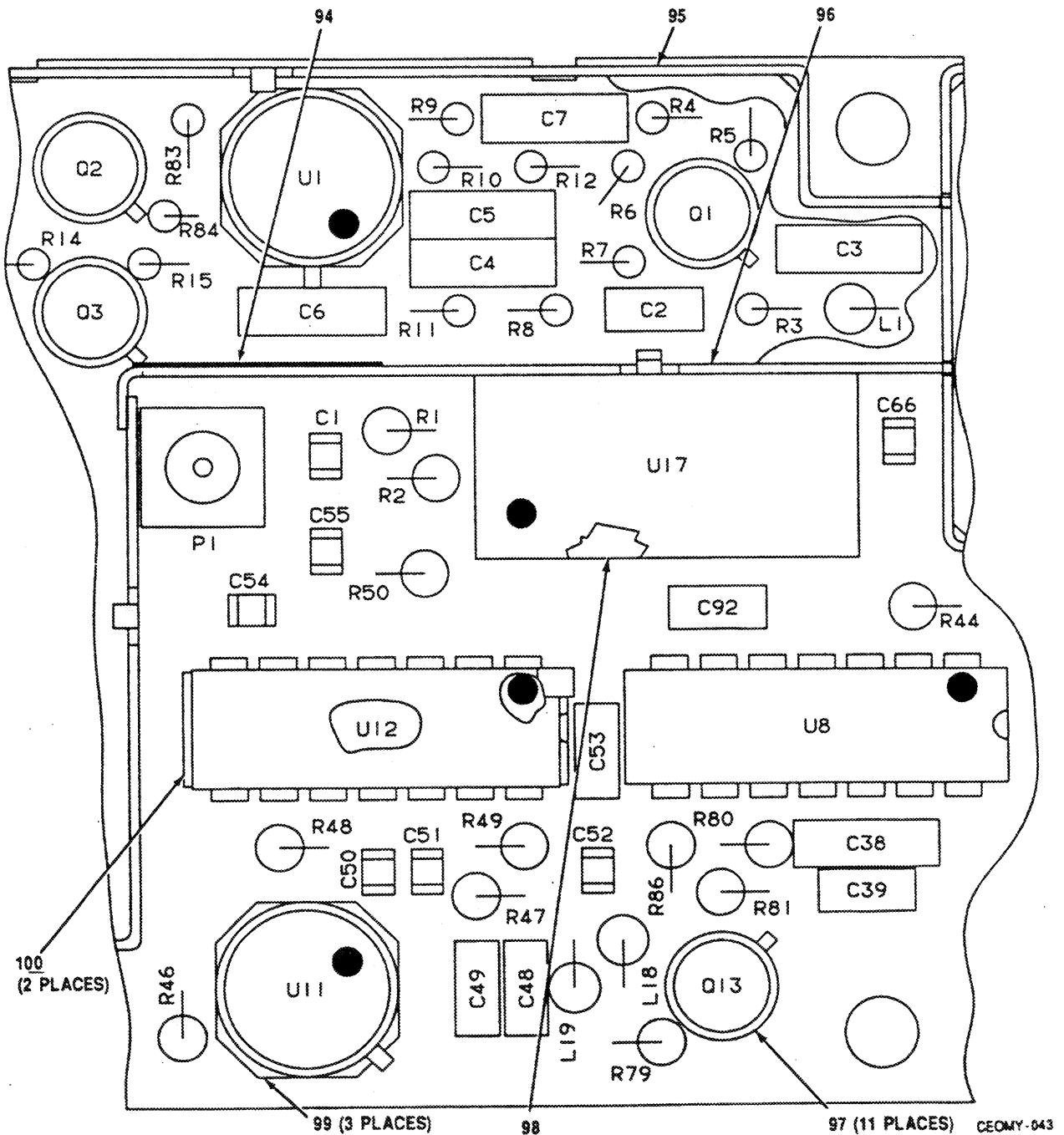
Figure 11. Sum Loop 2 CCA A3A2A2 (A3024360) (Sheet 3 of 6)
