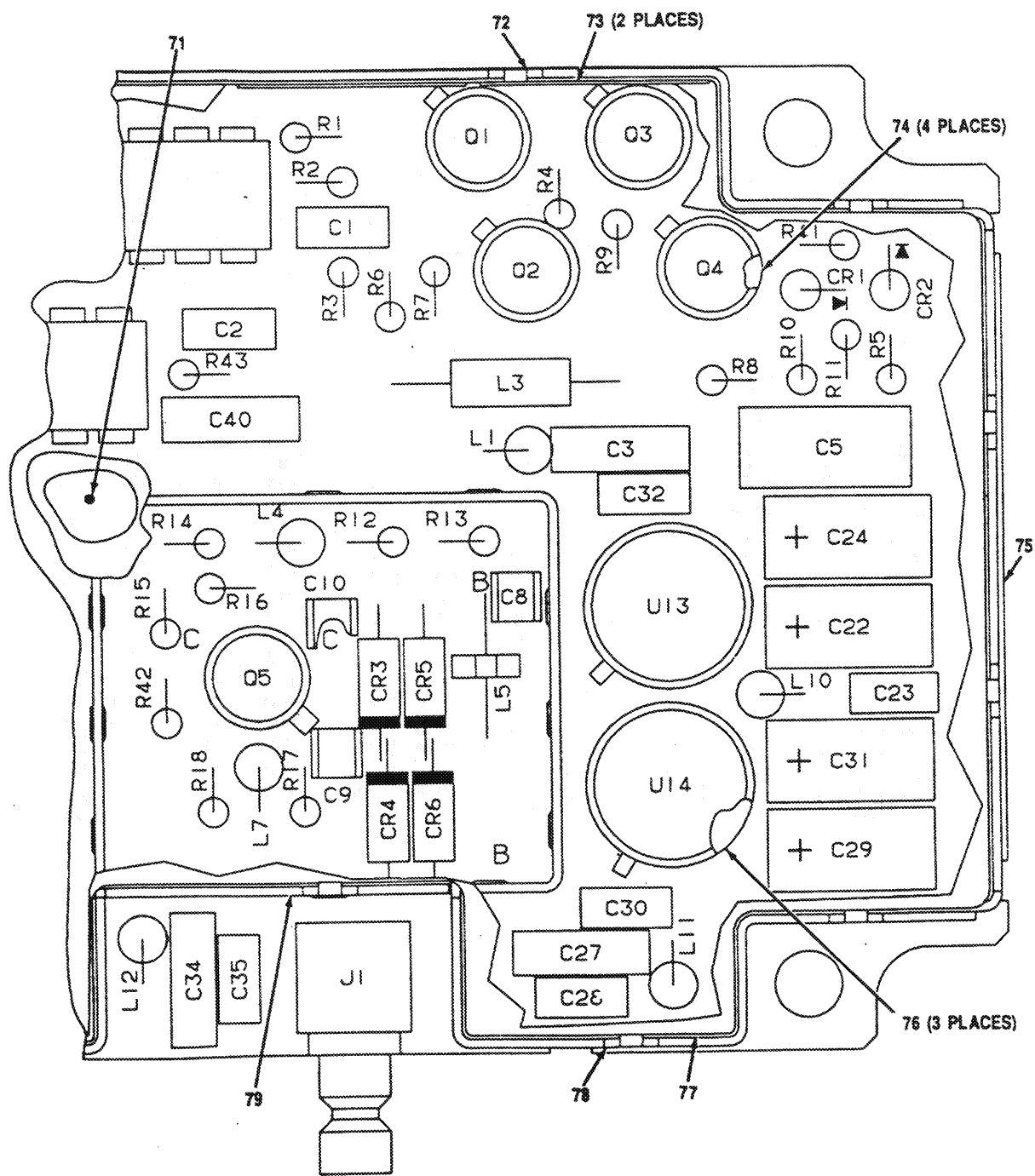
Figure 13. Loop 3 CCA A3A3A1 (A3024366) (Sheet 4 of 5)
