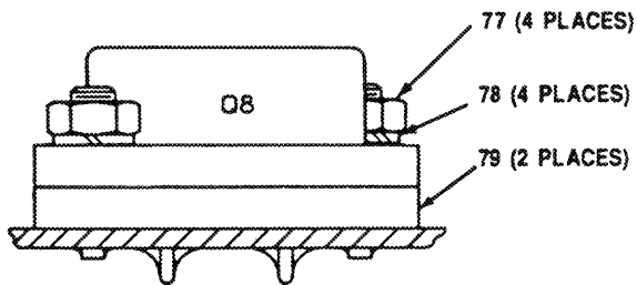
VIEW B-B
