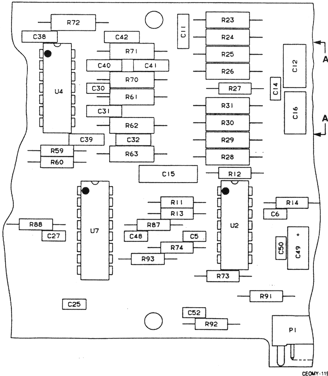
Figure 30. Audio Receiver CCA A10A1 (A3024655) (Sheet 3 of 5)
