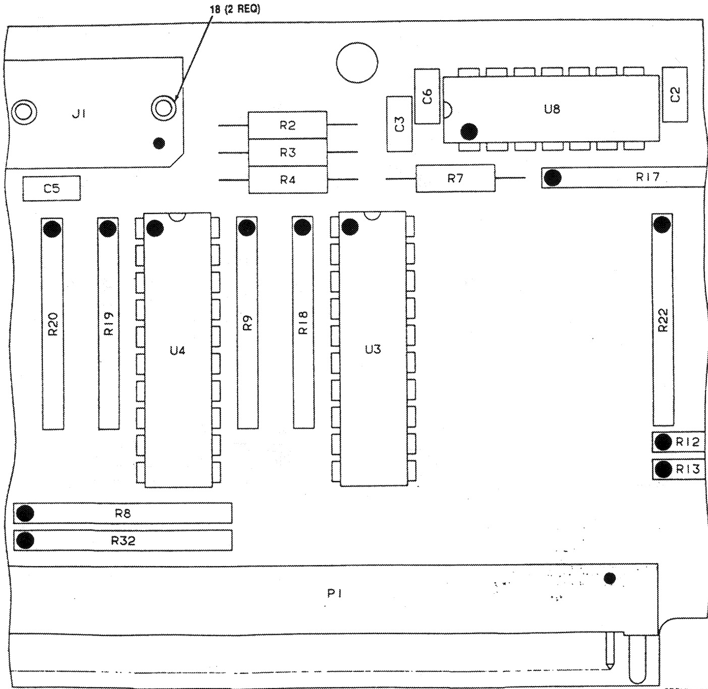
Figure 18. Status CCA A4A2 (A3024625) (Sheet 3 of 5)
