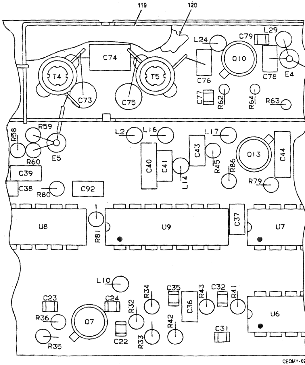
Figure 8. Sum Loop 1 CCA A3A1A2 (A3024350) (Sheet 4 of 6)
