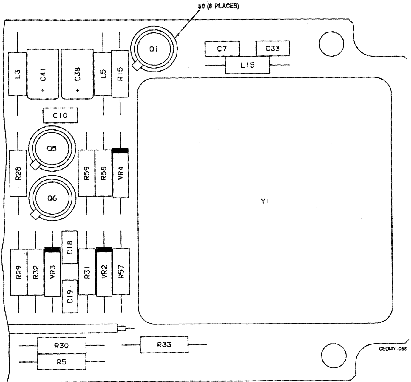
Figure 17. Reference Oscillator CCA A4A1 (A3024621) (Sheet 5 of 6)
