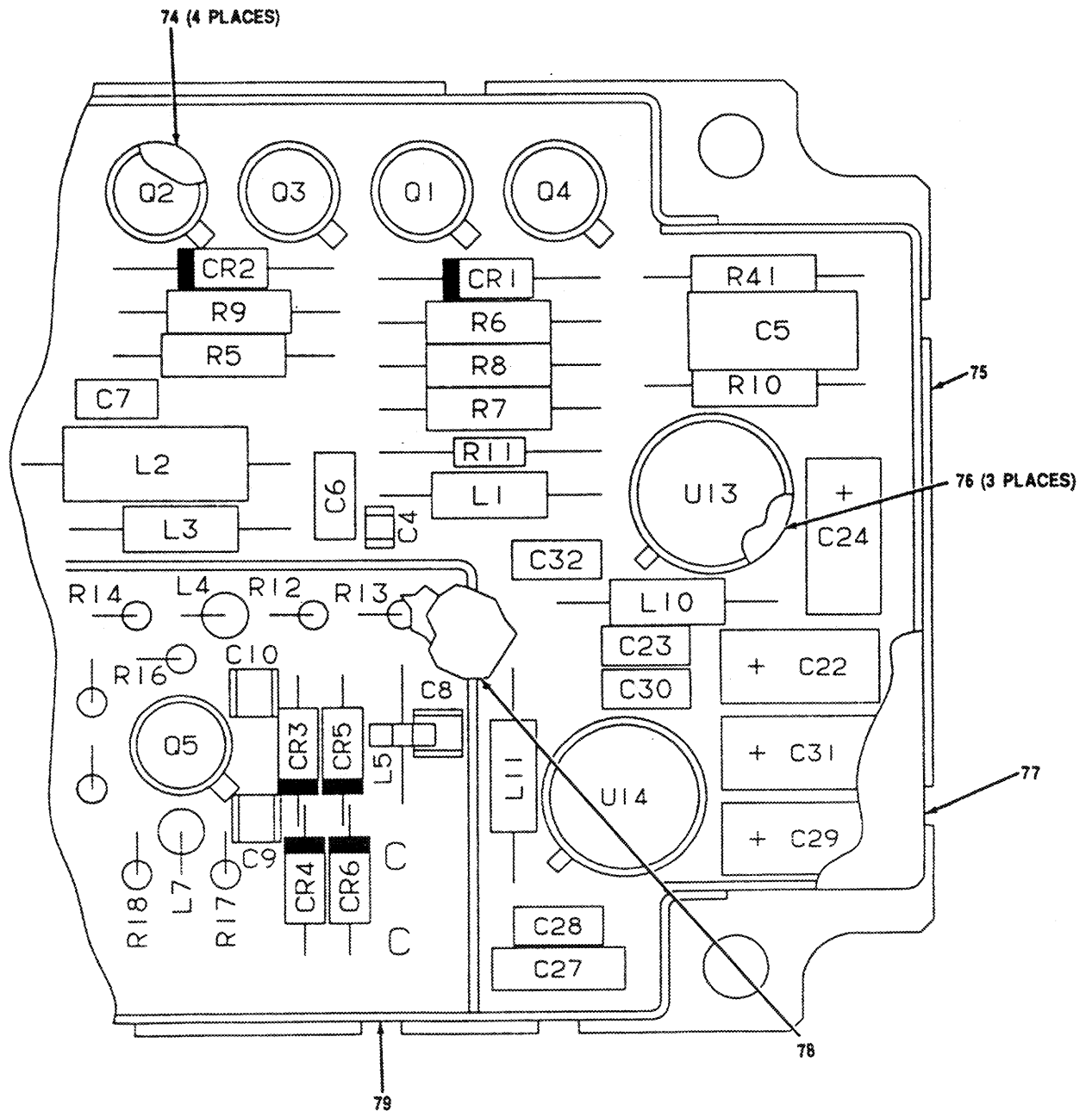
Figure 10. Loop 2 CCA A3A2A1 (A3024356) (Sheet 5 of 6)
