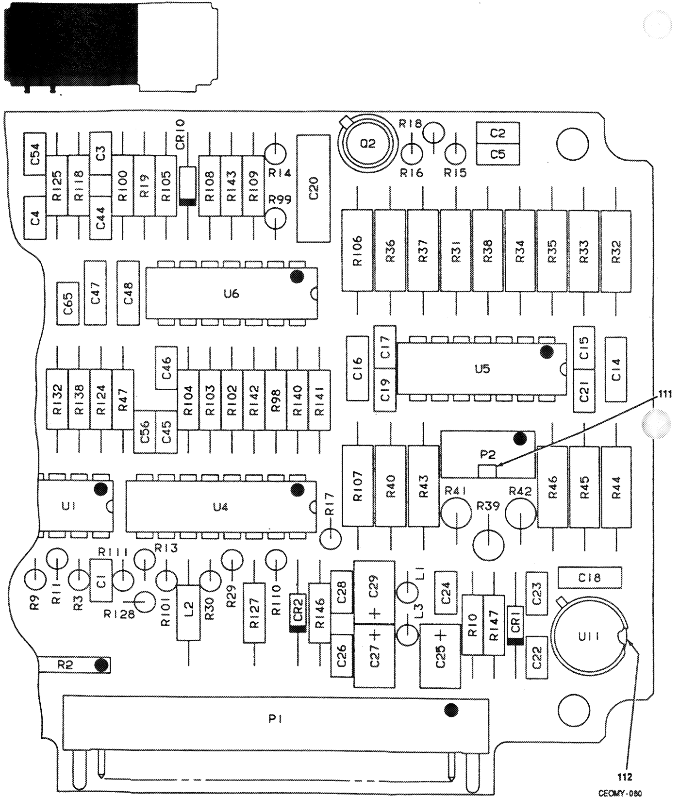
Figure 20. Audio Sideband Exciter CCA A5A1 (A3024630) (Sheet 4 of 5)
