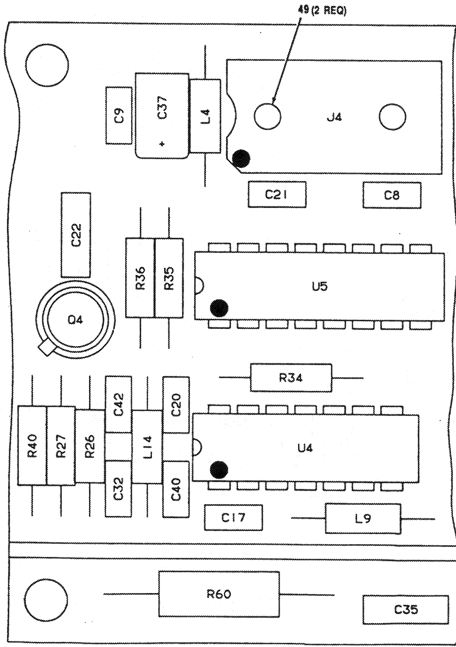
Figure 17. Reference Oscillator CCA A4A1 (A3024621) (Sheet 4 of 6)
