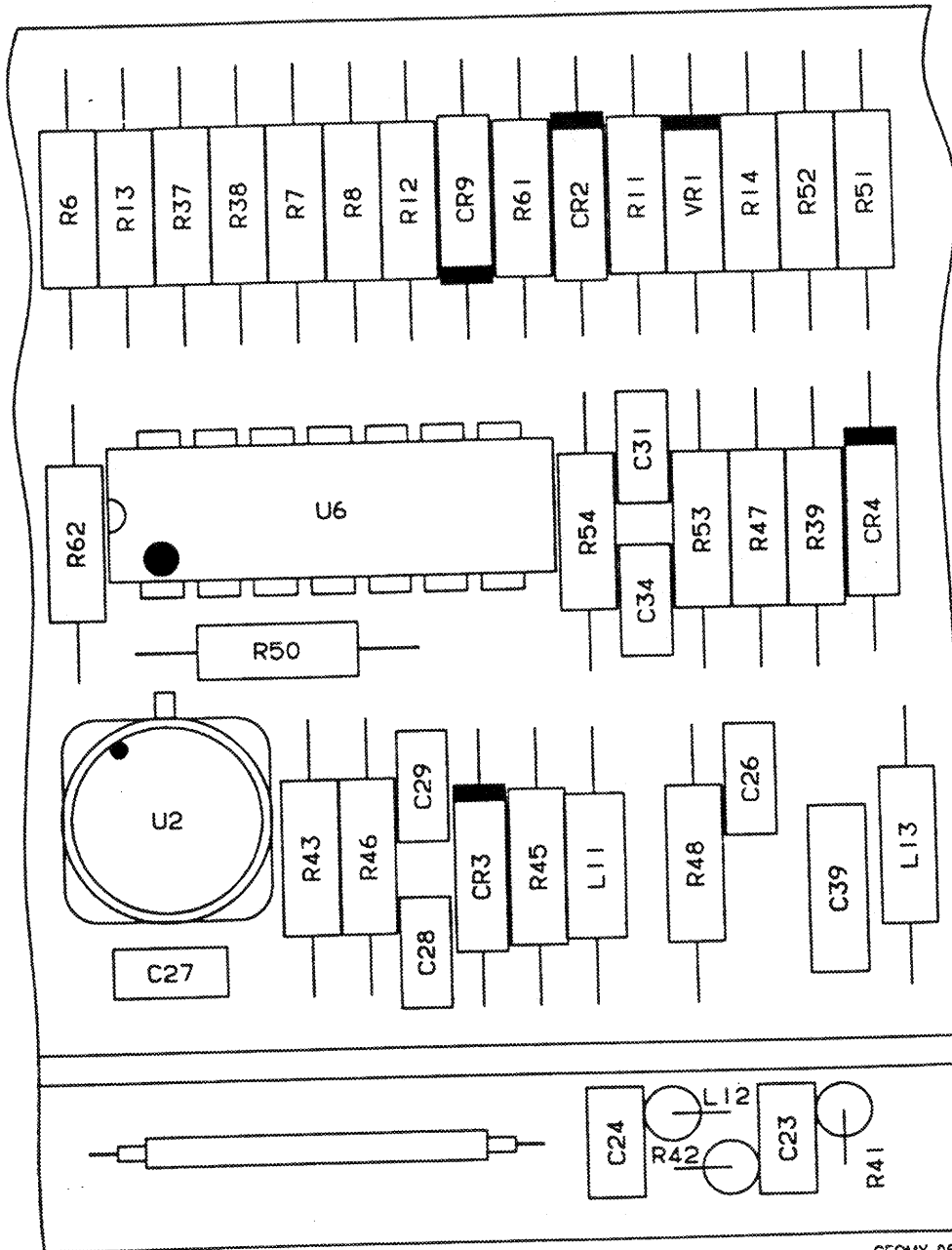
Figure 17. Reference Oscillator CCA A4A1 (A3024621) (Sheet 3 of 6)
