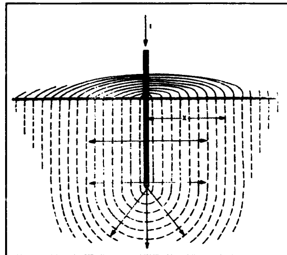
Figure 1 Grounding volume shells about the earth electrode.
