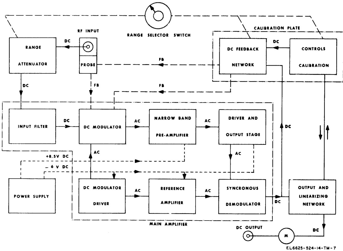
Figure 5-1. Block diagram.
