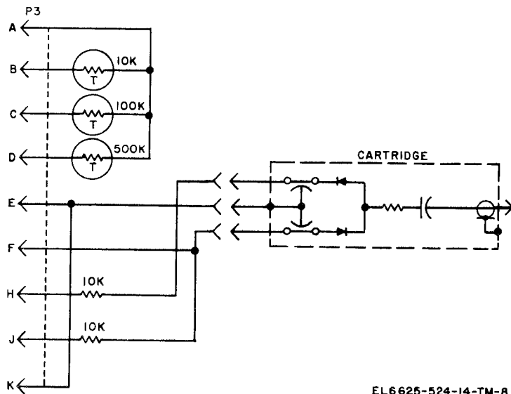
Figure 5-2. Rf probe, simplified schematic diagram.
