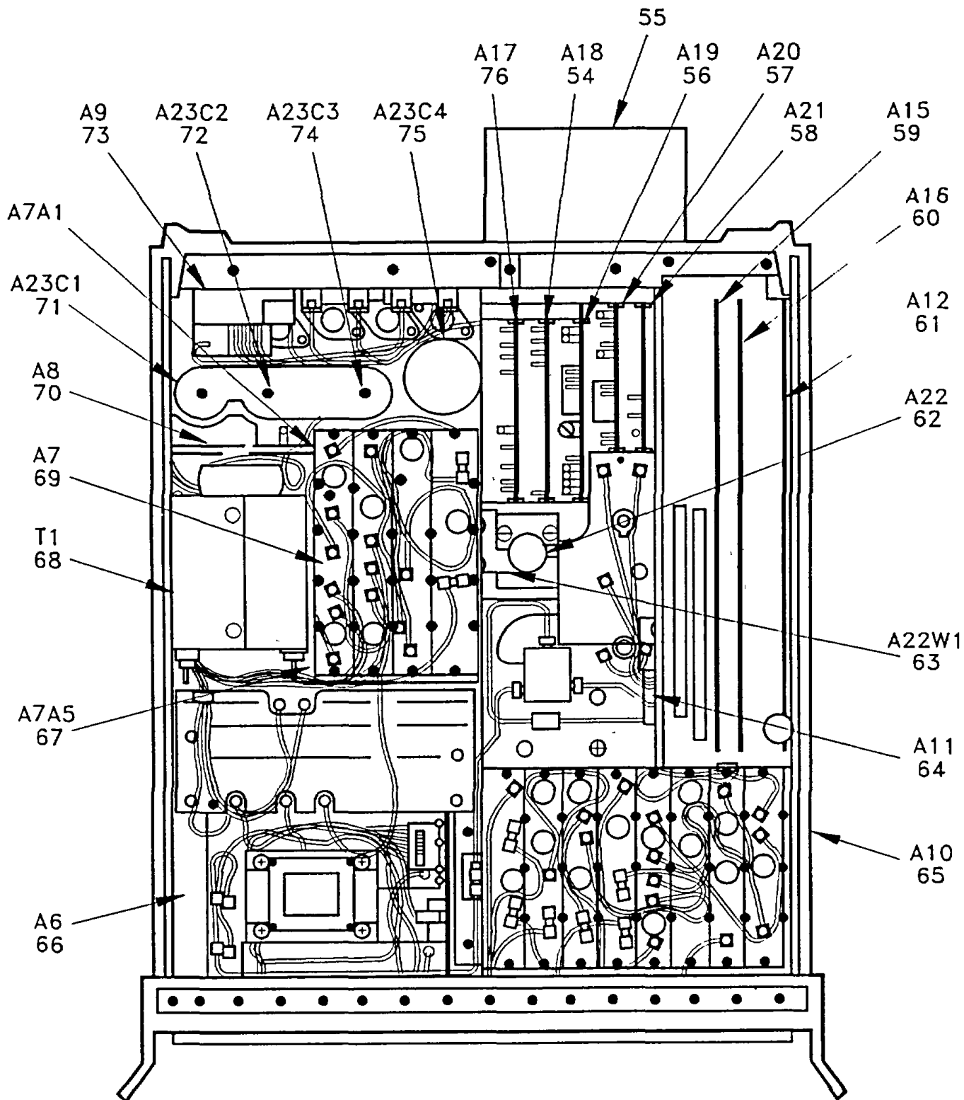
Figure 7. RF Section Top View (Sheet 2 of 2)
