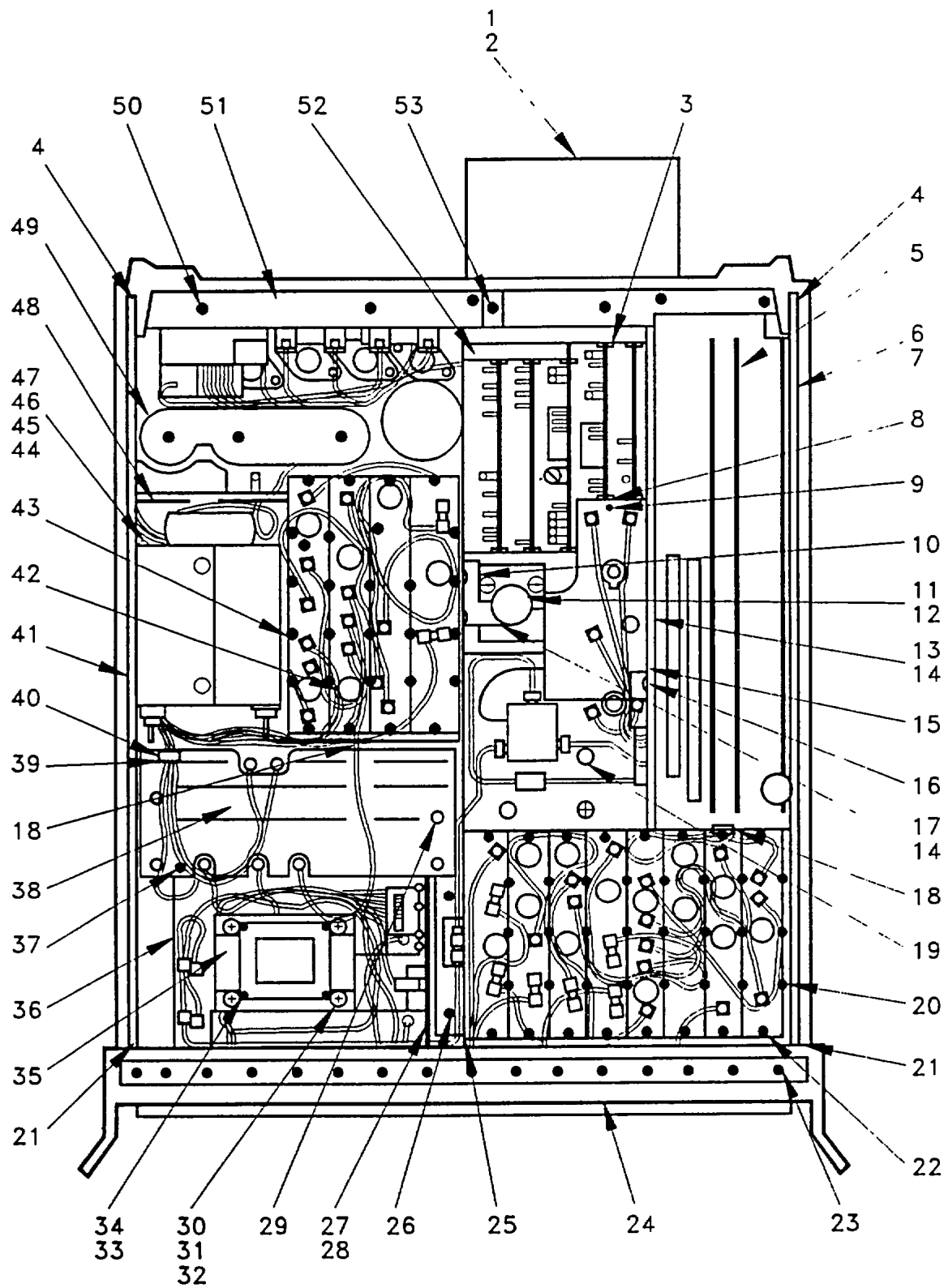
Figure 7. RF Section Top View (Sheet 1 of 2)
