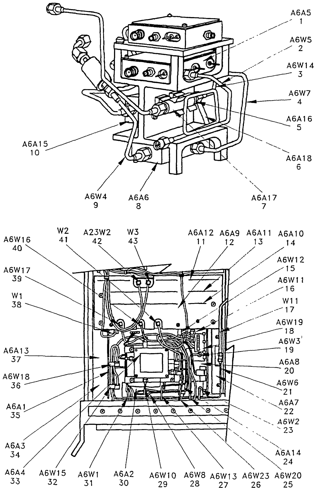
Figure 11. RF Module
