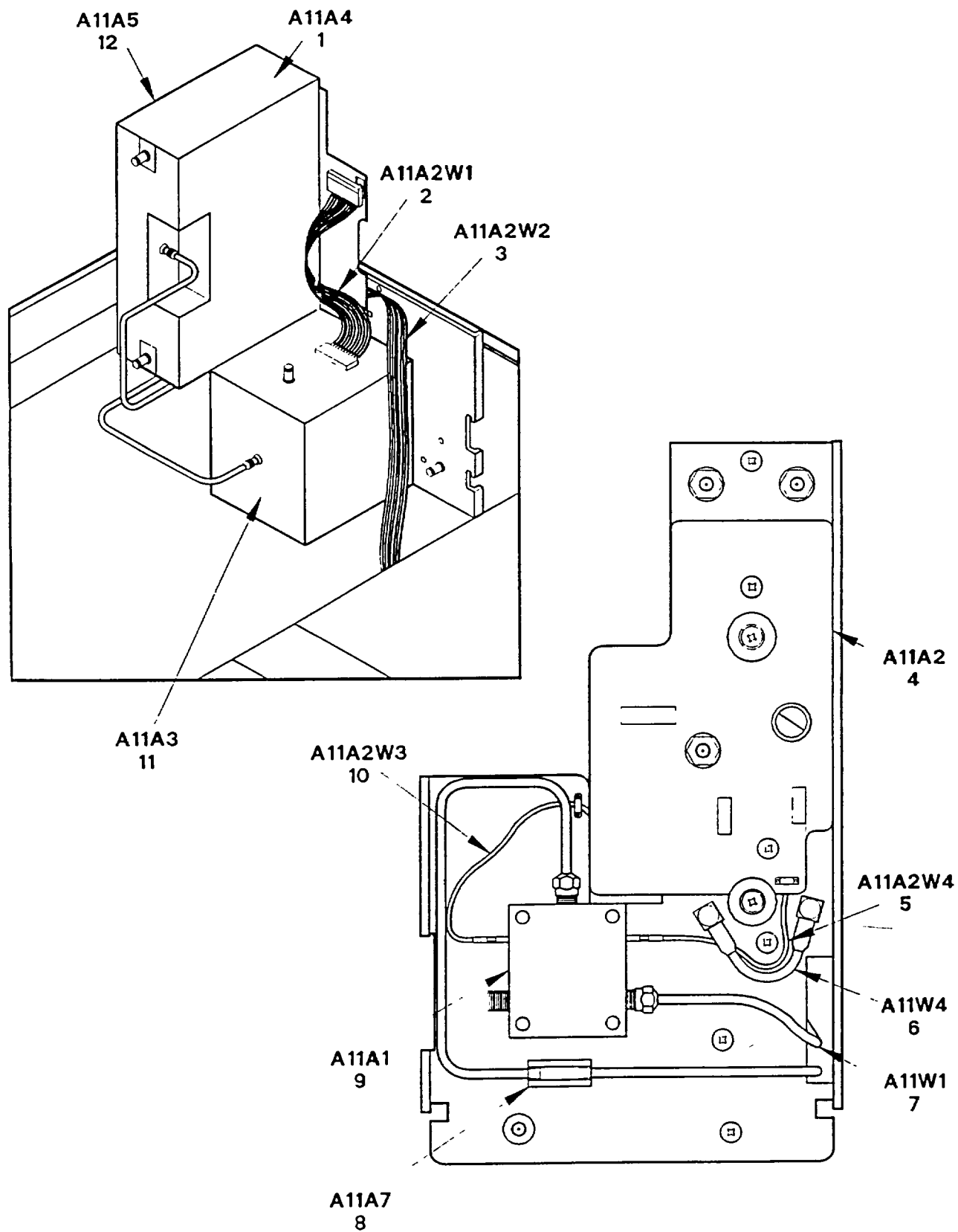
Figure 15. YTO Loop
